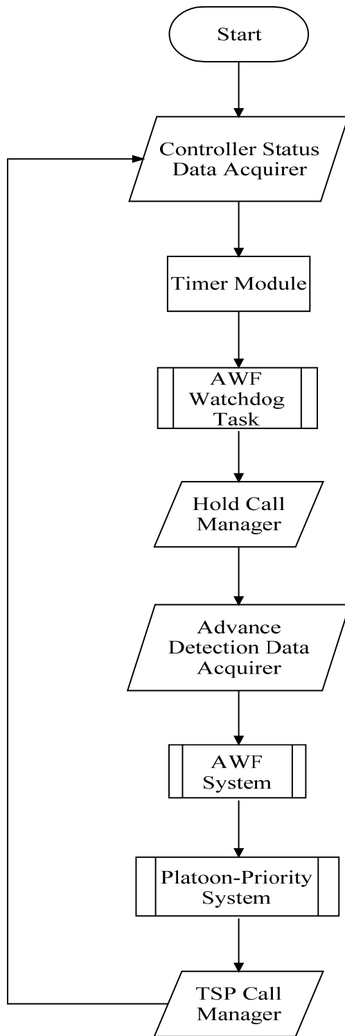
Figure 5-3 Integrated System flowchart
