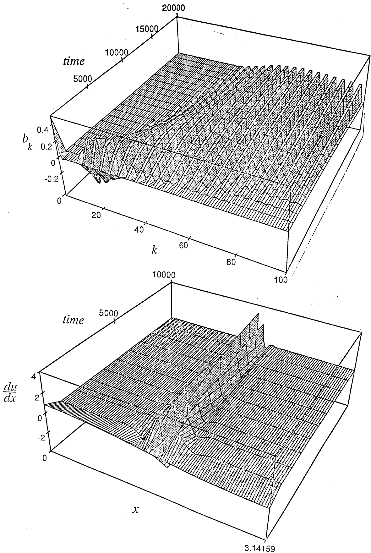
Figure 5. Localization and creation of fine structure. (a) Fourier spectrum of b_k(t) ; (b) u_x in physical space.
