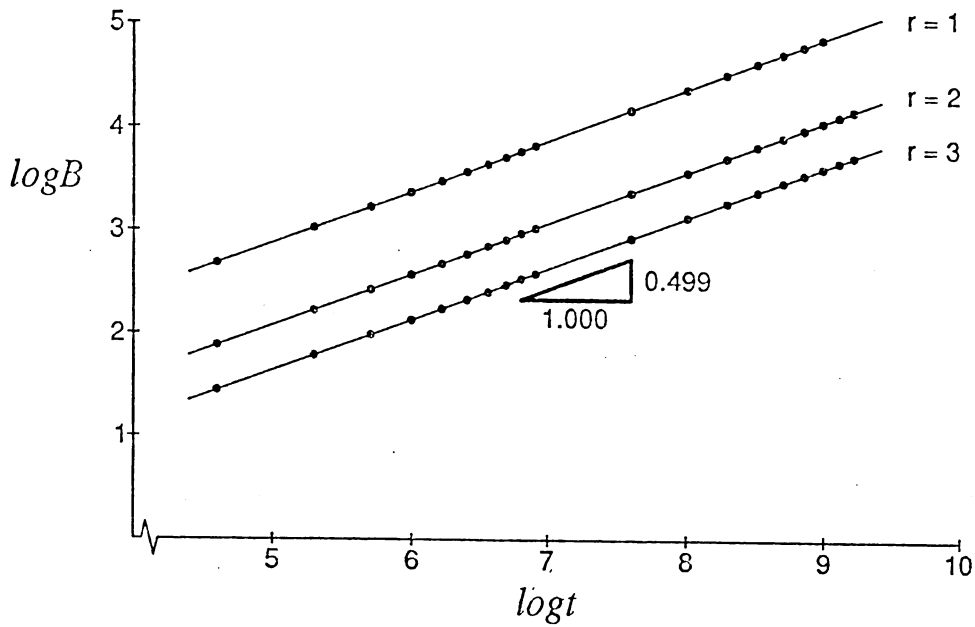
Figure 8. Asymptotic escape of energy for C^{r-1} initial data. (a)
