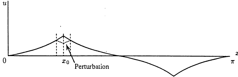
Figure 2 A small \|\cdot\|_\infty perturbation lowers V(u) .
