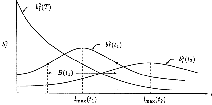
Figure 3 Evolution of modal energies.
