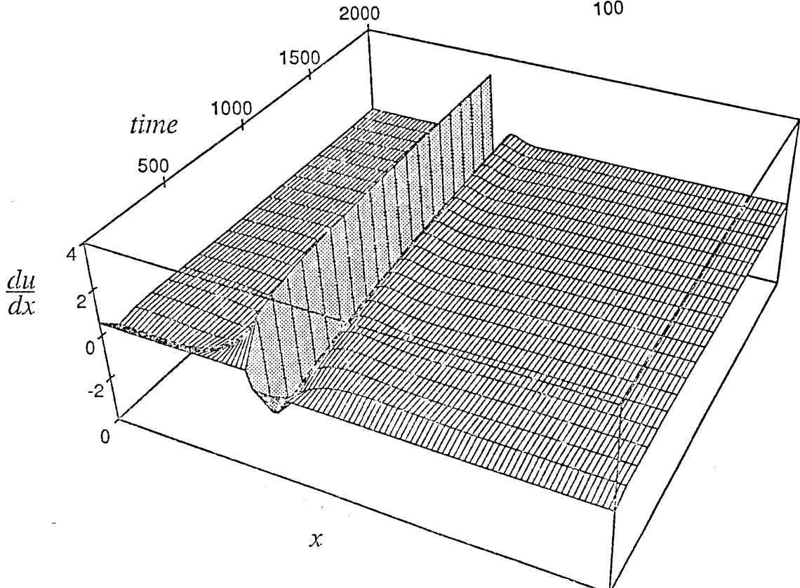
Figure 6. Preservation of a strain discontinuity. (a) Fourier spectrum (first 100 modes), (b) u_x in physical space.
