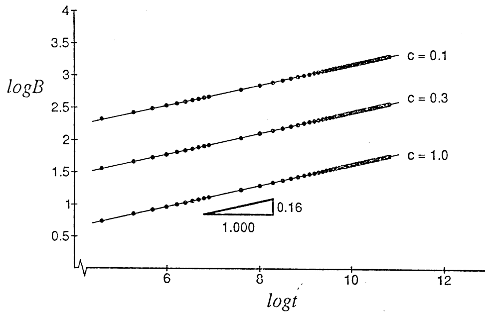
Figure 7. Asymptotic escape of energy for analytic initial data.
