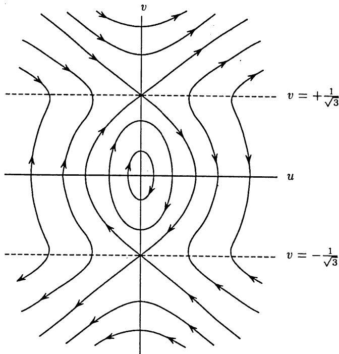
Figure 1 Phase portrait of (2.12)
