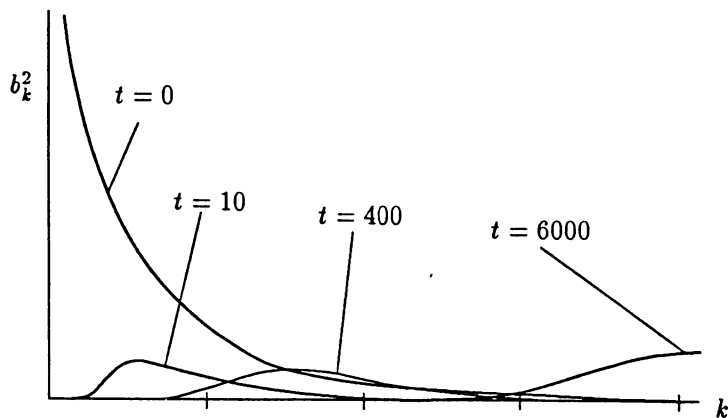
Figure 4 Development of the spectrum b_k^2(t) .
