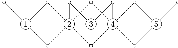
Figure 3.15: Hasse diagram of P_{[3,5]}
