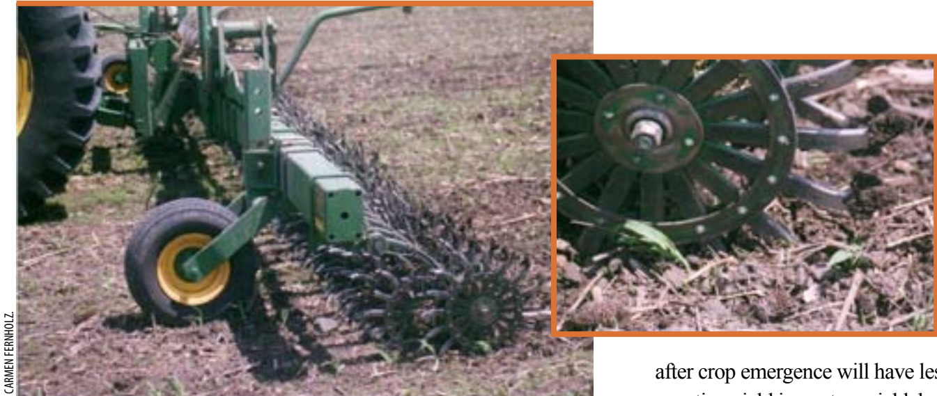
Figure 6-7. The rotary hoe has an operating depth of one inch or more.
