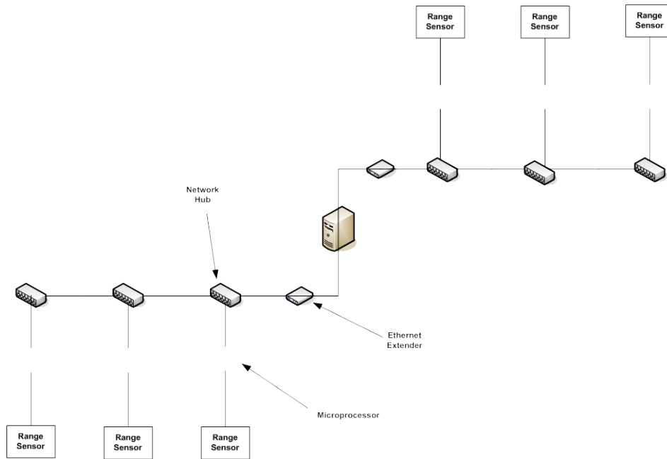
Figure 7: Minimal sensor surveillance system network topology. Daisy chained to reduce construction costs. Ethernet extenders (long distance) and Ethernet hubs (short distance) are employed for network connectivity to the central server. Microprocessors are used to interface with range sensor hardware.
