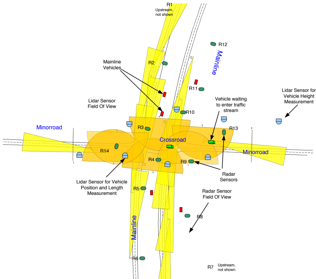
Figure 1: Plan view of a typical instrumented rural four lane expressway intersection. Sensors are radar (yellow triangles indicate field of view and) scanning lidar (orange semicircles); all data is sent from sensor processors to the main central processor.
