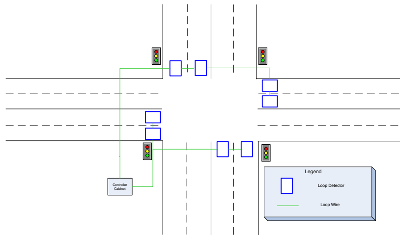
Figure 21: Hardware layout of inductive loop installation of a four leg intersection, two lanes per approach
