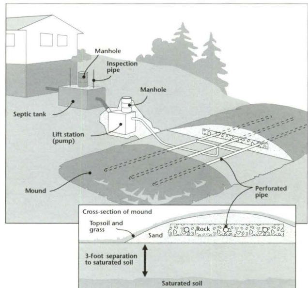
Figure 1. Cross section of a mound system.
