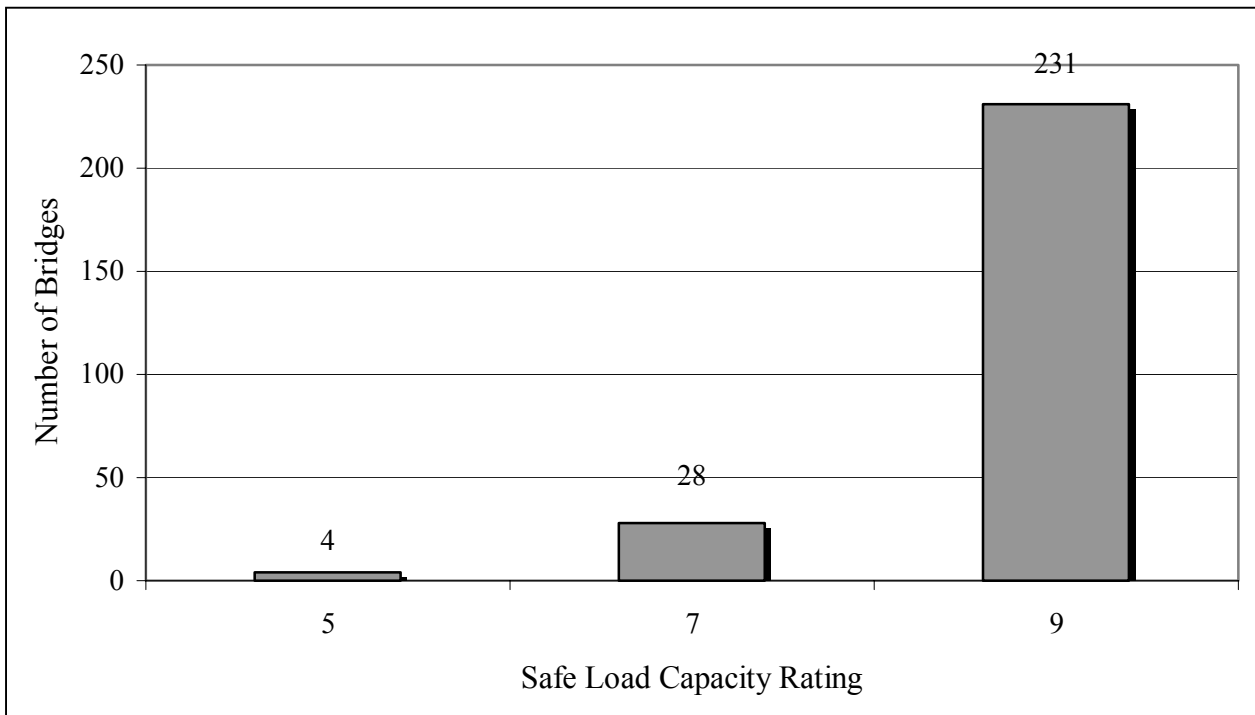
Figure 3.6 Safe load capacity rating
