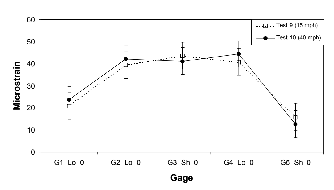
Figure 3.11 Dynamic response of bridge #04006 – Trucks 3 and 4 (measured)
