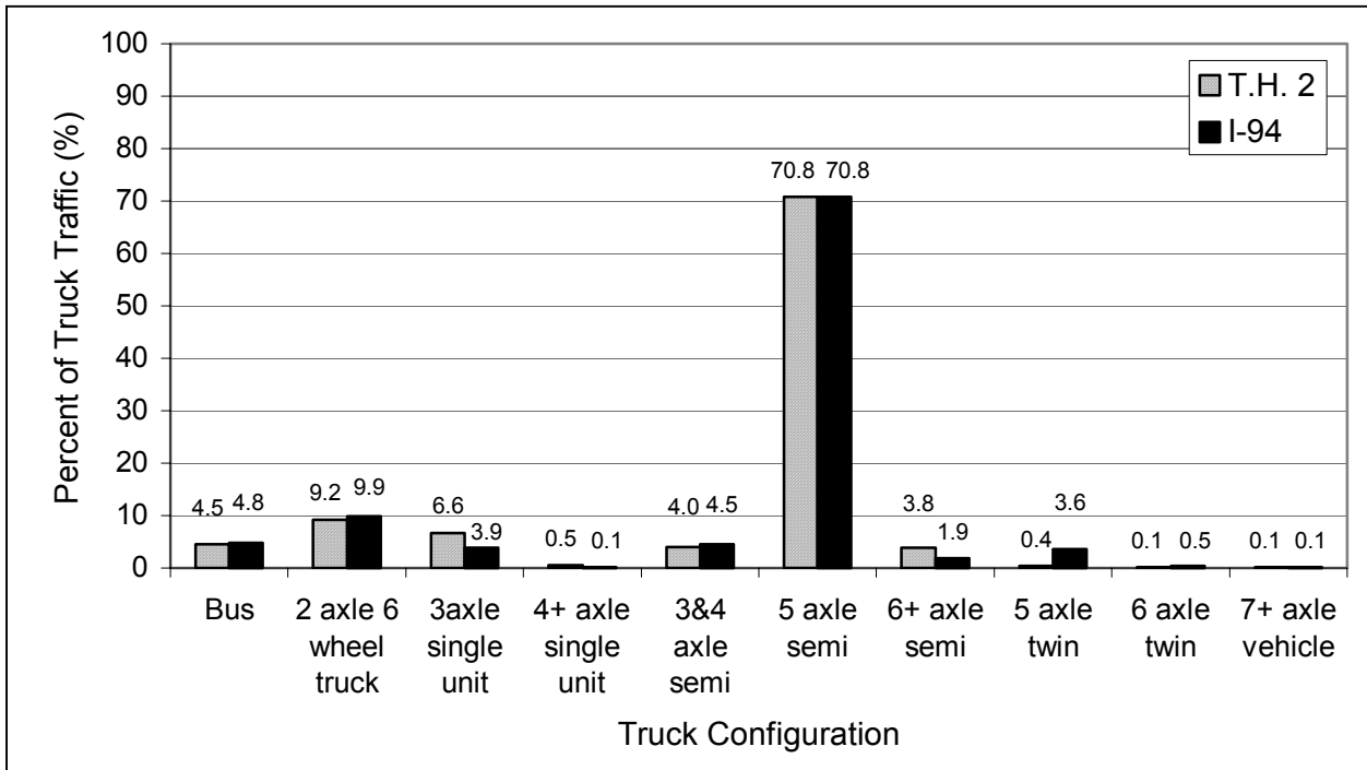
Figure 2.6 Percent of truck traffic by classification on T.H. 2 near Bemidji and I-94 at the Mn/ROAD research site from four months of 1992 WIM data.
