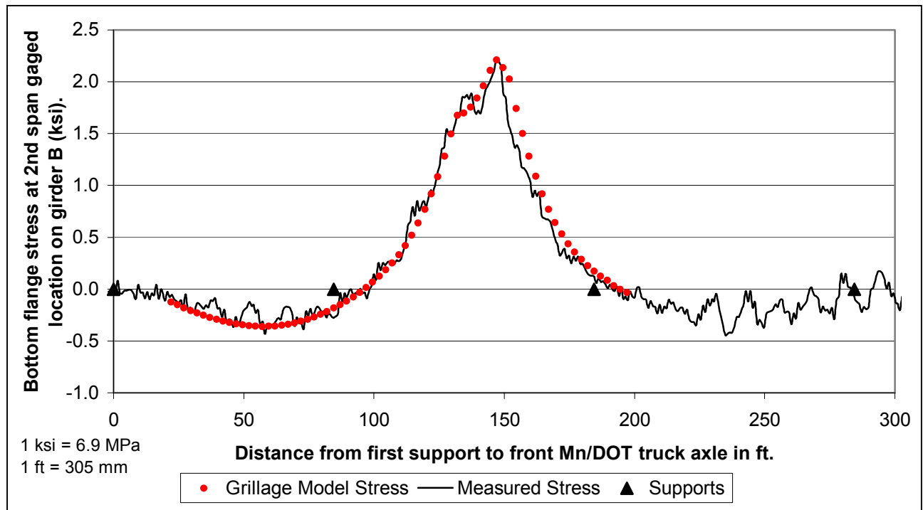
Figure 3.13 Bridge #54004 over the Red River Stress at 2 nd span gaged location vs. Mn/DOT truck position traveling in the westbound lane
