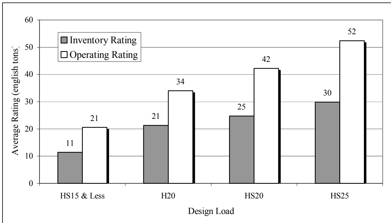
Figure 3.4 Average inventory and operating ratings for different design loads
