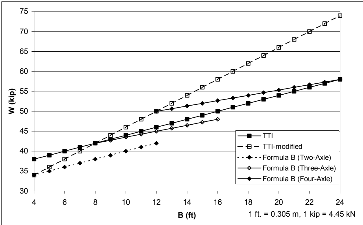
Figure 2.3 Comparison of different axle-group-weight formulas.
