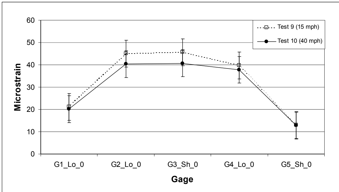
Figure 3.10 Dynamic response of bridge #04006 – Trucks 1 and 2 (measured)
