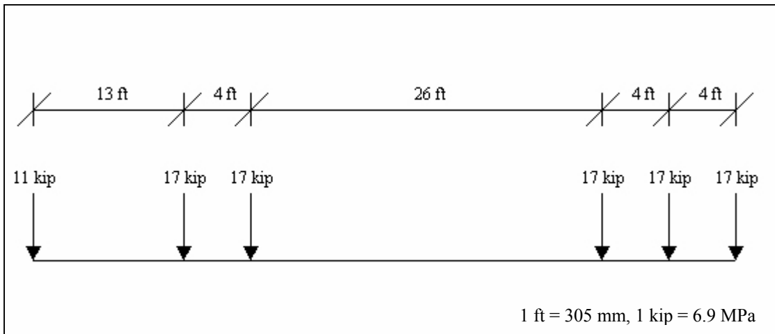
Figure 2.4 Canadian legal truck configuration.
