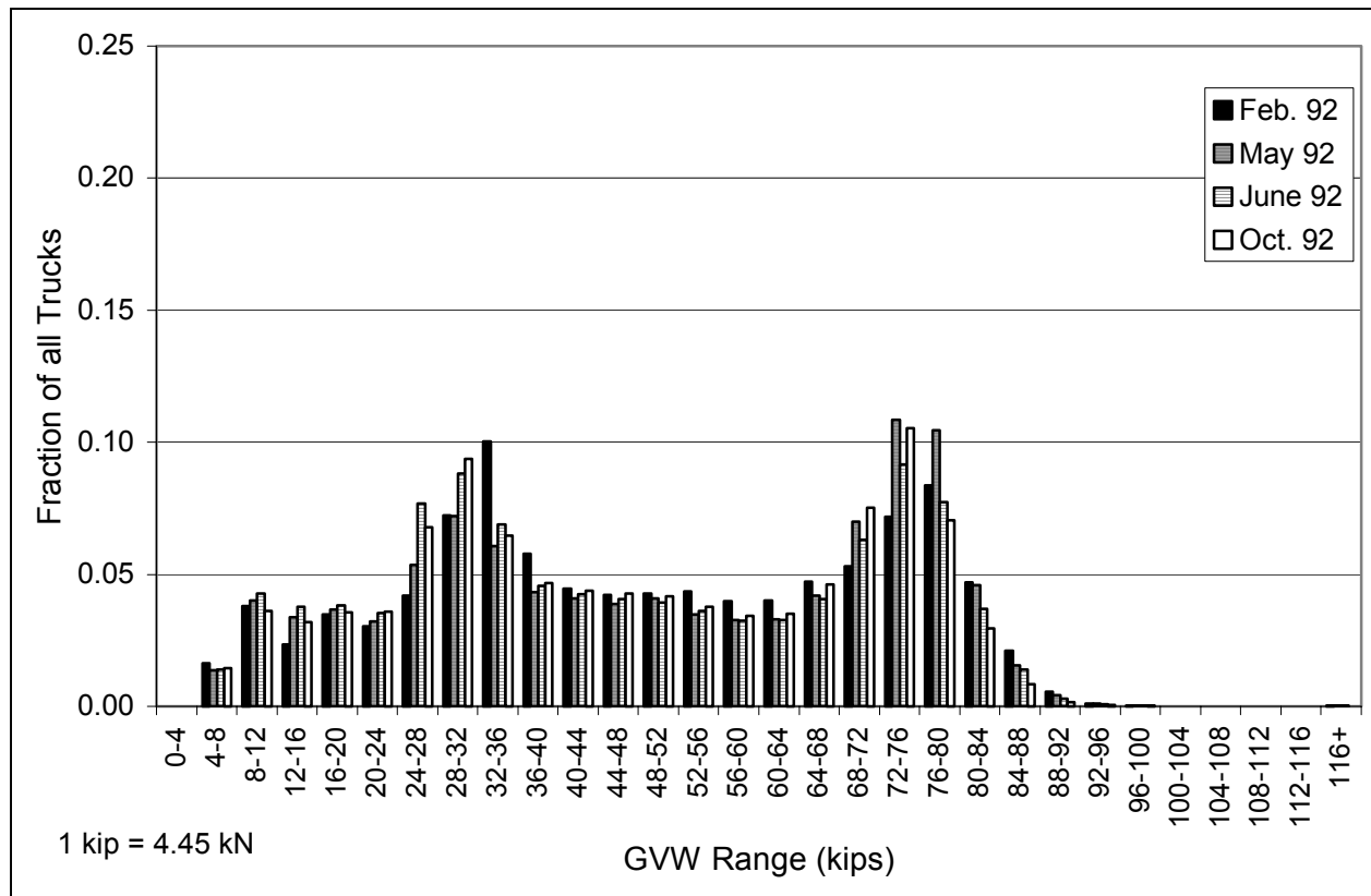
Figure 2.9 GVW histogram by month for westbound I-94 traffic for 1992 data.
