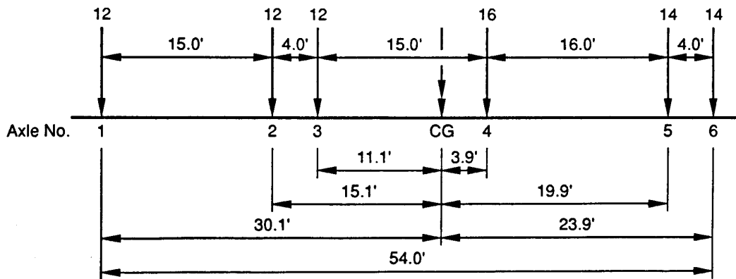
Figure 2.2 Example of rating vehicles that meet Formula B.
