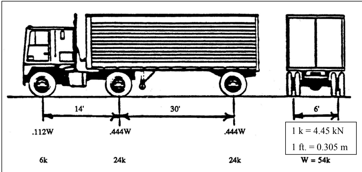
Figure 2.5 Fatigue truck. (Moses et al. 1987)
