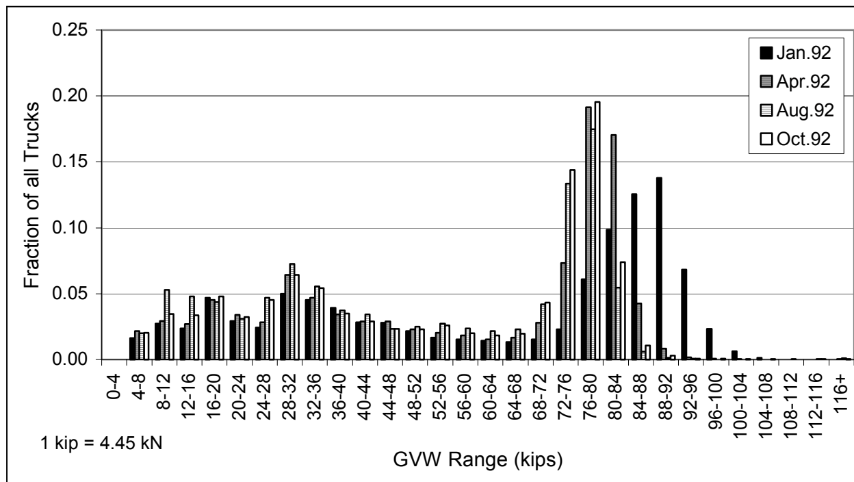
Figure 2.8 GVW histogram by month for eastbound T.H. 2 traffic for 1992 data.
