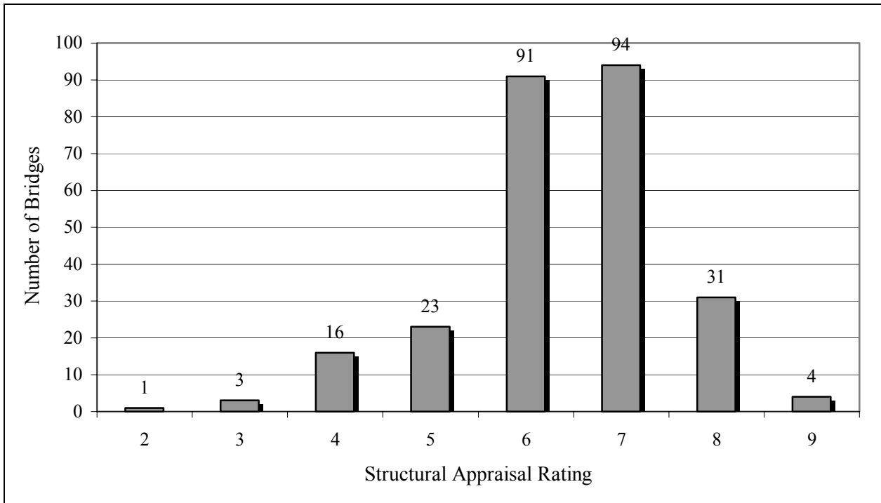
Figure 3.5 Structural valuation appraisal rating for bridges on the selected routes
