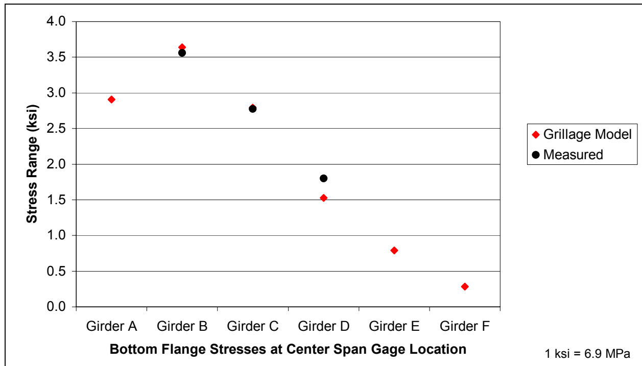
Figure 3.14 Bridge #9276, grillage analysis model and measured results for a Mn/DOT truck in the left lane
