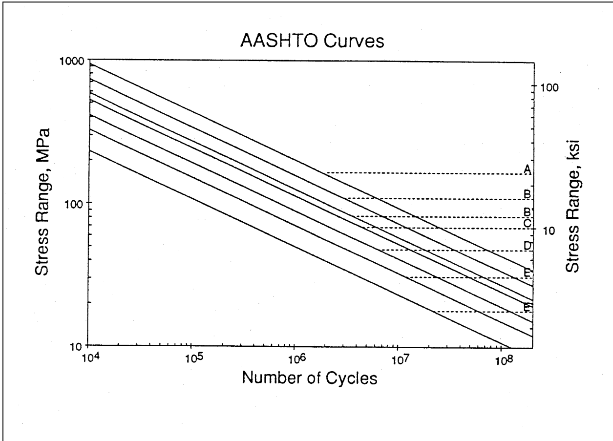
Figure 2.1 AASHTO S-N curves.
