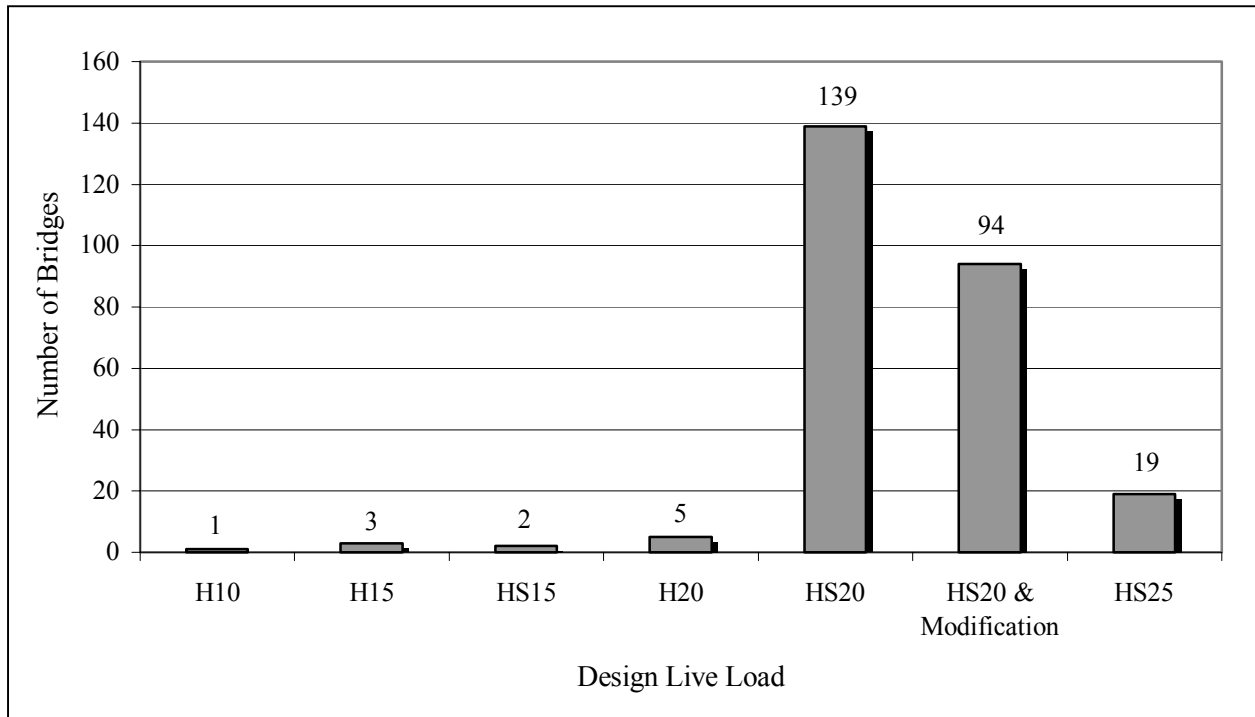
Figure 3.3 Number of bridges on the three selected routes for each design live load level
