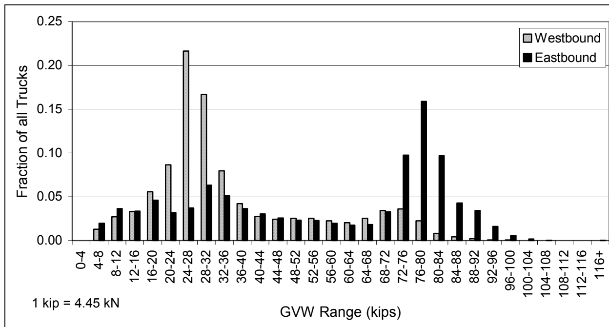
Figure 2.7 GVW histogram for T.H. 2 near Bemidji for 1992 data (from Jan., Apr., Aug, and Oct.).
