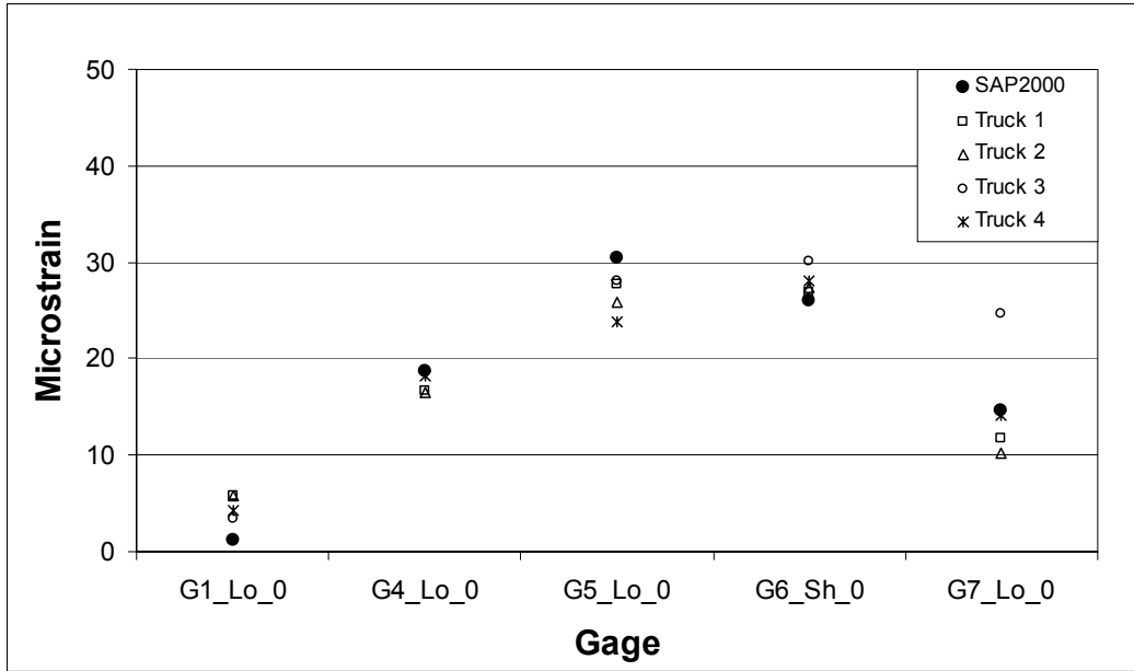
Figure 3.12 Bridge #9731 – Bottom fiber strains for Test 3 (test truck in lane 2)
