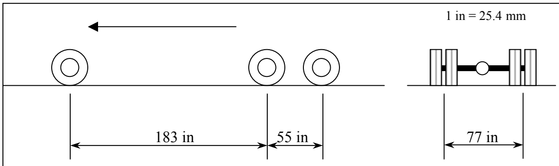
Figure 3.8 Average axle spacing of test trucks
