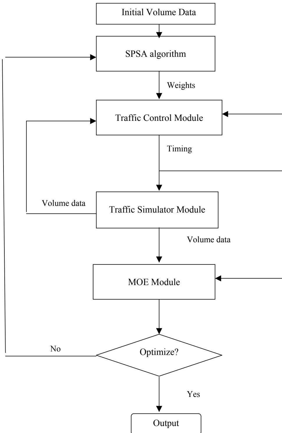
Fig. 4.3 Flow chart for the implementation of the NN-based SPSA algorithm
