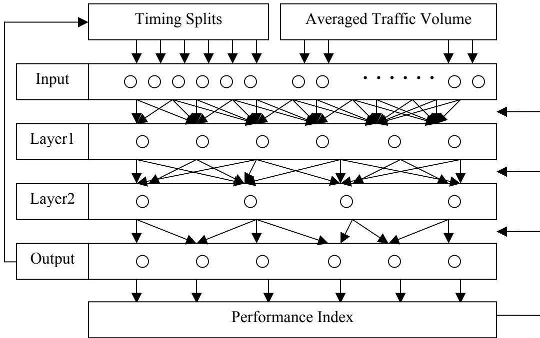
Fig. 4.2 The neural network controller's internal structure.
