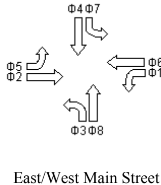
Fig. 5.1 NEMA phase numbering convention for east/west arterial.
