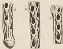
Fig. 10, Helopora quadrata ULRICH. Galena shales, near Cannon Falls, Minnesota. a , basal part of a segment; b , the central portion of another, and c , the upper extremity of a third, all x 18.
