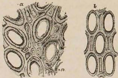
FIG. 9. Escharopora (?) limitaris ULRICH. a , small part of tangential section, x50, showing structure immediately beneath the point of bifurcation; b , another portion of same where the zoöcial margins are parallel.
