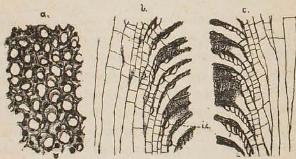
Fig. 12. Homotrypella mundula Ulrich, Galena shales, Decorah, Iowa. a, tangential section; b and c, opposite sides of a vertical section, showing differences in the number of cystiphragms; all x 18.
