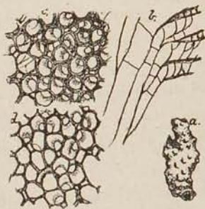
FIG. 14 Homotrypa tuberculata , n. sp. , upper third Trenton shales, near Cannon Falls, Minnesota. Collection of E. O. Ulrich. a , fragment of the natural size; b , small portion of a vertical section, x 18, showing two mesopores, the cystiphragms and diaphragms of the peripheral region, all of which are wanting in the axial region; c and d , two portions of a tangential section of a fully matured example, x 18, the former showing appearance immediately beneath the surface, the latter at a slightly deeper level.
