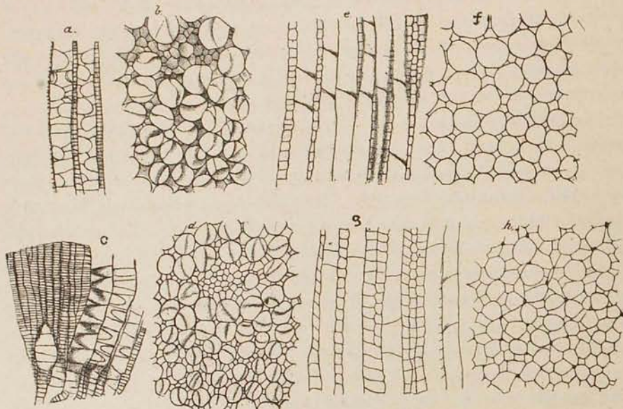
FIG. 15. a and b , vertical and transverse sections of Prasopora selwyni Nicholson, Trenton limestone, Ottawa, Canada; c and d , similar sections of Prasopora oculata Foord, Galena shales, near Cannon Falls, Minnesota; e and f similar sections of Mesotrypa quebecensis Ami, sp., Trenton limestone, Little Falls, N. Y.; g and h , similar sections of Mesotrypa whiteavesi Nicholson, sp., Trenton limestone, Ottawa, Can. All the figures are x18.
