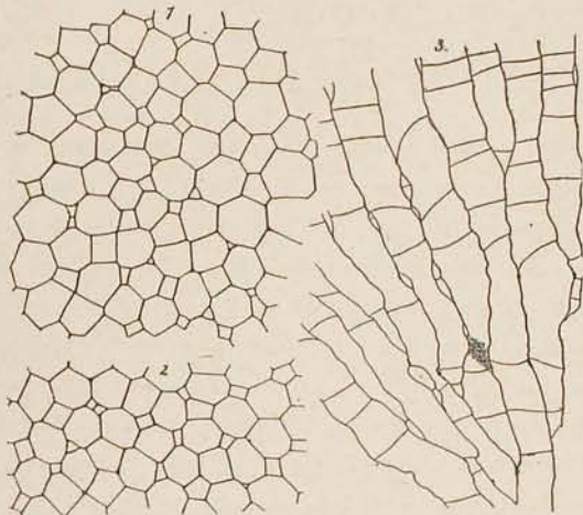
FIG. 19. Diplotrypa neglecta Ulrich, base of Galena limestone, Hader, Goodhue county, Minnesota. Collection of E. O. Ulrich. 1 and 2, two tangential sections, x 18, and 3, a vertical section, similarly enlarged.
