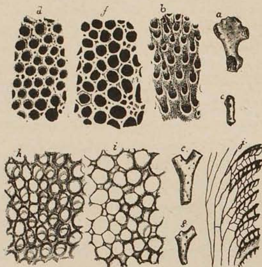
FIG. 13. Homotrypa (?) intercalaris , n. sp. , middle Trenton shales, Minneapolis, Minnesota. Collection of E. O. Ulrich. a and b , a specimen of the natural size, and small portion of its surface \times 18 , showing unusually oblique zoecial apertures; c and d , similar views of a fragment of a form doubtfully referred to this species, having somewhat smaller zoecia and mural papillae; e and f , similar views of a typical example; g , more slender fragment, natural size; h , tangential section, \times 18 , showing structure immediately beneath surface of fully matured example; i , another portion of same section, showing structure at a deeper level; j , vertical section, \times 18 , showing the peripheral region with the mesopores and cystiphragms, and a small part of the untabulated axial region.
