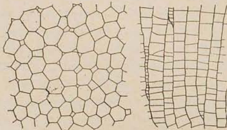
FIG. 18. Diplotrypa limitaris Ulrich, upper beds of the Galena shales, Goodhue county, Minnesota. Collection of E. O. Ulrich. Transverse and vertical sections, \times 18 , showing the tabulation of the tubes and the great reduction in the number of mesopores characterizing the species.
