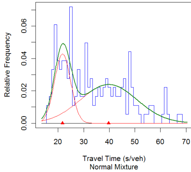
Figure A-24 Travel Time Relative Frequency Plot of Site 53
