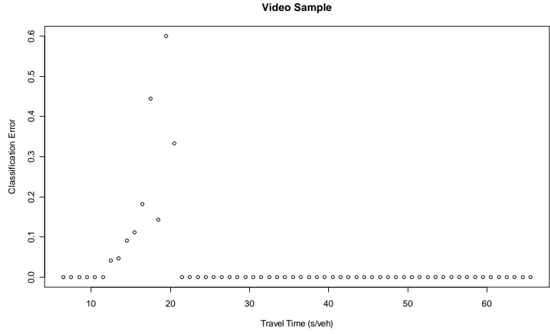
Figure 3-7 Classification Error Plot of Non-stopping Vehicles
