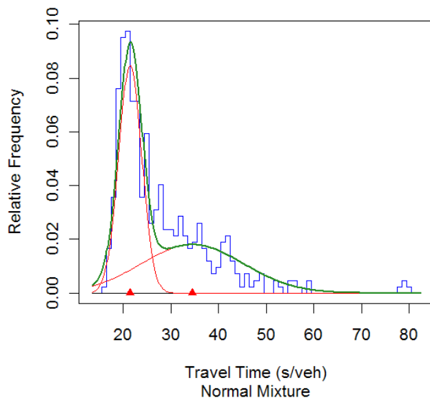
Figure A-54 Travel Time Relative Frequency Plot of Site 148
