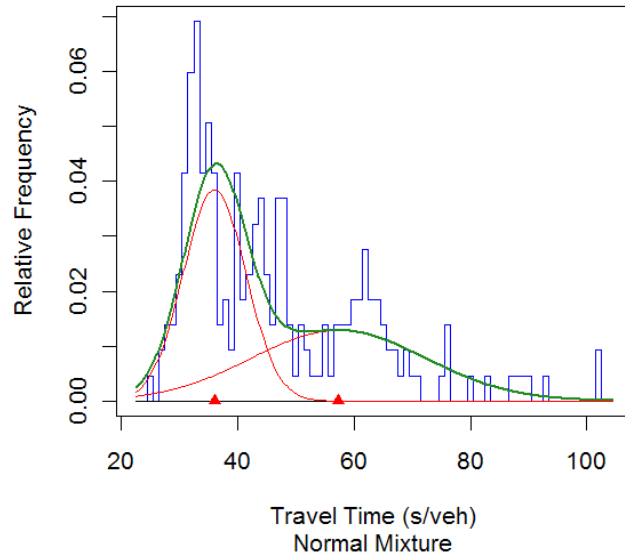
Figure A-37 Travel Time Relative Frequency Plot of Site 83
