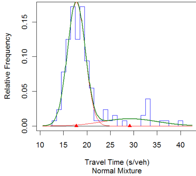
Figure A-23 Travel Time Relative Frequency Plot of Site 52
