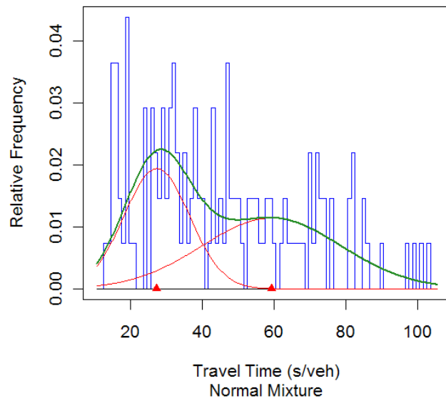
Figure A-22 Travel Time Relative Frequency Plot of Site 51
