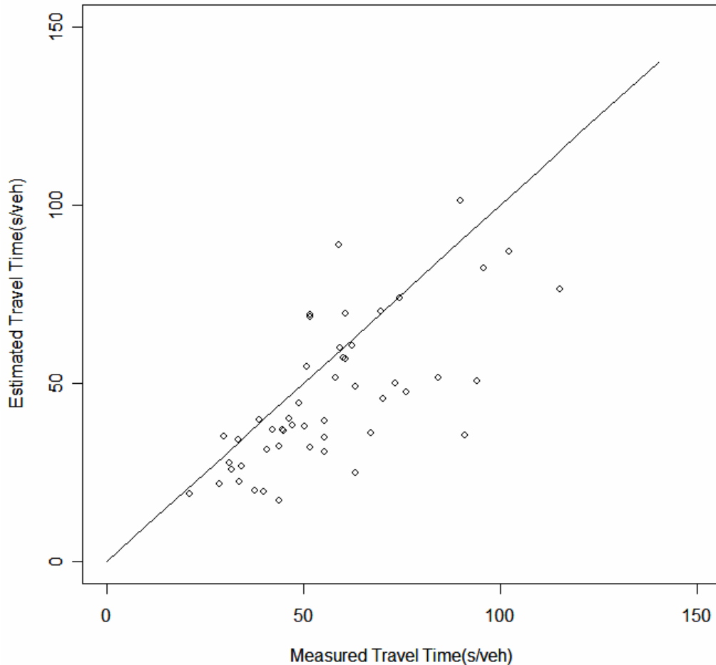
Figure 5-2 Measured Travel Time vs Estimated Travel Time (Conical Volume-Delay Function)
