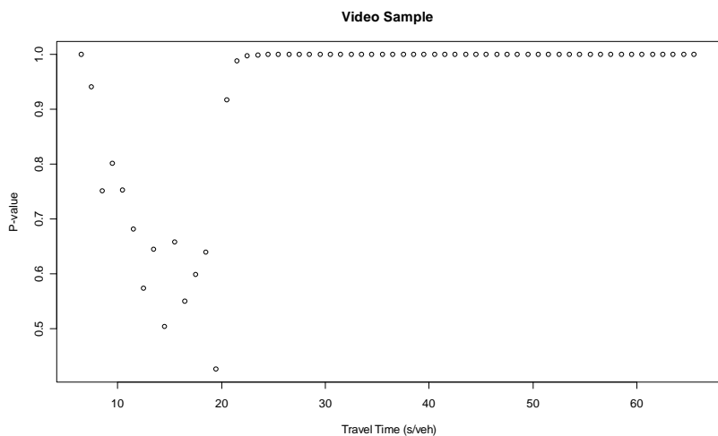
Figure 3-8 Classification P-value Plot of Non-stopping Vehicles
