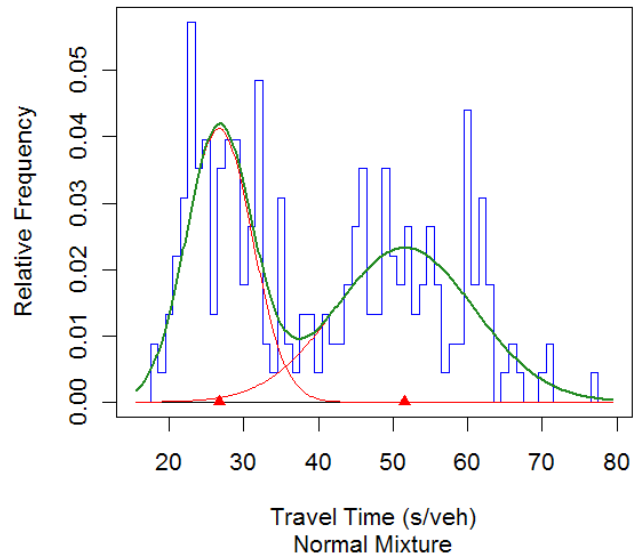
Figure A-44 Travel Time Relative Frequency Plot of Site 100
