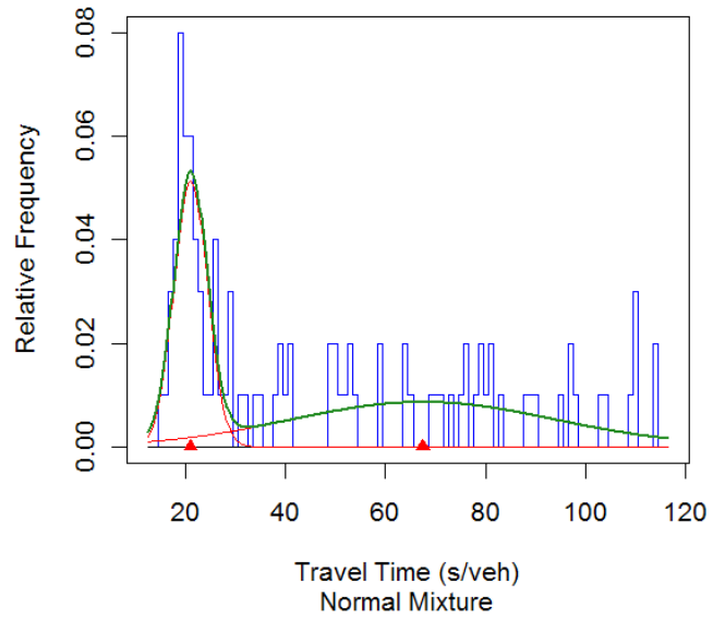
Figure A-21 Travel Time Relative Frequency Plot of Site 50
