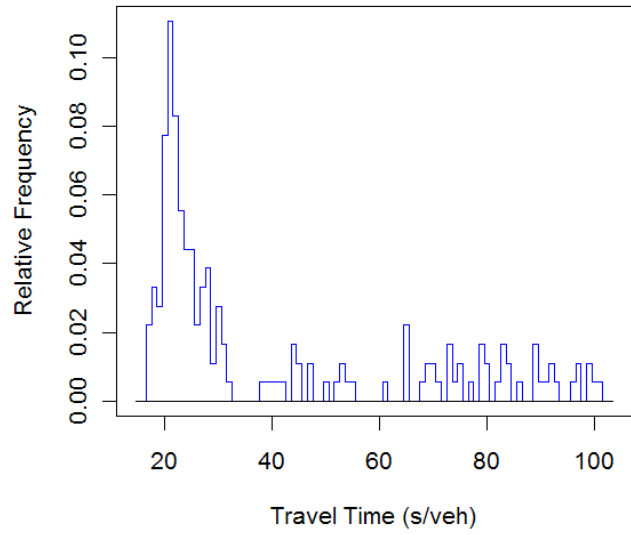
Figure A-41 Travel Time Relative Frequency Plot of Site 96
