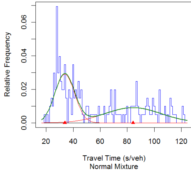
Figure A-17 Travel Time Relative Frequency Plot of Site 38
