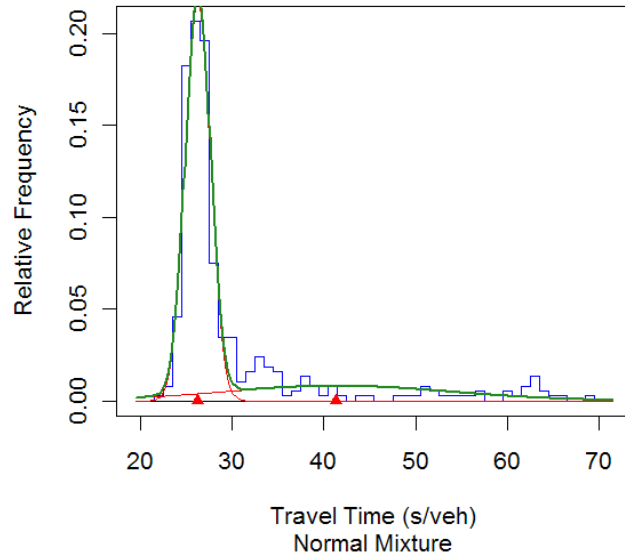
Figure A-13 Travel Time Relative Frequency Plot of Site 33
