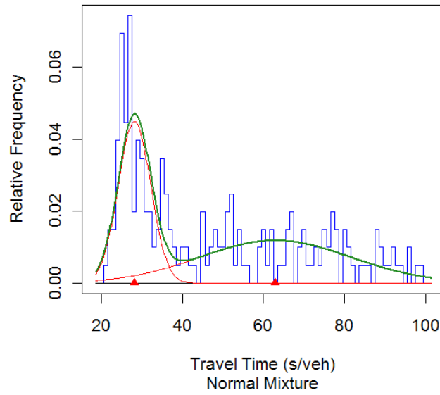
Figure A-26 Travel Time Relative Frequency Plot of Site 55
