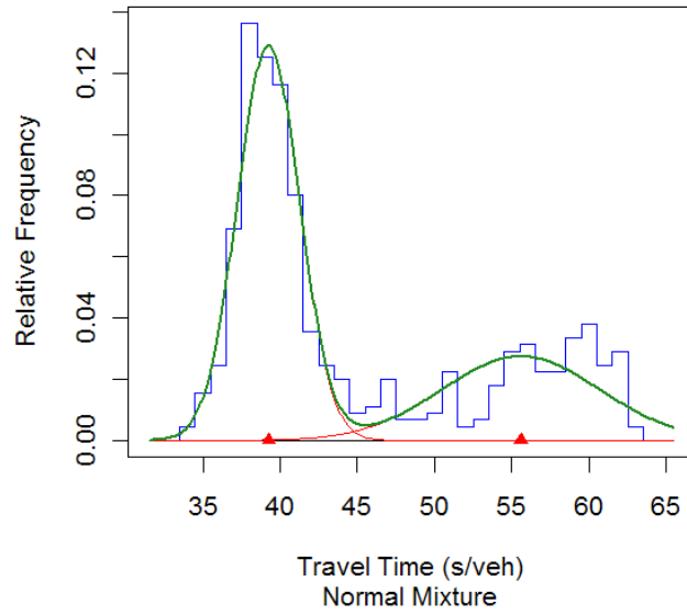
Figure A-43 Travel Time Relative Frequency Plot of Site 98
