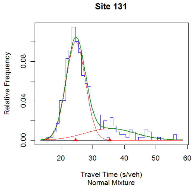
Figure A-49 Travel Time Relative Frequency Plot of Site 131
