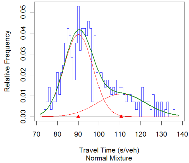
Figure A-55 Travel Time Relative Frequency Plot of Site 149
