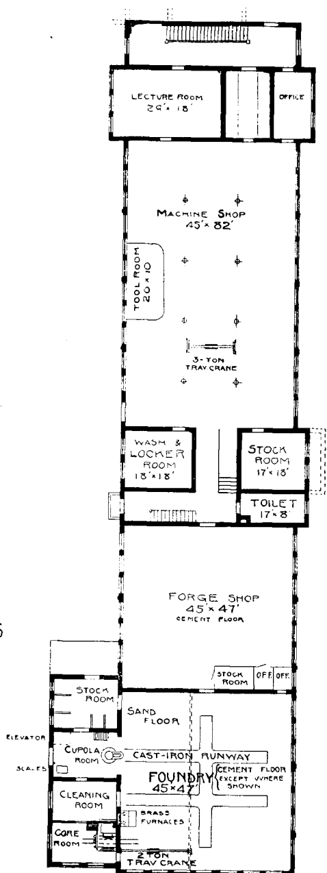
PLAN OF NEW SHOPS FOR THE UNIVERSITY OF MINNESOTA
