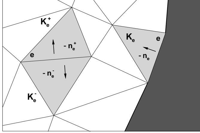
FIGURE 1. A representation of the lifting \mathbf{q}_{h,m} when \mathbf{m} = \chi_e for interior and boundary edges e . In this case, we have taken d = 0 and c = Id .
