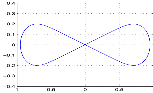
Figure 9: The L^2 Spectrum of the classical double layer potential operator for the Laplacian on a sector of angle \frac{\pi}{5} .
