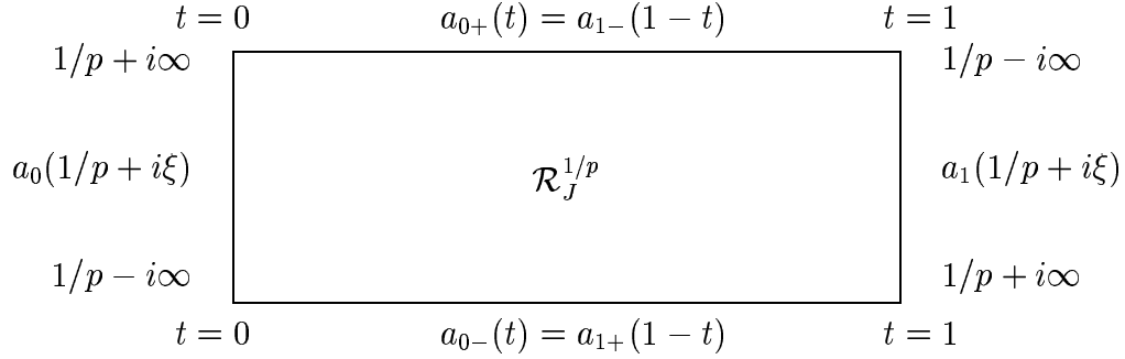
Figure 11: The symbol of the operator A .
