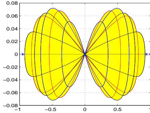
Figure 3: The L^6 Spectrum of the elastostatic (pseudostress) double layer potential operator on glass for a curvilinear triangle of angles \frac{\pi}{6} , \frac{\pi}{3} and \frac{\pi}{2} .
