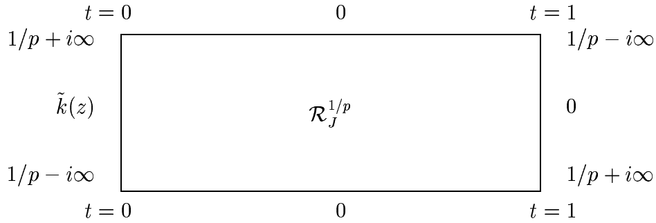
Figure 12: The symbol of a Hardy kernel operator.
