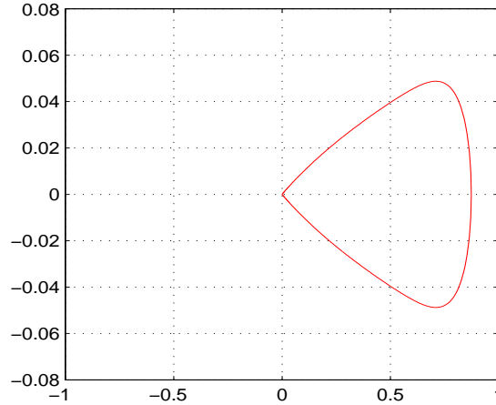
Figure 5: The curve \Sigma_+^+(\pi/4, 6) corresponding to a glass material.
