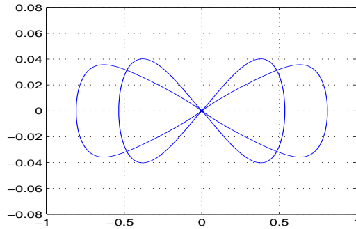
Figure 2: \Sigma_{\pi/3}(10) - or the L^{10} Spectrum of the elastostatic (pseudostress) double layer potential operator on glass for a sector of angle \frac{\pi}{3} .
