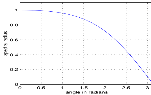
Figure 10: The L^2 Spectral radius of the elastostatic (pseudostress) double layer potential operator on glass versus the opening of the sector.
