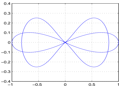
Figure 8: The L^2 Spectrum of the hydrostatic (stress) double layer potential for a sector of angle \frac{\pi}{5} .
