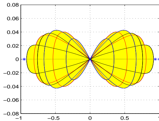
Figure 4: The L^{10} Spectrum of the elastostatic (pseudostress) double layer potential operator on glass for a curvilinear triangle of angles \frac{\pi}{6} , \frac{\pi}{3} and \frac{\pi}{2} .
