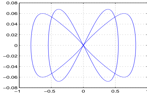
Figure 1: \Sigma_{\pi/3}(6) - or the L^6 Spectrum of the elastostatic (pseudostress) double layer potential operator on glass for a sector of angle \frac{\pi}{3} .
