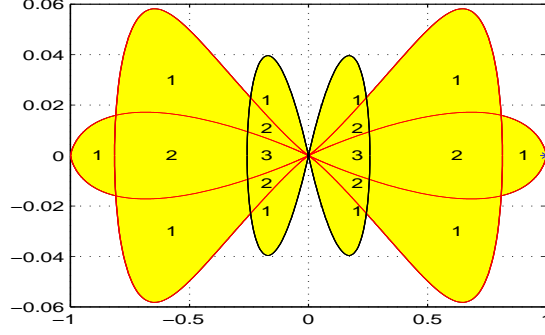
Figure 14: The L^6 Spectrum of the hydrostatic (stress) double layer potential operator on glass for a curvilinear polygon of angles \frac{\pi}{10} and \frac{5\pi}{6} .
