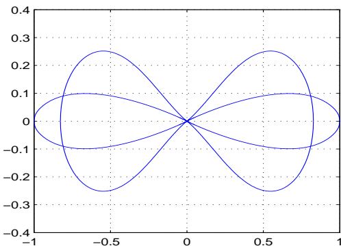
Figure 7: The L^2 Spectrum of the elastostatic (pseudostress) double layer potential operator on rubber for a sector of angle \frac{\pi}{5} .
