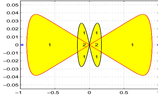
Figure 15: The L^6 Spectrum of the classical double layer potential operator for the Laplacian on glass for a curvilinear polygon of angles \frac{\pi}{10} and \frac{5\pi}{6} .
