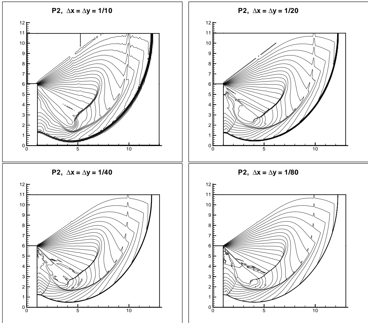
Figure 4.10: Shock diffraction problem. Third order P^2 results. Density \rho . 20 equally spaced contour lines from \rho = 0.066227 to \rho = 7.0668 . Mesh refinement study. From top to bottom: \Delta x = \Delta y = \frac{1}{10} , \frac{1}{20} , \frac{1}{40} , and \frac{1}{80} .
