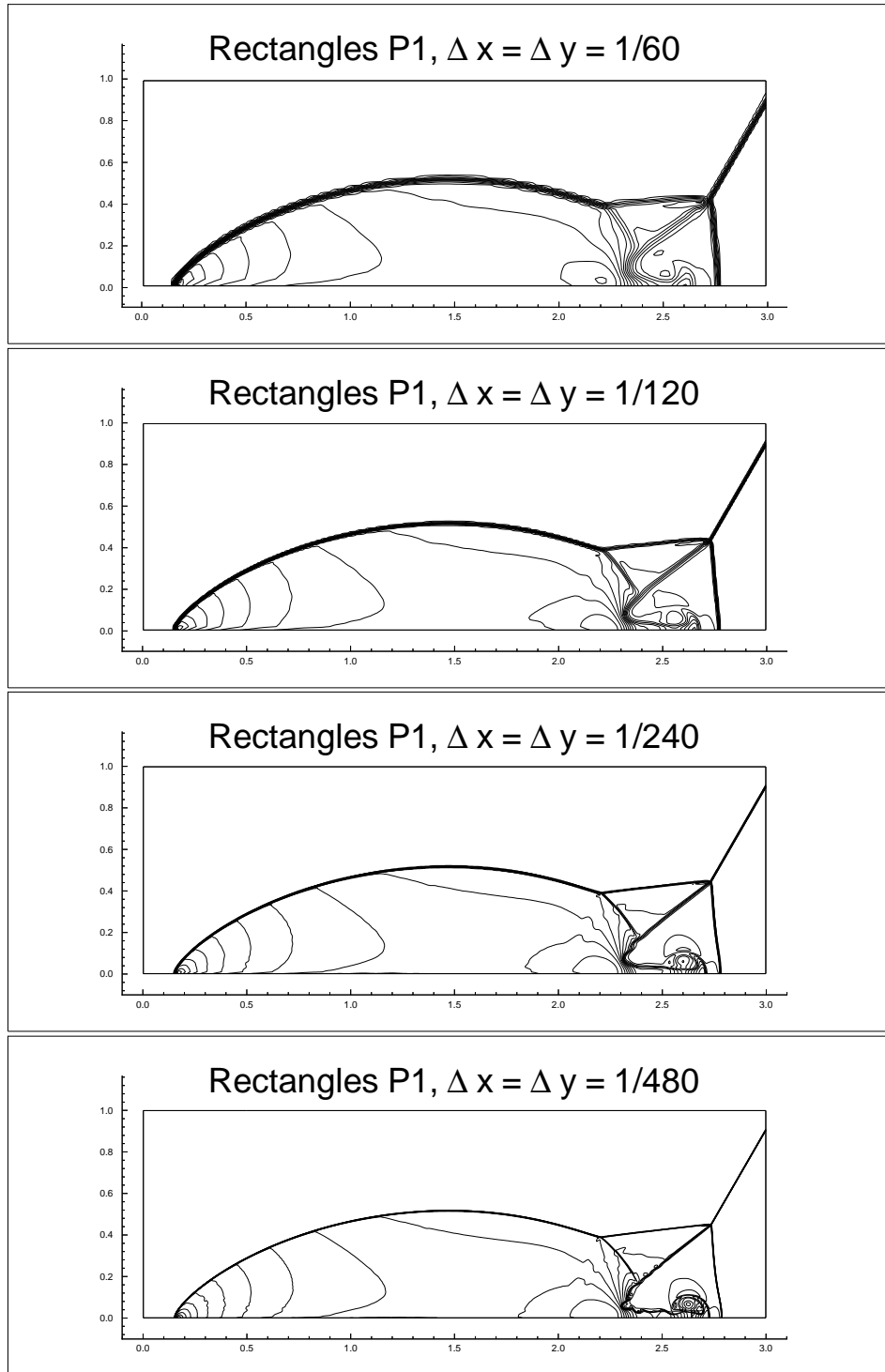
Figure 4.1: Double Mach reflection problem. Second order P^1 results. Density \rho . 30 equally spaced contour lines from \rho = 1.3965 to \rho = 22.682 . Mesh refinement study. From top to bottom: \Delta x = \Delta y = \frac{1}{60} , \frac{1}{120} , \frac{1}{240} , and \frac{1}{480} .
