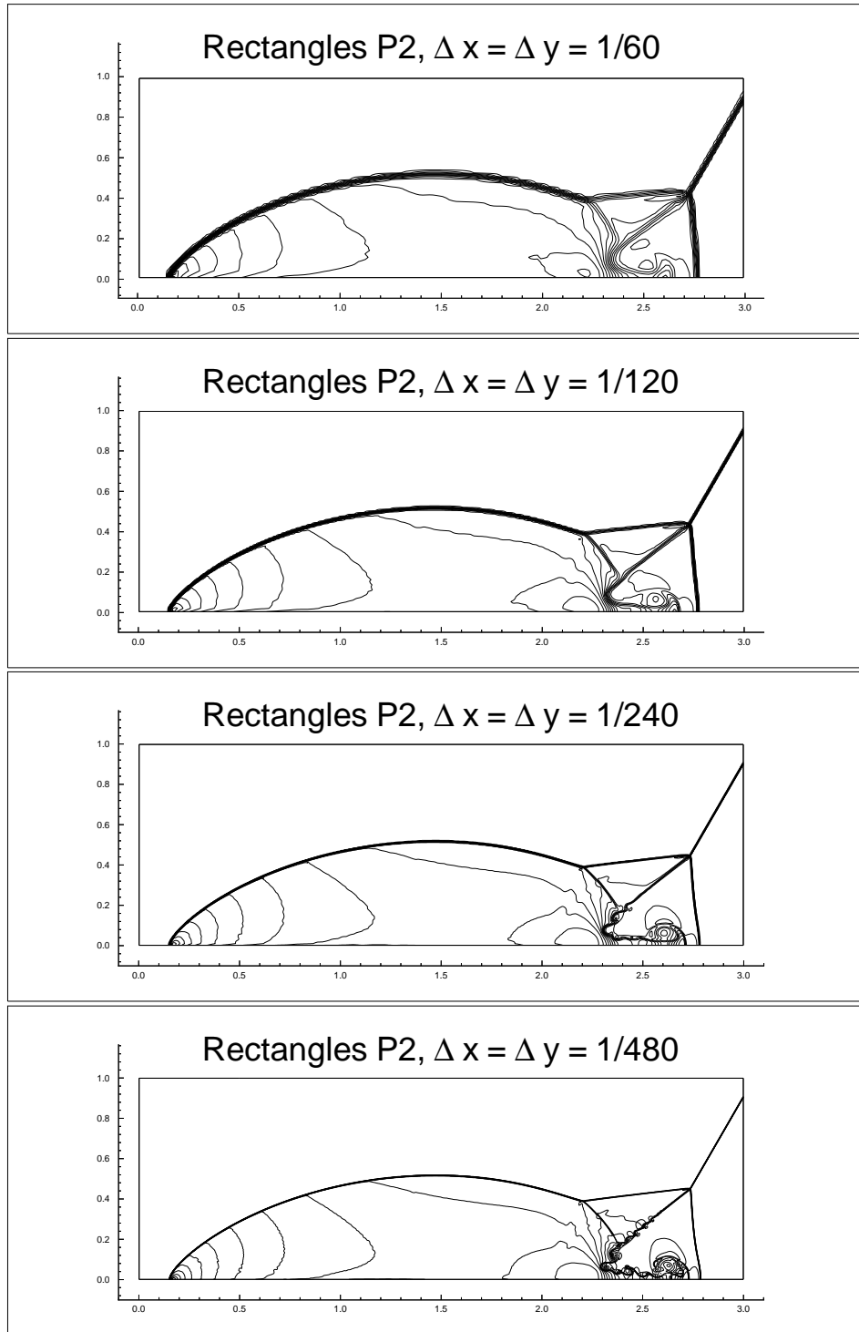
Figure 4.2: Double Mach reflection problem. Third order P^2 results. Density \rho . 30 equally spaced contour lines from \rho = 1.3965 to \rho = 22.682 . Mesh refinement study. From top to bottom: \Delta x = \Delta y = \frac{1}{60} , \frac{1}{120} , \frac{1}{240} , and \frac{1}{480} .
