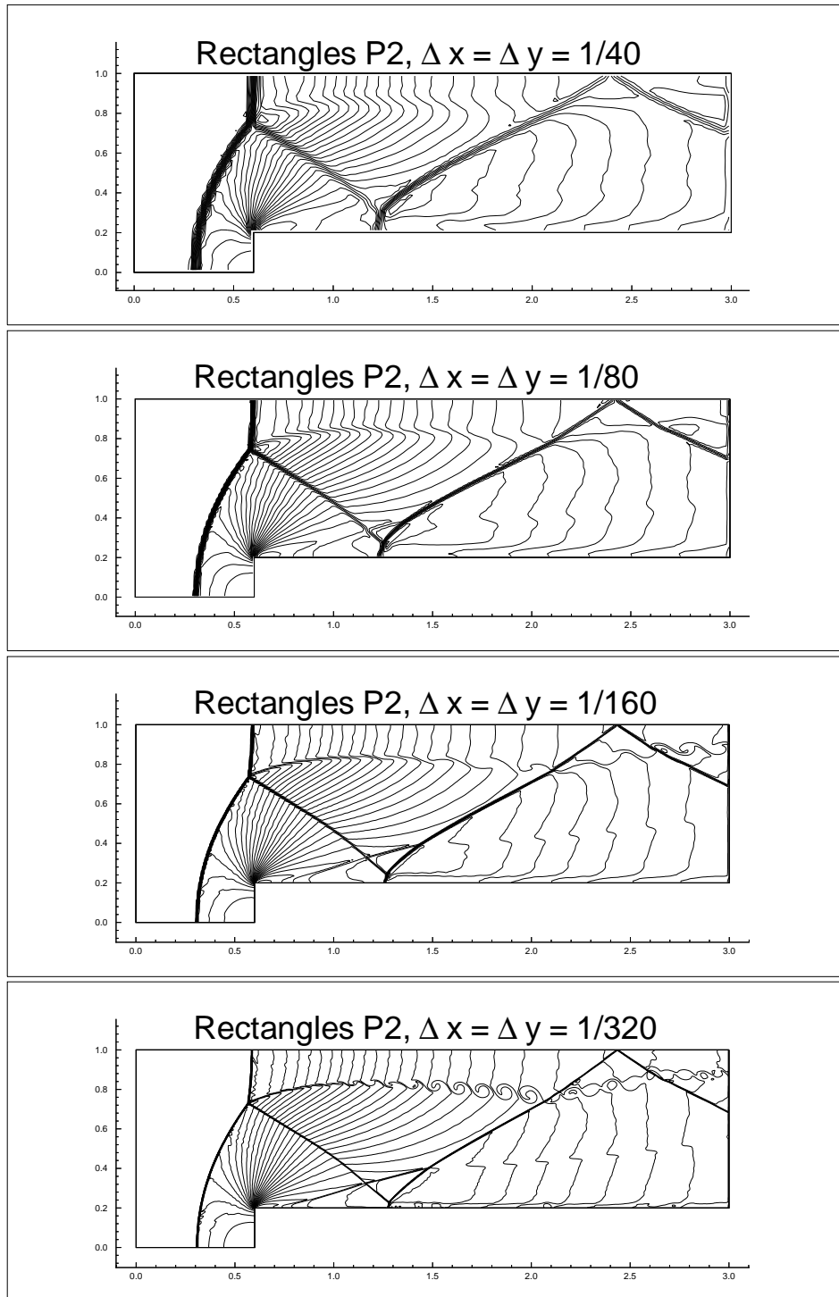
Figure 4.5: Forward facing step problem. Third order P^2 results. Density \rho . 30 equally spaced contour lines from \rho = 0.090338 to \rho = 6.2365 . Mesh refinement study. From top to bottom: \Delta x = \Delta y = \frac{1}{40} , \frac{1}{80} , \frac{1}{160} , and \frac{1}{320} .
