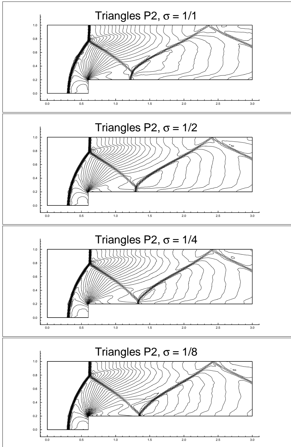
Figure 4.8: Forward facing step problem. Third order P^2 results. Density \rho . 30 equally spaced contour lines from \rho = 0.090338 to \rho = 6.2365 . Triangle code. Progressive refinement near the corner, using the triangulations shown in Figure 4.6.
