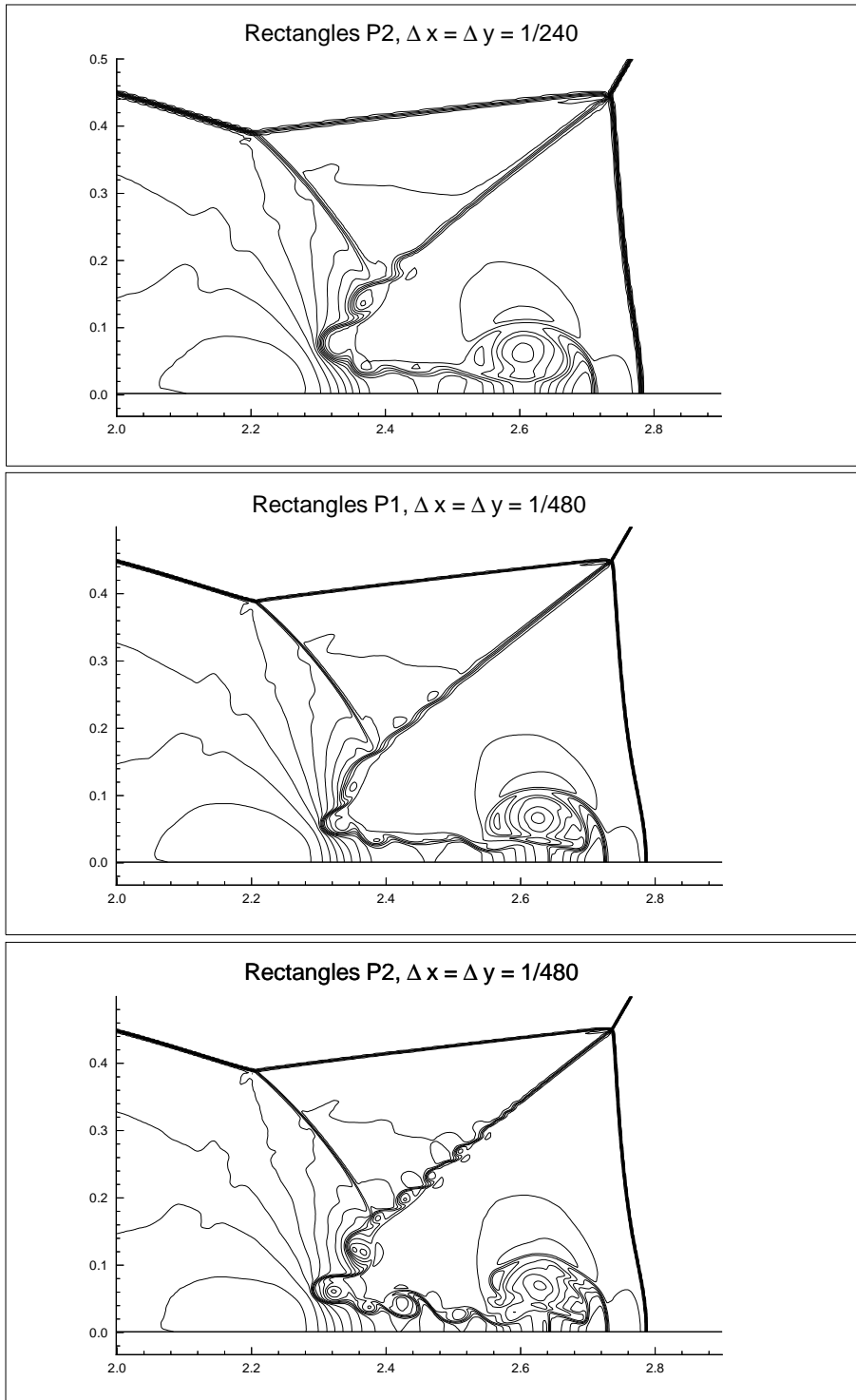
Figure 4.3: Double Mach reflection problem. Blowed-up region around the double Mach stems. Density \rho . Third order P^2 with \Delta x = \Delta y = \frac{1}{240} (top); second order P^1 with \Delta x = \Delta y = \frac{1}{480} (middle); and third order P^2 with \Delta x = \Delta y = \frac{1}{480} (bottom).
