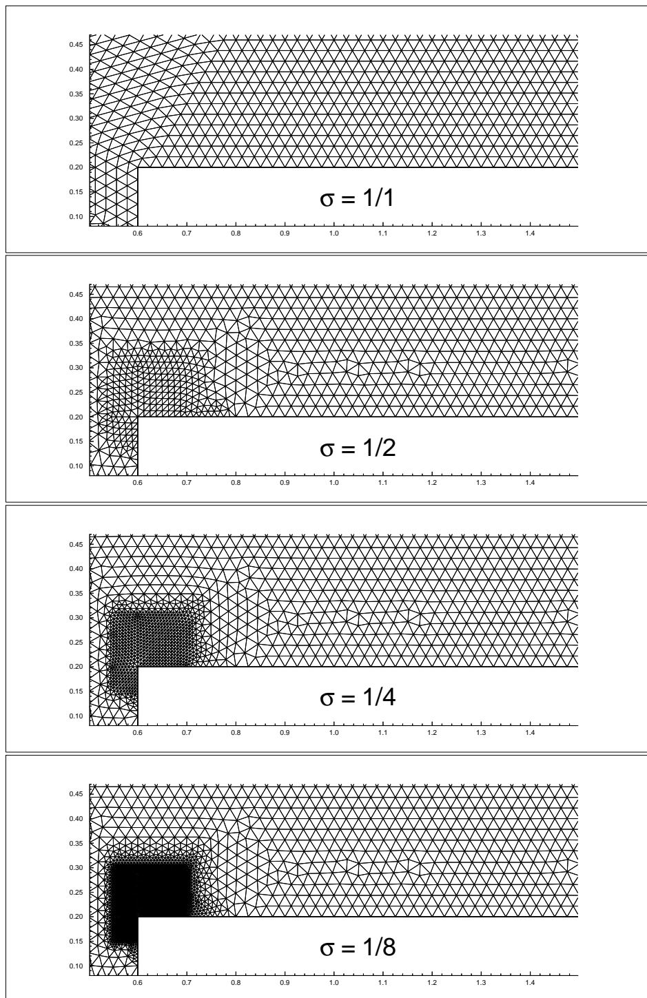
Figure 4.6: Forward facing step problem. The triangulations used for results in Figures 4.7 and 4.8. \sigma is the ratio between the typical size of the triangles near the corner and that elsewhere.
