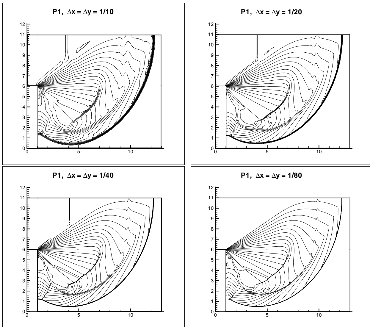
Figure 4.9: Shock diffraction problem. Second order P^1 results. Density \rho . 20 equally spaced contour lines from \rho = 0.066227 to \rho = 7.0668 . Mesh refinement study. From top to bottom: \Delta x = \Delta y = \frac{1}{10} , \frac{1}{20} , \frac{1}{40} , and \frac{1}{80} .
