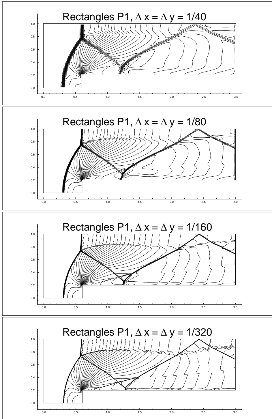
Figure 4.4: Forward facing step problem. Second order P^1 results. Density \rho . 30 equally spaced contour lines from \rho = 0.090338 to \rho = 6.2365 . Mesh refinement study. From top to bottom: \Delta x = \Delta y = \frac{1}{40} , \frac{1}{80} , \frac{1}{160} , and \frac{1}{320} .
