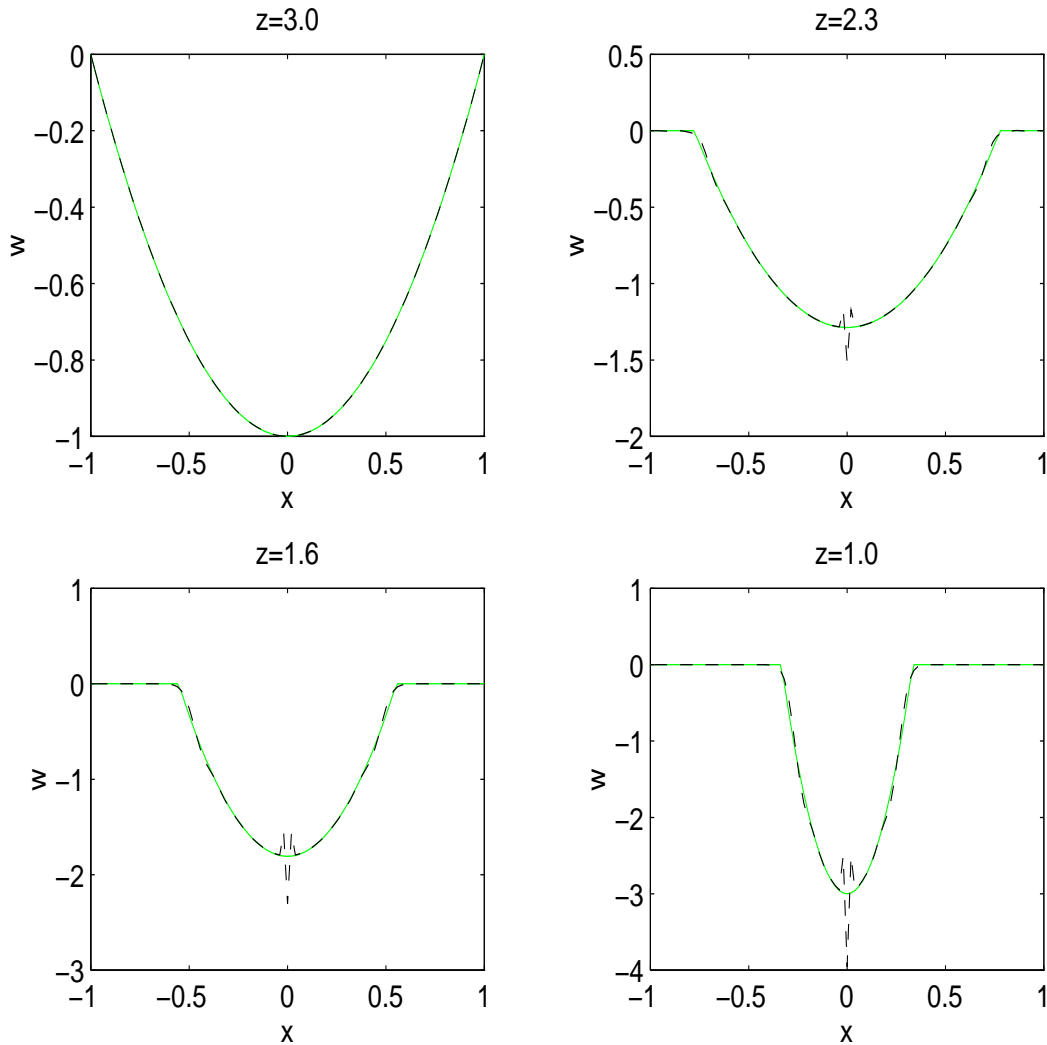
Figure 4.2: The exact solution (solid line) and the numerical solution (dashed line) of the adjoint equation for different depth. The depth z = 3 is the initial data curve. The scheme is not consistent in x = 0 .
