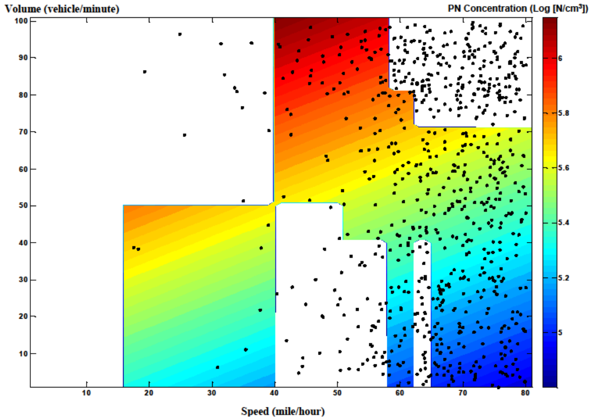
Figure 2: Prediction of total number of UFP given by different volume and speed combinations. Black dots represent observed traffic conditions – specifically, the 1-minute observations at all 454 freeway loop-detector station pairs during the 44 modeled days in 2008. For visual display, each dot represents 0.1% of all 28,765,440 one-minute-station observations.
