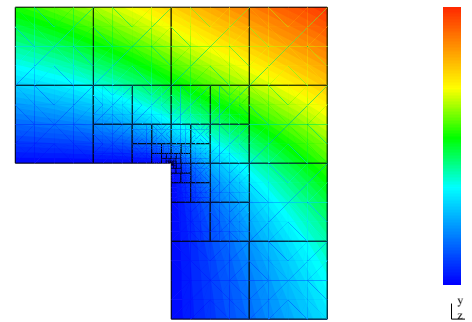
(f) The x -component of the computed displacement ( u_x ). The color scale indicates value of u_x .
