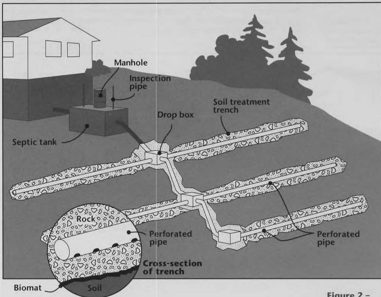
Figure 2 – Gravity flow to trench system
