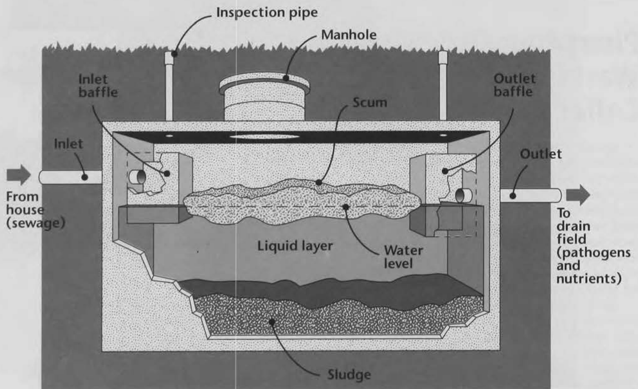
Figure 1 - Septic tank
