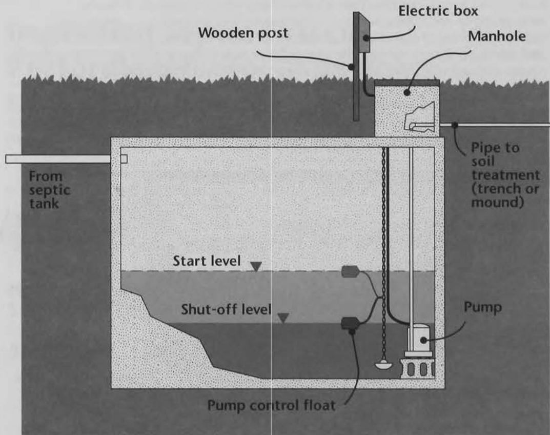
Figure 5 – Lift station
