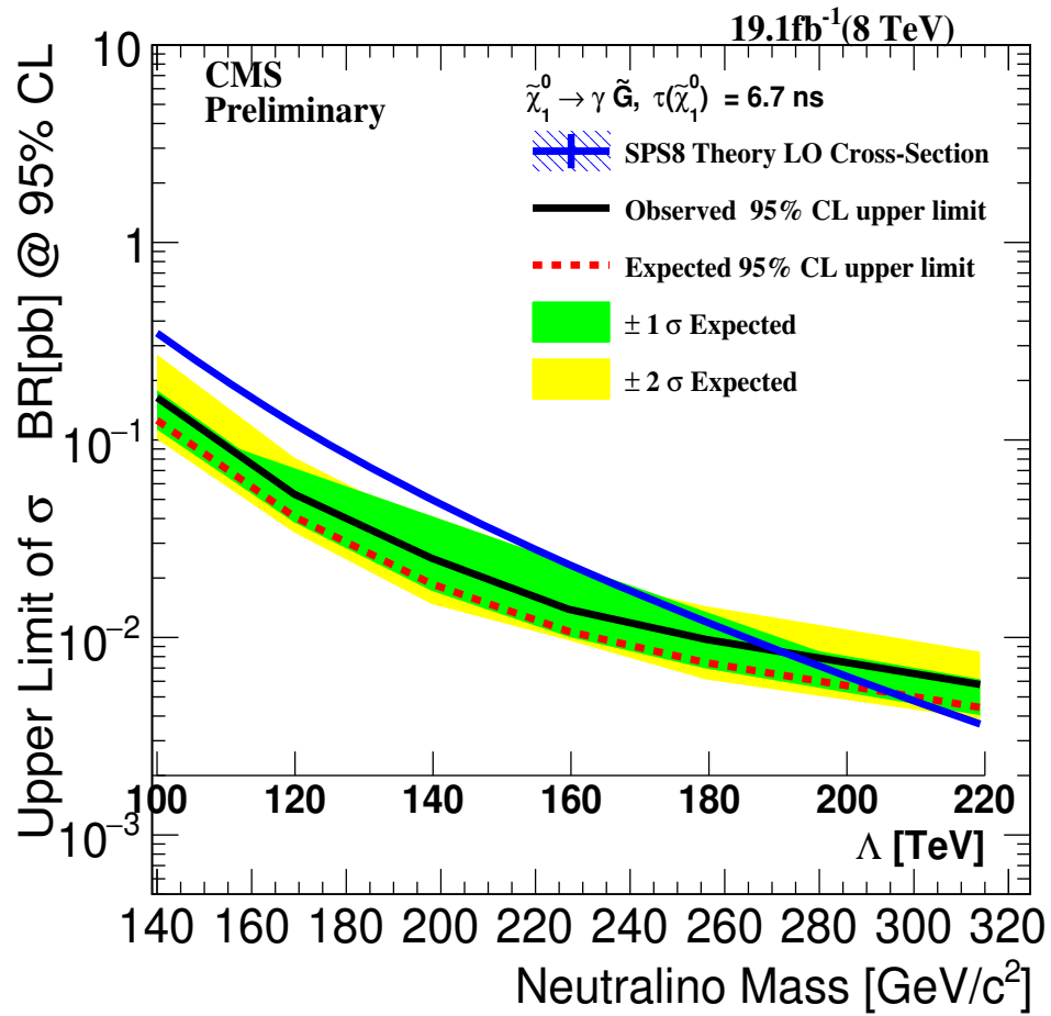
Figure 7.3: 95% CL_S CL on neutralino production cross-section times branching ratio ( \sigma_{\text{sig}} \times BR_{\tilde{\chi}_1^0}[\text{pb}] ) for different masses of the neutralino (or \Lambda ) with \tau = 6.7 \text{ ns} ( c\tau = 2000 \text{ mm} ) in the SPS8 benchmark GMSB model.
