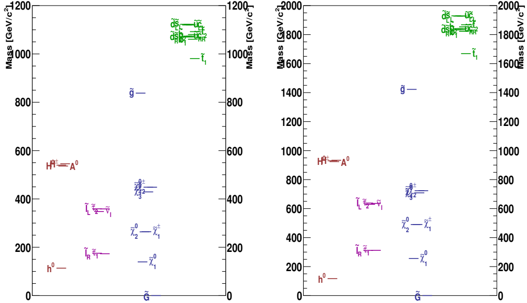
Figure 2.6: Sparticle mass spectra for SPS8 benchmark model: \Lambda = 100 TeV (left) and \Lambda = 180 TeV (right) with C_{grav} = 93.5 . The sparticle mass increases with \Lambda
