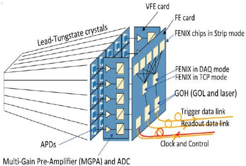
Figure 3.9: Schematic diagram of the ECAL electronics readout Trigger Tower (TT) or Front End (FE) board.
