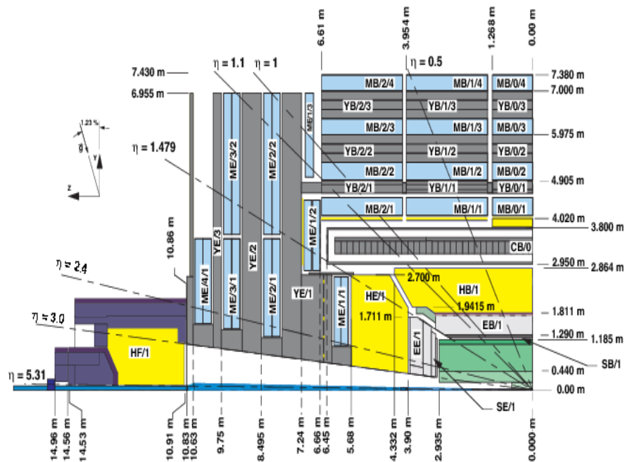
Figure 3.12: Cross section view showing the coverage range of CMS sub-detectors and their longitudinal distance from the IP.
