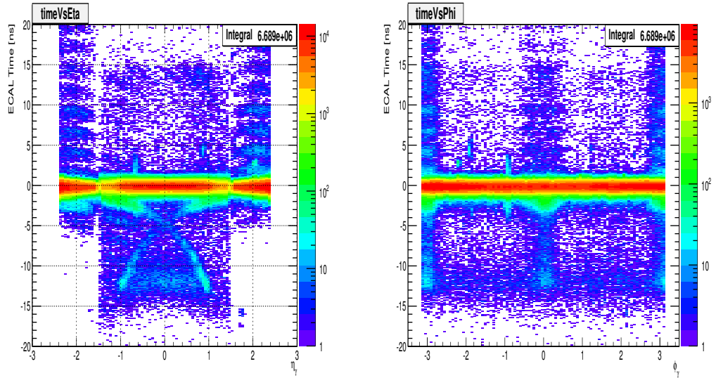
Figure 6.7: ECAL time against \eta (left) and ECAL time against \phi (right) for photons with p_T > 60 GeV from data.
