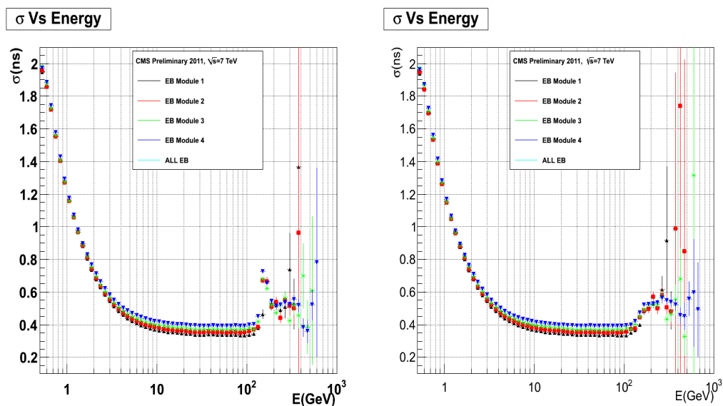
Figure 4.6: The standard deviation against rehit energy for EB in CMSSW44X (left) and CMSSW53X (right). The time bias corrections don't affect the standard deviation on the time.
