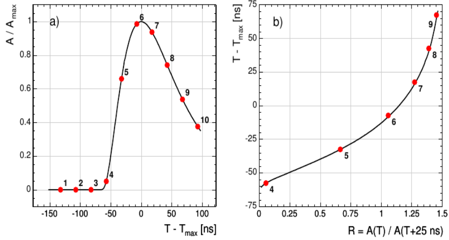
Figure 4.1: (a) A measured ECAL pulse shape for a single channel. Solid line is pulse shape from test beam while dots are typical 10 discrete samples corresponding to signal from proton-proton collision. (b) \mathbf{T} - \mathbf{T}_{\max} Vs R(T) relationship whose inverse is T(R) .
