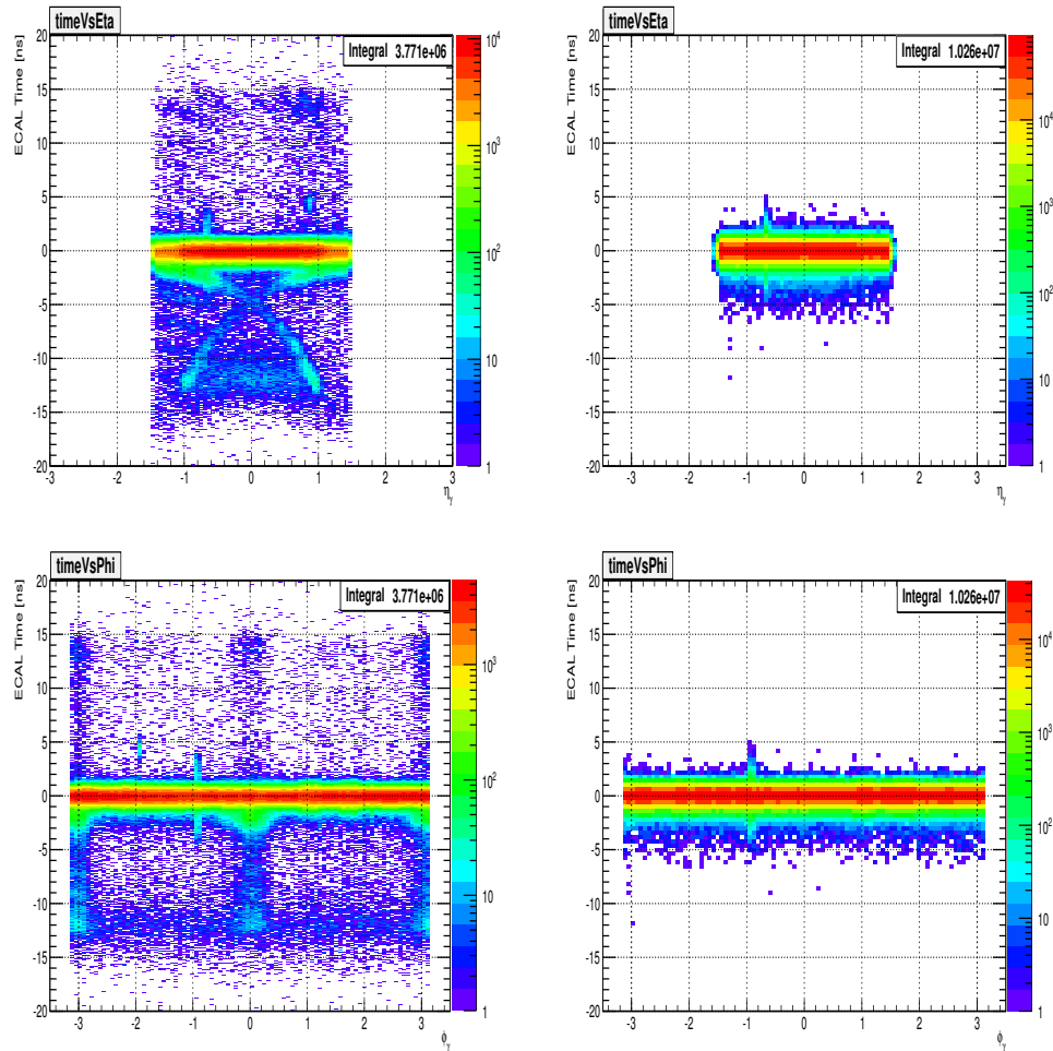
Figure 6.14: ECAL time Vs \eta (top plots) and Vs \phi (bottom plots) for electromagnetic particle candidates from SinglePhoton data sample (left) compared to electromagnetic particle candidates from the Single/DoubleElectron data sample (right). All electromagnetic particle candidates are in barrel. Most of the electromagnetic particles with “cross-shape” and at \phi = 0, \pm\pi , are halo-induced photons.
