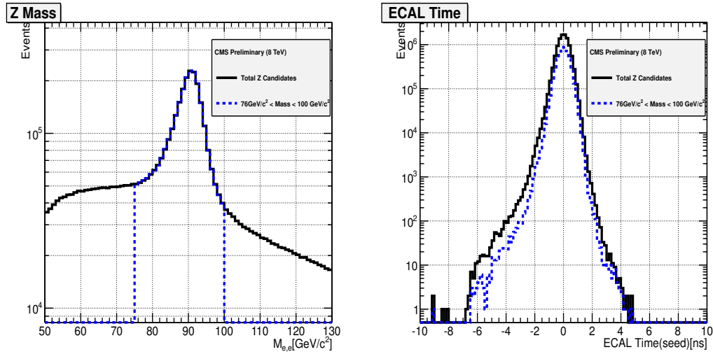
Figure 6.13: Di-electron mass distribution (left) and the time (right) of the two electron candidates for the signal, 76 < m_{e^+e^-} < 100 \text{ GeV}/c^2 , of Z boson sample. Events are from the Single/DoubleElectron data sample.
