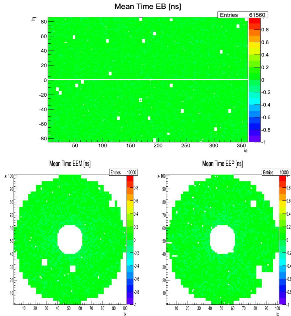
Figure 4.4: Timing maps showing the distribution of average time of each crystal after synchronization with most crystals having an average time of zero indicating the success of the crystal synchronization process and validity of the time constants.
