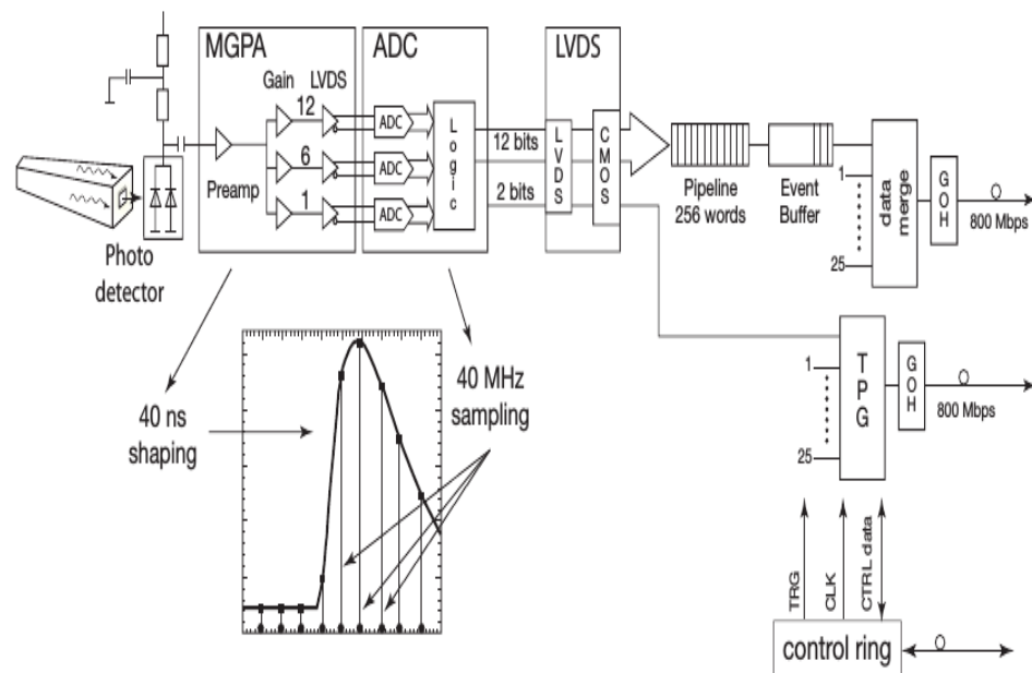
Figure 3.10: Schematic diagram of the ECAL electronics readout for a single crystal.
