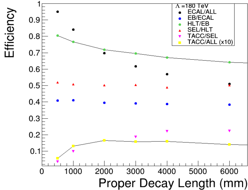
Figure 7.1: The efficiency for different mean decay length, c\tau [mm] with \Lambda = 180 TeV. TACC/ALL (yellow square markers) is the Efficiency \times Acceptance( t > 3 ns) i.e. \varepsilon \times A , used in evaluating the exclusion limits. The TACC/ALL is magnified by factor \times 10 for display purpose.
