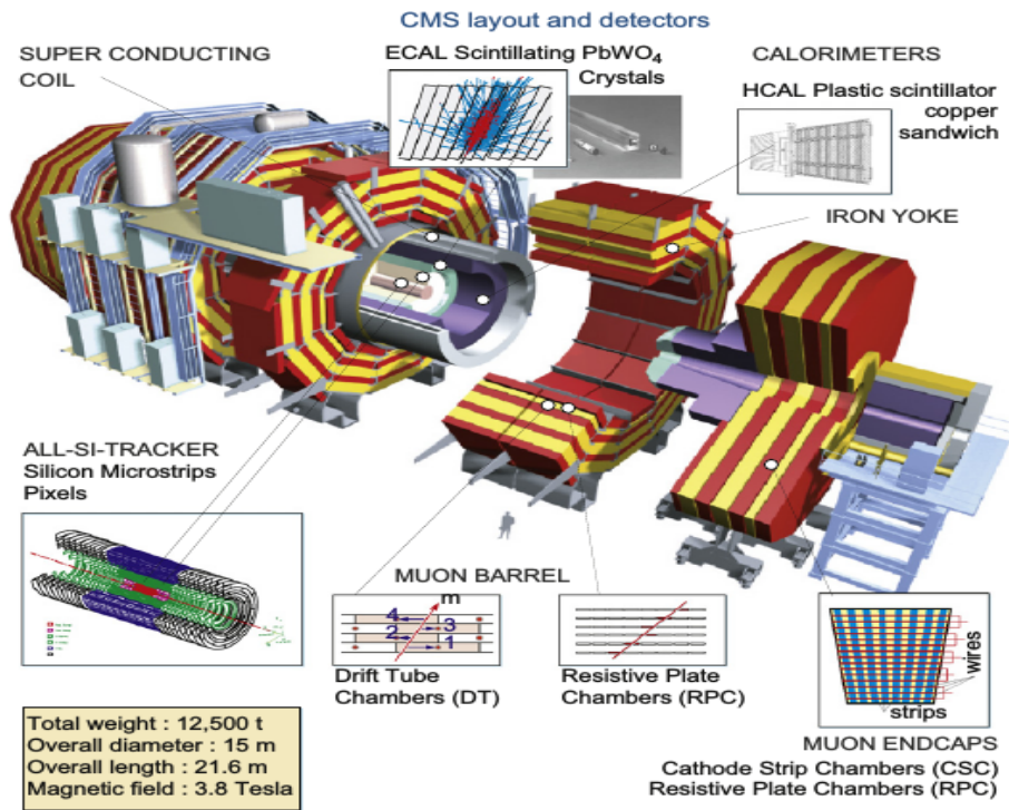
Figure 3.6: CMS Detector showing the different subdetectors and their material.
