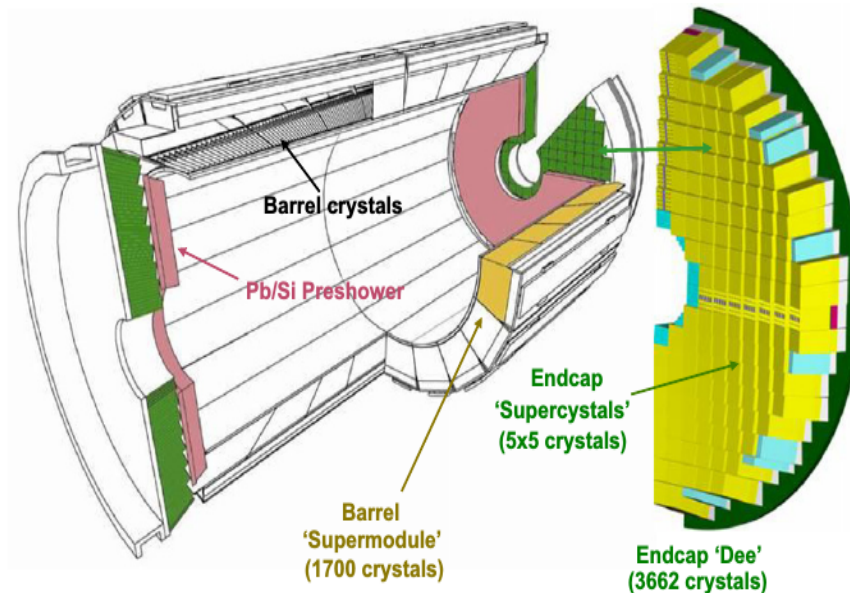
Figure 3.8: Layout of the CMS electromagnetic calorimeter showing the arrangement of crystal modules, supermodules in the barrel with the preshower in front of endcap with supercrystals.
