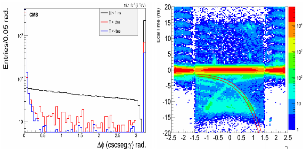
Figure 6.8: ECAL time vs \Delta\phi(\text{CSC Seg}, \gamma) (left) for in time (black) and out-of-time (red and blue) photons. Photon ECAL time V.s \eta (right), expected halo-induced photon time is shown as two red lines.
