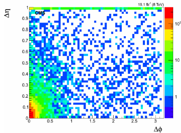
Figure 6.10: Scatter plot of \Delta\eta(\text{DT Seg}, \gamma) against \Delta\phi(\text{DT Seg}, \gamma) for photons from pure cosmic muon data. Small \Delta\eta and \Delta\phi are cosmic photons.
