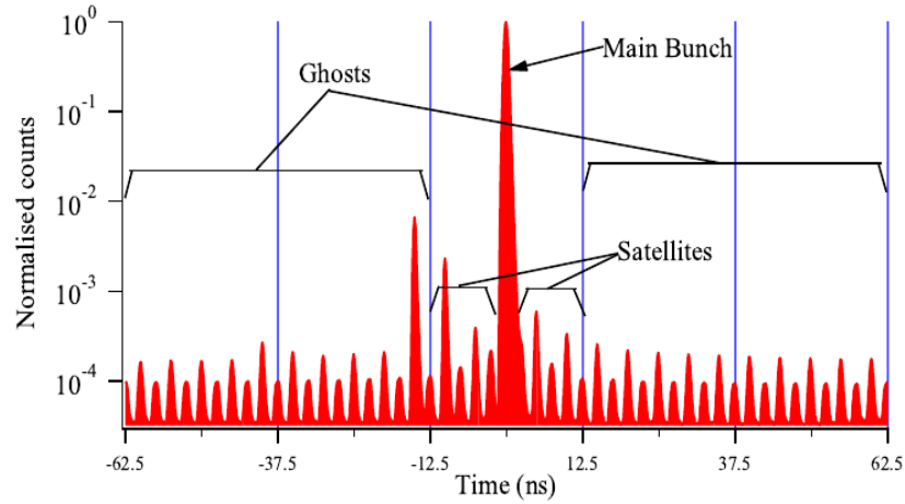
Figure 3.3: Longitudinal profile of a typical LHC proton beam taken with the Longitudinal Density Monitor (LDM) detector. Ghost/Satellite bunches and the main proton bunch shown.
