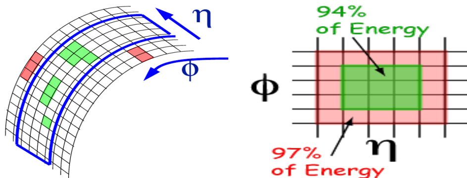
Figure 5.1: Superclustering algorithm direction (left) in the (\eta, \phi) plane in EB and fraction (right) of electromagnetic shower energy coverage in a crystal energy matrix.
