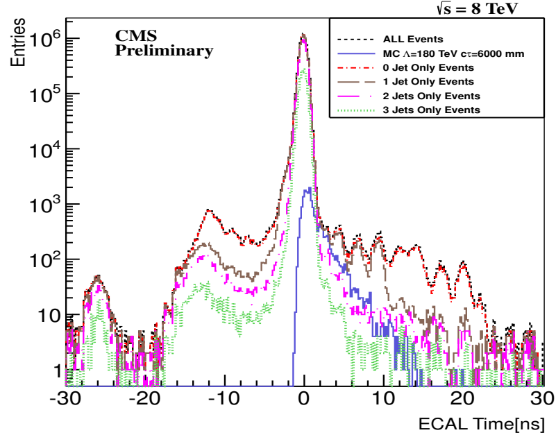
Figure 6.6: Comparing ECAL time distribution of events with different jet multiplicity from small sample of data and a single GMSB \Lambda = 180 TeV and c\tau = 6000 mm sample. Accepted photons must have p_T > 60 GeV and belong to barrel and encaps.
