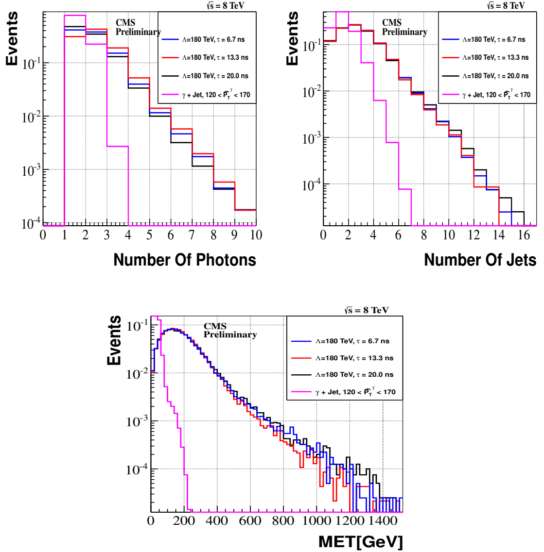
Figure 2.8: Number of photons with photon p_T > 50 GeV/c (top left), number of jets (top right) and E_T^{\text{miss}} (bottom) for events with \tilde{\chi}_1^0 decay to \gamma and \tilde{G} for different lifetimes \tau = 6.7 ns, 13.3 ns, 20.0 ns and \Lambda = 180 TeV of the SPS8 benchmark GMSB model. A \gamma +jet with 120 < p_T^\gamma < 170 GeV/c sample shown for comparison with the signal samples.
