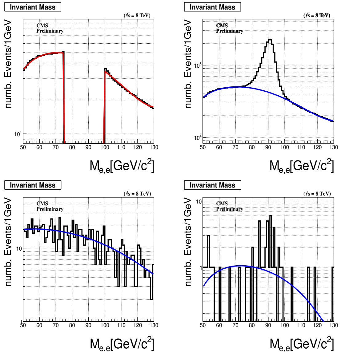
Figure 6.15: Di-electron invariant mass and polynomial fit (red) for sideband sample ( 50 < m_{e^+e^-} < 76 \text{ GeV}/c^2 and 100 < m_{e^+e^-} < 130 \text{ GeV}/c^2 ). Di-electron invariant mass and polynomial fit (blue) for in-time ( |t| < 2 \text{ ns} ) Z candidates ( top right ). Di-electron invariant mass and polynomial fit for out-of-time ( t < -3 \text{ ns} ) Z candidates ( bottom left ). Di-electron invariant mass and polynomial fit for out-of-time ( t > 3 \text{ ns} ) Z candidates ( bottom right ). The fits are used to estimate the number of true Z bosons in the in-time and out-of-time Z candidate samples.
