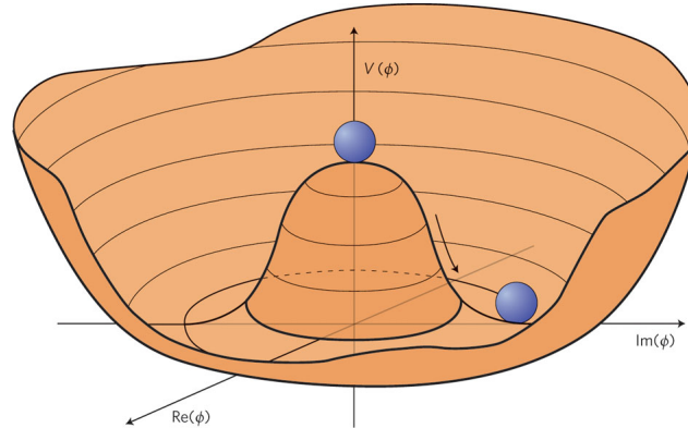
Figure 2.1: Higgs boson “Mexican hat” potential, V(\phi^*\phi) = \mu^2(\phi^*\phi) + \lambda(\phi^*\phi)^2 , which leads to spontaneous symmetry breaking with choice of parameters \mu^2 < 0 , \lambda > 0 .
