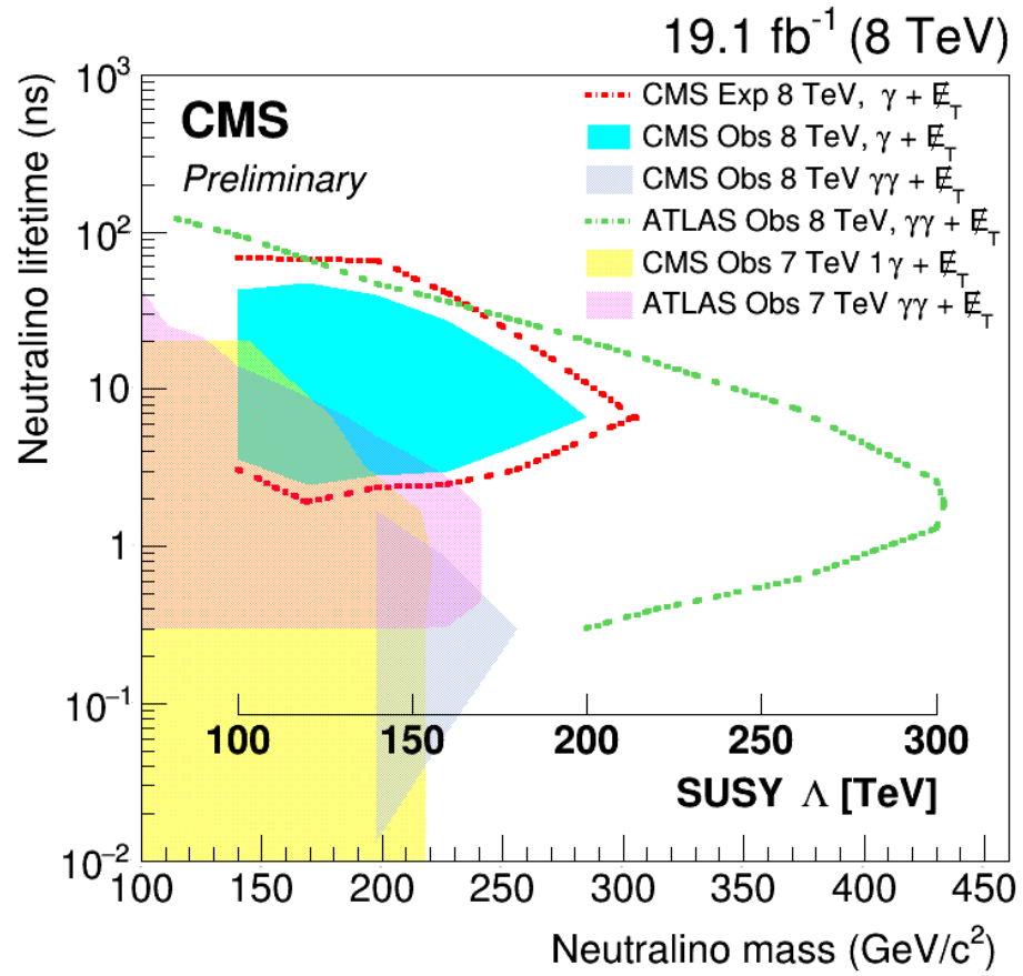
Figure 7.4: Exclusion limits in neutralino mass (or \Lambda ) against mean lifetime in SPS8 benchmark GMSB model. The limits from previous experiments are also shown.
