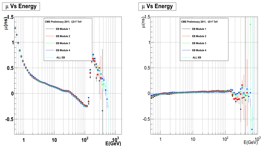
Figure 4.5: Average time ( \mu ) against rehit energy for EB. The first gain transitions (gain-12 to 6) happens at about 130 GeV and time bias on energy is seen in CMSSW44X (left) and very little in CMSSW53X (right) where the corrections have been applied during rehit reconstruction.
