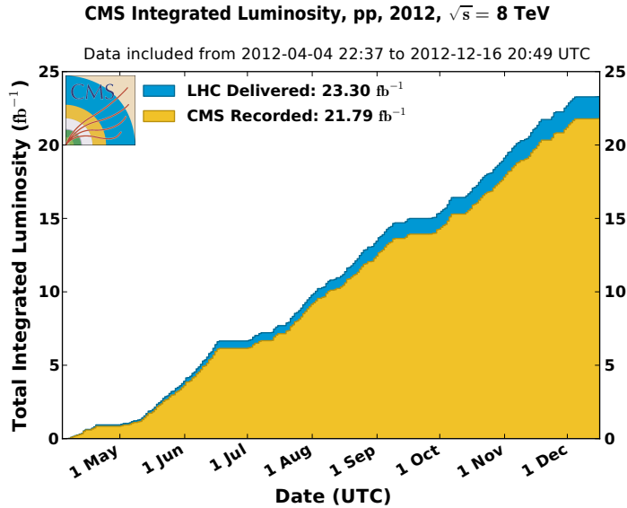
Figure 3.2: Cumulative luminosity versus month delivered (blue) by the LHC and recorded (orange) by CMS detector during stable beams of pp collisions at \sqrt{s} = 8 \text{ TeV} in 2012.
