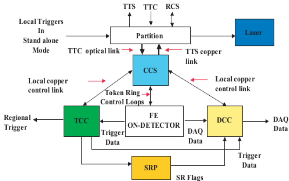
Figure 3.11: Schematic diagram of the ECAL Off-Detector and Readout Architecture.
