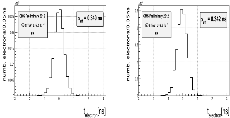
Figure 4.8: Absolute time of a single reconstructed electron in Z \rightarrow e^-e^+ decay. The electron time is the seed (crystal with highest energy deposit) time of the electron in EB and EE.
