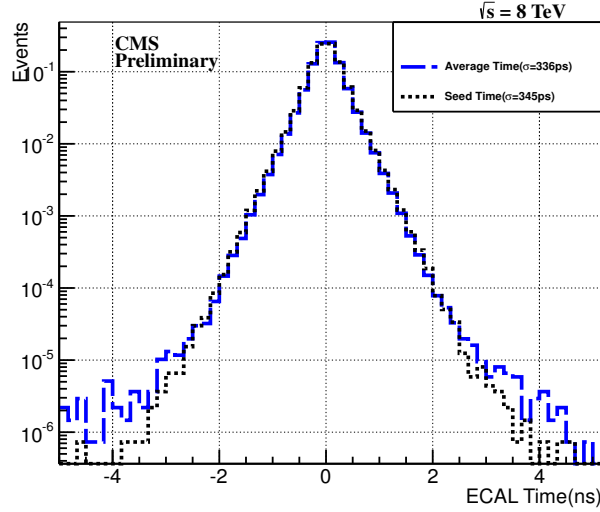
Figure 6.1: Seed (black) and Average (blue) times as the measured photon time.
