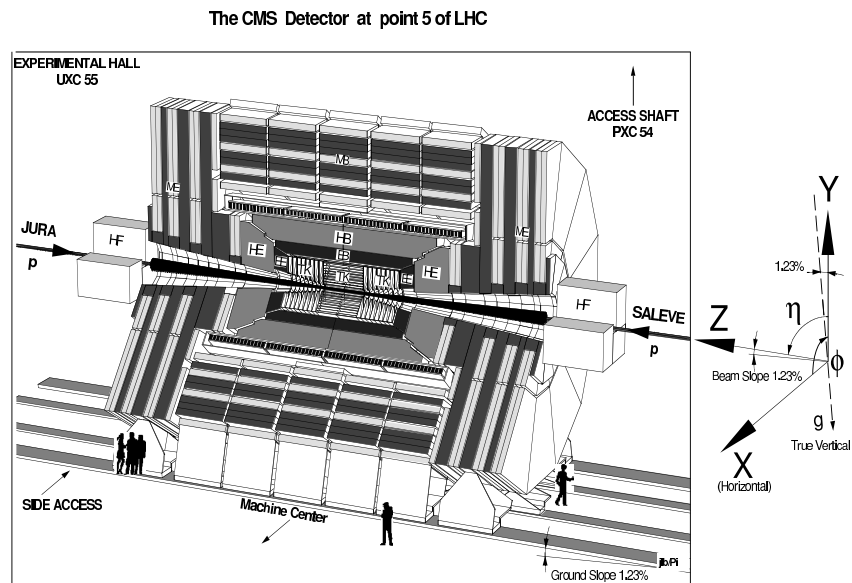
Figure 3.7: CMS detector schematic view with definition of x - y - z coordinates.
