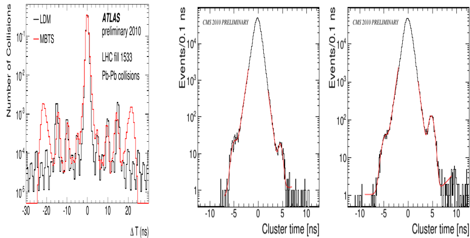
Figure 3.4: Left: Arrival time (red) of events in ATLAS for LHC fill 1533 during 2010 PbPb collision and an LDM profile (black) for Beam2 (same for Beam1). Right: Cluster time in the CMS endcap calorimeters from fill 1089 of the positive endcap detector(left side of IP, z > 0 ) (left) and negative endcap detector(right side of IP, z < 0 ) (right). Both plots show a clear presence of events from Ghost/Satellite bunches with the expected time separation.
