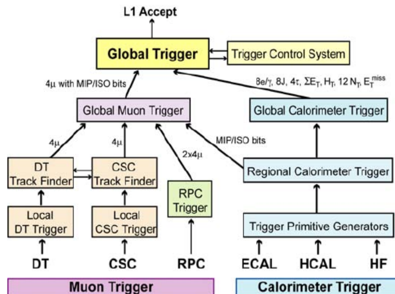
Figure 3.13: Level-1 Trigger Architecture of CMS.
