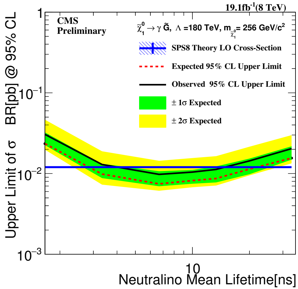
Figure 7.2: 95% CL_S CL on neutralino production cross-section times branching ratio ( \sigma_{\text{sig}} \times BR_{\tilde{\chi}_1^0} [pb]) against mean lifetime[ns] for m_{\tilde{\chi}_1^0} = 256 \text{ GeV}/c^2 in the SPS8 benchmark GMSB model.
