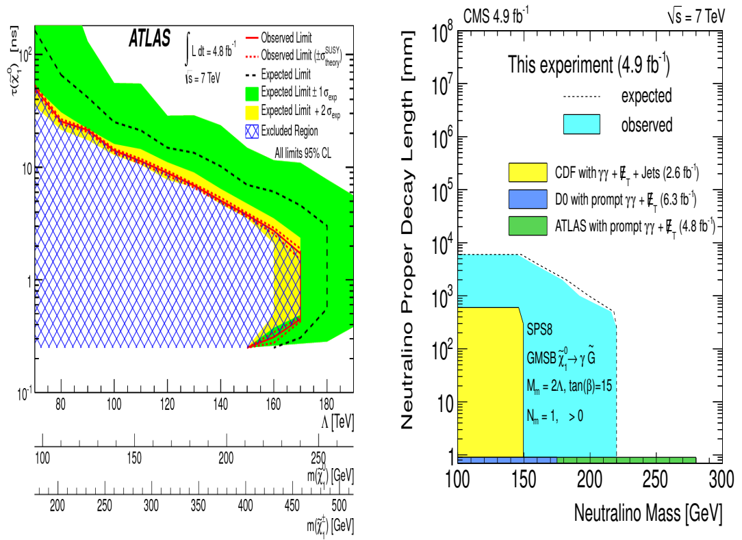
Figure 2.11: Neutralino lifetime and mass upper limit from ATLAS (left) and CMS (7 TeV), DØ and CDF experiments (right) from the search for events with delayed or non-pointing photons.
