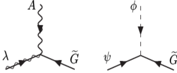
Figure 2.5: Feynman diagrams of Gravitino-Gaugino-Gauge boson ( \tilde{G}, \lambda, A ) (left) and Gravitino-Scalar-Chiral fermion ( \tilde{G}, \phi, \psi ) (right) couplings. The coupling strength goes like \frac{1}{\sqrt{\mathbf{F}}} .
