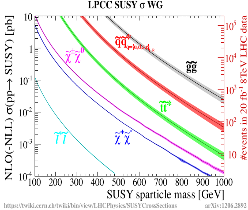
Figure 2.4: Cross section for producing sparticles with different mass and in different type of interaction at the LHC. More higher mass sparticles are produced through strong interaction, pp \rightarrow \tilde{g}\tilde{g} , than the others, pp \rightarrow \tilde{\chi}^{\pm}\tilde{\chi}^{\mp}, \tilde{\chi}^0\tilde{\chi}^{\pm}
