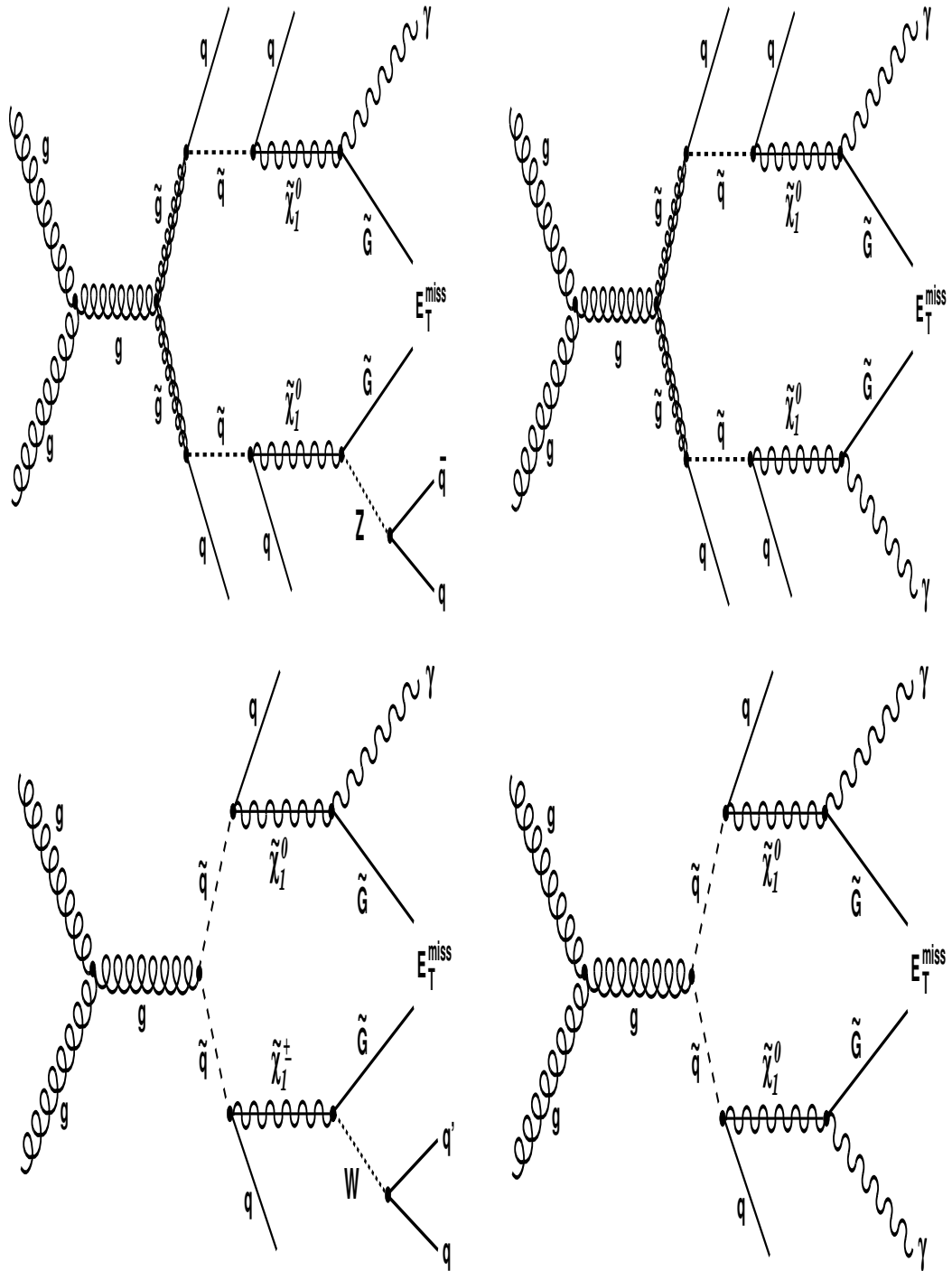
Figure 2.7: Feynman diagrams for lightest neutralino ( \tilde{\chi}_1^0 ) production from the cascade decay of a pair of gluinos ( top ) and squarks ( bottom ). The final state can either have a single ( left diagrams ) or double photons ( right diagrams ).
