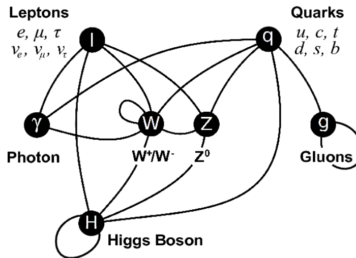
Figure 2.2: Fermions and bosons and their interactions in the SM. The bosons (except the Higgs boson) mediate the interactions between fermions.
