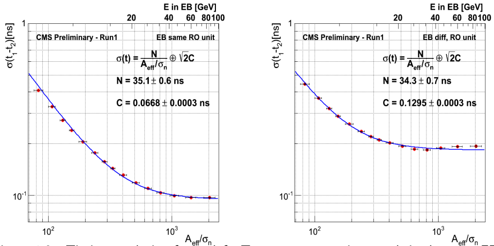
Figure 4.9: Timing resolution from: left : Two most energetic crystals in the same FE electronics, right : Two most energetic crystals belonging to different FE electronics, as a function of effective amplitude ( A_{eff} = A_1 A_2 / \sqrt{A_1^2 + A_2^2} ) normalized to noise in EB. Both crystals are from reconstructed electrons in Z \rightarrow e^- e^+ events.
