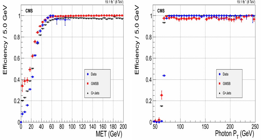
Figure 6.5: Our HLT efficiency turn-on curves in event \cancel{E}_T (left) and photon p_T (right). The \gamma +jets samples require photon p_T > 170 GeV/c.
