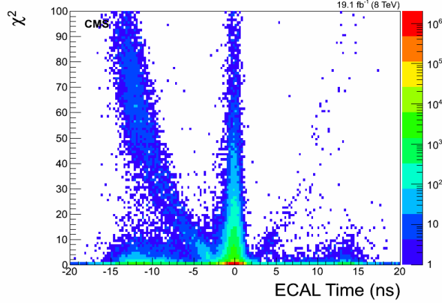
Figure 6.2: A \chi^2 against photon time distribution. Spikes misidentified as photons have very large \chi^2 and negative time particularly the region where \chi^2 > 4 and t < -4 ns.
