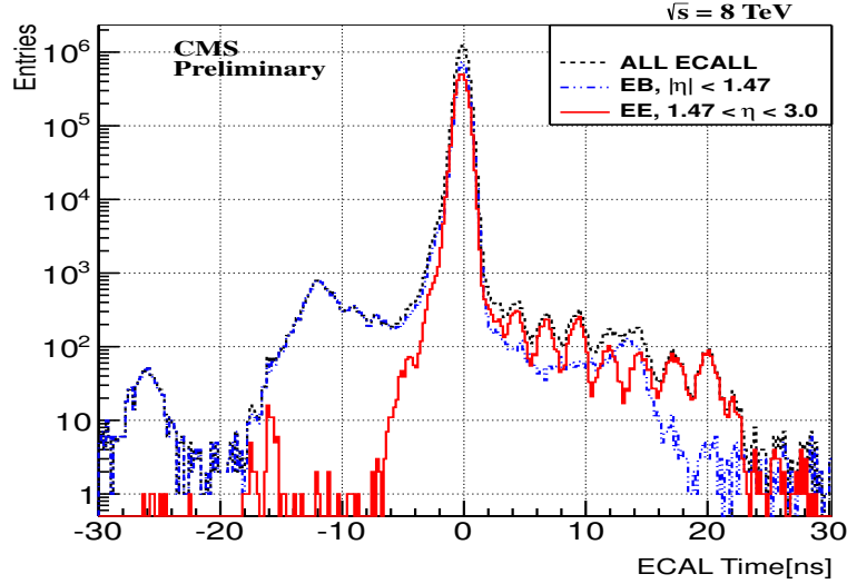
Figure 6.4: Time distribution of photons in barrel (EB), endcap (EE) and all of ECAL (ALL ECAL) with p_T > 50 GeV from data. A 2.5 ns delay timing pattern is observed in ECAL with clarity in EE.
