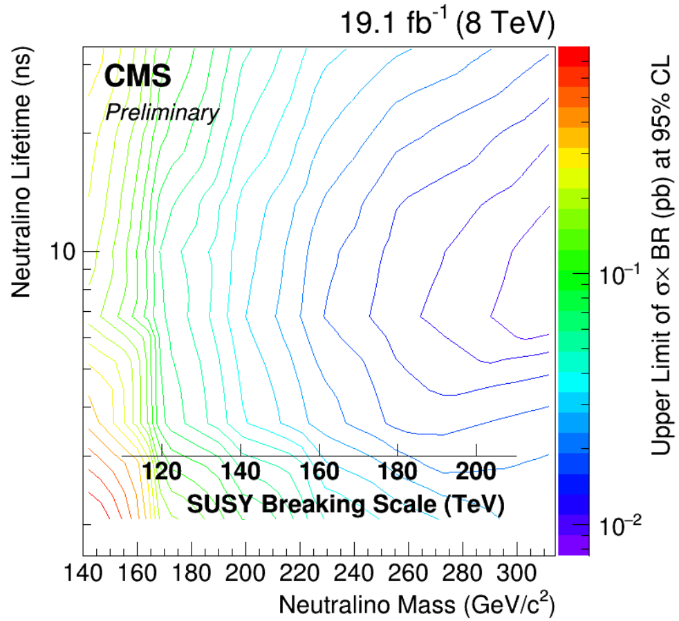
Figure 7.5: Cross-section upper limits at 95% CL_S CL for different mass and lifetime of the neutralino using 8 TeV data corresponding to an integrated luminosity of 19.1 \text{ fb}^{-1} of the CMS experiment.
