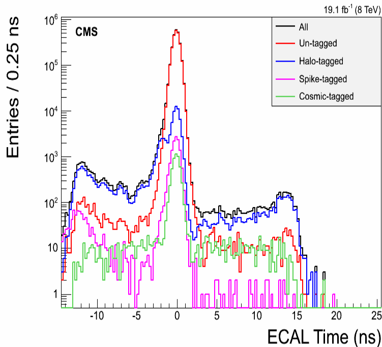
Figure 6.12: Photon ECAL time, for a data sample of 0 and 1-jet events, showing our tagging performance for non-collision background events.
