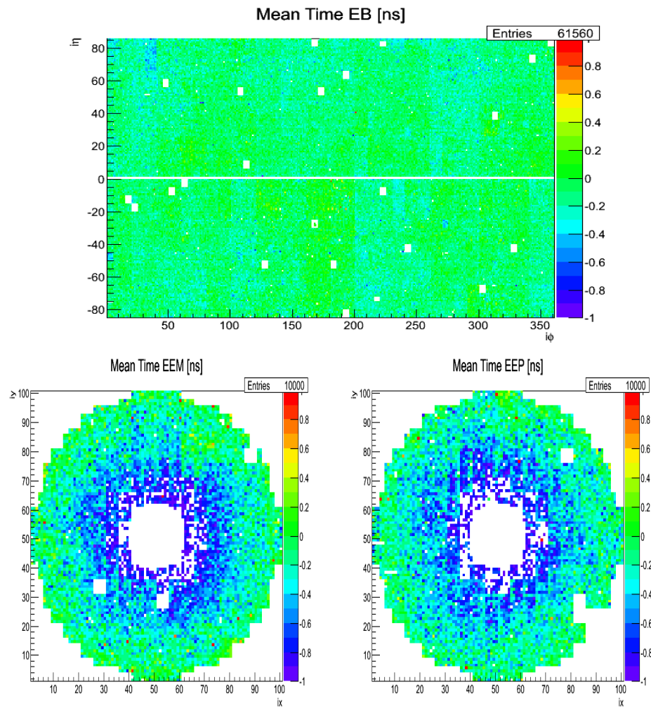
Figure 4.3: Timing maps showing the distribution of average (mean) time for each \text{PbWO}_4 crystal in EB (top) and EE (below: EE-(left), EE+(right)) before crystal synchronization.
