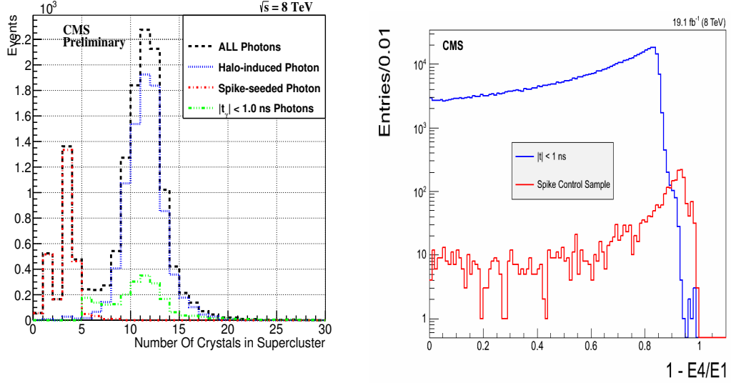
Figure 6.11: Number of crystals in photon supercluster (left) comparing all photon candidates in EB (black), halo-induced photon candidates (blue), spike-seeded photon candidates (red) and photons with |t_\gamma| < 1.0 (green). The spike-seeded photon candidates are selected using a Swiss-Cross variable (1 - E_4/E_1) (right) which is comparing in-time photons ( |t_\gamma| < 1.0 ) to spike candidate photons which were selected using S_{Minor} .
