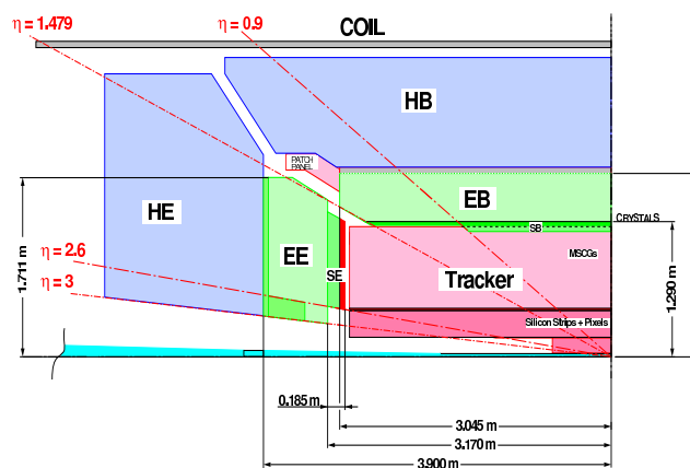
Figure 3.5: Schematic diagram of CMS calorimetry system with HCAL enclosing ECAL in the barrel and endcap regions.
