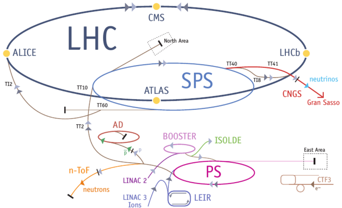
Figure 3.1: Schematic diagram showing the full Large hadron Collider.
