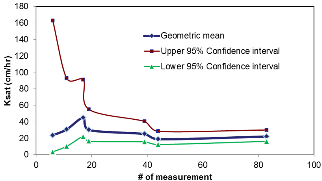
Figure 12. Relationship between number of measurements and K_{sat} for the Madison swale.
