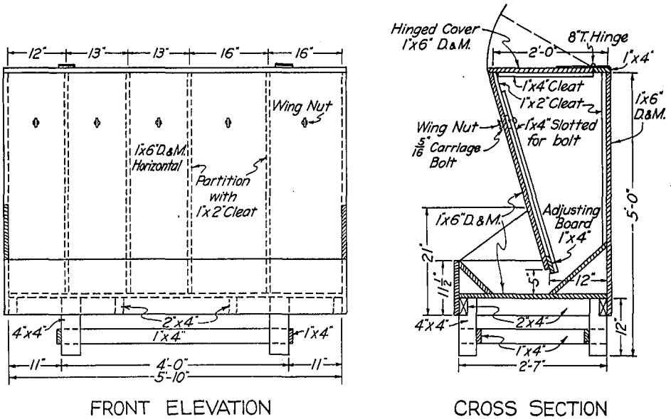
FIG. 9. A FREE-CHOICE, FIVE-COMPARTMENT SELF-FEEDER FOR CALVES Inside partitions may be omitted and a single grain mixture fed.
