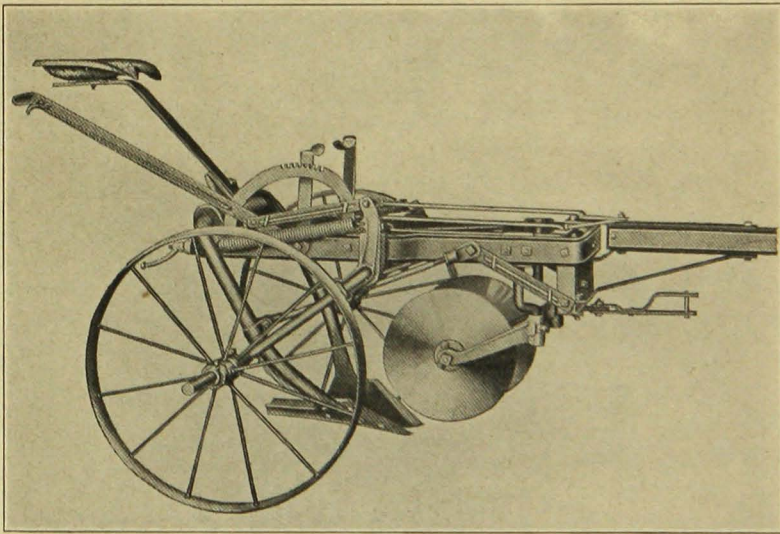
Fig. 3. Two-Blade Riding Beet Lifter
