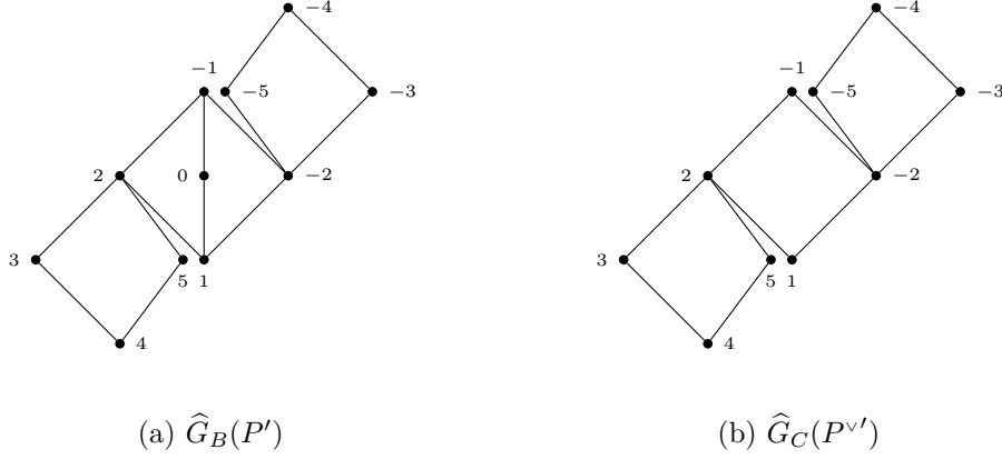
Figure 4.18: Having opened one notch to obtain P'
