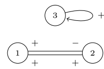
(a) Hasse diagram
