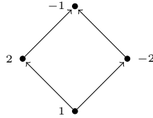
Figure 4.4: Another signed covering
