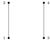
(a) A forest F
