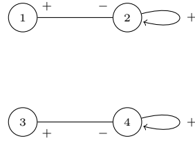
(b) F embedded as a signed poset, F_B
