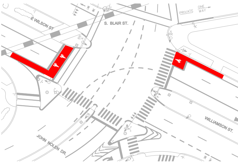
Figure 18. Illustration of the red bike boxes on Williamson Street. source: City of Madison 2010
