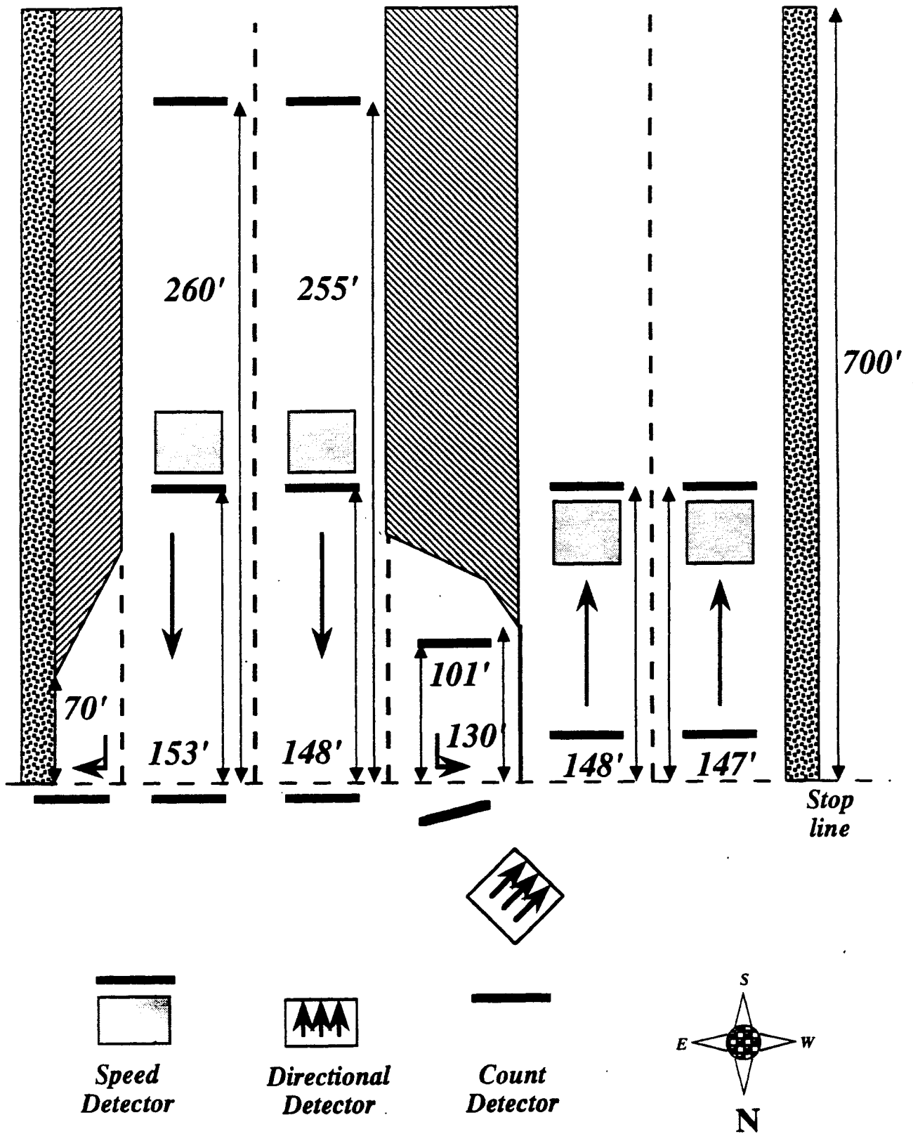
Figure 7.1 Northbound detector layout (not to scale).
