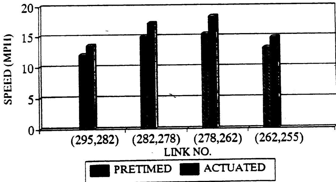
FIGURE 4.14. AVERAGE SPEED COMPARISON (1ST AVE.)
