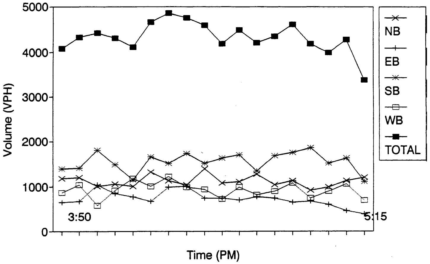
Fig. 5.3 PM-peak demand
