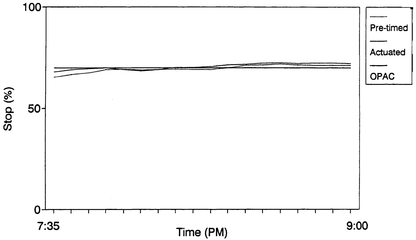
Fig. 5.21 Period Stop Percentage Comparison (Off-peak)
