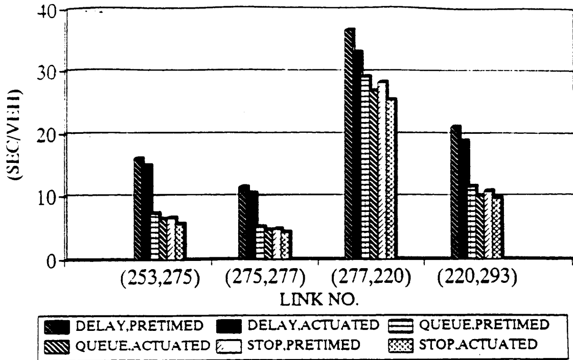
FIGURE 4.5. DELAY, QUEUE, STOP TIME COMPARISON (HENNEPIN AVE.)
