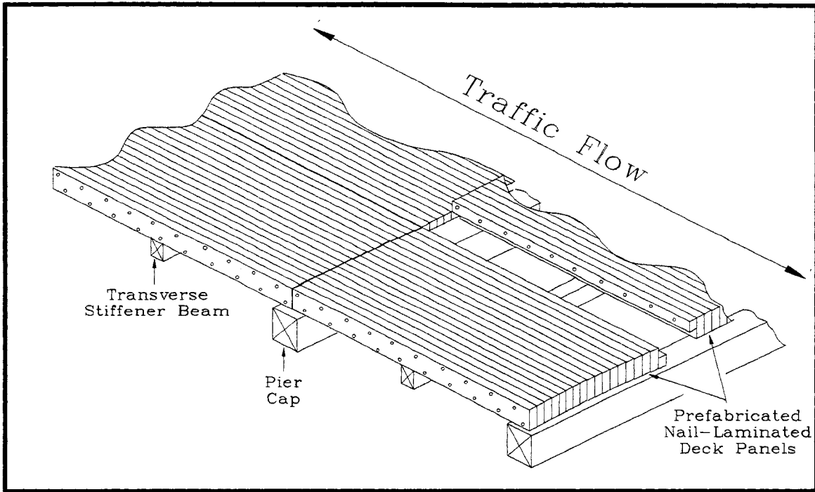
Figure 3.5 Panelized Longitudinal Nail-Laminated Superstructure (Cut-Away Representation)
