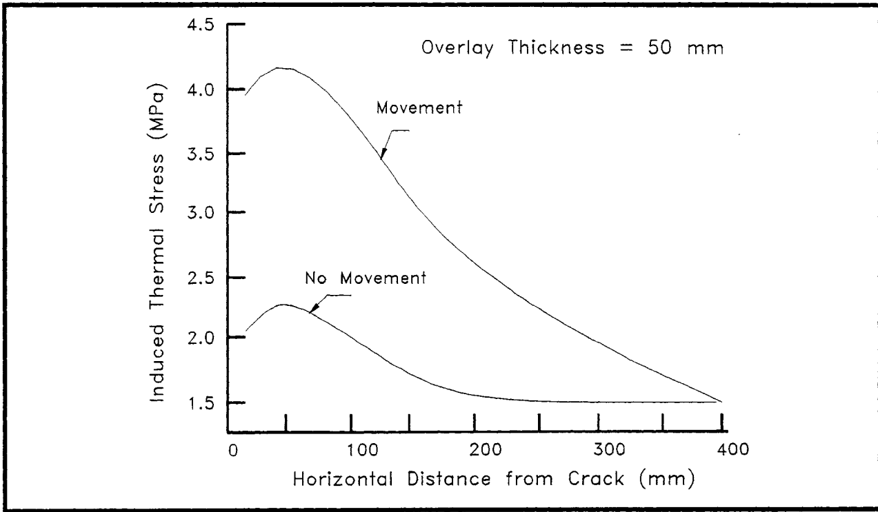
Figure 3.14 Stress Distribution in the Top of the Asphalt Overlay for Different Conditions [after ref. 9]
