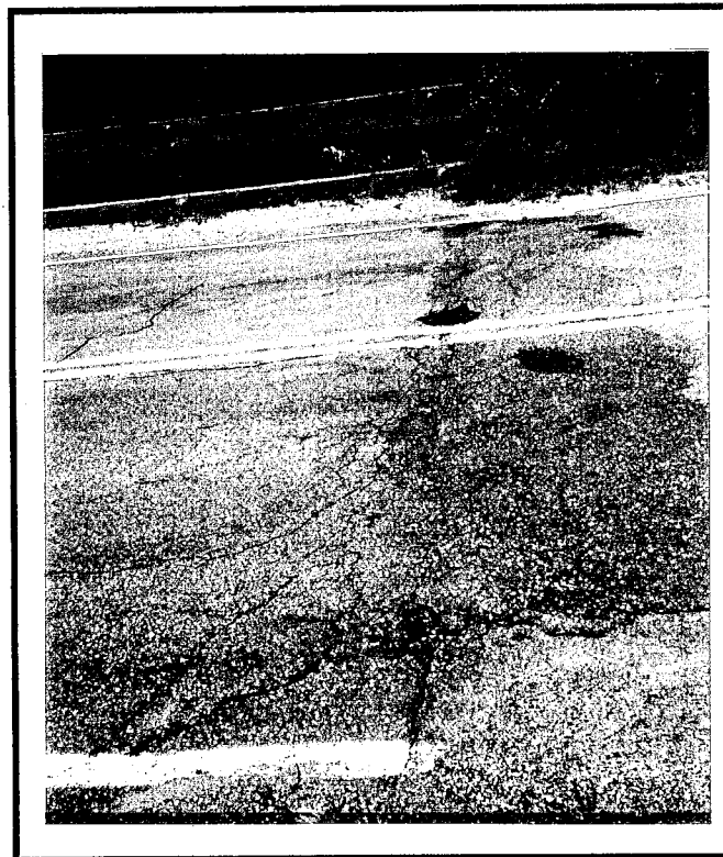
Figure 2.5 Asphalt Fatigue and Transverse Cracking
