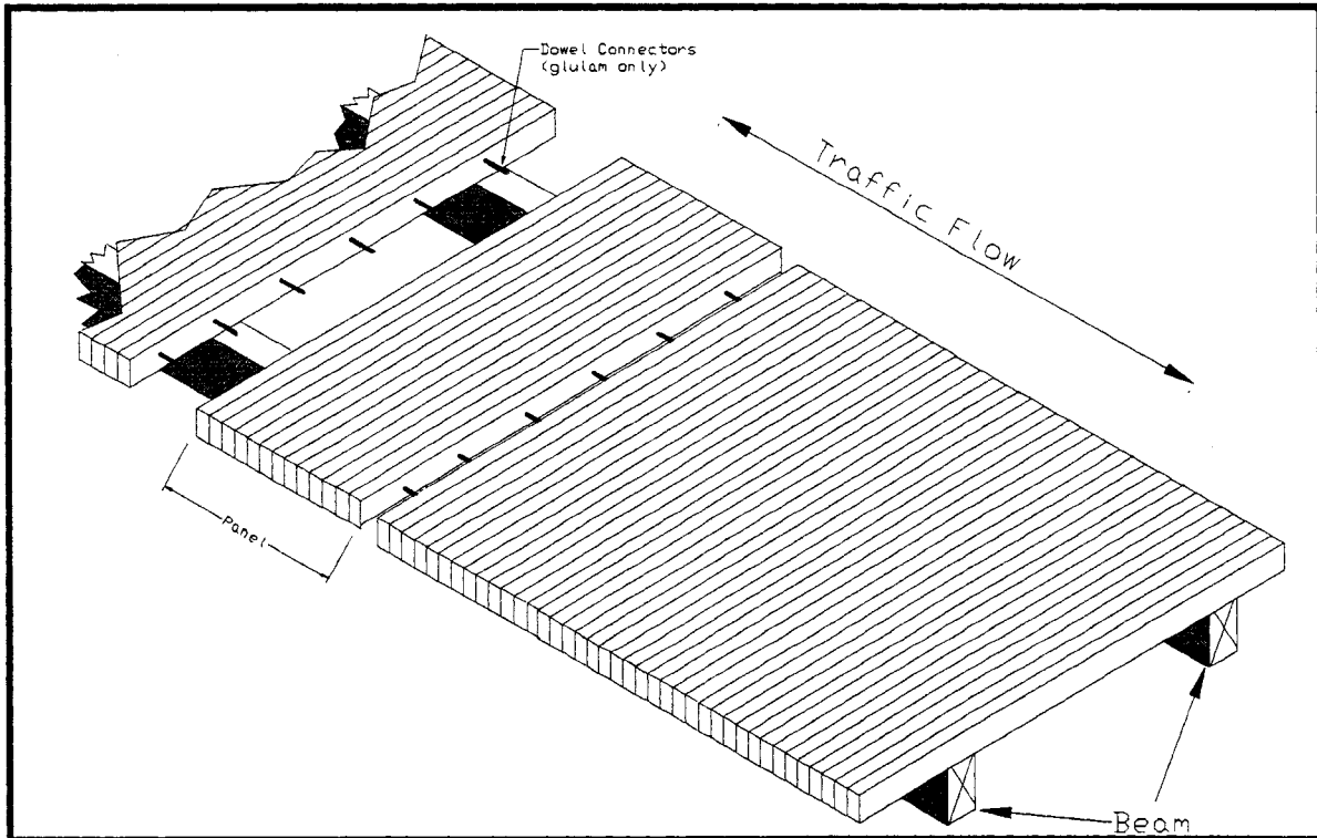
Figure 3.6 Beam Bridge with Transverse Laminated Deck
