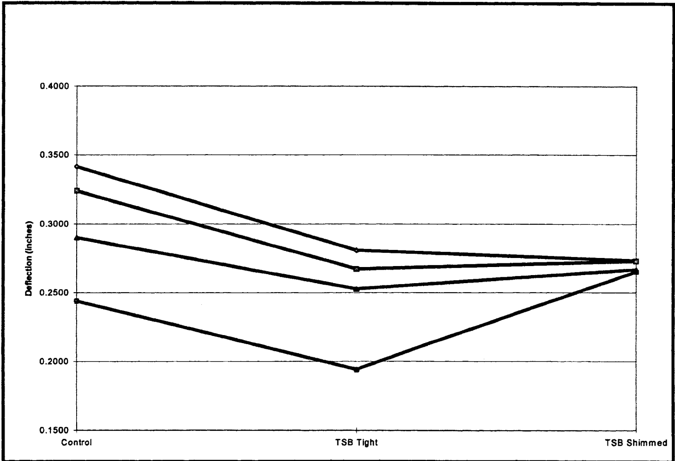
Figure 3.18 Deflection Change From Tightening of Transverse Stiffener Beams
