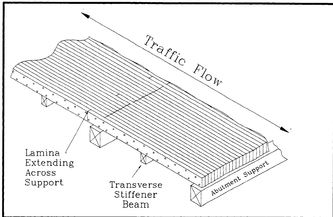
Figure 3.7 Simple Span Longitude Nail-Laminated Timber Deck (Cut-Away Representation)
