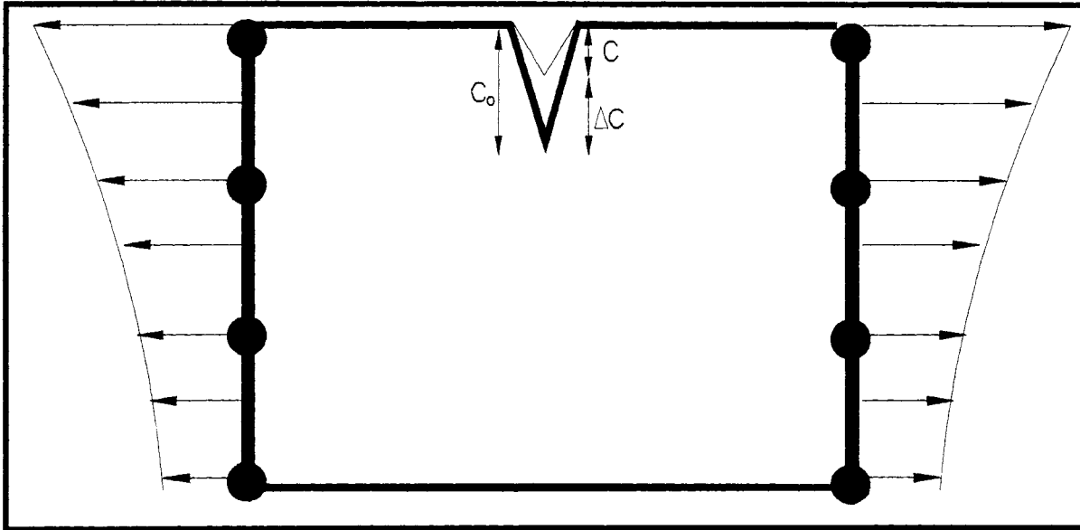
Figure 3.1 Schematic of Thermal Crack Model
