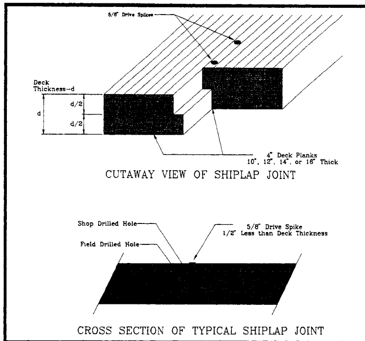
Figure 3.8 Illustration of Ship-lap Panel Joint
