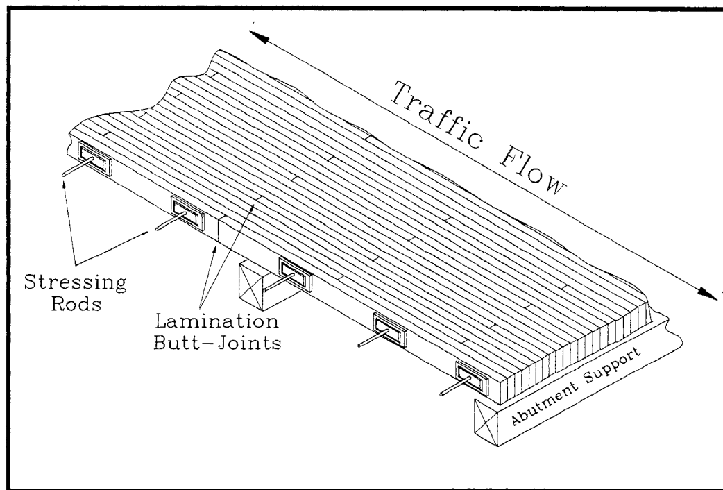
Figure 3.9 Stress-Laminated Superstructure (Cut-Away Representation)
