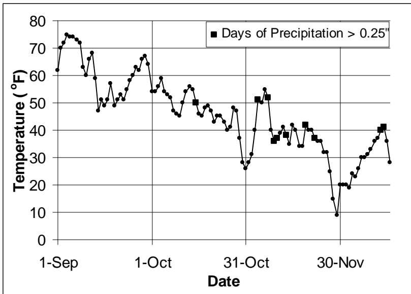
Figure G.5 Spokane County, WA, weather pattern during survey period
