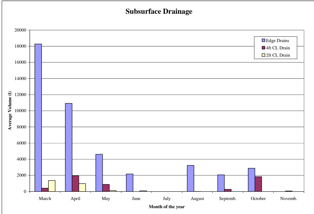
Figure 3.2 Average drained volumes from edge/centerline drains (l) – 2007
