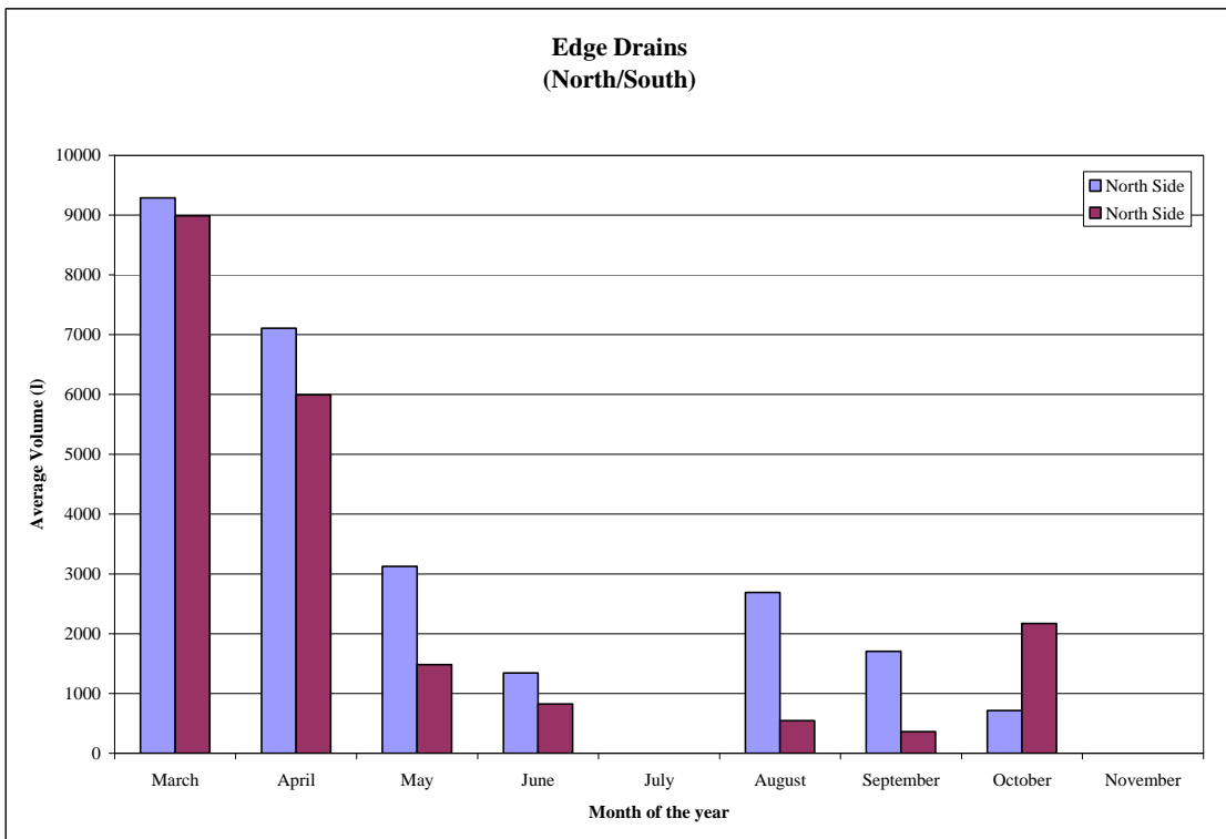
Figure 3.5 Average drained volumes from north/south edgedrains (l) - 2007
