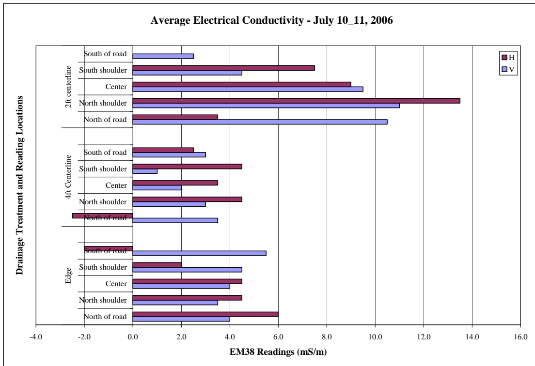
Figure 4.7 Differences in average E.C. (mS/m) by treatment and location – July 10-11, 2006
