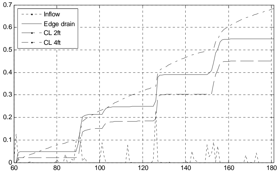
Figure 6.7 Cumulative water flux ( \text{m}^3 water / m roadway) from the three drain configurations for the case where the bottom of the soil profile is an impermeable boundary for the Prinsberg silty clay loam soil
