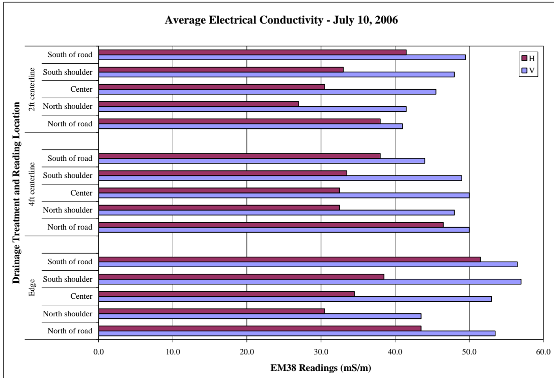
Figure 4.3 Average E.C. (mS/m) by treatment and location – July 10, 2006
