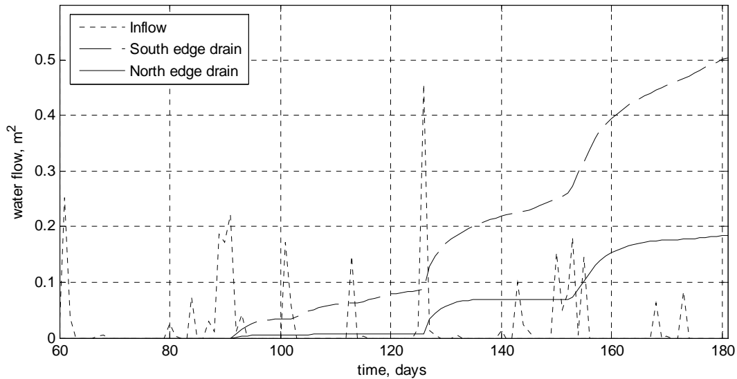
Figure 6.9 Cumulative water flux ( m^3 water /m roadway) from the edgedrain configuration for the north and south side edgedrains
