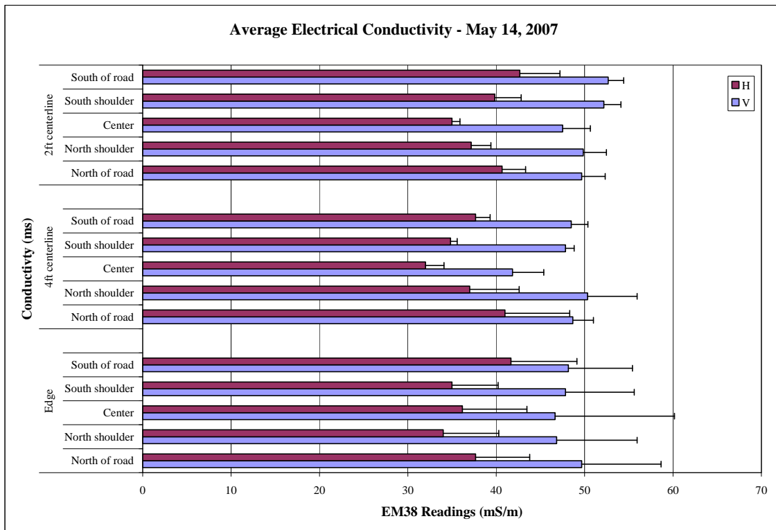
Figure 4.13 Average E.C. (mS/m) by treatment and location – May 14, 2007
