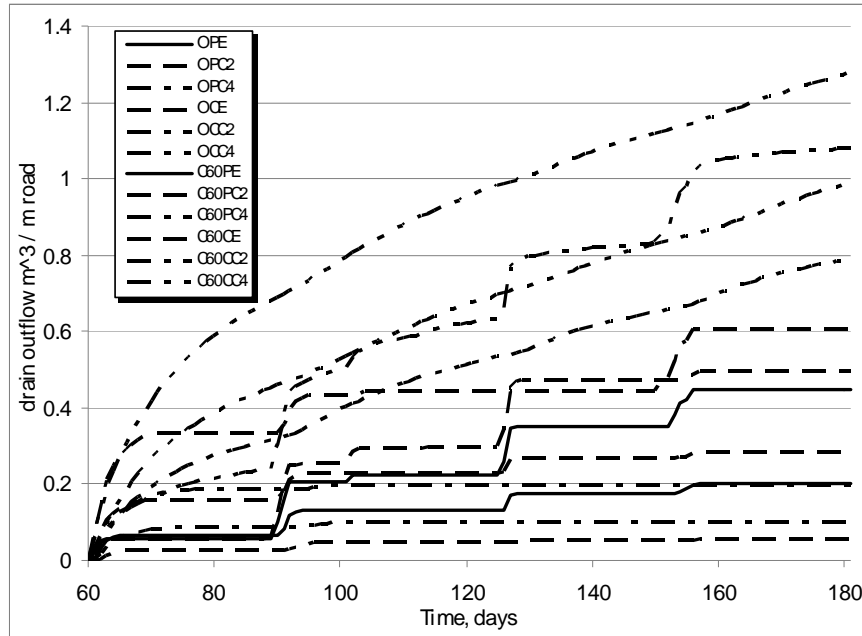
Figure 6.10 Cumulative drain outflow for the different drain configurations, subgrade soil types, and compaction condition
