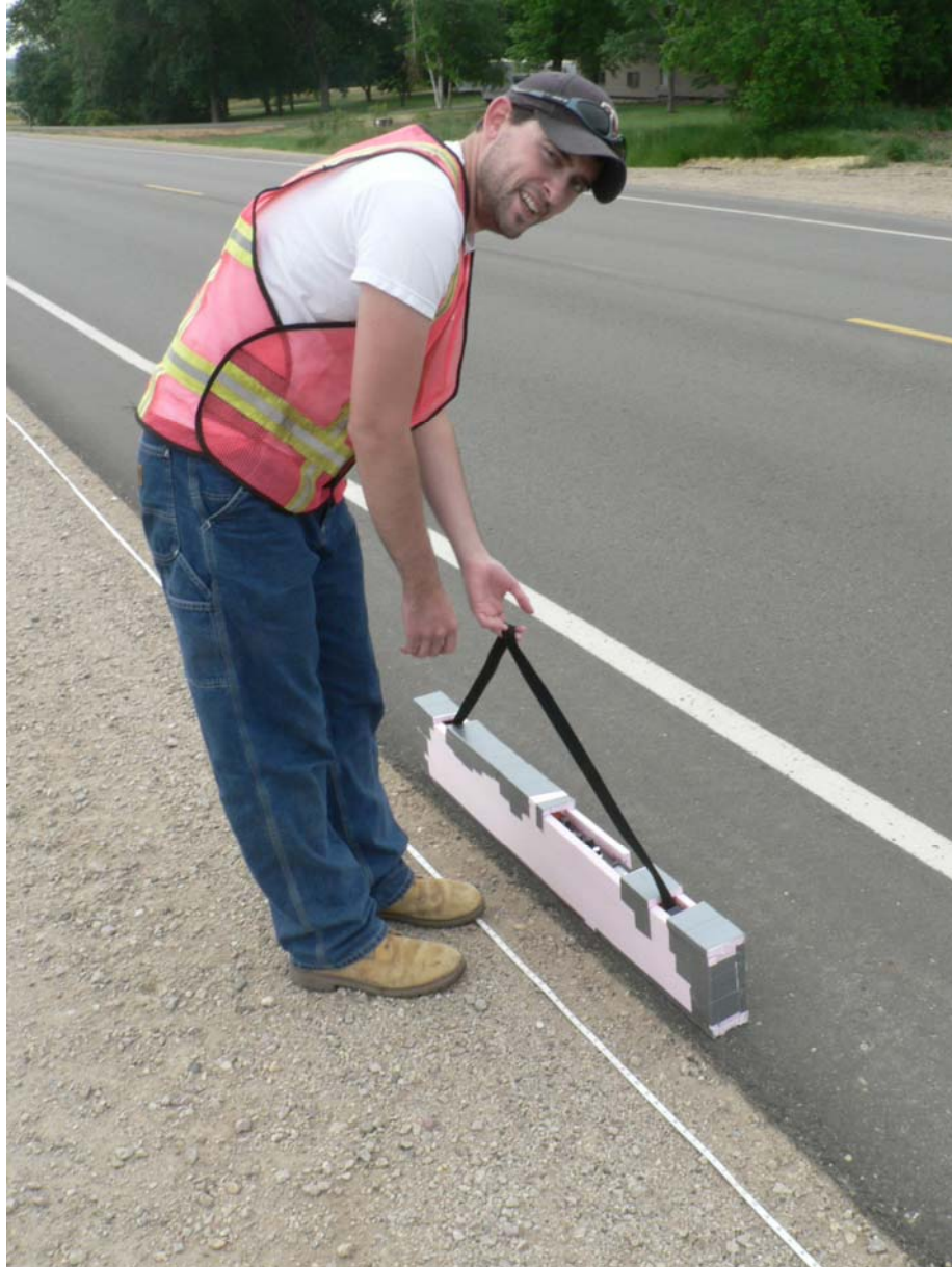
Figure A.14 The EM38 instrument in use
