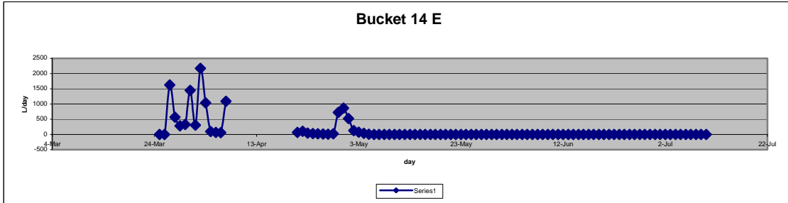
Figure A.8 Distribution of drainage for one of the edgedrain treatments for the early part of the 2006 season
