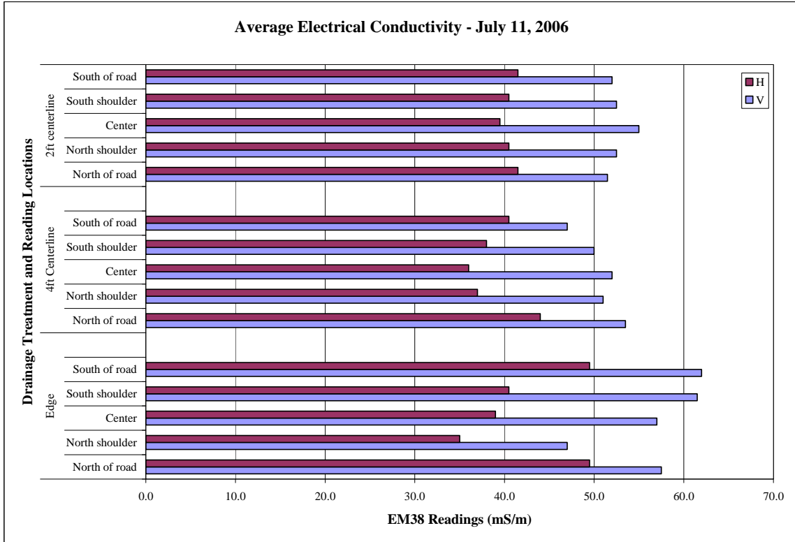
Figure 4.5 Average E.C. (mS/m) by treatment and location – July 11, 2006
