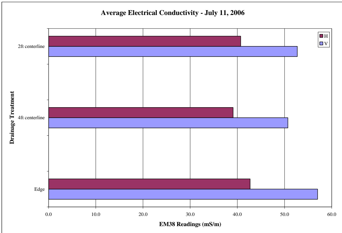
Figure 4.6 Average E.C. (mS/m) by treatment only – July 11, 2006
