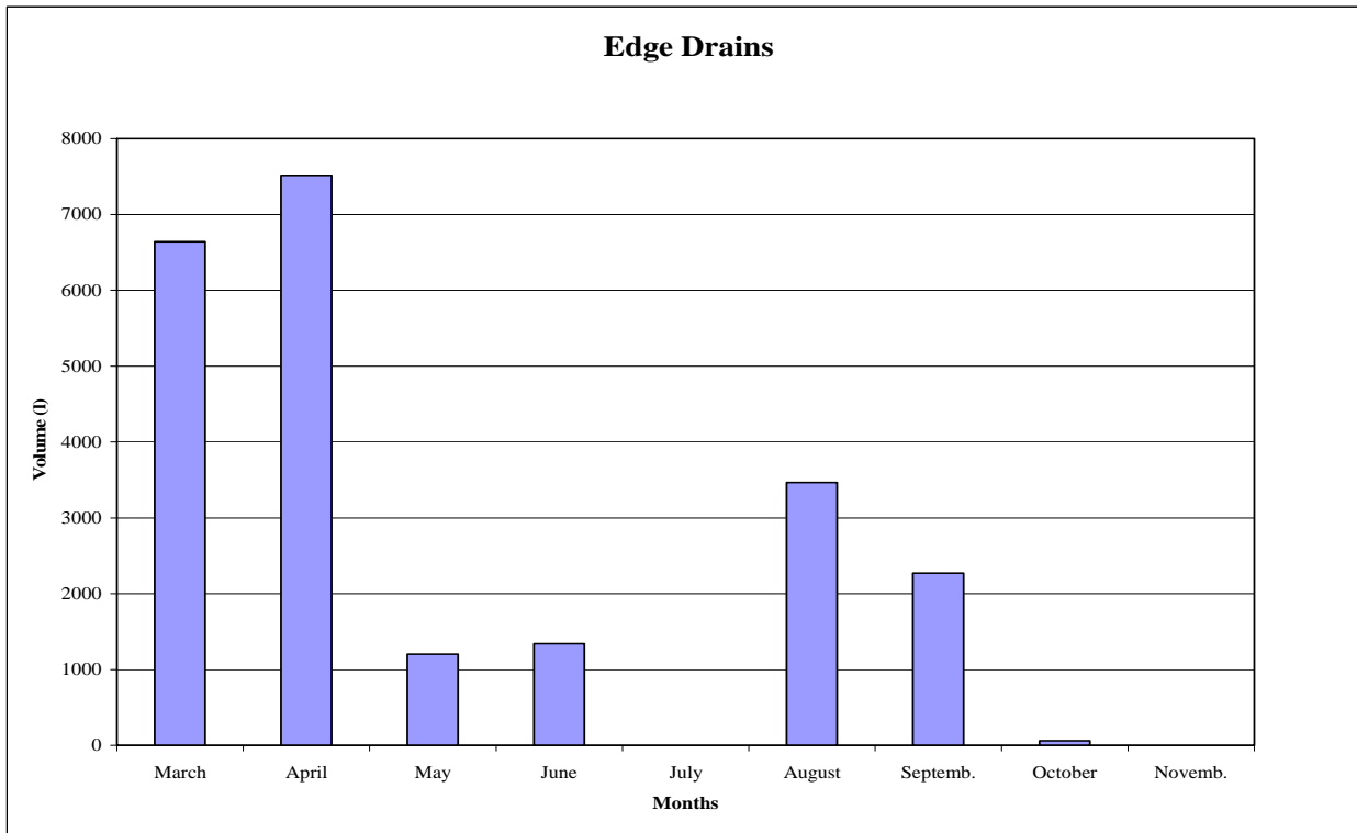
Figure B.1 Average volume drained from edgedrains (l) - 2006
