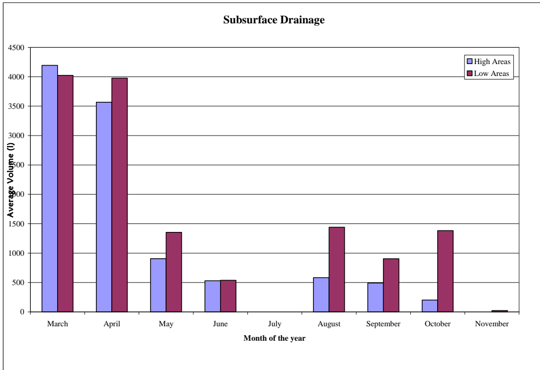
Figure 3.10 Average drained volume from high/low areas (l) – 2006/2007
