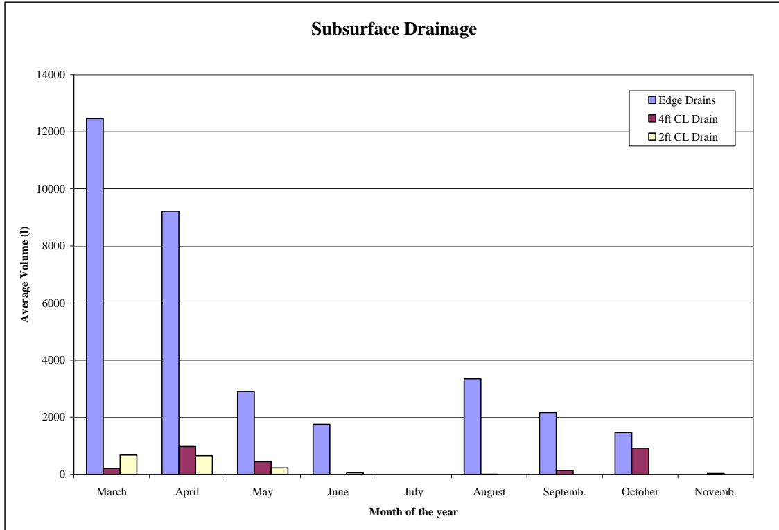
Figure 3.3 Average drained volumes from edge/centerline drains (l) – 2006/2007
