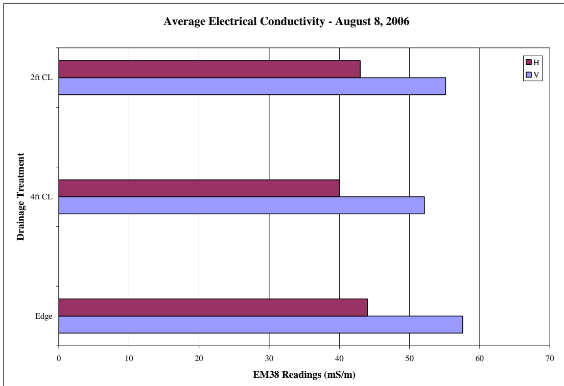
Figure 4.10 Average E.C. (mS/m) by location only – August 8, 2006
