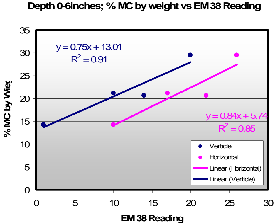
Figure A.11 EM38 reading for vertical and horizontal orientation of the instrument and the moisture content taken from the 0-6 inch depth increment
