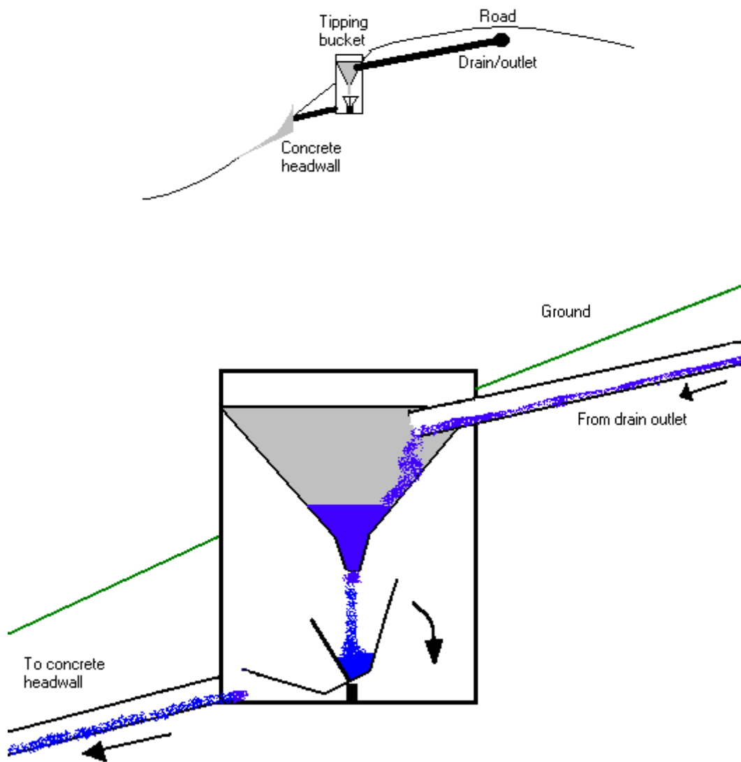
Figure 2.1 Tipping bucket system
