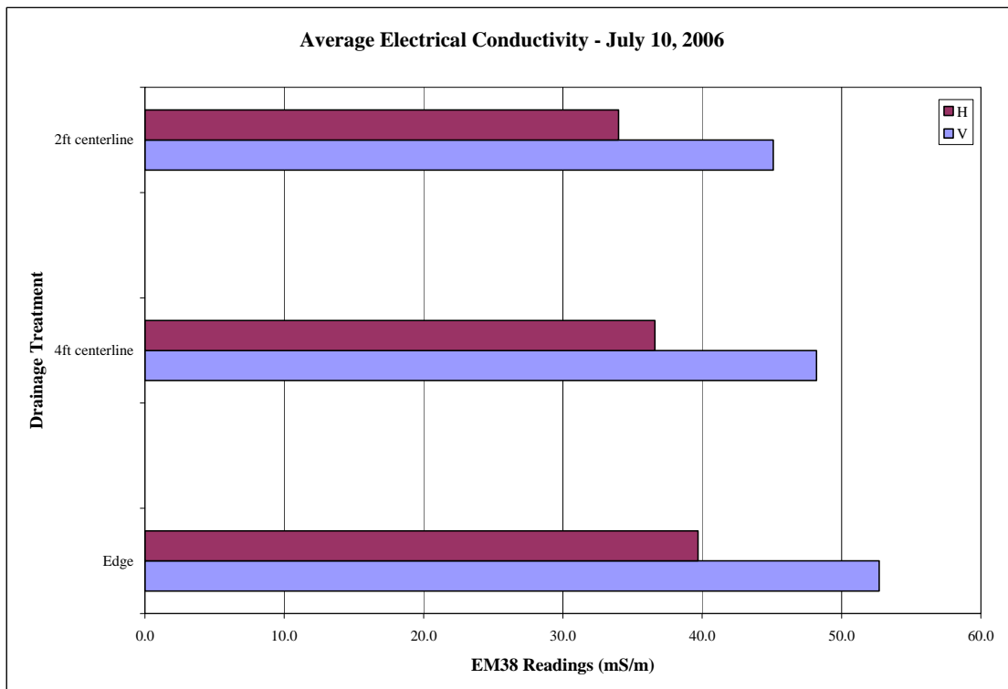
Figure 4.4 Average E.C. (mS/m) by treatment only – July 10, 2006
