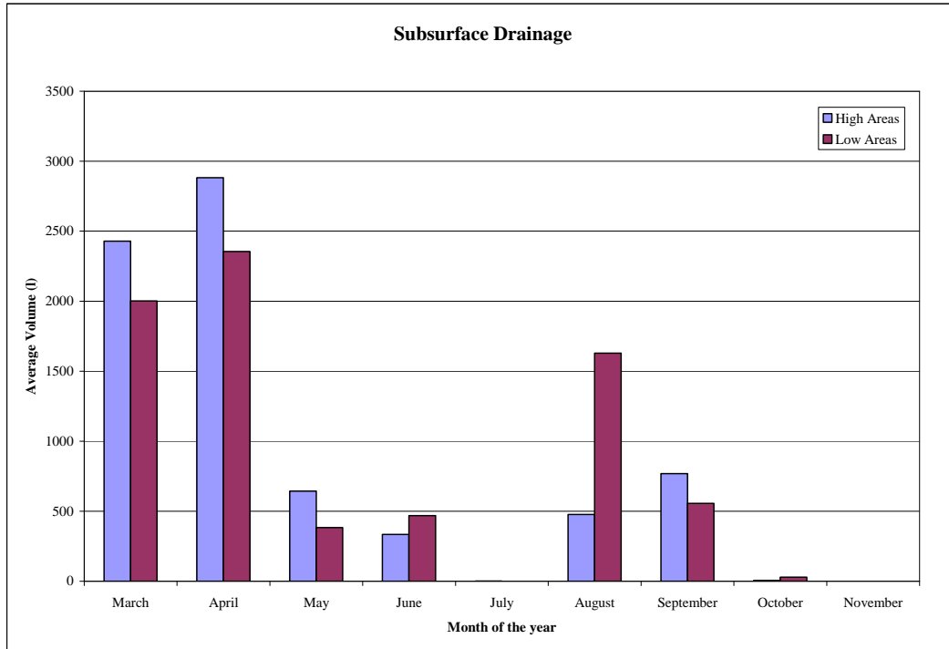
Figure 3.8 Average drained volumes from high/low areas (I) – 2006
