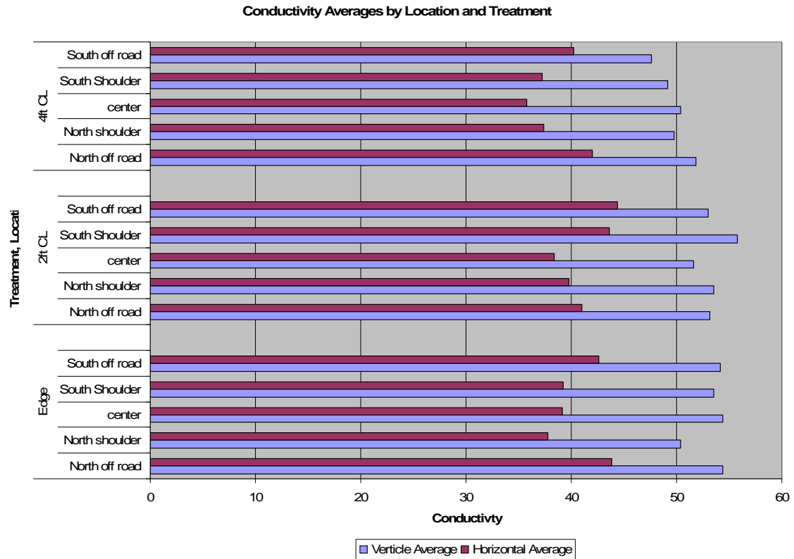
Figure A.15 Electrical conductivity readings from the EM38 for the various drainage treatments for both vertical and horizontal configuration
