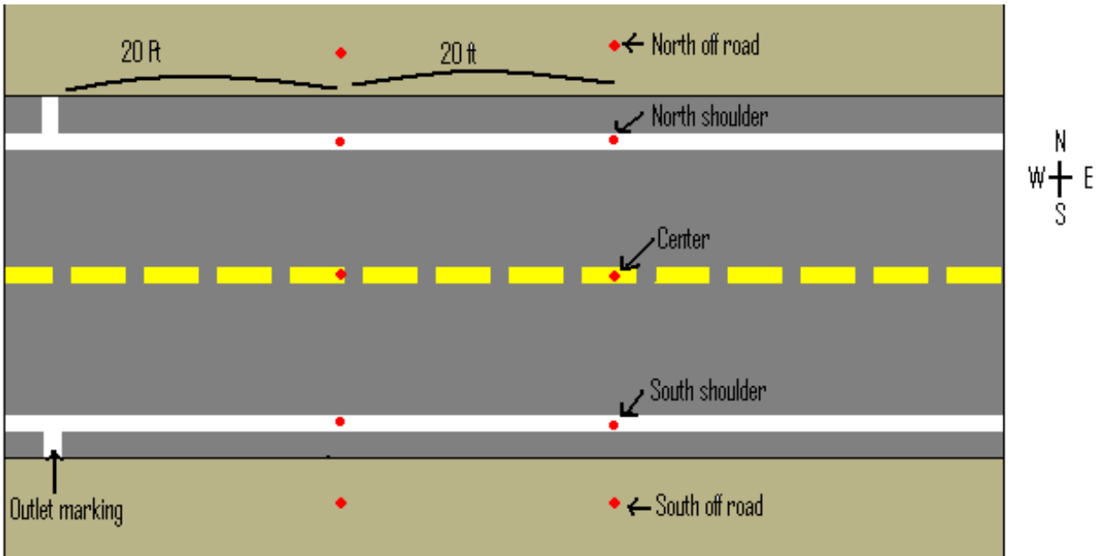
Figure A.12 Measurement scheme for the EM38 instrument at the Noble Co. Rd 35 site
