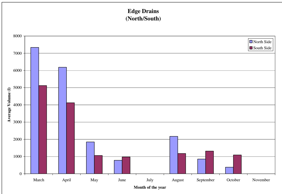
Figure 3.6 Average drained volumes from north/south edgedrains (l) – 2006-2007
