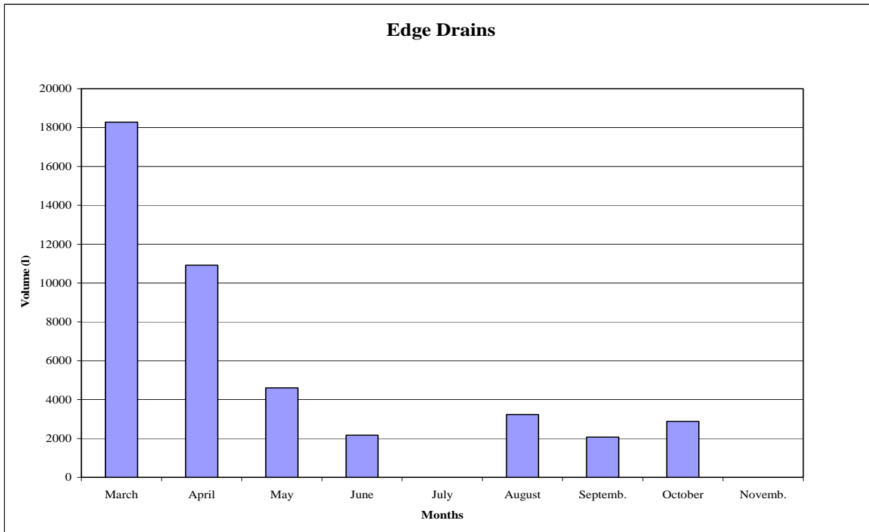
Figure B.4 Average volume drained from edgedrains (l) – 2007
