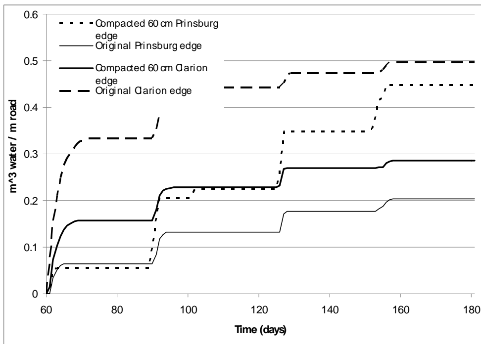
Figure 6.13 Cumulative drainage outflow for the two soil types and the two compaction conditions
