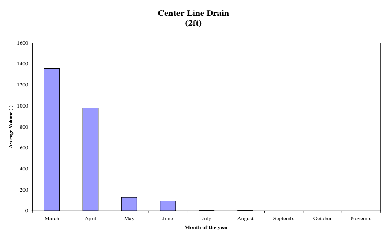
Figure B.6 Average volume drained from 2-ft centerline drains (l) – 2007
