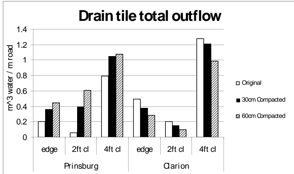
Figure 6.11 Effect of compaction on total drain outflow for different subgrade materials and compaction conditions
