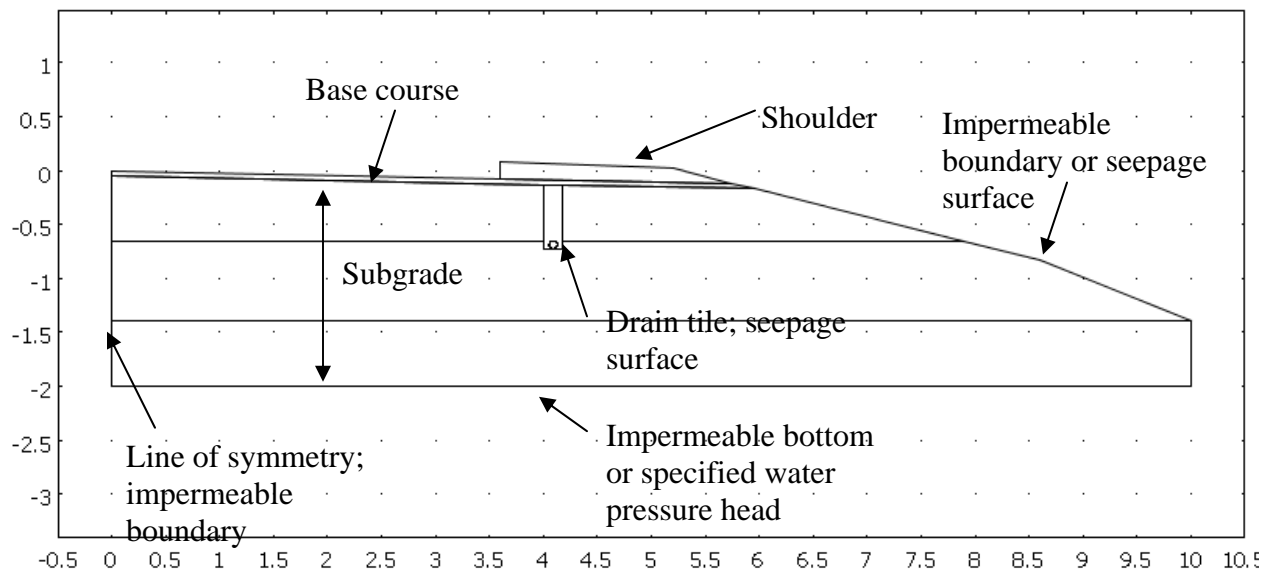
Figure 6.1 Typical cross-sectional view of edgedrain geometry
