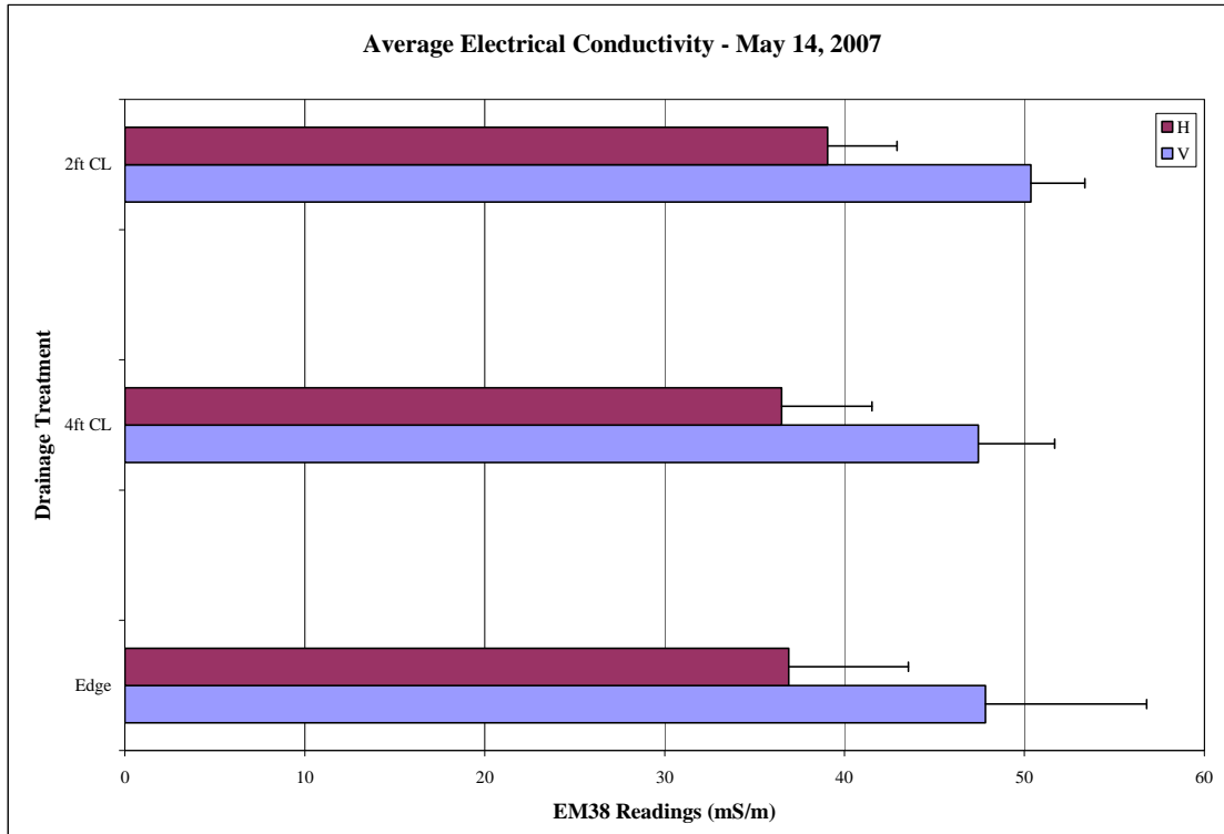
Figure 4.14 Average E.C. (mS/m) by treatment only – May 14, 2007
