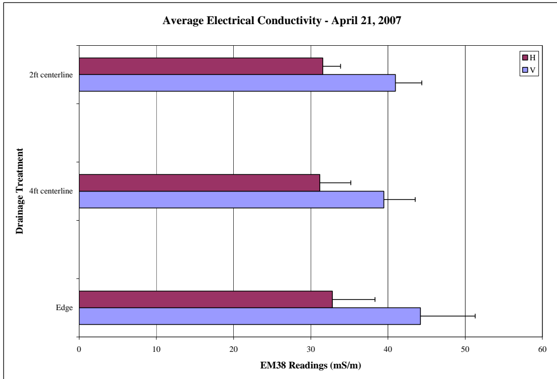
Figure 4.12 Average E.C. (mS/m) by treatment only – April 21, 2007
