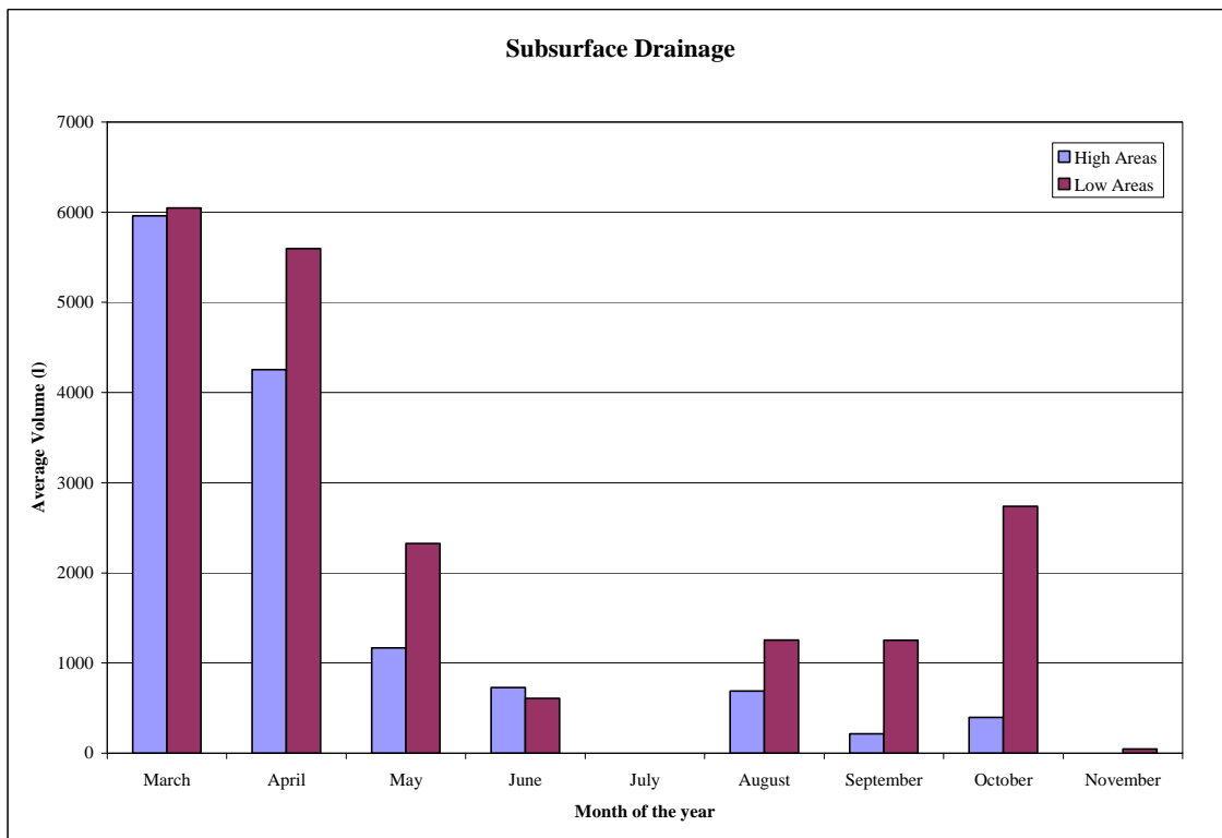
Figure 3.9 Average drained volumes from high/low areas (I) – 2007
