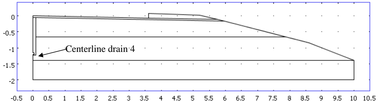
Figure 6.2 Typical cross-sectional view of centerline drain geometry; in this case the 4-ft depth drain. Other features pointed out in Figure 6.1 are the same for this drainage condition
