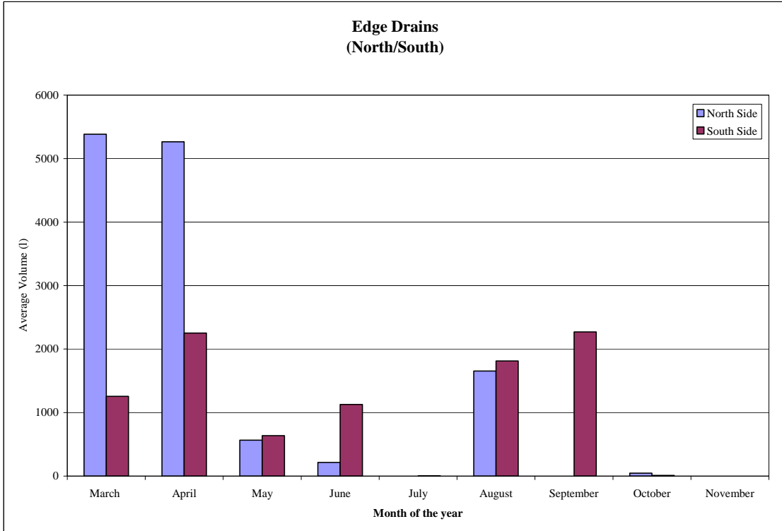
Figure 3.4 Average drained volumes from north/south edgedrains (l) - 2006
