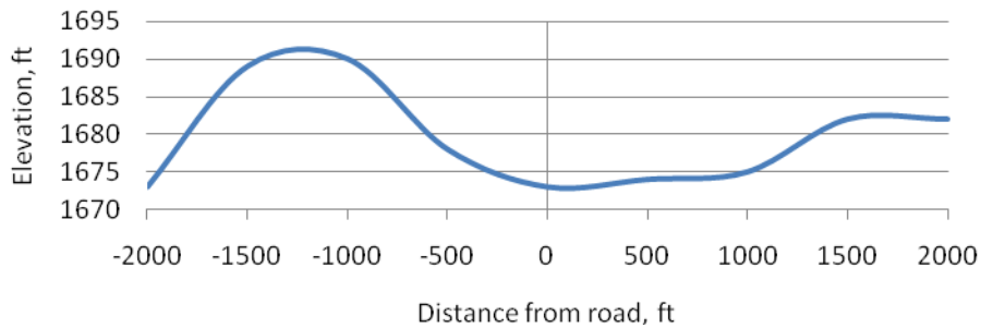
Figure 6.8 Elevation profile across the road at about 6.5 miles east of Rushmore. The south side of the road is to the left of the origin in the graphical plot
