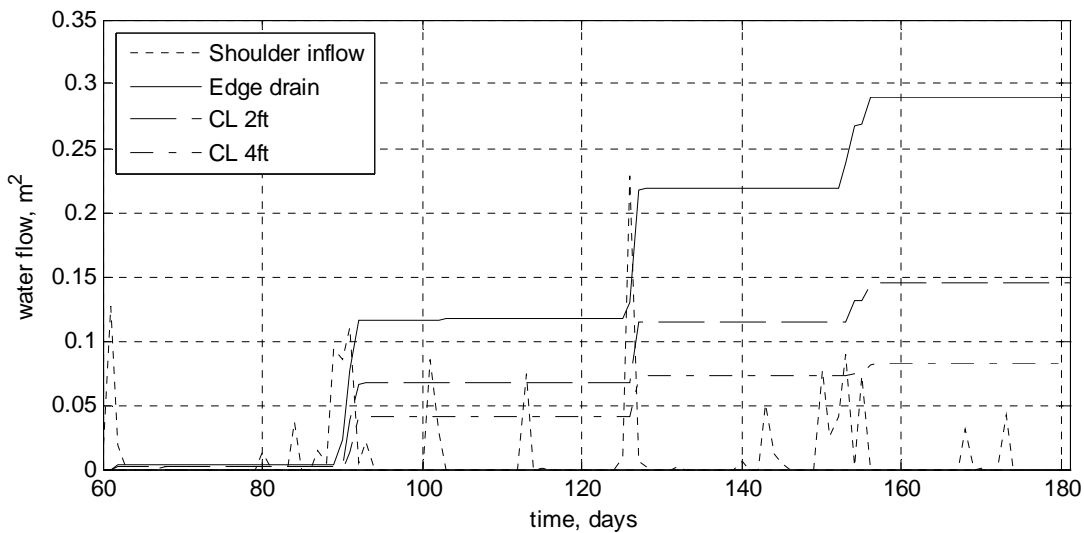
Figure 6.6 Cumulative water outflow (m 3 water /m roadway) from the three drain configurations for the case where the pressure is fixed at the bottom of the soil profile for the Prinsberg silty clay loam soil
