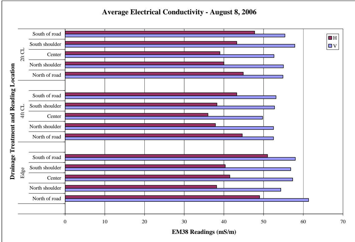
Figure 4.9 Average E.C. (mS/m) by treatment and location – August 8, 2006
