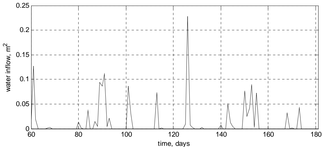
Figure 6.4 Rate of water infiltrating into the roadway shoulder ( \text{m}^3 water /m roadway)
