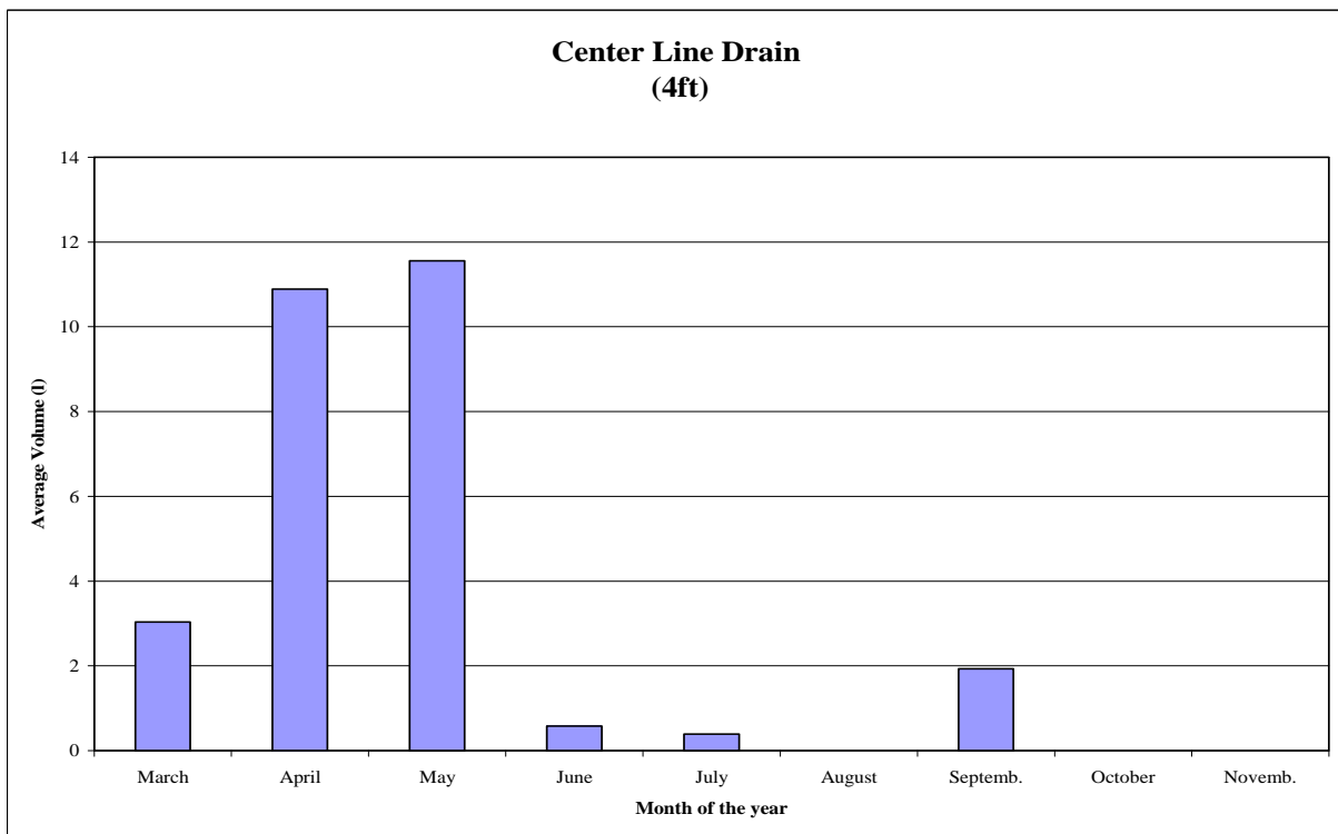
Figure B.2 Average volume drained from 4-ft centerline drains (l) - 2006
