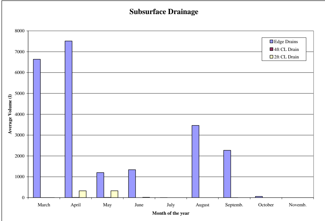
Figure 3.1 Average drained volumes for edge/centerline drains (l) – 2006
