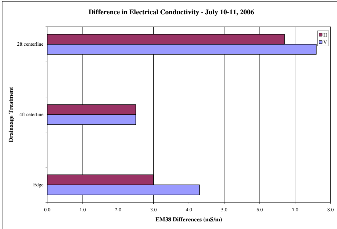
Figure 4.8 Differences in average E.C. (mS/m) by treatment only – July 10-11, 2006
