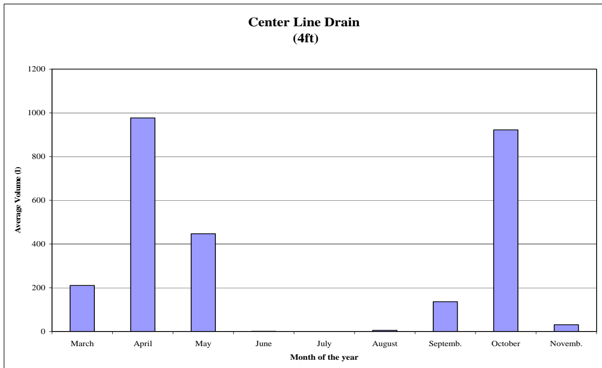
Figure B.8 Average volume drained from 4-ft centerline drains (l) – 2006-07
