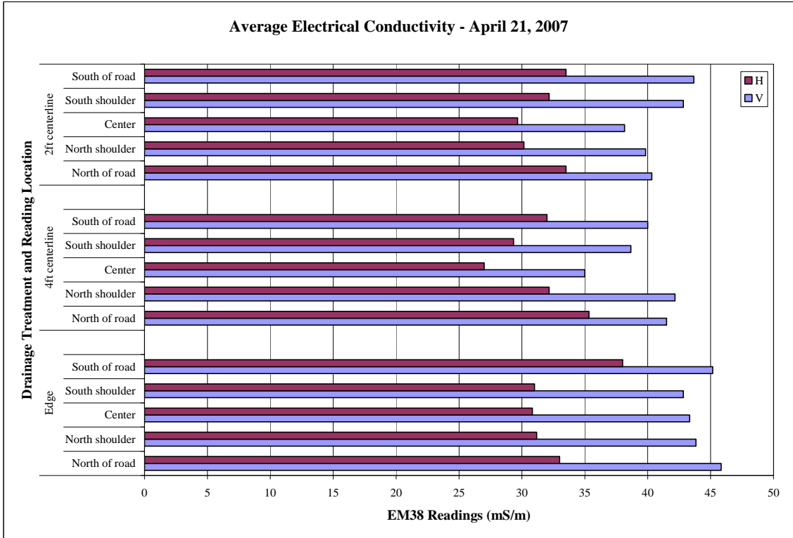
Figure 4.11 Average E.C. (mS/m) by treatment and location – April 21, 2007
