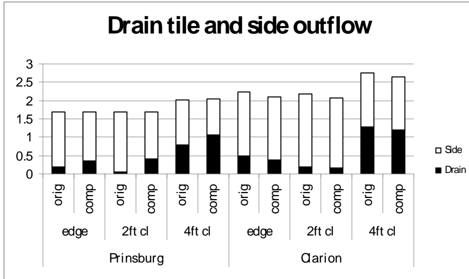
Figure 6.12 Total water outflow through drain tile and side of the domain for the various configurations
