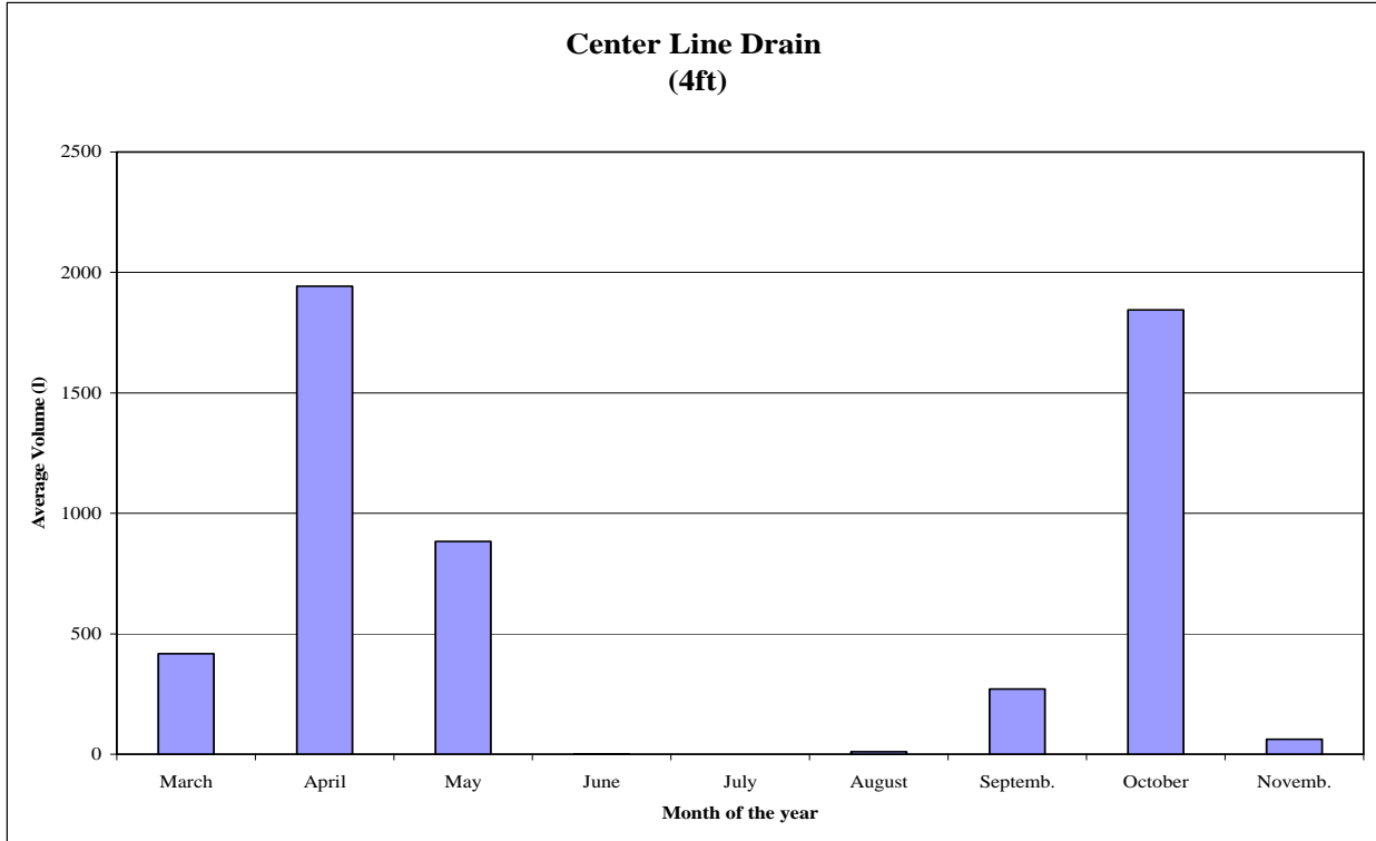
Figure B.5 Average volume drained from 4-ft centerline drains (l) – 2007
