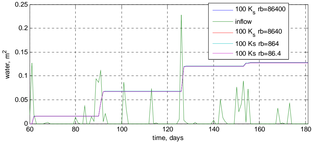
Figure 6.5 Simulation results for different values of empirical conductance parameter
