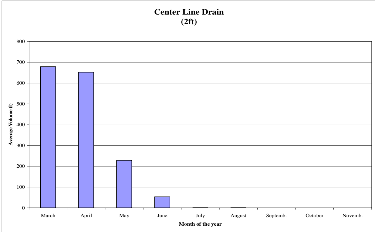
Figure B.9 Average volume drained from 2-ft centerline drains (l) – 2006-07
