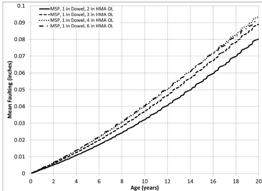
Figure 4-45: Influence of HMA overlay thickness on predicted faulting in HMA-PCC using TPF-5(149) modified MEPDG for HMA-PCC project with 1-inch dowels.
