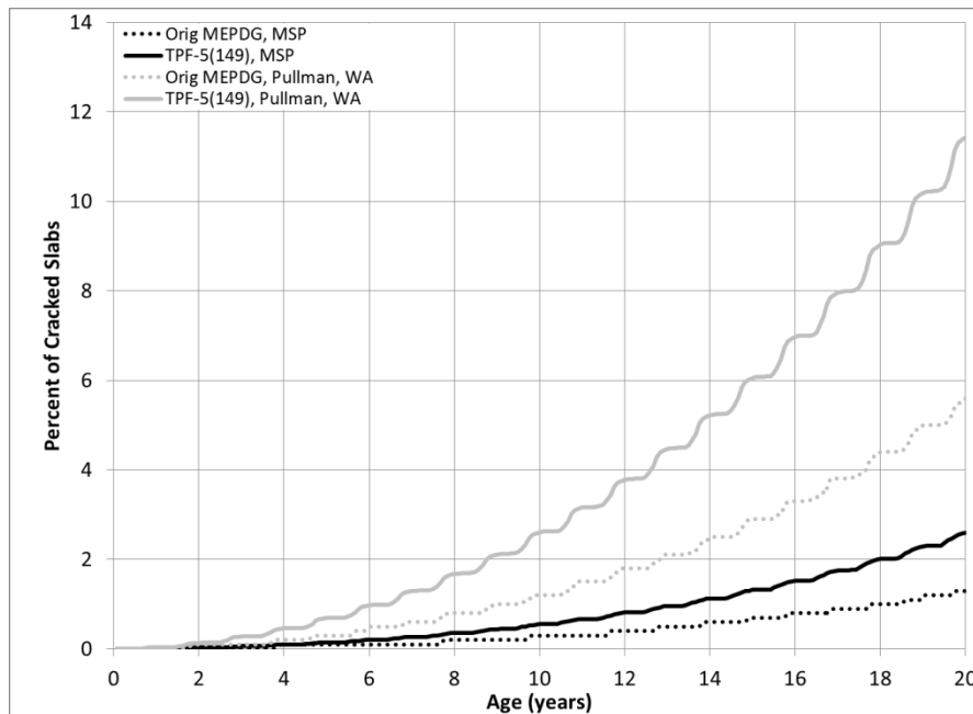
Figure 4-39. Predicted JPCP transverse cracking in HMA-PCC projects for Minneapolis, MN, and Pullman, WA, according to the original and TPF-5(149) modified MEDPG.
