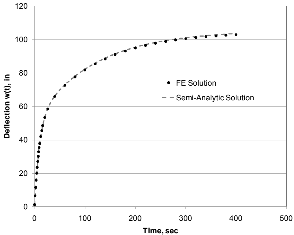
Figure 3-15: Comparison of deflections for a viscoelastic plate with simply supported corners.
