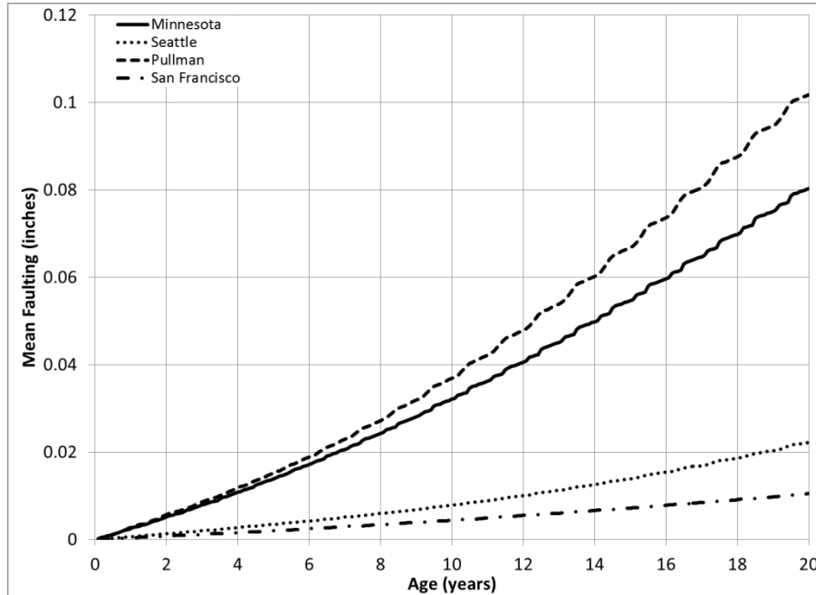
Figure 4-43: Influence of climate on predicted faulting in HMA-PCC using TPF-5(149) modified MEPDG for HMA-PCC project with 1-inch dowels.
