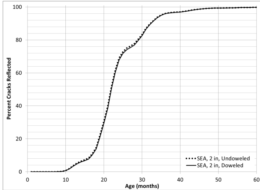
Figure 4-33: Influence of dowels on TPF-5(149) procedure for L+M+H severity reflective cracking for project using Seattle, WA, climate file.
