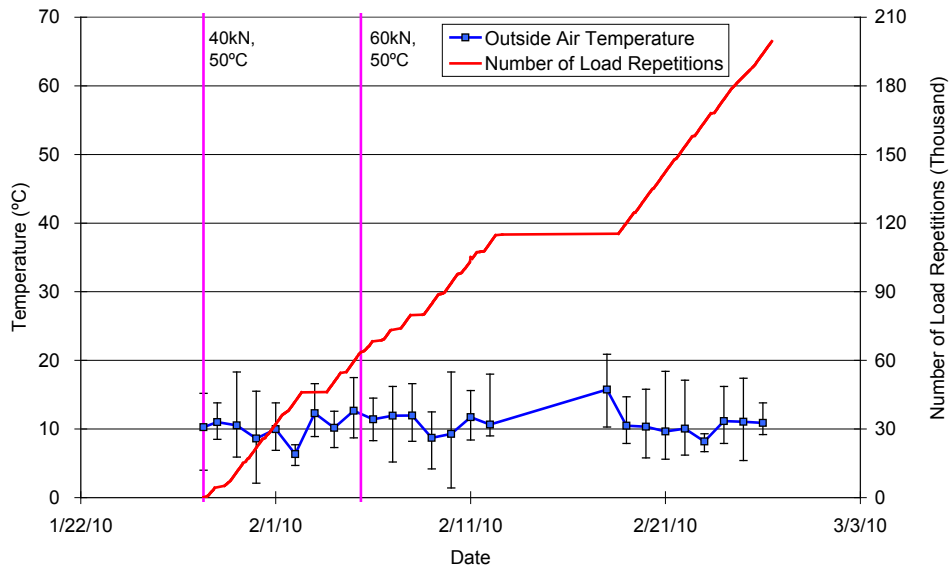
Figure 4-11: Daily average outside air temperatures.
