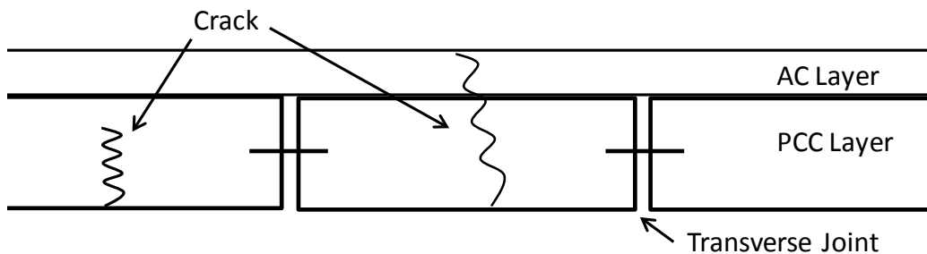
Figure 4-34: Propagation of fatigue cracking in a composite pavement.
