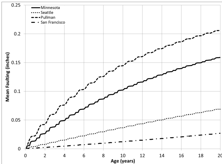
Figure 4-44: Influence of climate on predicted faulting in HMA-PCC using TPF-5(149) modified MEPDG for HMA-PCC project without dowels.
