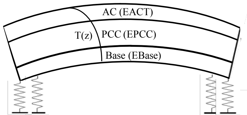
Figure 3-29: System 1 under positive temperature gradient T(z) only.
