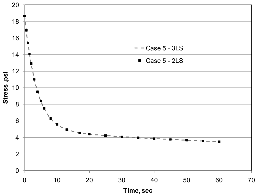
Figure 3-19: Stress versus time for case 5 using the viscoelastic FE model.
