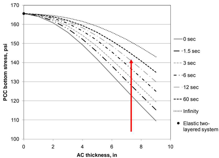
Figure 3-26: PCC bottom stresses versus AC thickness.
