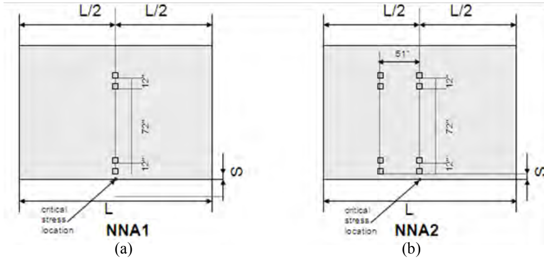
Figure 3-3: Structural model for (a) NNA1 (corresponding to single axle load) and (b) NNA2 (corresponding to tandem axle load).
