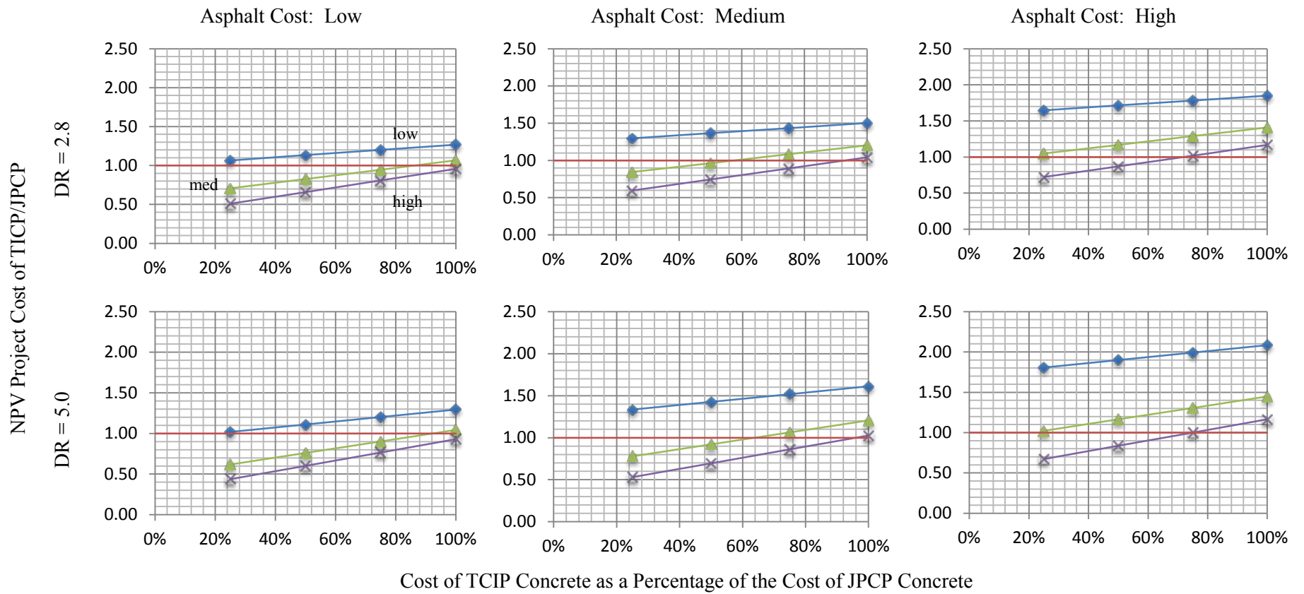
Figure 6-1: The ratio of the NPV of TICP to the NPV of JPCP, which are dependent on asphalt cost, JPCP concrete cost, TICP concrete cost as a percentage of JPCP concrete cost, and discount rate.
