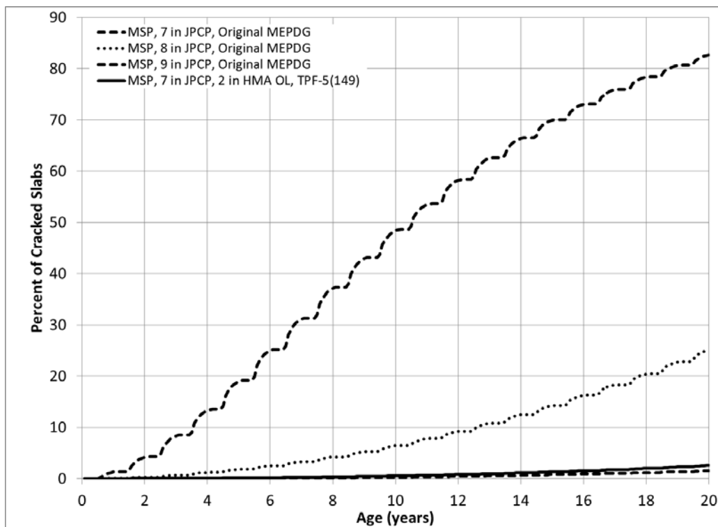
Figure 4-35: Predicted JPCP transverse performance for three JPCP projects (according to original MEPDG) and a HMA-PCC project (according to TPF-5(149) procedure).
