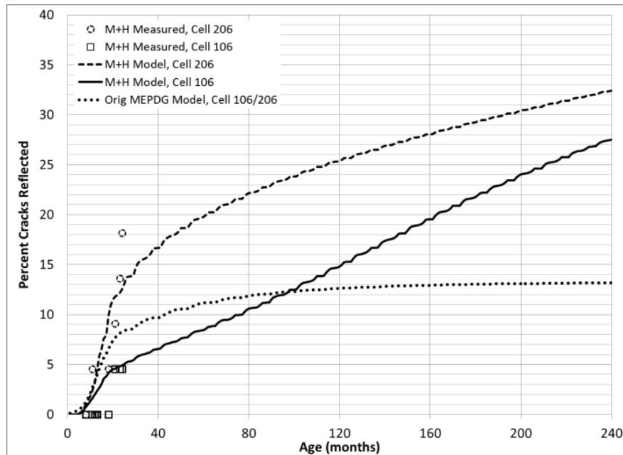
Figure 4-23: TPF-5(149) procedure predicted 20-year M+H severity reflective cracking performance for MnROAD Cells 106 and 206.
