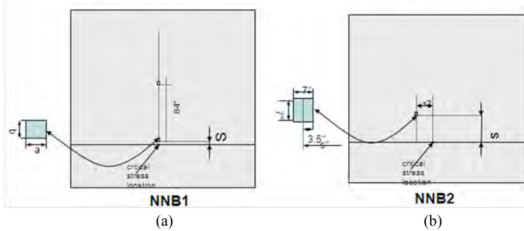
Figure 3-4: Structural model for (a) NNB1 (corresponding to single axle single wheel load) and (b) NNB2 (corresponding to single wheel load).
