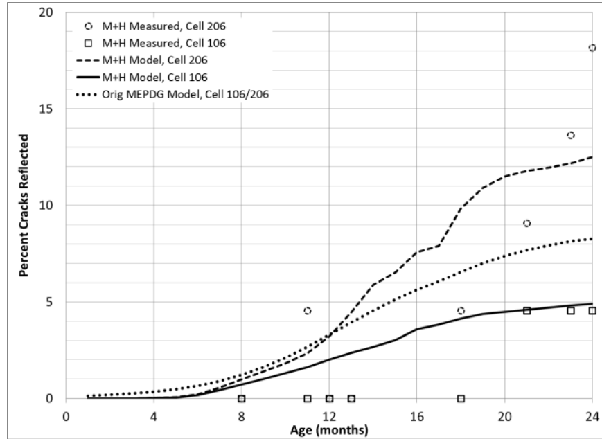
Figure 4-24: The first two years of MnROAD Medium and High (M+H) severity reflection cracking data versus TPF-5(149) modeled M+H performance and Original MEPDG modeled performance.
