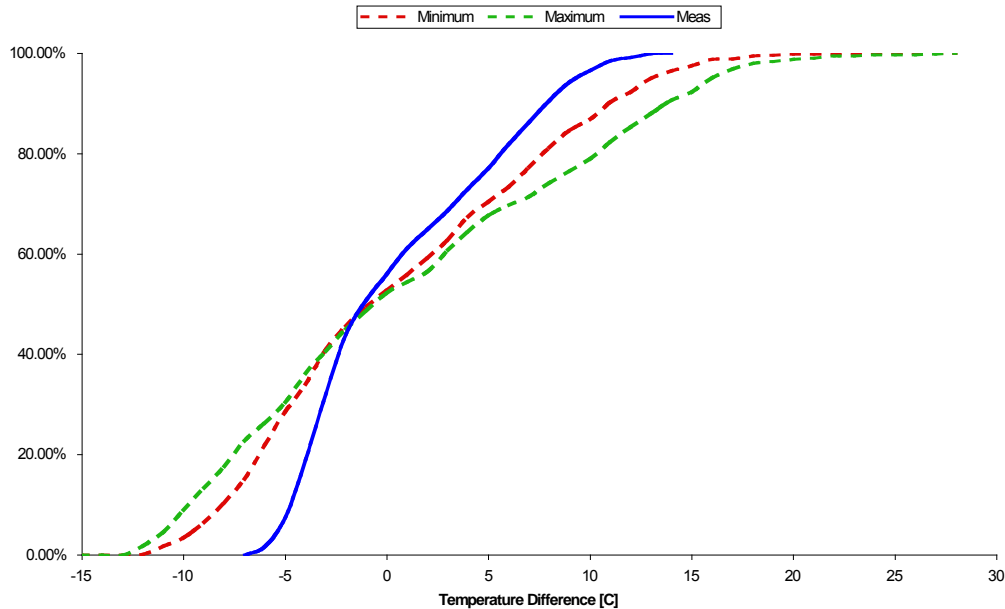
Figure 2-29: Measured versus modeled cumulative frequency distribution for thermal gradient through JPCP pavement in July with k = 0.85 \text{ BTU / hr-ft-}^\circ\text{F} .
