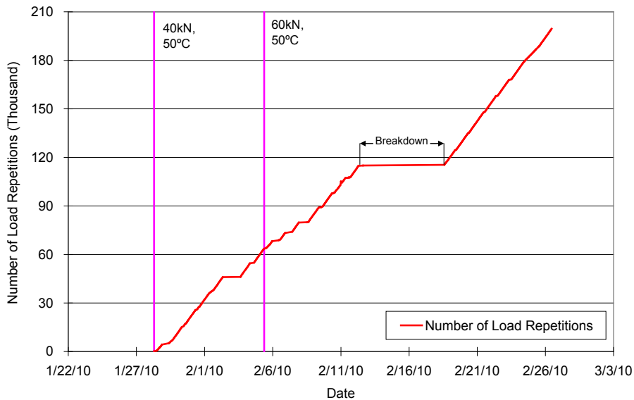
Figure 4-10: Section 609HB load history.
