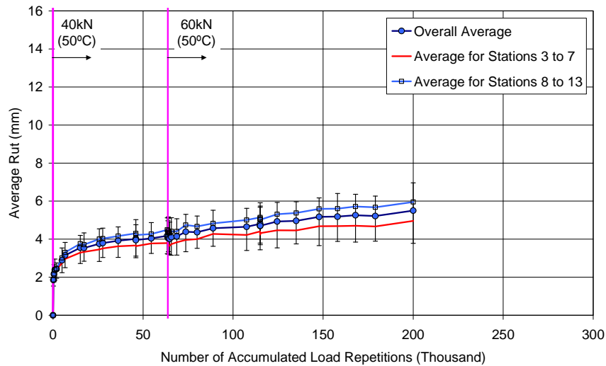
Figure 4-16: Average deformation for Section 609HB.
