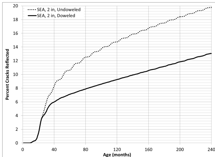
Figure 4-32: Influence of dowels on TPF-5(149) procedure for M+H severity reflective cracking for project using Seattle, WA, climate file.
