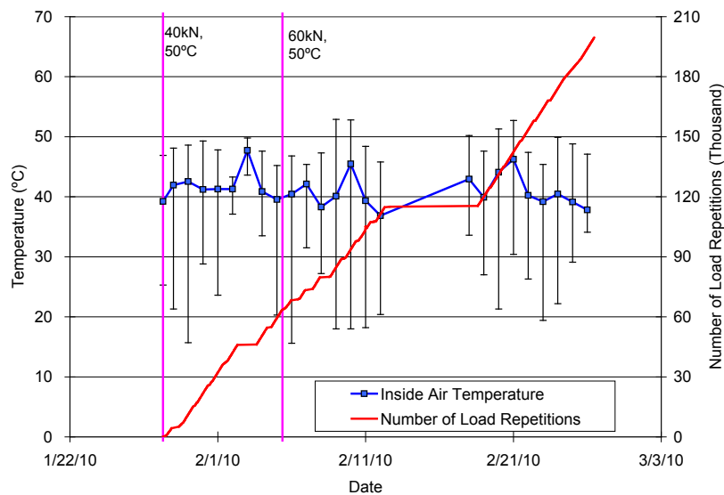
Figure 4-12: Daily average inside air temperatures.
