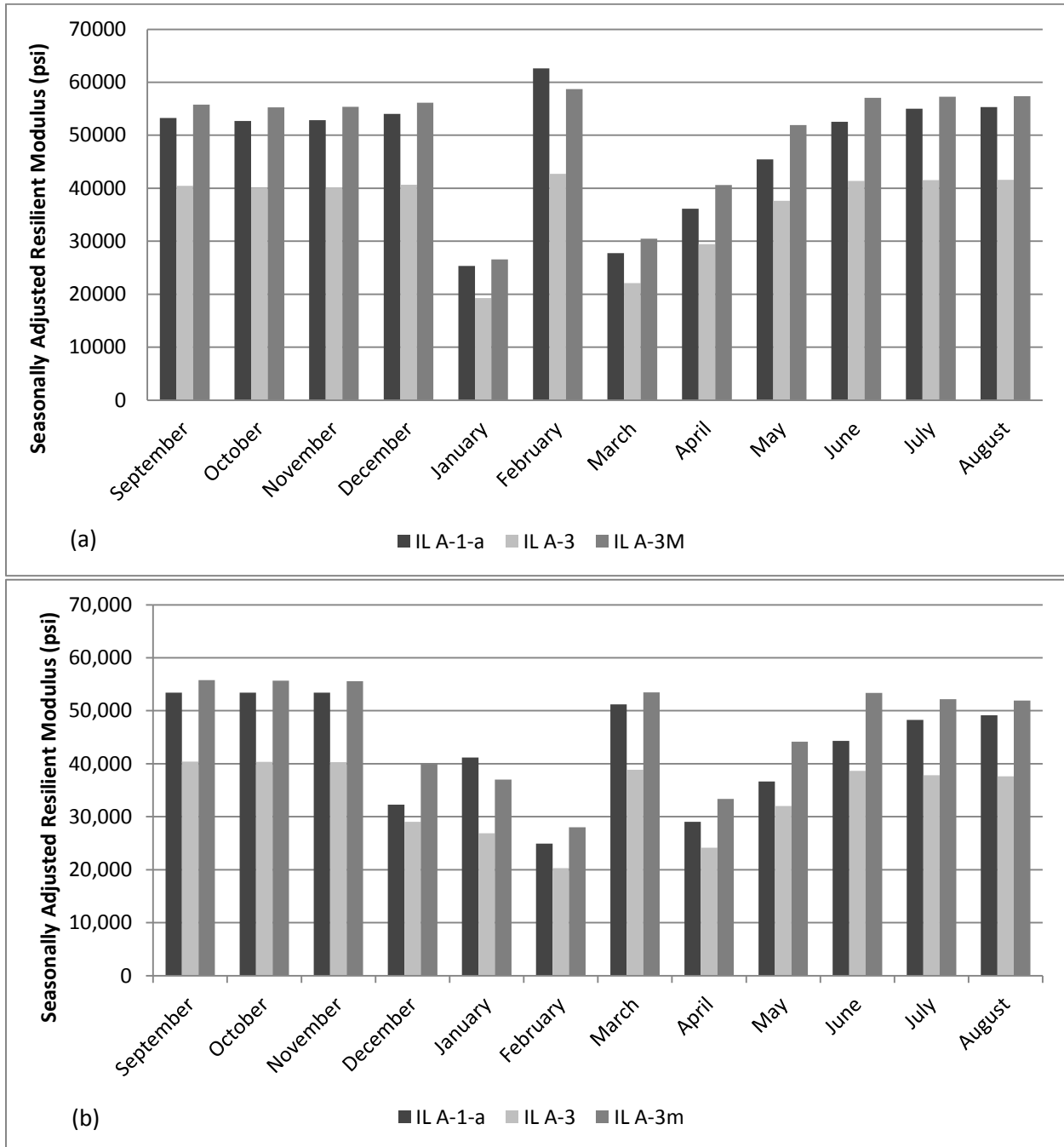
Figure 2-39: Seasonally adjusted resilient modulus of the base layer under a flexible pavement with different bases and an A-6 subgrade in Champaign analyzed with a) the MEPDG and b) DARWin-ME.
