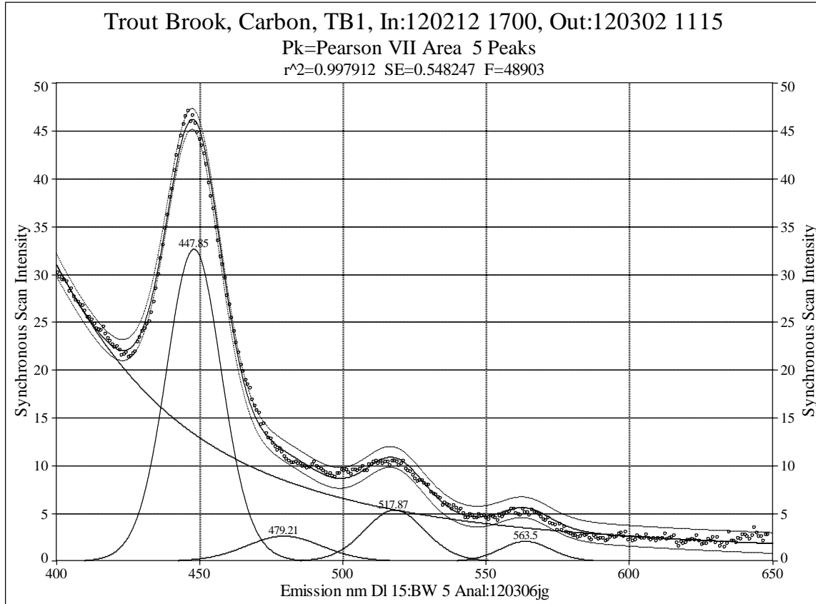
Graph 10: Fluorescent Spectrum, TB1 Bug, 12 Feb to 2 Mar 2012
