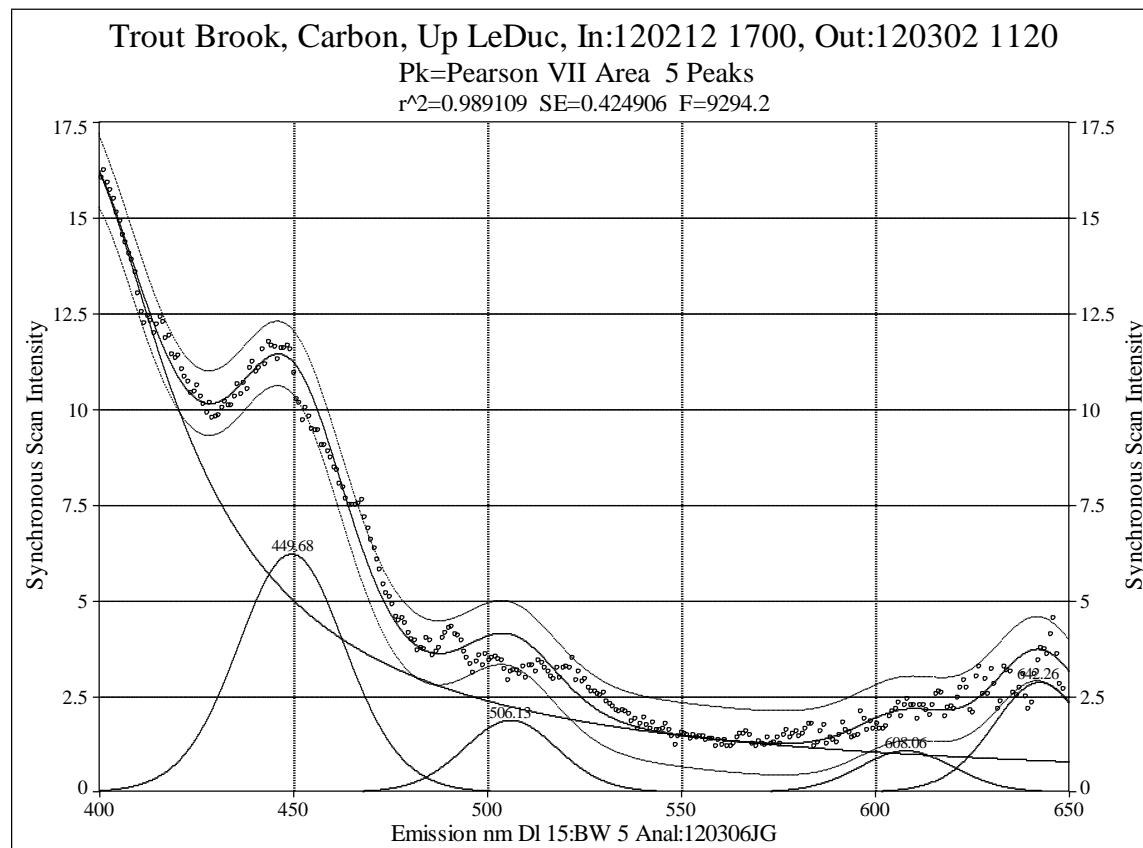
Graph 8: Fluorescent Spectrum, Upstream of LeDuc Bug, 12 Feb to 2 March 2012
