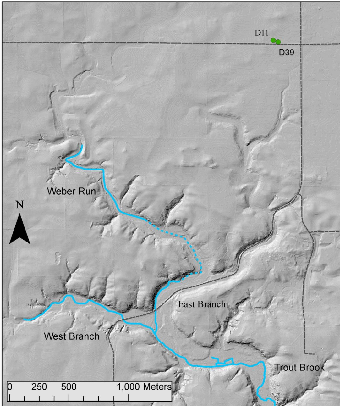
Figure 21: Trout Brook in the SE portion of Douglas Township, Dakota County, Minnesota. Enlarged portion of the 2008 LiDAR shaded relief DEM basemap. Light blue lines denote perennial running water in Weber Run, the East and West Branches of upper Trout Brook, and the Main Stream of Trout Brook. Light blue dashes denote an ephemeral reach. Dashed gray lines denote roads. The two green dots represent sinkholes that were discovered after the 14-15 June 2012 flood event. See Figures 22 and 23.
