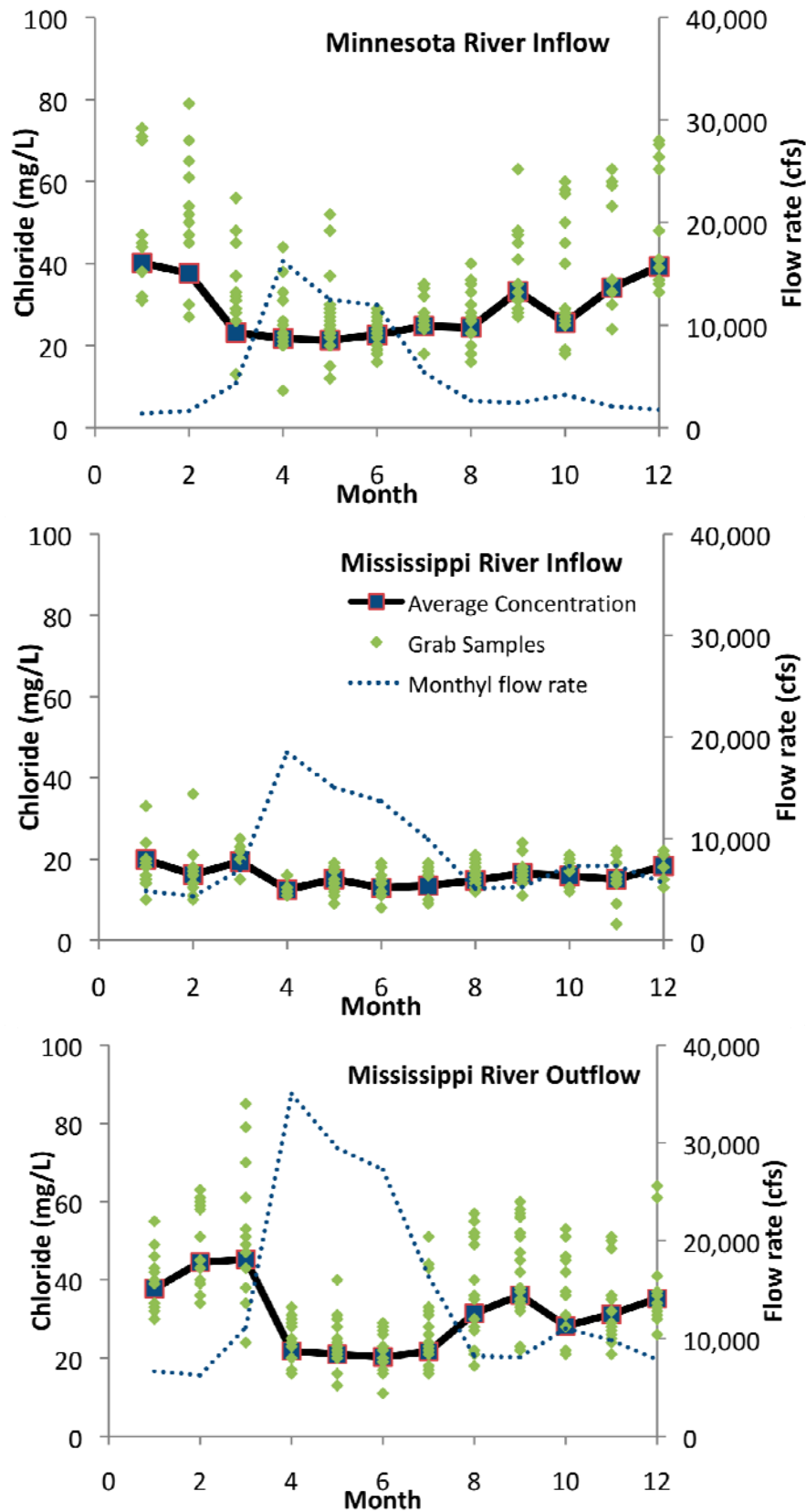
Figure 3.3 Chloride concentrations in individual grab samples from the Minnesota and Mississippi Rivers. Flow-weighted average monthly values for concentrations and flow rates are plotted as solid and dotted lines, respectively. All values are from measurements taken between the years 2000 and 2007.
