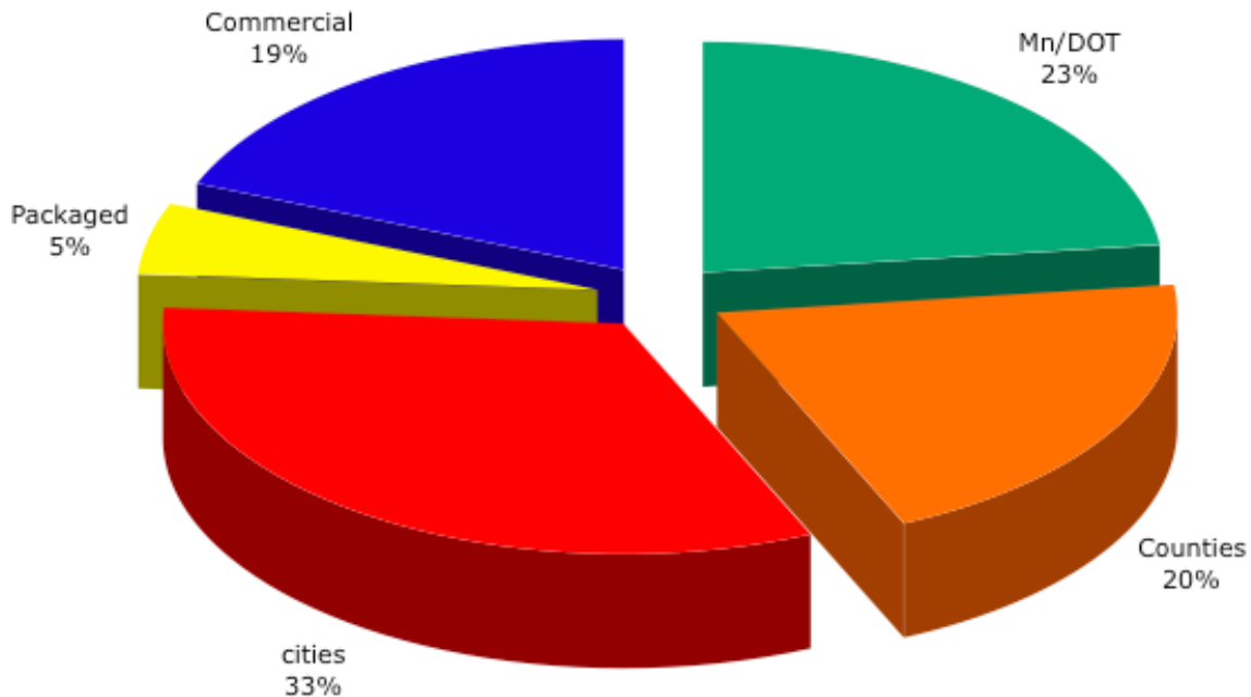
Figure 2.1 Distribution of road salt applications in the Twin Cities Metropolitan Area (TCMA). The total amount of road salt applied is approximately 350,000 (short) tons per season.
