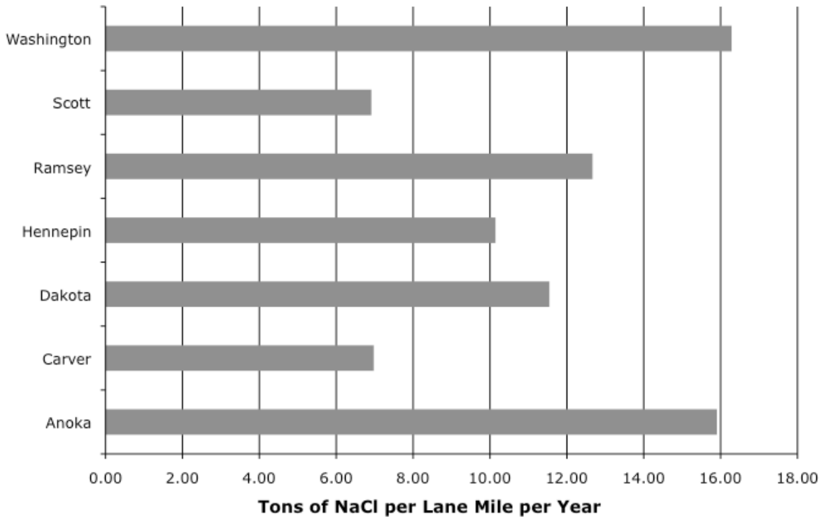
Figure 2.7 Annual road salt use by counties in the TCMA per lane mile.
