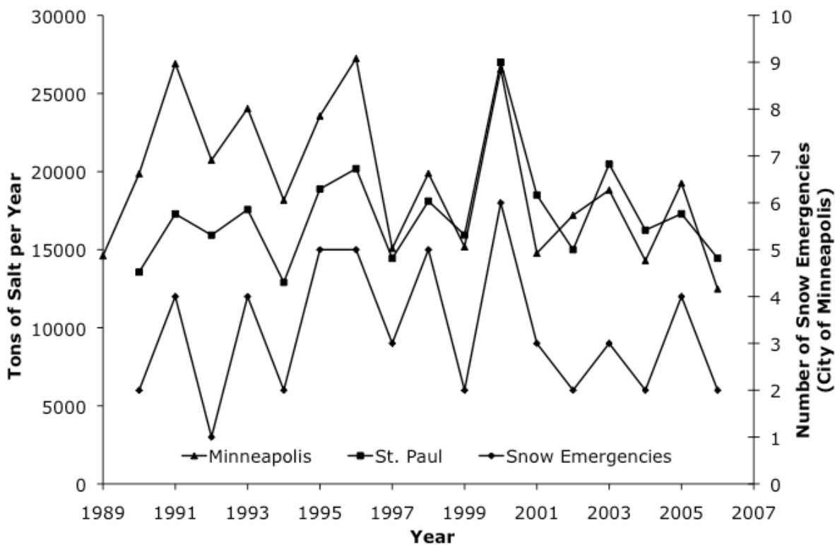
Figure 2.2 Road salt use (tons per season) and declared snow emergencies in Minneapolis and St. Paul.
