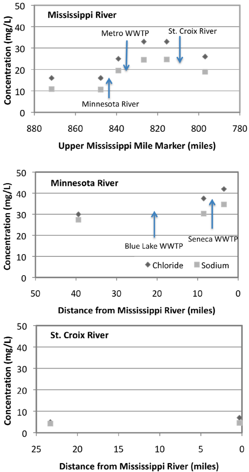
Figure 3.2 Median concentrations (2000-2008) of sodium and chloride for the three major rivers in the Twin Cities Metropolitan area.
