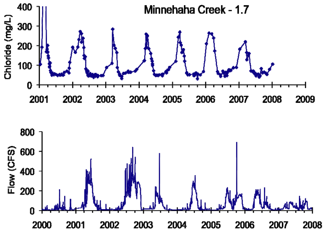
Figure 4.1 Chloride concentrations in Minnehaha Creek (1.7 miles from its outlet into the Mississippi River).
