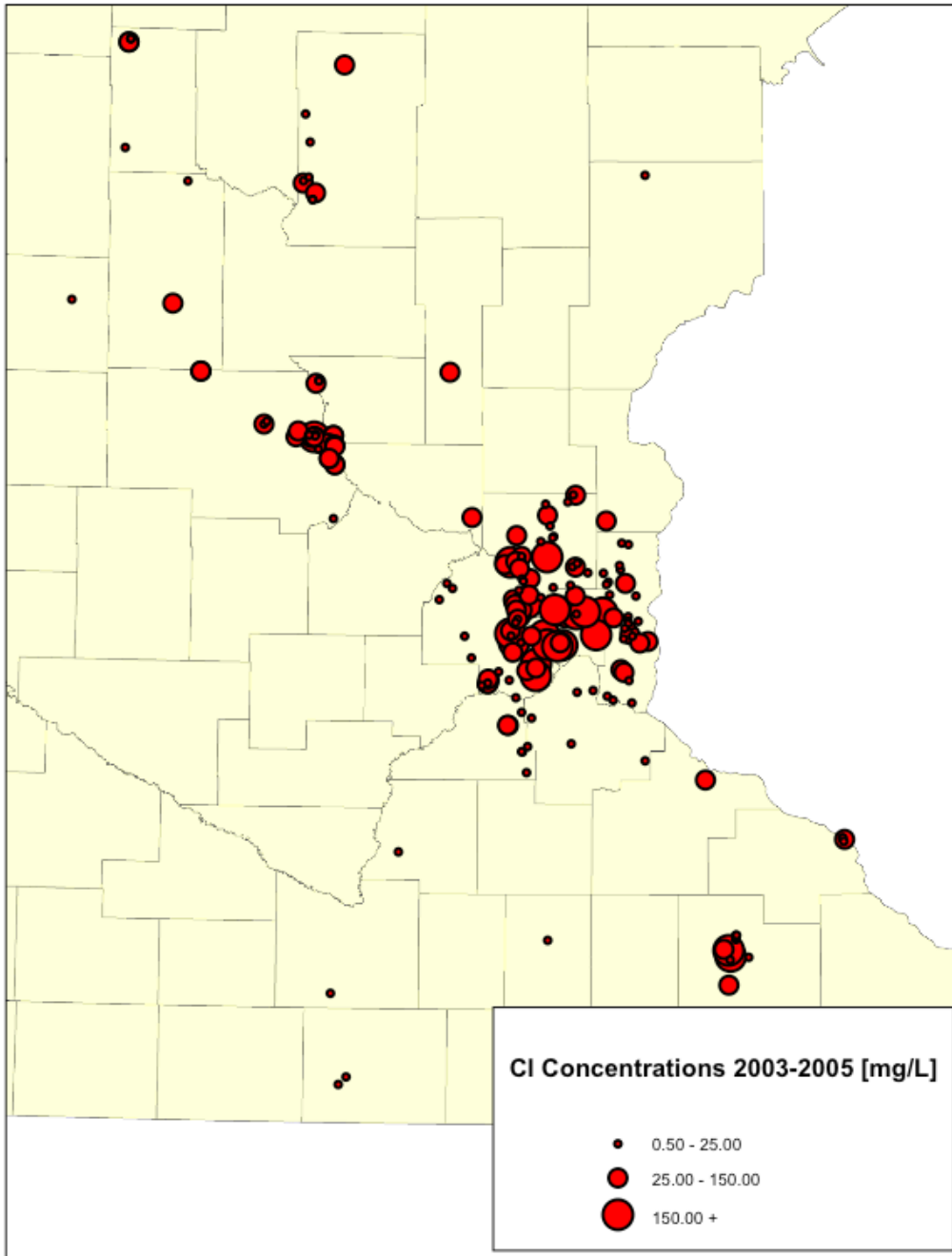
Figure 5.3 Chloride concentrations in wells of southeastern Minnesota, especially near St. Cloud, Minneapolis/St. Paul, and Rochester. The largest circles represent over 150 mg/L of chloride, the smallest less than 25 mg/L of chloride (2003-2005 data from MPCA).
