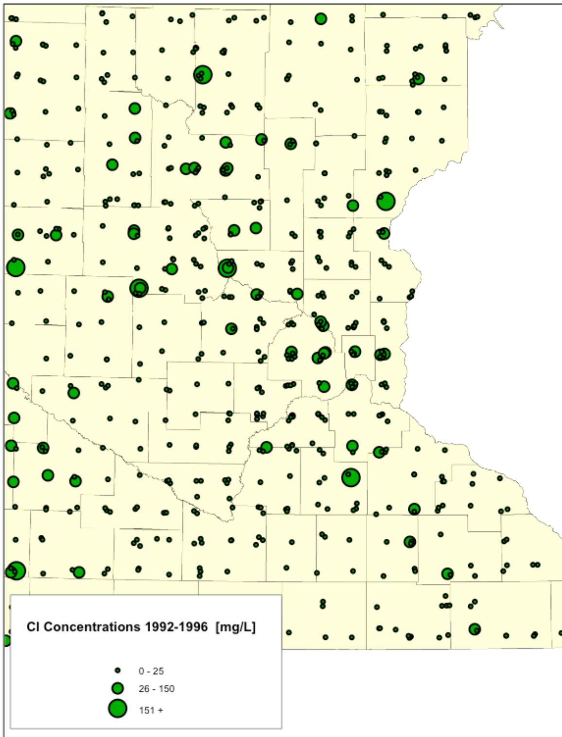
Figure 5.2 Chloride concentrations in wells of southeastern Minnesota. The largest circles represent over 150 mg/L of chloride, the smallest less than 25 mg/L of chloride (1992-1996 data from MPCA).
