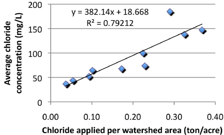
Figure 3.11 Mean annual chloride concentrations in small streams of the TCMA vs. seasonal road salt (NaCl) applications.
