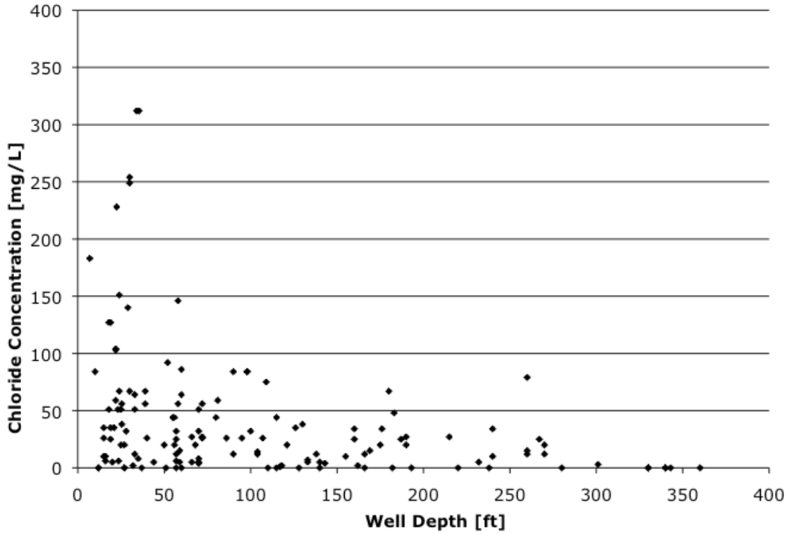
Figure 5.6 Chloride concentrations in groundwater of the TCMA.
