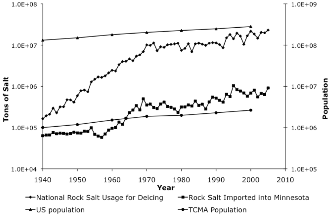
Figure 2.10 Road salt use in the U.S. and rock salt imported into Minnesota since 1940. For comparison population growth is also shown.
