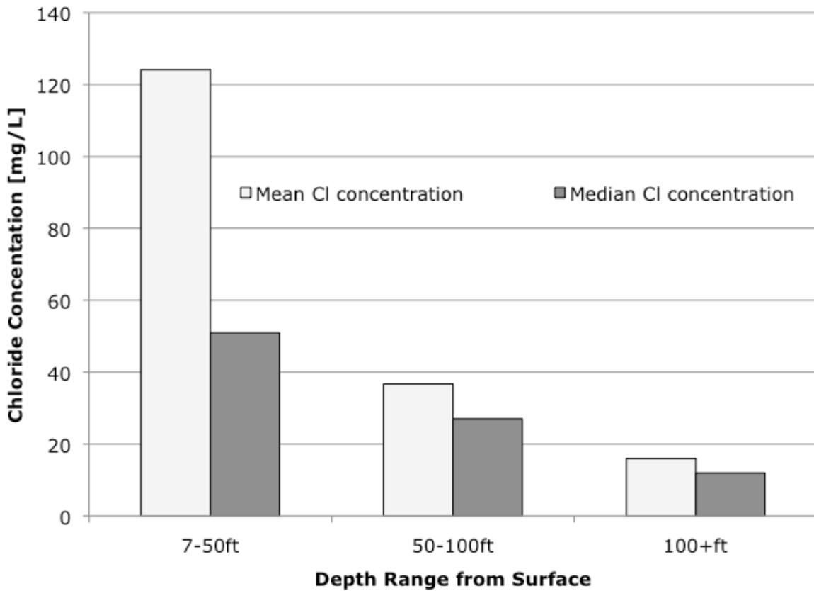
Figure 5.7 Chloride concentration vs. depth of groundwater in the TCMA (MPCA 2004-2005 DATA).
