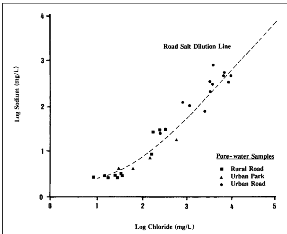
Figure 5.9 Sodium vs. chloride relationship attributed to NaCl use for winter road maintenance (Howard and Beck 1992).
