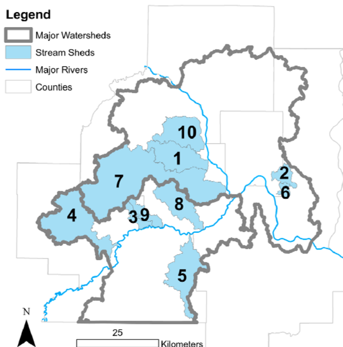
Figure 3.10 Location of small stream watersheds in the TCMA. Position numbers are referenced in Table 3.3.
