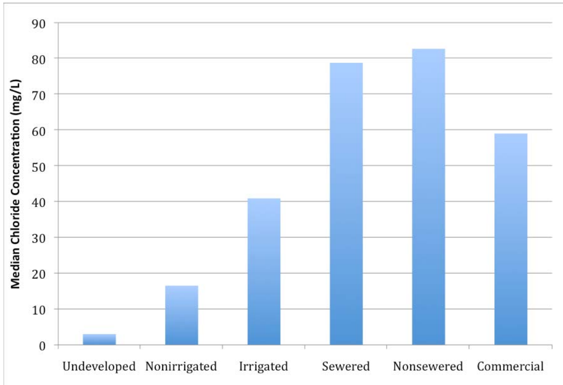
Figure 5.5 Chloride concentrations in groundwater below different land covers/uses (Trojan et. al. MPCA 2003).
