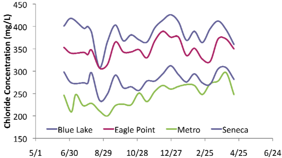
Figure 3.7 Chloride concentrations in WWTP effluents (June 2007-May 2008).
