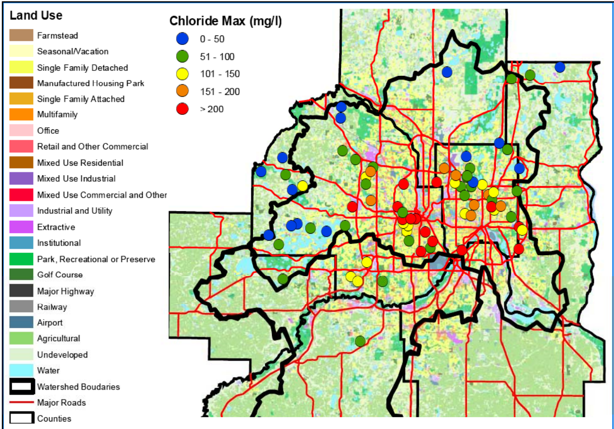
Figure 4.13 Maximum chloride concentrations in 71 lakes of the TCMA.
