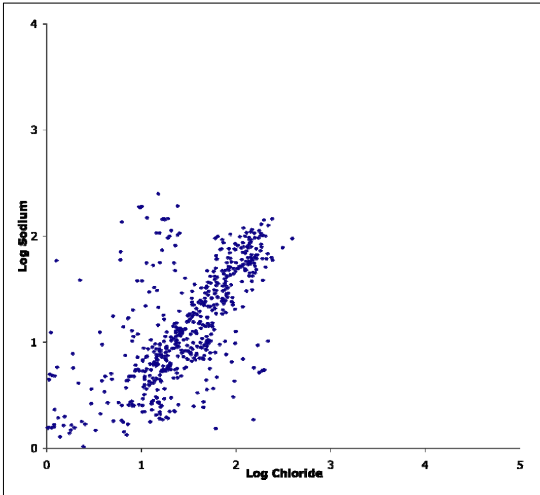
Figure 5.10 Chloride vs. sodium concentrations in groundwater of the TCMA.
