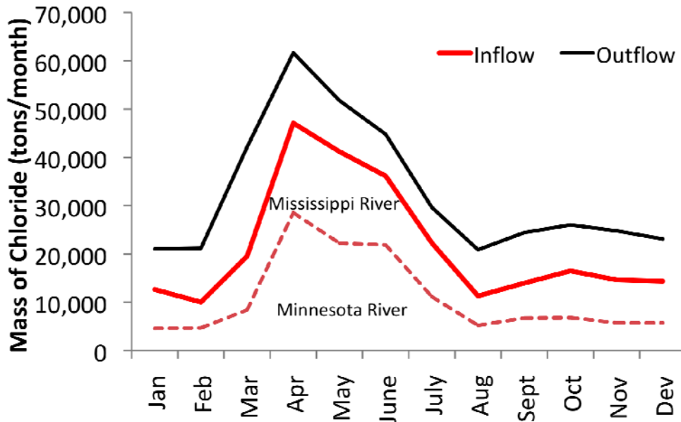
Figure 3.5 Mean monthly (2000-2007) chloride transport (tons/month) by the Minnesota and the Mississippi River into and out of the Metro watershed.
