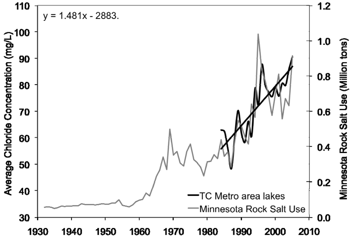
Figure 4.12 Comparison of lake chloride concentrations in 39 TCMA lakes and rock salt purchases by the state of Minnesota (Novotny et al. 2007).
