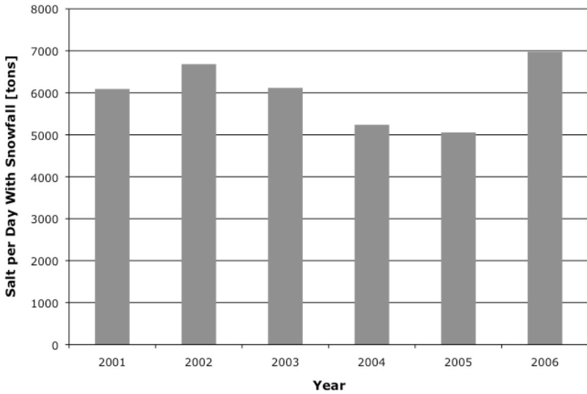
Figure 2.4 Salt use per day with snowfall.
