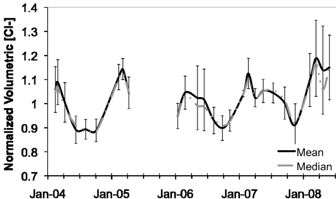
Figure 4.7 Seasonal salinity (Cl-) cycles illustrated by normalized (volume-weighted) average chloride concentrations. Averages are for all lakes in each time period. Bars represent the standard deviation for the set of lakes. Reference for normalization is the (volume-weighted) average concentration for each lake during the sampling period.
