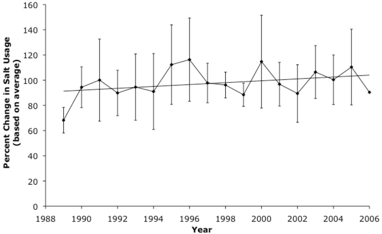
Figure 2.9 Annual road salt use as a percentage of the long-term (1989-2006) average.
