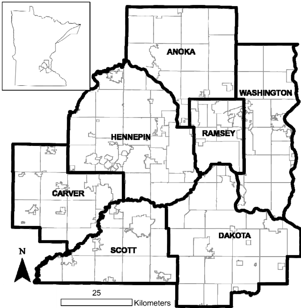
Figure 1.2 Twin Cities Metropolitan Area (TCMA), Minnesota.
