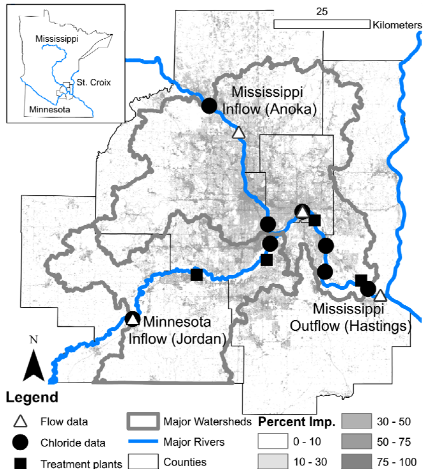
Figure 3.1 Boundaries of TCMA watershed (control volume) used for the salt (chloride) mass balance.
