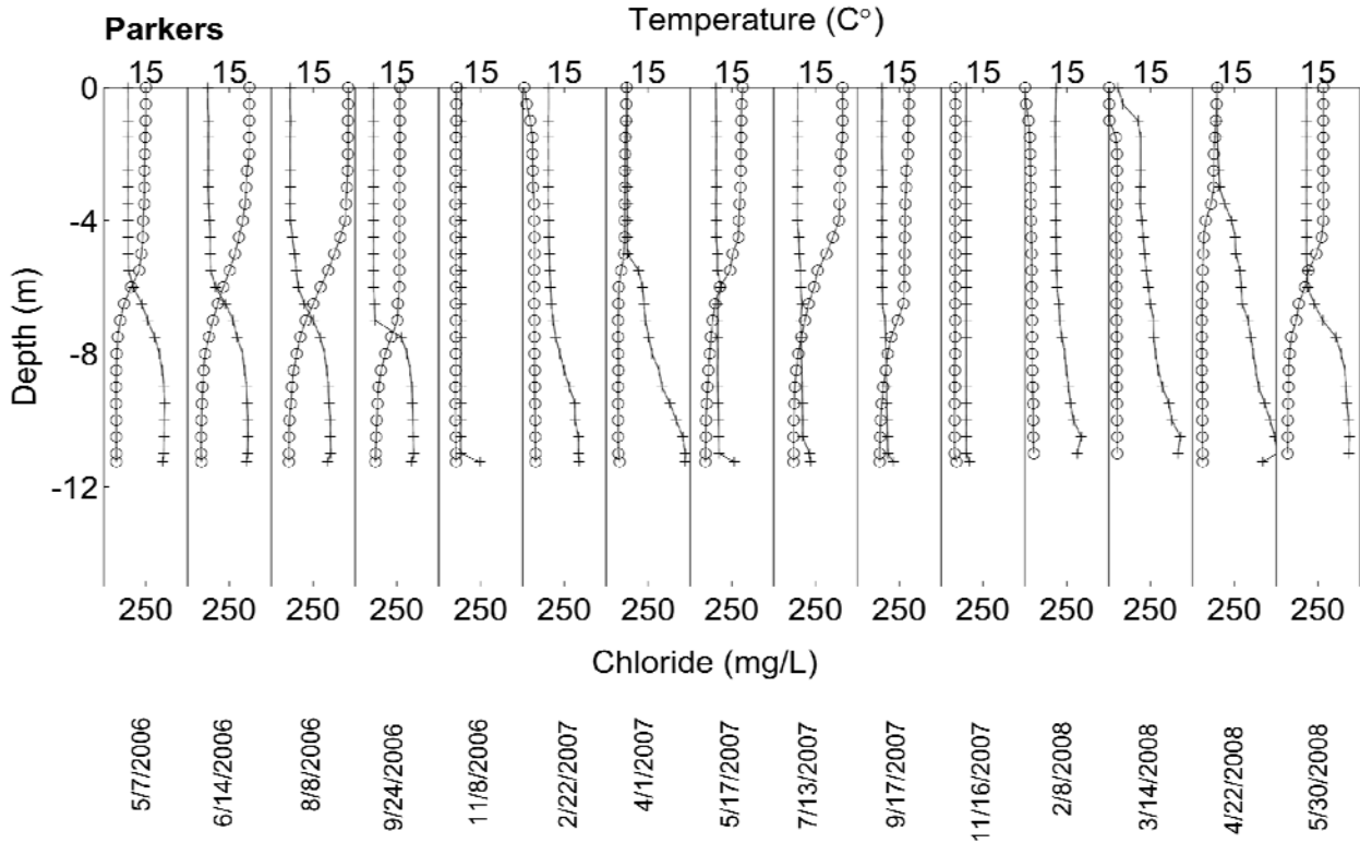
Figure 4.10 Chloride and temperature profiles in Parkers Lake.
