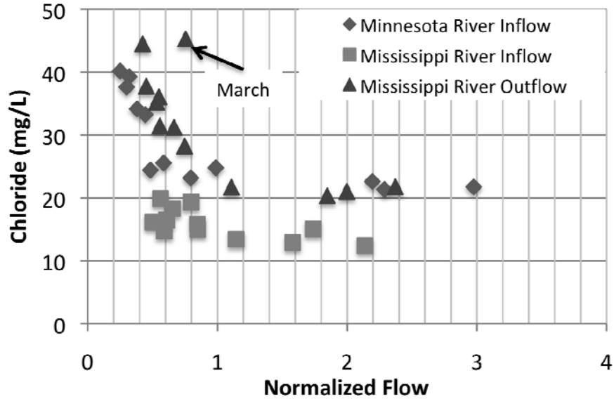
Figure 3.4 Monthly flow-weighted average chloride concentration vs. normalized monthly average flow at each of the sampling stations on the Minnesota and Mississippi Rivers.
