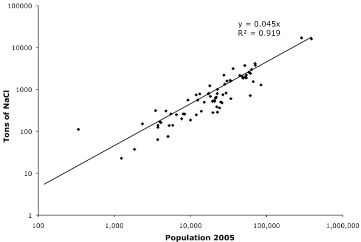
Figure 2.6 Road salt use (tons per season) in cities of the TCMA. The slope of the line is the per capita salt use by cities (not the total).
