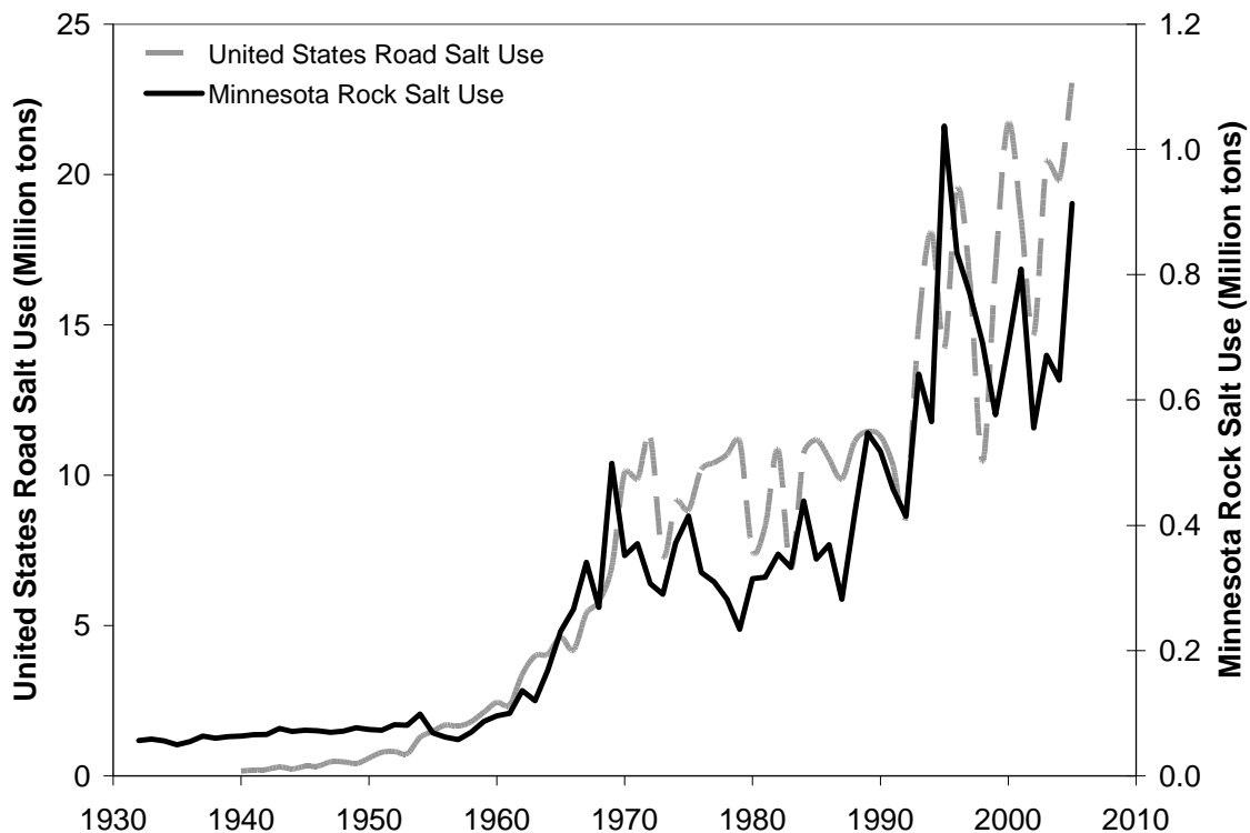
Figure 1.1 Annual road salt purchases for de-icing application in the United States and rock salt purchases for road de-icing by the state of Minnesota.
