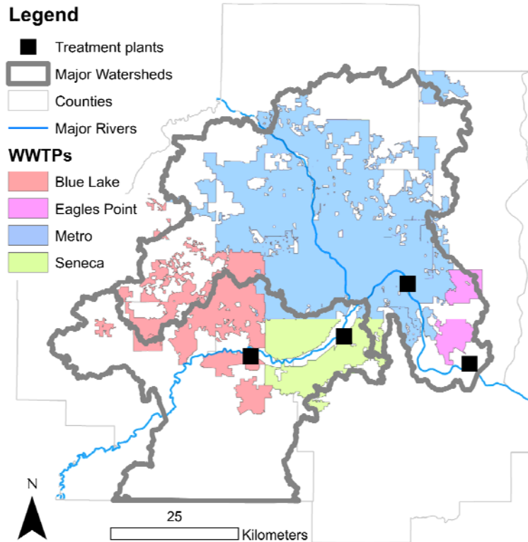
Figure 3.6 Coverage of the four WWTPs discharging into the watershed. Data layers obtained from Metropolitan Council GIS database.
