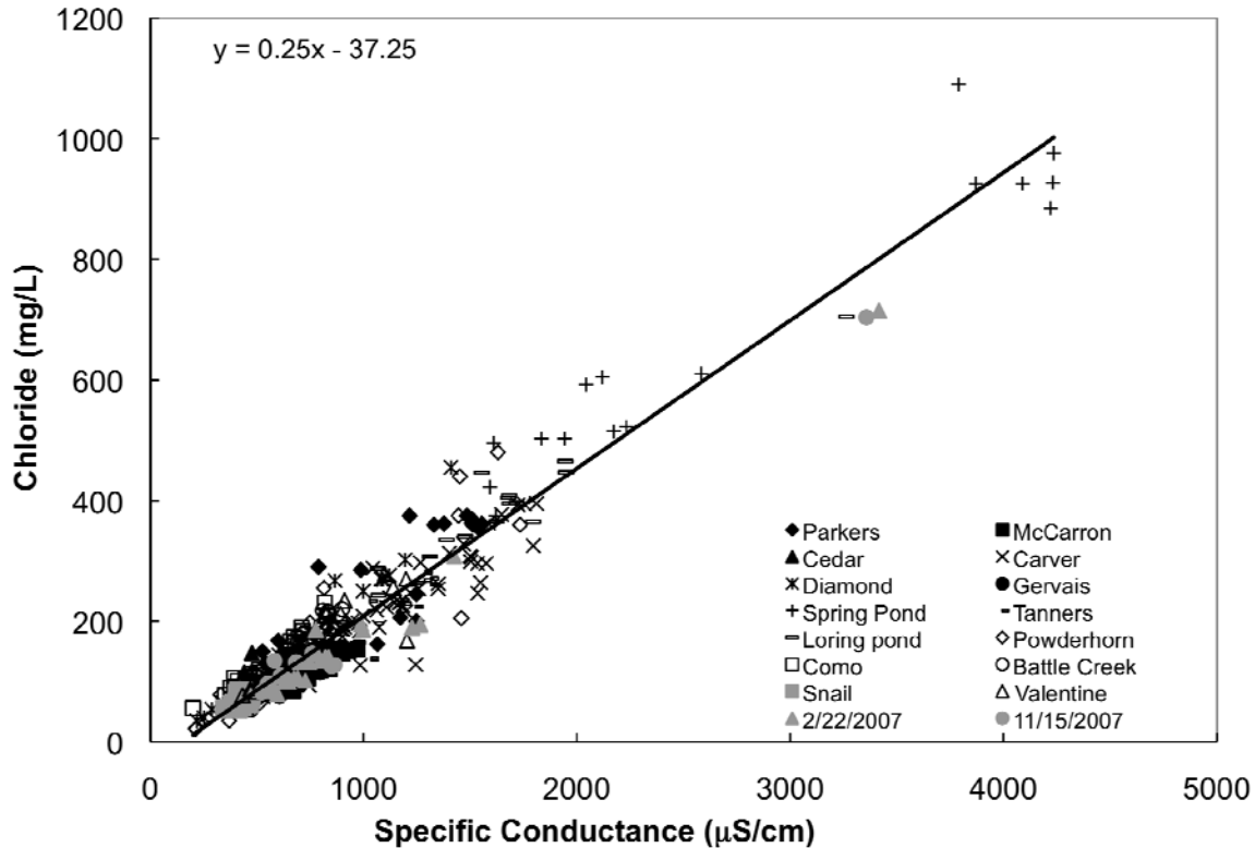
Figure 4.4 Relationship between specific conductance and chloride concentration in TCMA lakes. Data from 14 lakes in the MPCA Environmental Data Access (listed by names), and water samples from 9 TCMA lakes (2/22/2007) were used.
