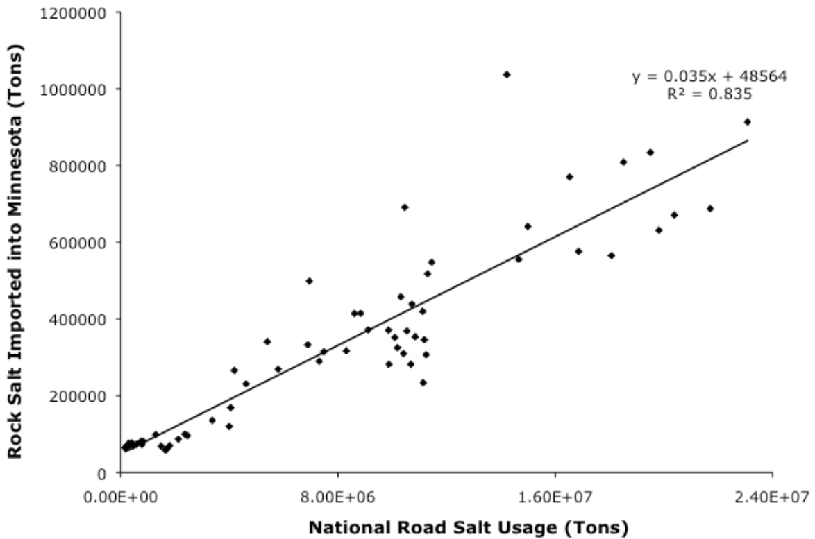
Figure 2.11 Correlation between national road salt use and rock salt imported into Minnesota.
