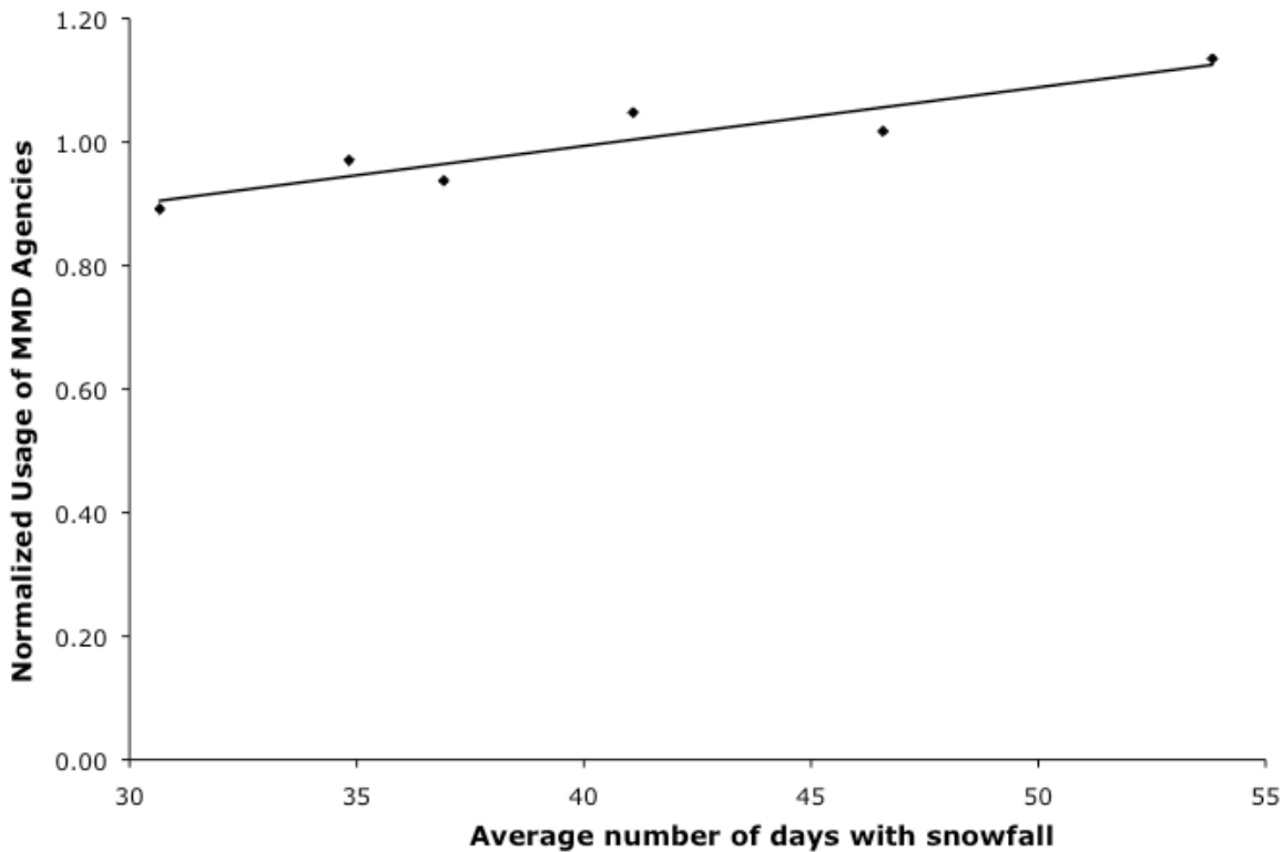
Figure 2.3 Annual road salt use in the TCMA by MMD contract participants vs. annual average number of days with snowfall.
