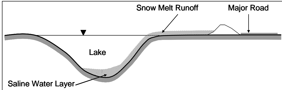
Figure 4.2 Schematic of a saline water intrusion into a lake.
