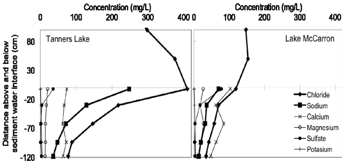
Figure 4.11 Ionic composition of pore water from sediment cores extracted at the deepest locations of Lake McCarron and of Tanners Lake.
