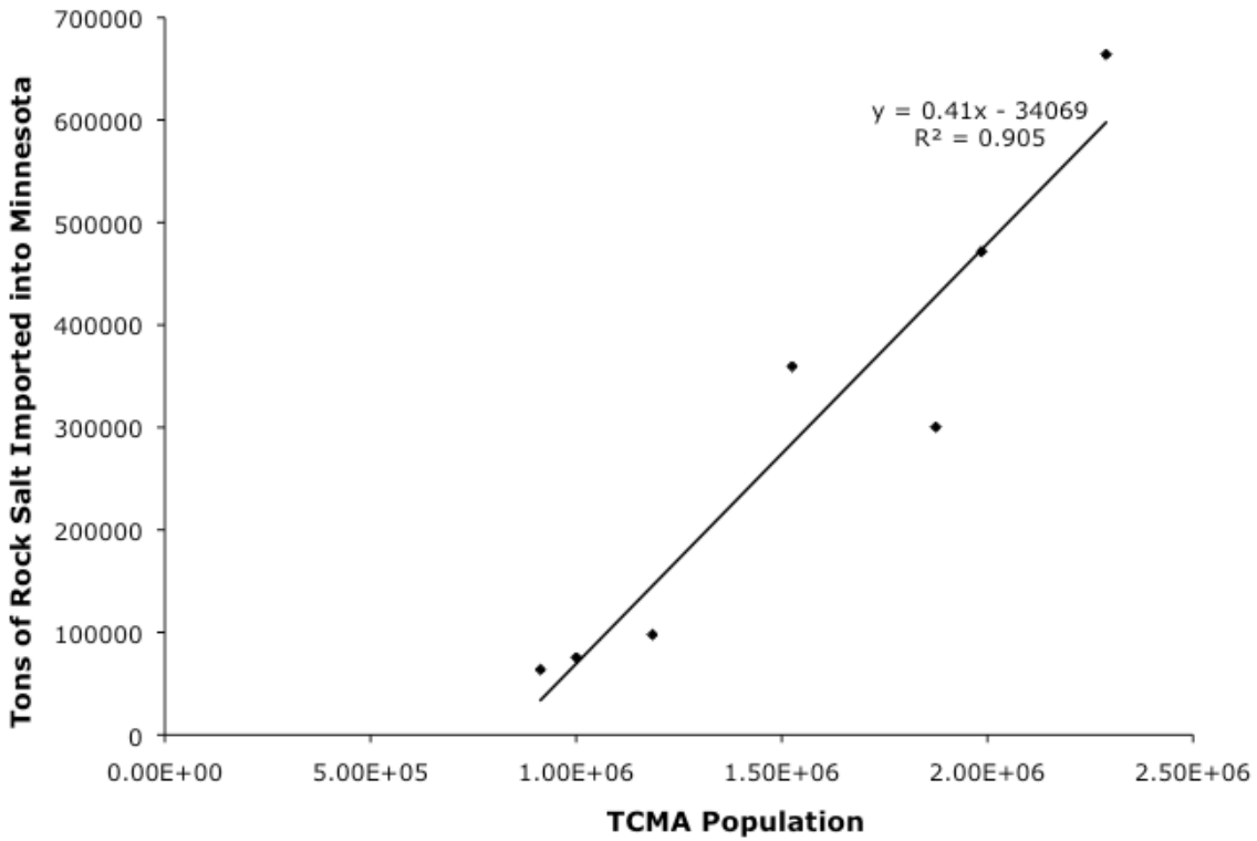
Figure 2.5 Rock salt imported into Minnesota and TCMA population 1930-1993.
