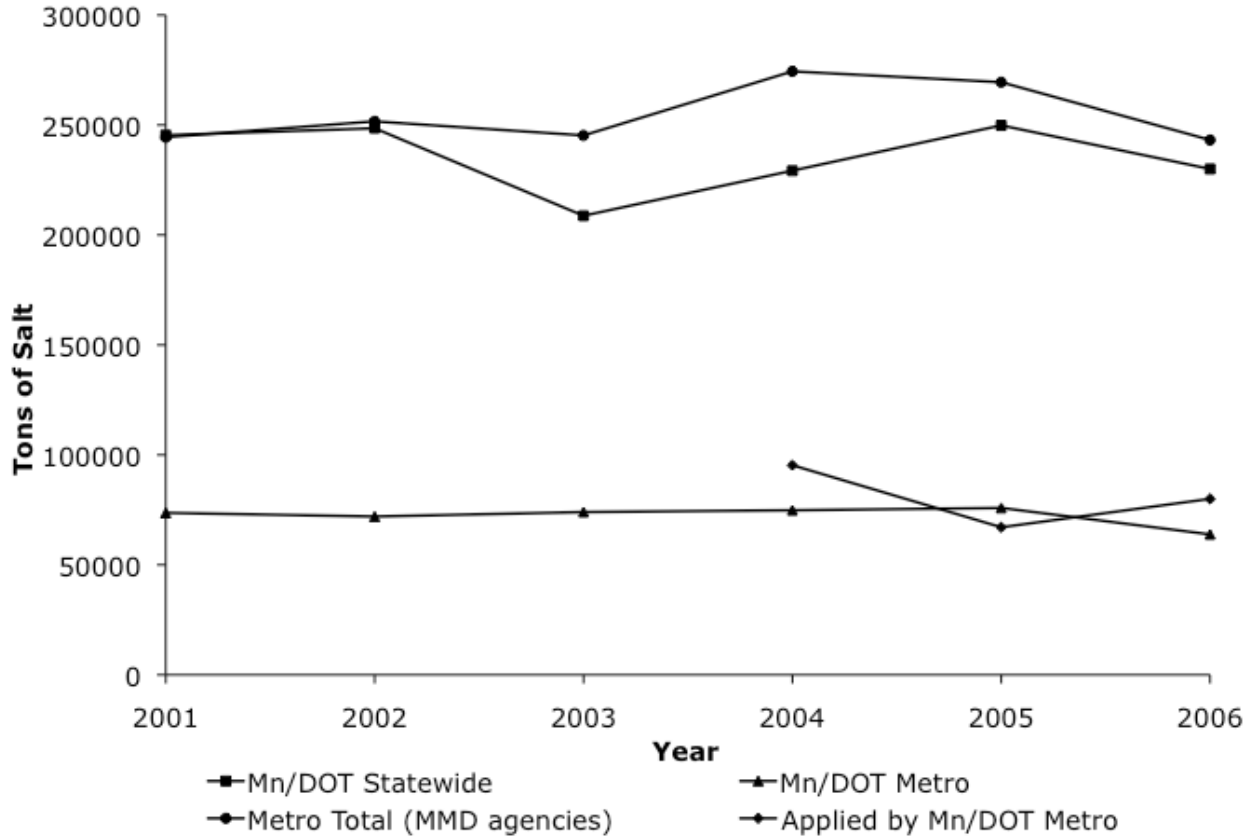
Figure 2.8 MMD salt contract amounts for the TCMA.
