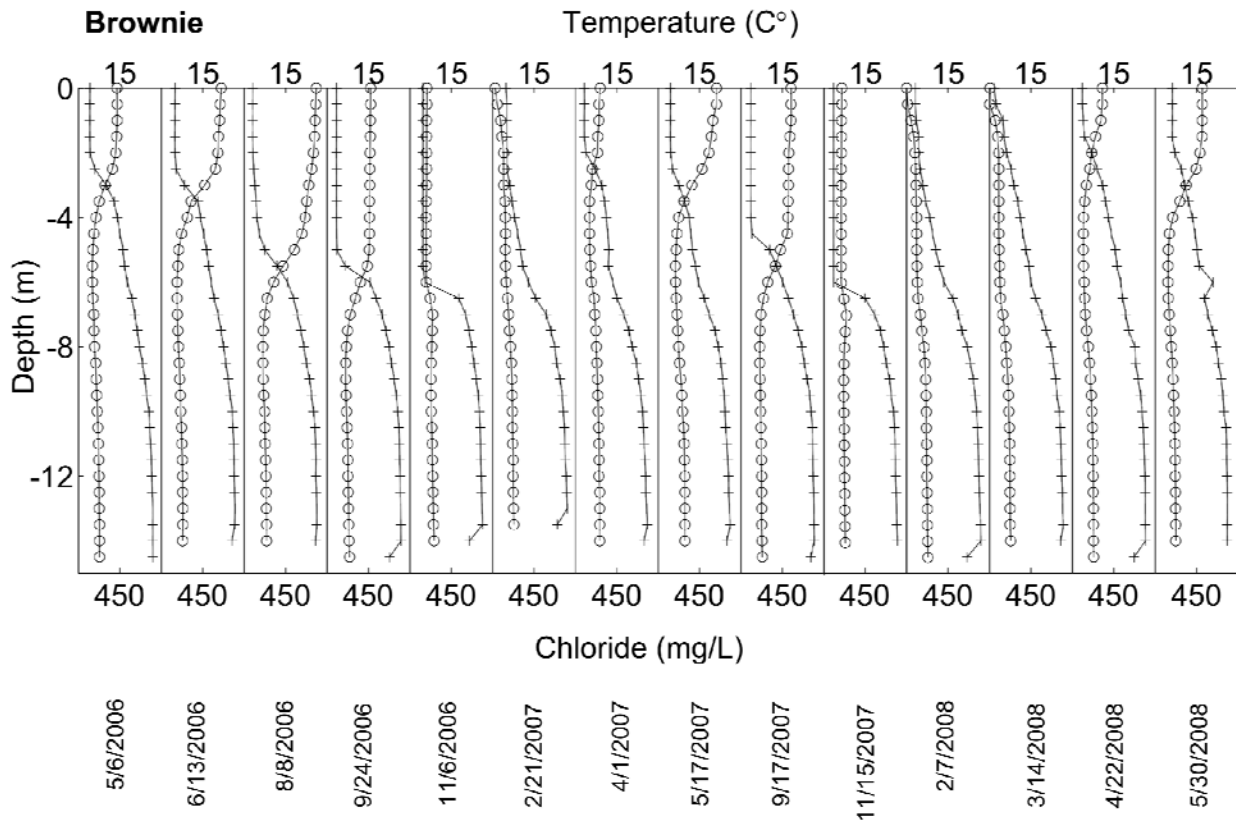
Figure 4.8 Chloride and temperature profiles for Brownie Lake.
