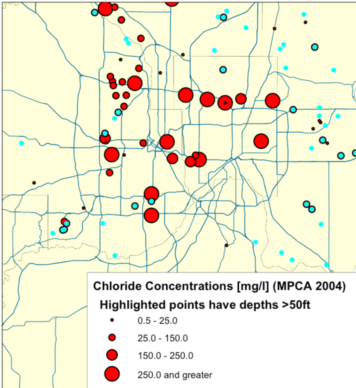
Figure 5.4 Chloride concentrations in TCMA wells. Dark (red) circles represent shallow wells ( depth < 50ft ). Light (blue) circles represent deep wells ( depth > 50ft ) (2003-2005 data from MPCA).
