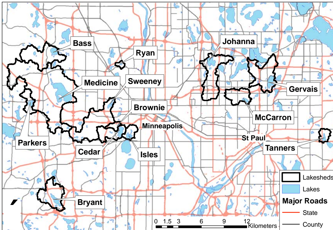
Figure 4.3 Locations of the study lakes and their watersheds in the Minneapolis-St. Paul Metropolitan Area (TCMA).
