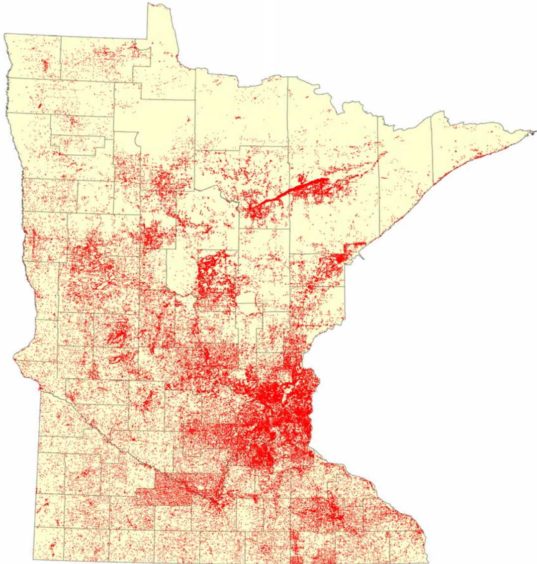
Figure 5.1 Wells in Minnesota.
