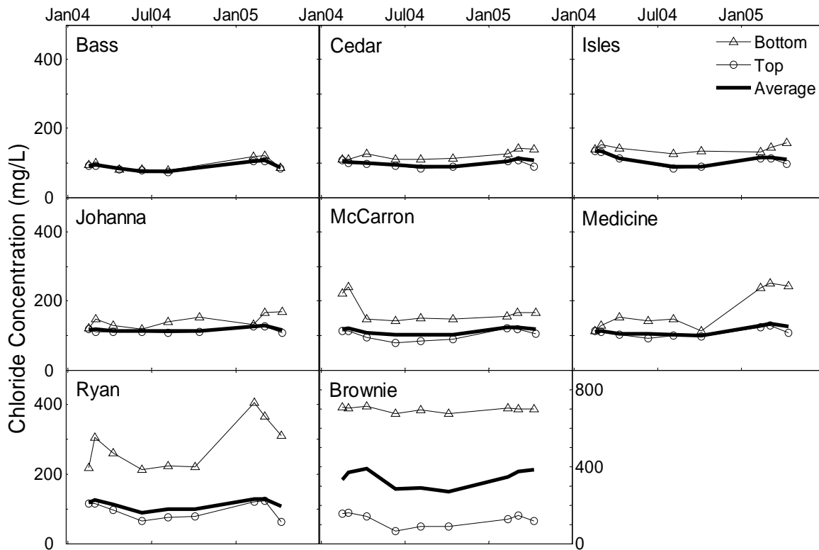
Figure 4.5 Chloride concentrations 0.5 m below the surface and 0.5 m above the bottom of 8 TCMA lakes, and average chloride concentrations in each lake sampled from Feb 2004 to April 2005.
