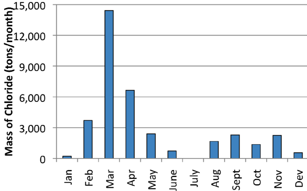
Figure 3.9 Net monthly chloride export from the TCMA watershed (Net export = difference between export and import in Figure 3.8).
