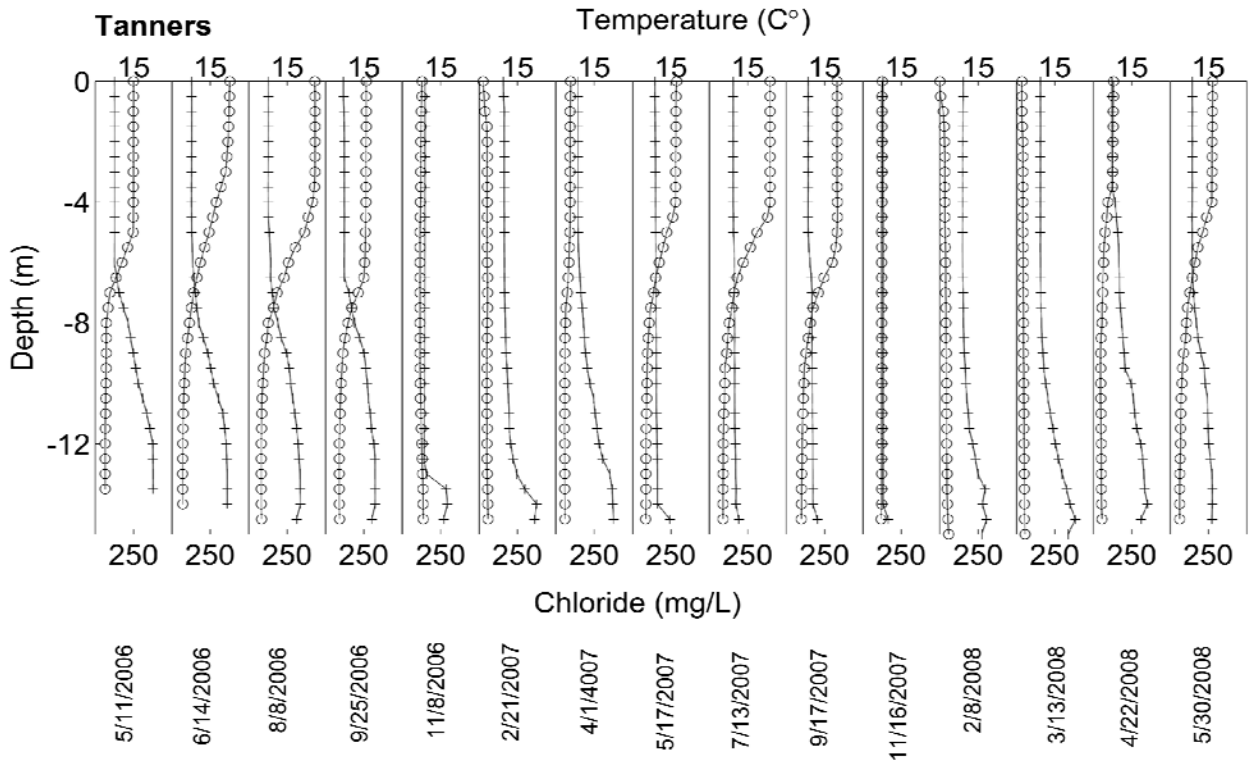
Figure 4.9 Chloride and temperature profiles in Tanners Lake.
