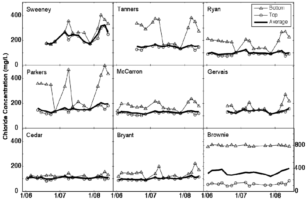
Figure 4.6 Chloride concentrations 0.5 m below the surface and 0.5 m above the bottom of 9 TCMA lakes, and average chloride concentrations in each lake sampled from Jan 2006 to May 2008.
