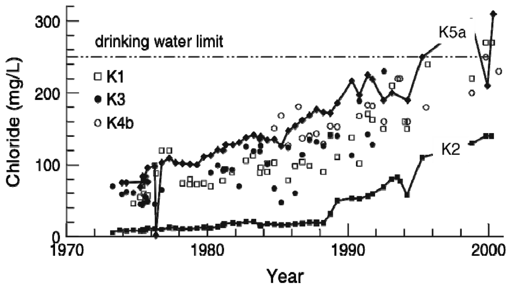
Figure 5.8 Canadian measurements of chloride concentrations in five groundwater wells (K1, K2, K3, K4b and K5a) in the Toronto area (Bester et al. 2006).
