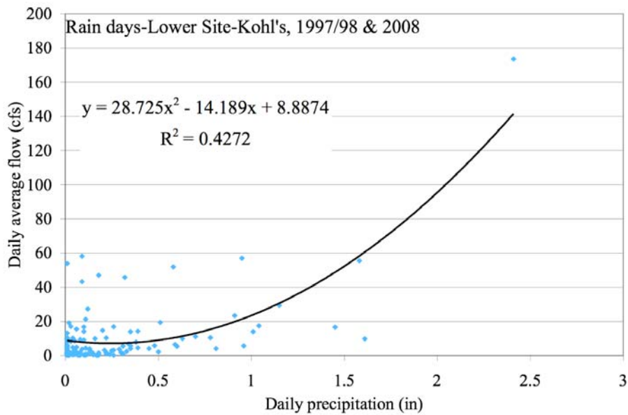
Figure 4.4 Average daily stream flow in Miller Creek on rainy days at the lower (26 th Ave) stream flow gage vs. daily precipitation from Duluth Airport (upper panel), and from Kohl's site (lower panel).
