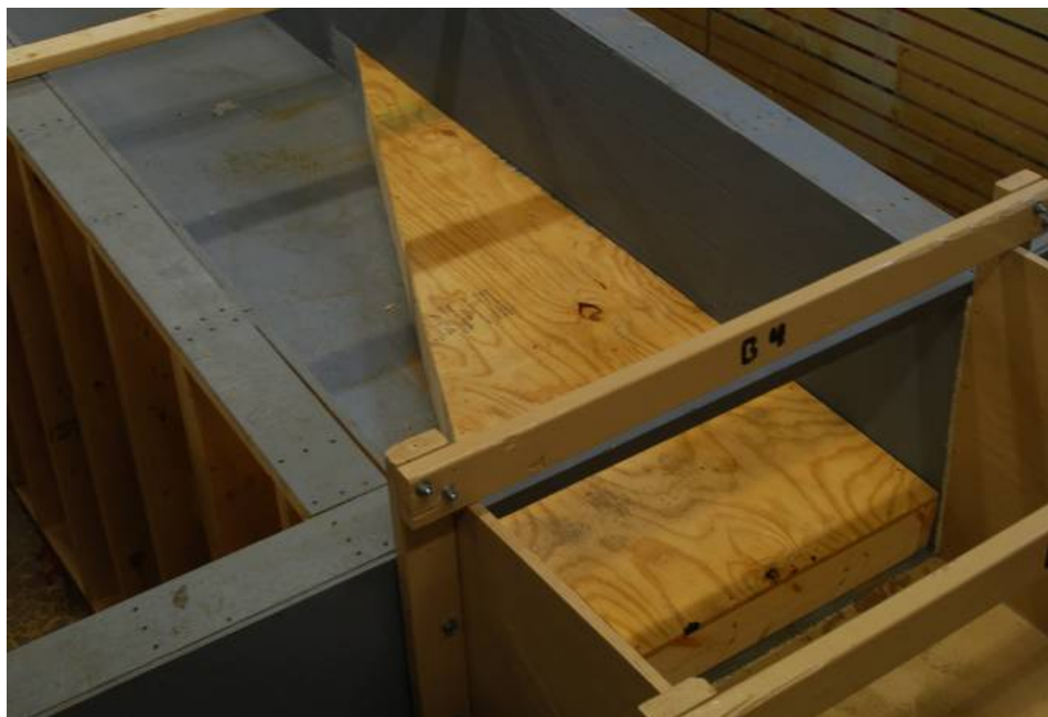
Figure 4. Wedge in approach slope.
