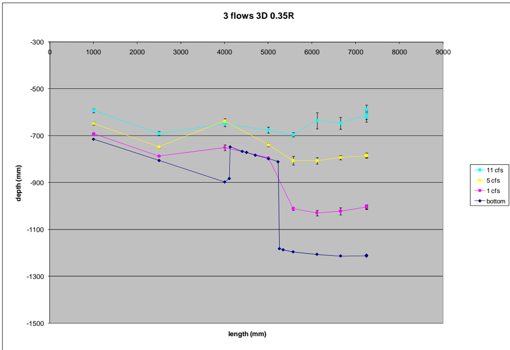
Figure 16. Water surface profiles for the 3d approach section length and 0.35d recessed depth trials.
