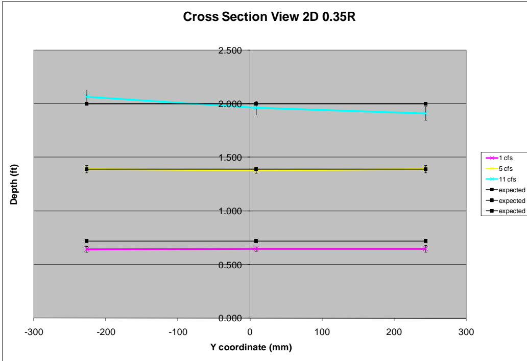
Figure 15. Cross sectional view of water surface measured within the H Flume for the 2d approach section length and 0.35d recessed depth. The point at -250 mm is the location specified by the manufacturer for discharge measurement. The black line is the water surface elevation equivalent to the actual discharge passing through the system as specified by the manufacturer. Error bars indicate one standard deviation about the mean value.
