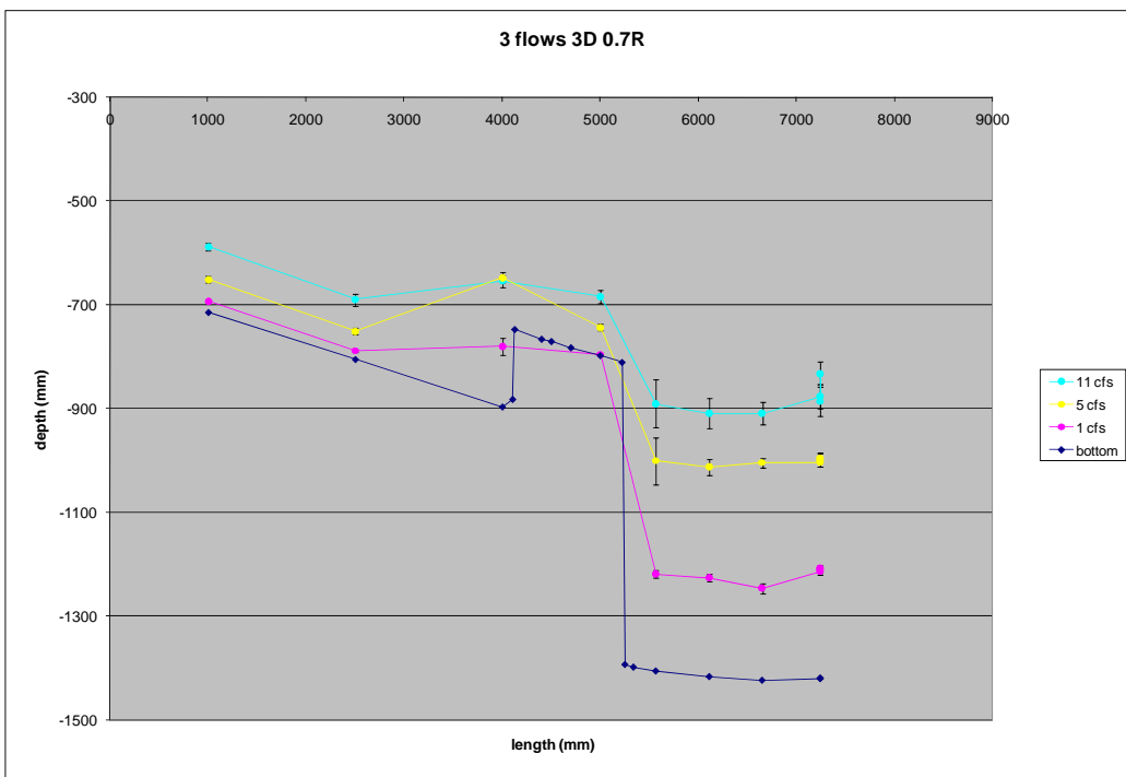
Figure 22. Water surface profiles for the 3d approach section length and 0.7d recessed depth trials.
