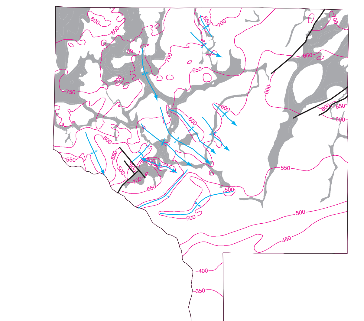
Figure 3. Map of Anoka County contoured at the stratigraphic top of the Wenocese Sandstone showing geologic structure, scale: 1:300,000. Contour interval is 50 feet (15 meters). The approximate areas where some of all of the Wenocese Sandstone is missing because of erosion, and where the Wenocese Sandstone, Eau Claire Formation, or Mt. Simon Sandstone are first bedrock is shaded; contours in those areas are inferred from projection using the estimated full thickness of the formations. The inferred traces of faults and folds are shown.
