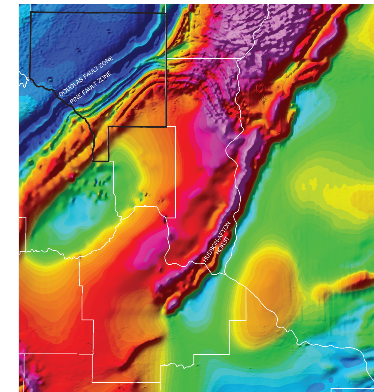
Figure 2. Acromagnetic map for the metropolitan area showing anomalies related to geologic structures shown on the bedrock map and on Figure 3. Shown in color shaded relief format with false illumination from the northwest at 45° inclination (Chandler, 2007).
