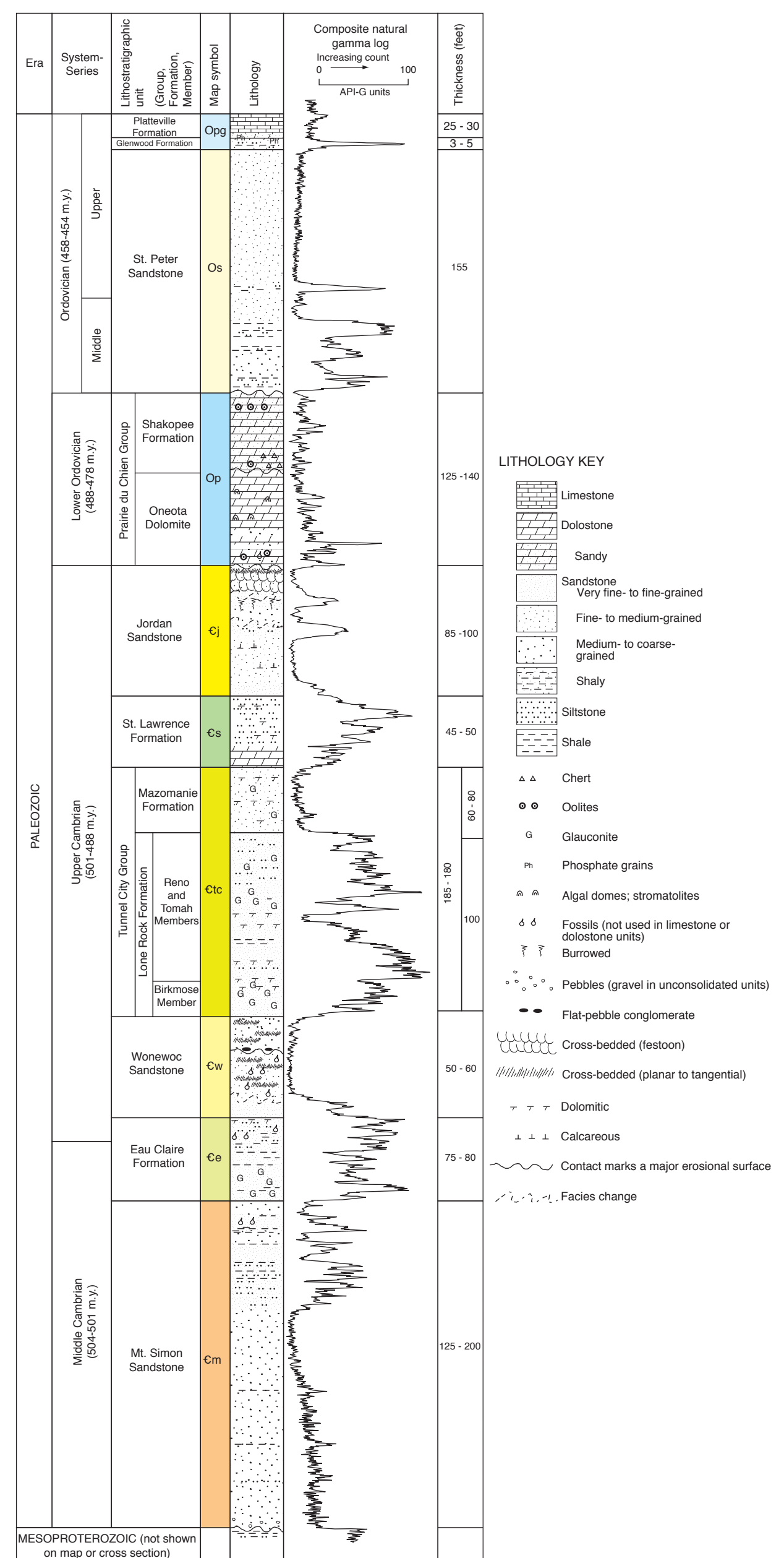
Figure 1. Stratigraphic column depicting the lithology, thickness, and vertical succession of rock units shown on the map. Includes the approximate age in millions of years for the rocks in Minnesota. The gamma log is a compilation of the following gamma logs from Anoka and Hennepin Counties: 44789, 20292, 20665, 578957, and 225599. A higher gamma count typically reflects increased shale or clay content.
