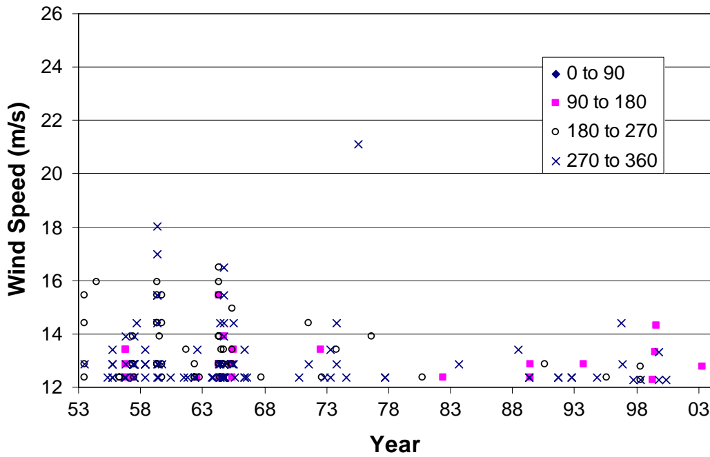
Figure 6.7. Highest hourly wind velocities versus time and direction for Winnipeg, May – October, 1953 – 2003.
