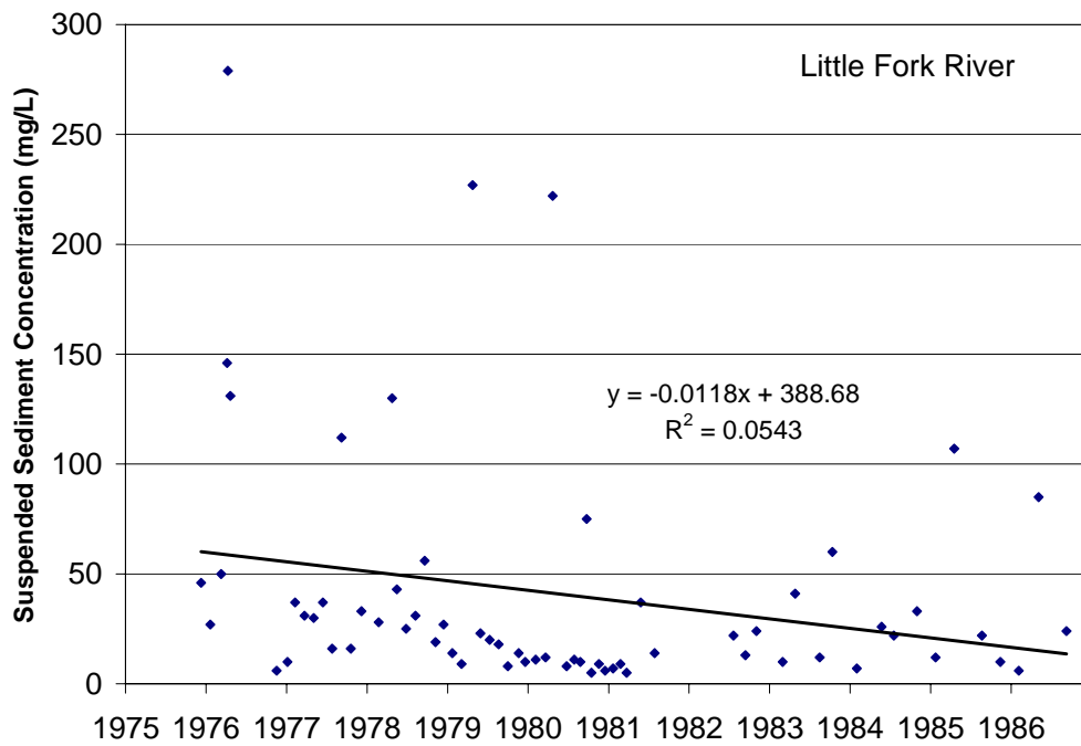
Figure 9.5. Suspended sediment concentration vs. time for the Rainy River at Baudette (upper panel) and Little Fork River at Little Fork, MN.
