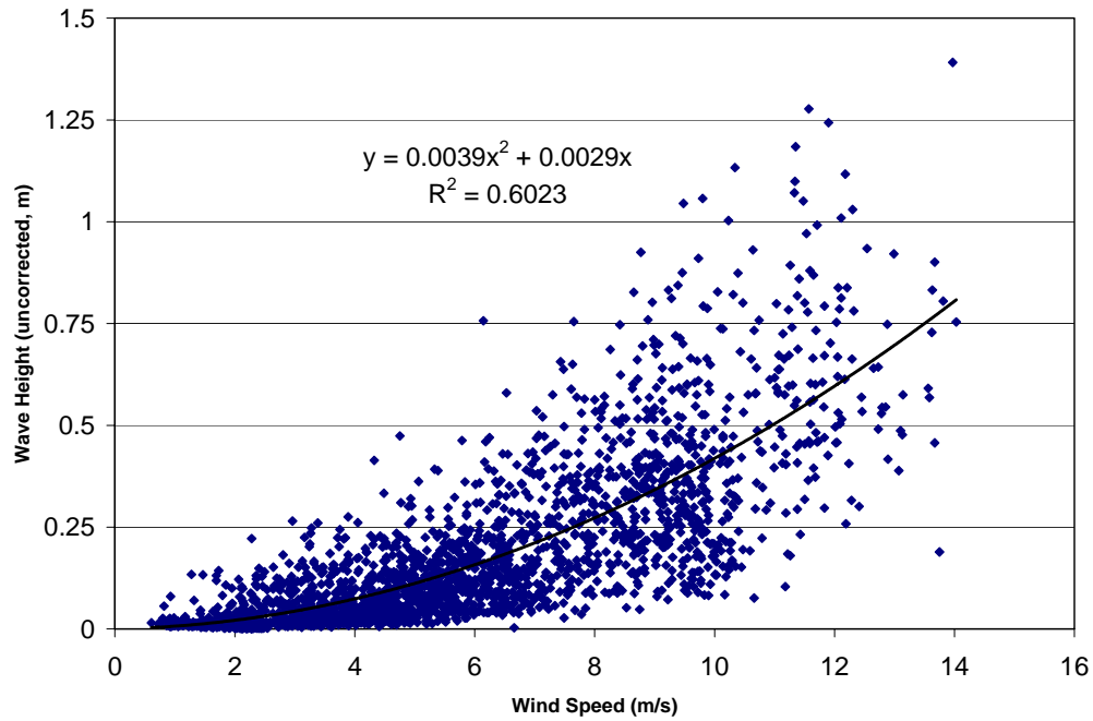
Figure 3.5. Raw station wind speed versus wave height for the Pine Island station. Wind speed values are 10 minute averaged, while wave height values are instantaneous measurements at 10 minute intervals.
