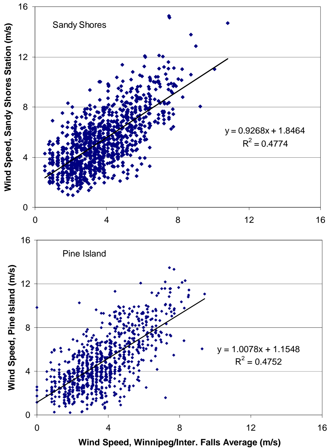
Figure 5.5. Measured wind speed versus averaged Winnipeg-International Falls wind speed for Sandy Shores (upper panel) and Pine Island (lower panel) for 1 hour averaged data, all directions.
