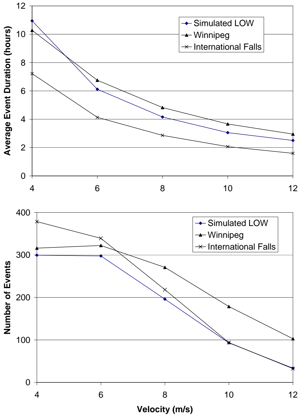
Figure 6.11. Average number of wind events per year and average event duration versus wind velocity for simulated LOW wind data, Winnipeg, and International Falls, 1956 – 2003. Event duration analysis was performed only on years with 1 hour data sets (37 years).
