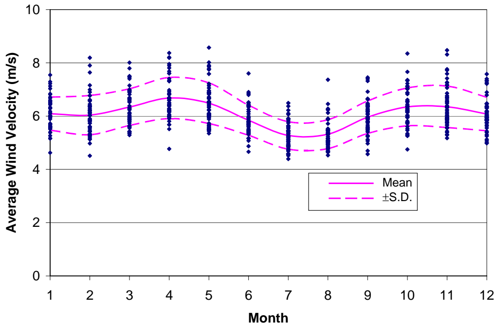
Figure 6.4. Monthly averaged wind velocity versus month for simulated LOW wind data, 1953 – 2003. Monthly mean values are plotted as a solid line with \pm 1 STD as a dashed line.
