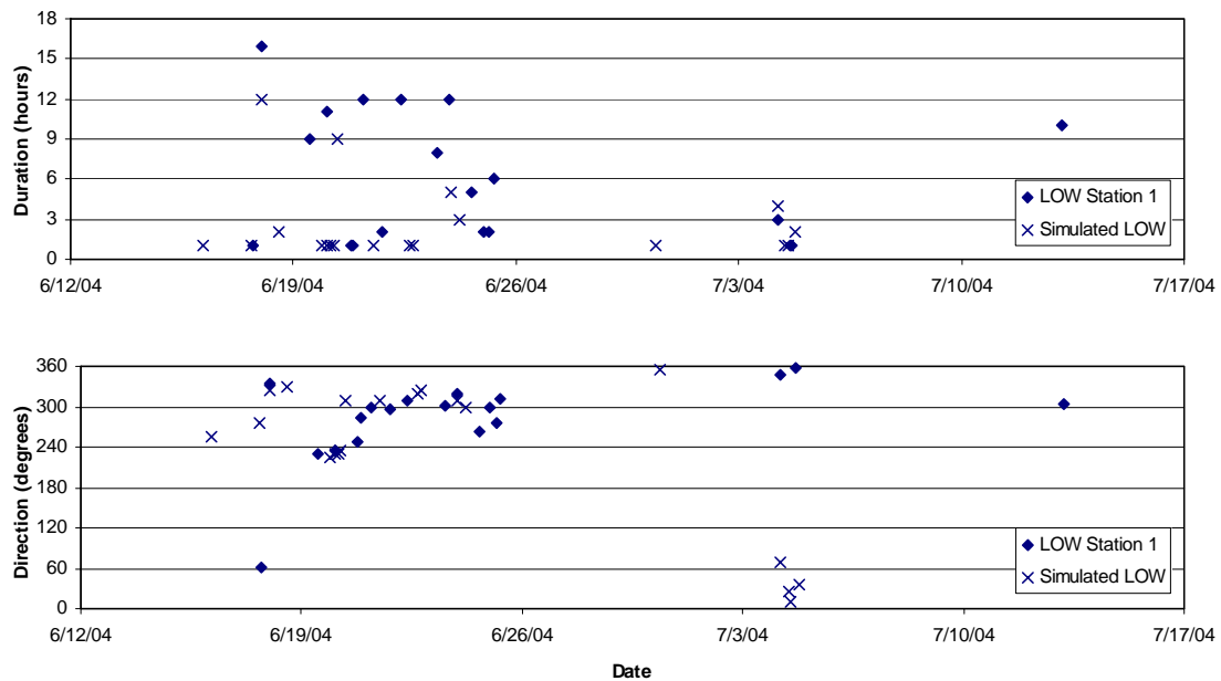
Figure 5.8. Duration and mean direction versus time for wind events exceeding 8 m/s for LOW Station 1 and simulated LOW, June 16 to July 20, 2004.
