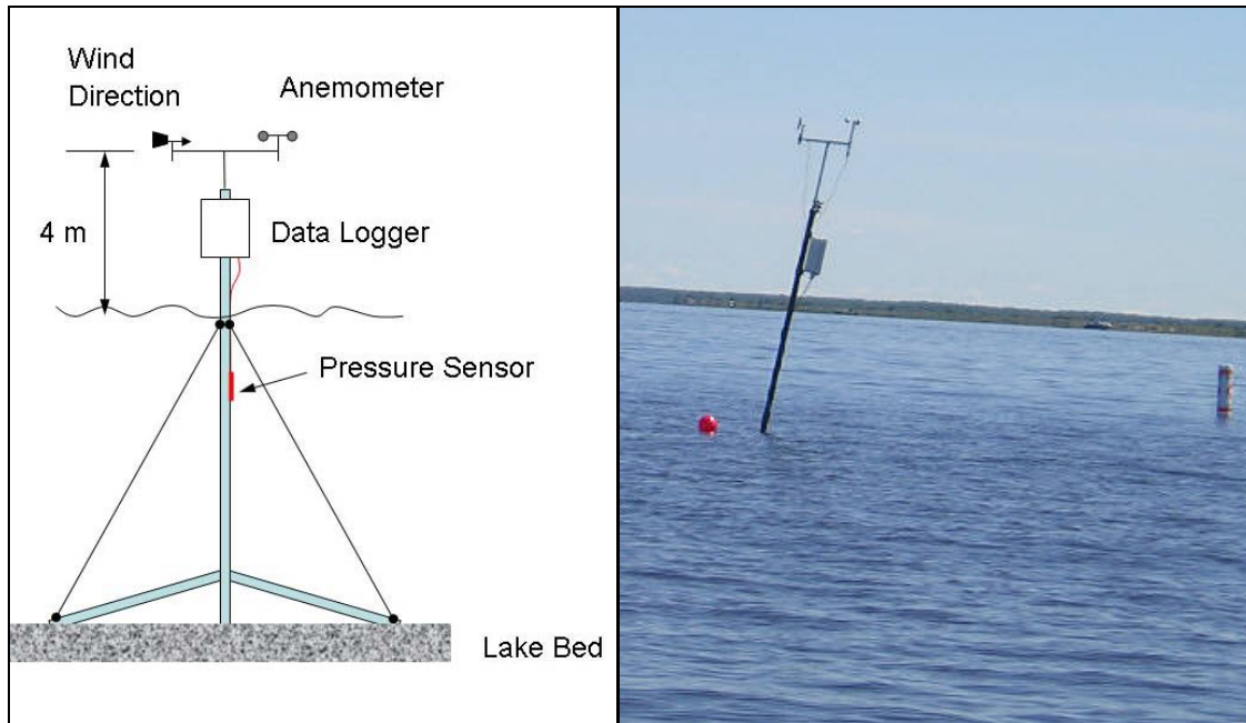
Figure 3.1. Schematic drawing and photograph of the Pine Island wind/wave measurement station.
