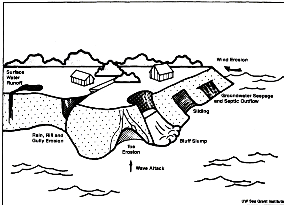
Figure 1.1. Diagram of consolidated coastline erosion processes (taken from UW Sea Grant, 1998).
