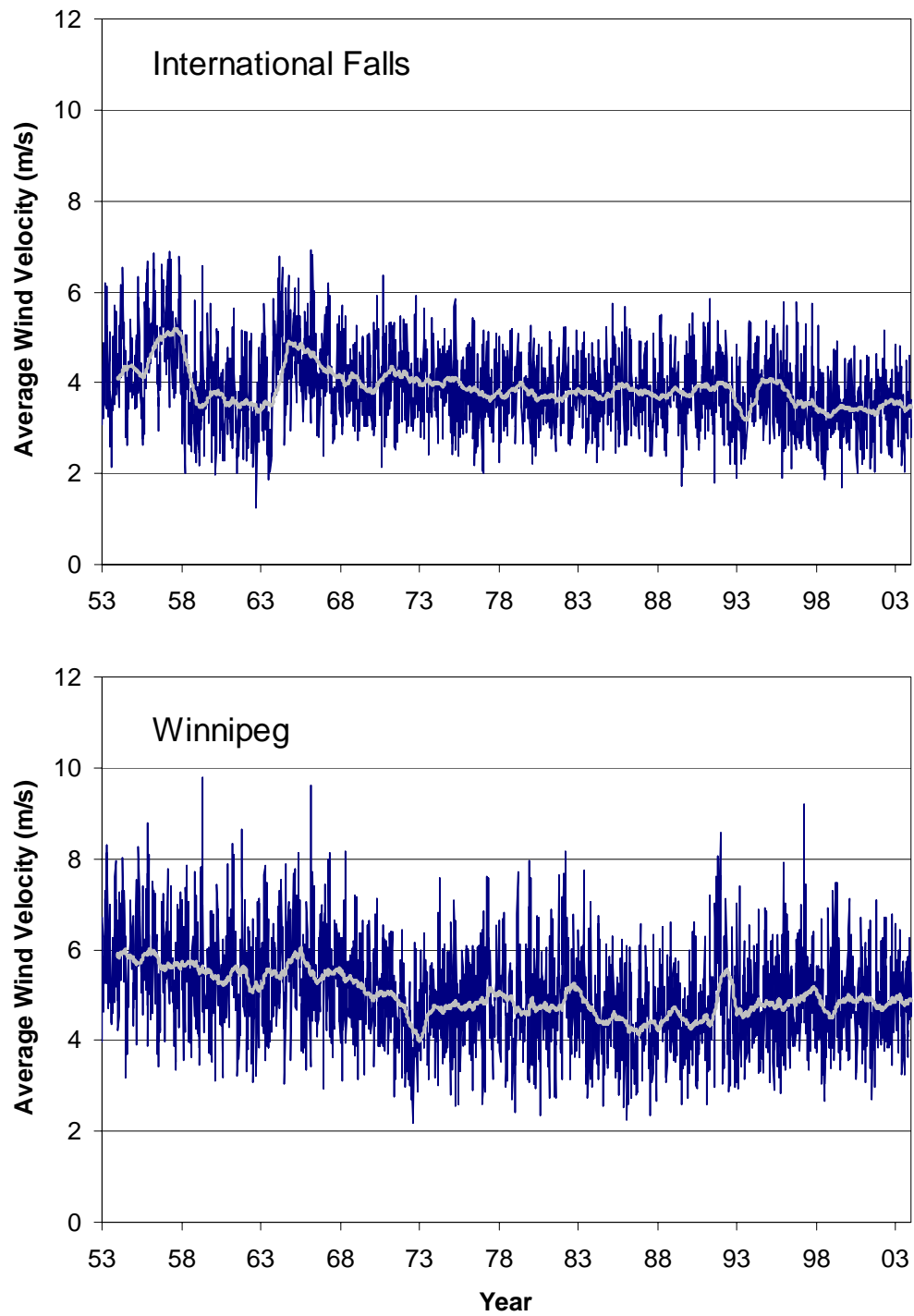
Figure 6.2. Weekly averaged wind velocity versus time for International Falls (upper panel) and Winnipeg (lower panel). The 52 week running average is shown for both locations.
