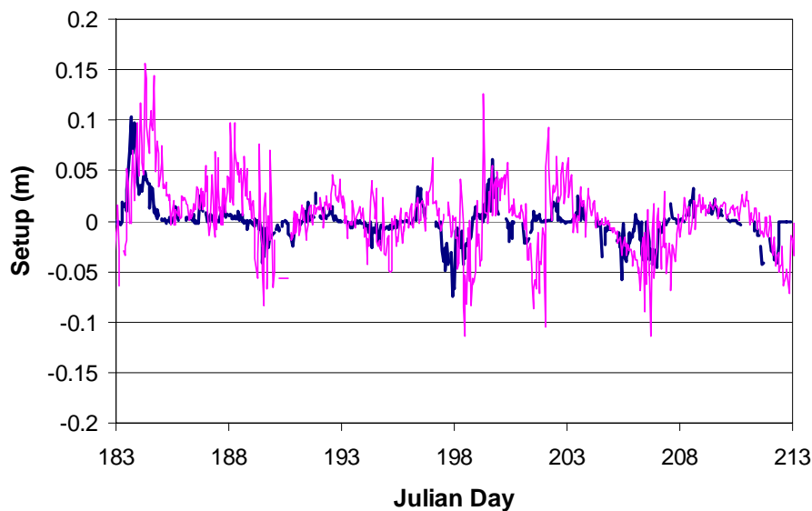
Figure 7.1. Theoretical (dark line) and measured (light line) wind setup vs. time for Warroad and Cyclone Island gages, 1 hour averaging time.
