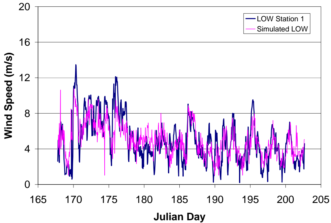
Figure 5.7. One hour averaged wind speed versus time for LOW station #1 (Pine Island) and simulated LOW.
