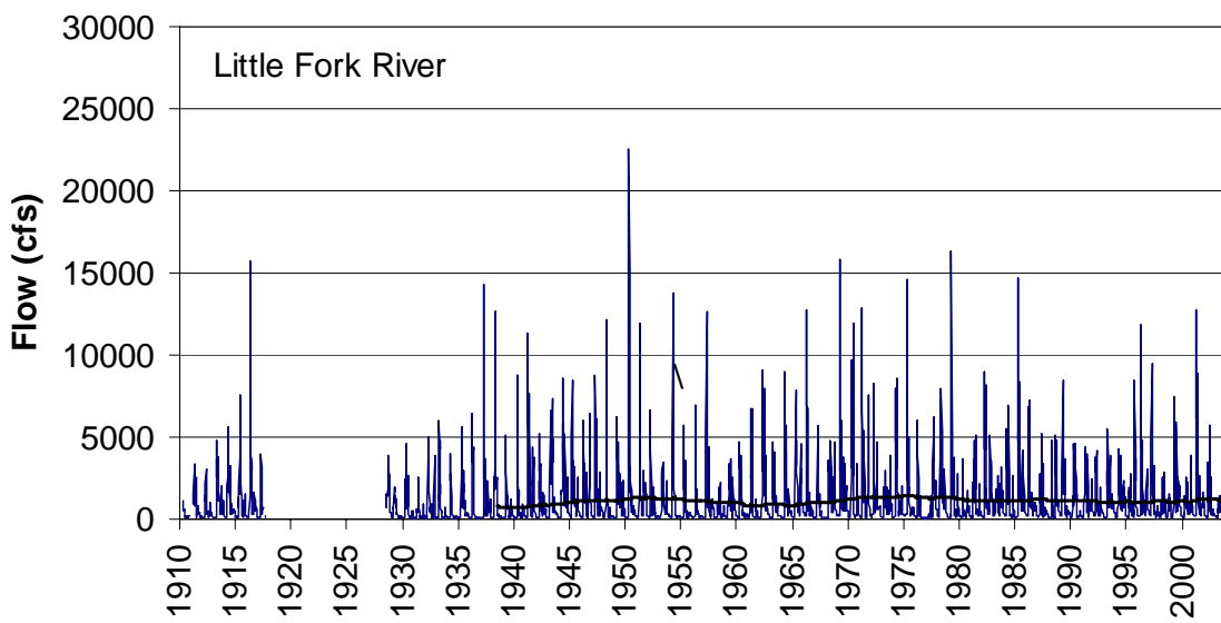
Figure 9.3. Weekly average flow rate and 10 year running average for the Rainy River at Manitou Falls and the Little Fork River at Little Fork, MN, from USGS stream gaging stations.
