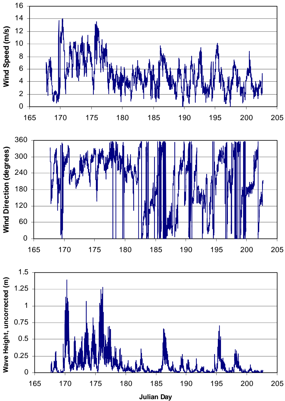
Figure 3.2. 10 minute wind speed, wind direction, and wave height data (uncorrected) for the Pine Island station, June 16 to July 20, 2004.
