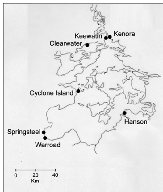
Figure 2.12. Lake level measurement stations on Lake of the Woods.
