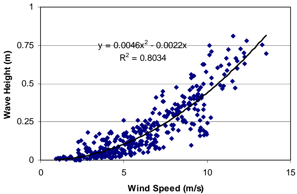
Figure 3.8. Raw station wind speed versus wave height for 1 hour averaging for the Pine Island station.
