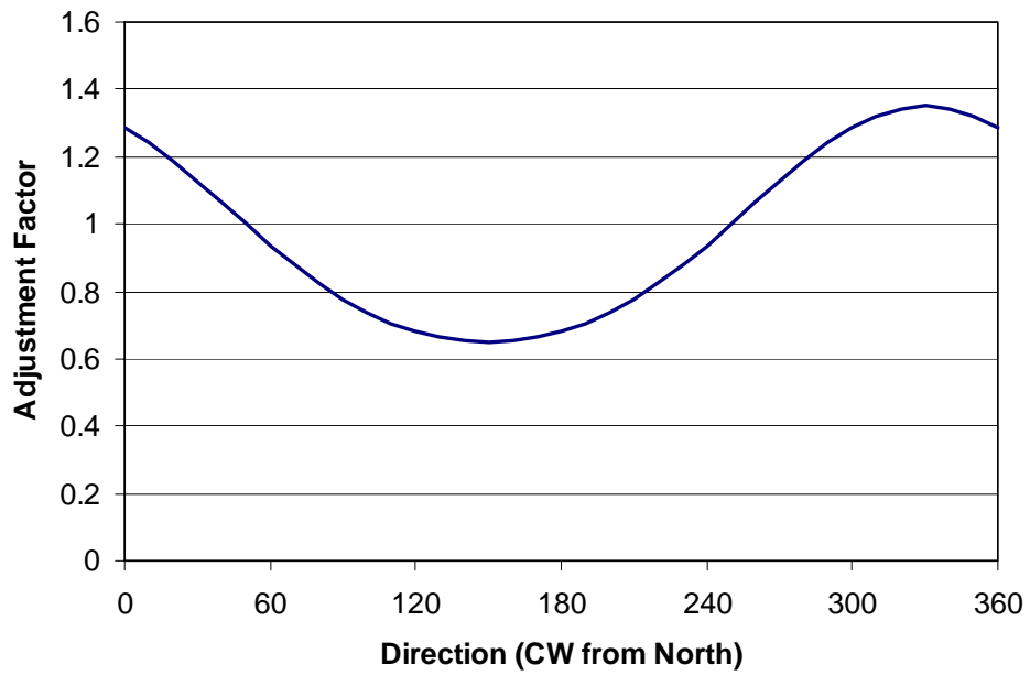
Figure 3.7. Wind speed adjustment factor versus wind direction for the Pine Island station.
