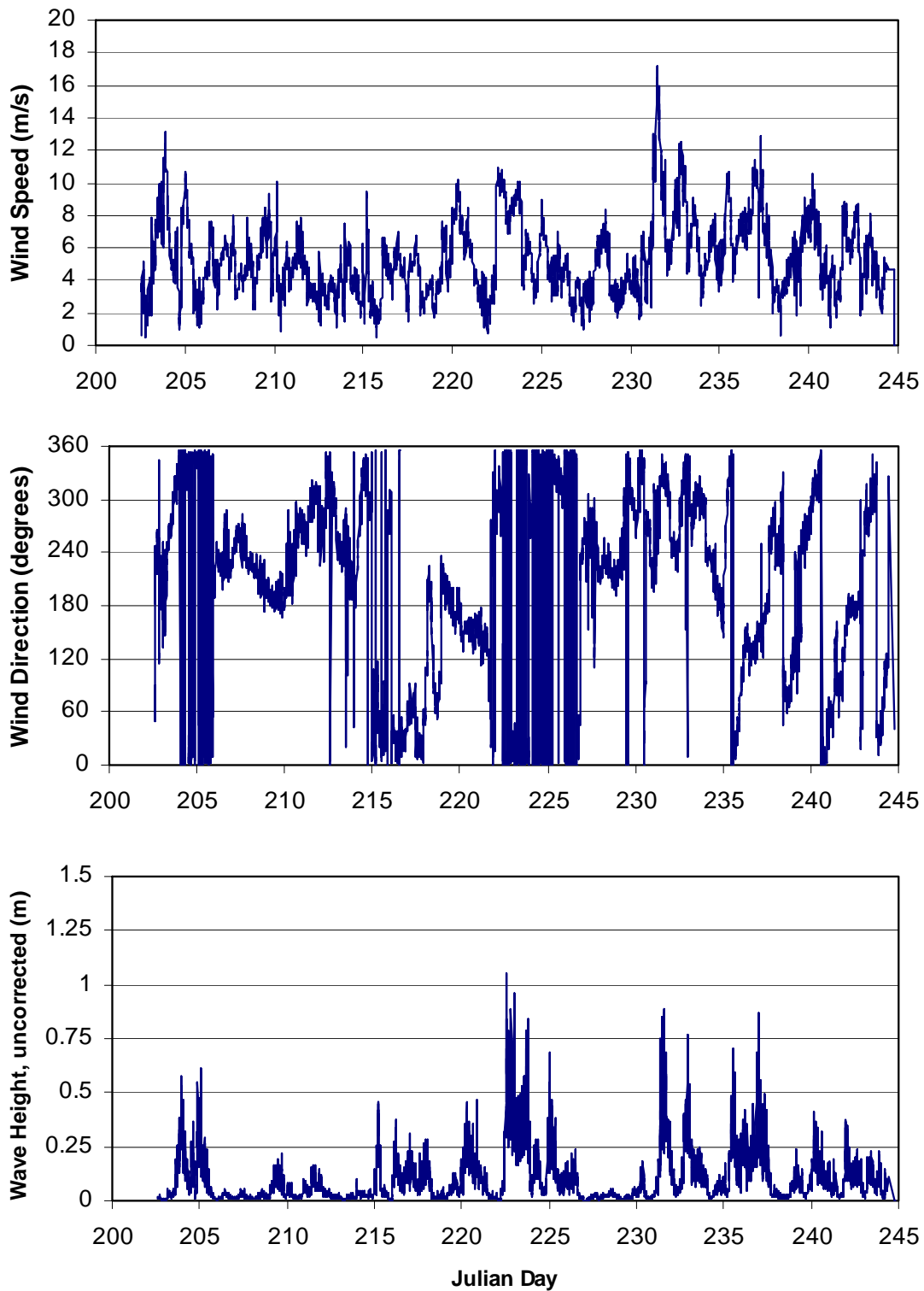
Figure 3.3. 10 minute wind speed, wind direction, and wave height data (uncorrected) for the Sandy Shores station, July 20 to August 31, 2004.
