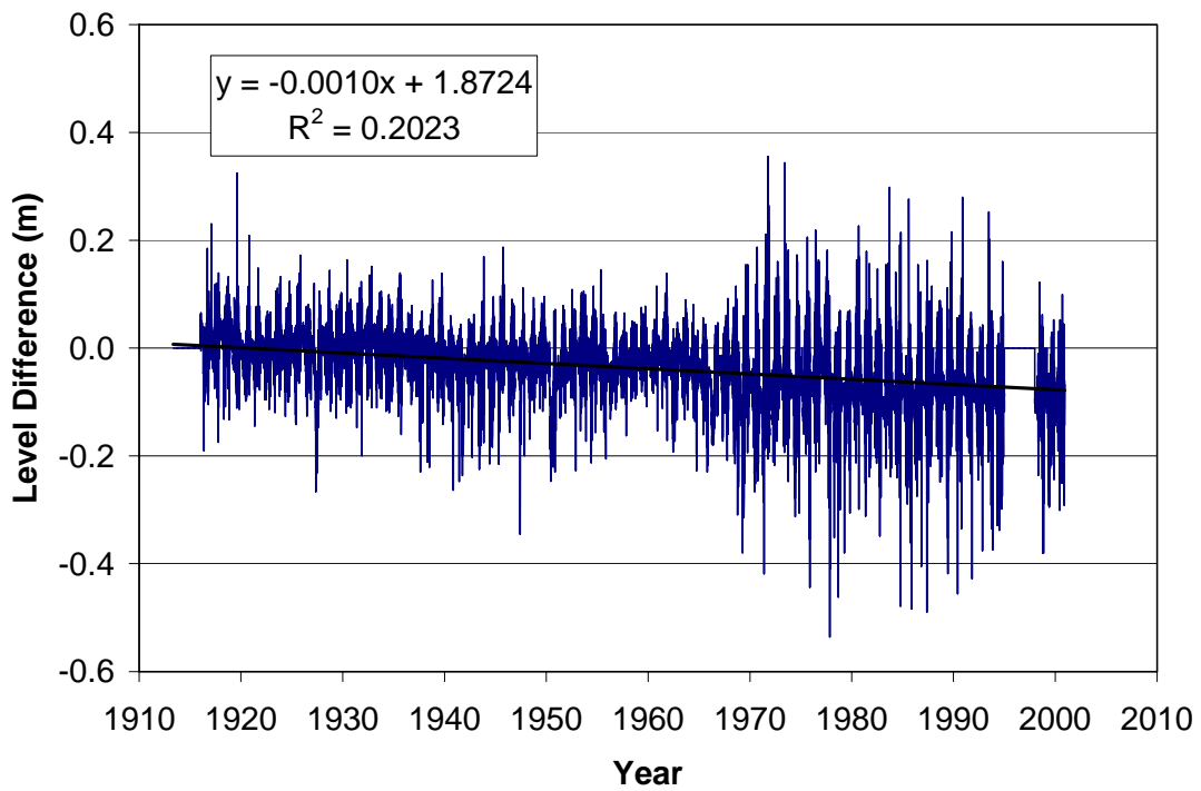
Figure 4.4. Lake level difference (Warroad-Keewatin) for monthly mean values, 1916-2003.
