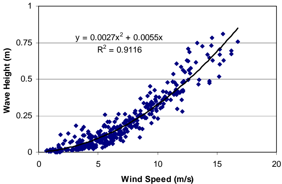
Figure 3.9. Adjusted station wind speed versus wave height for 1 hour averaging for the Pine Island station.
