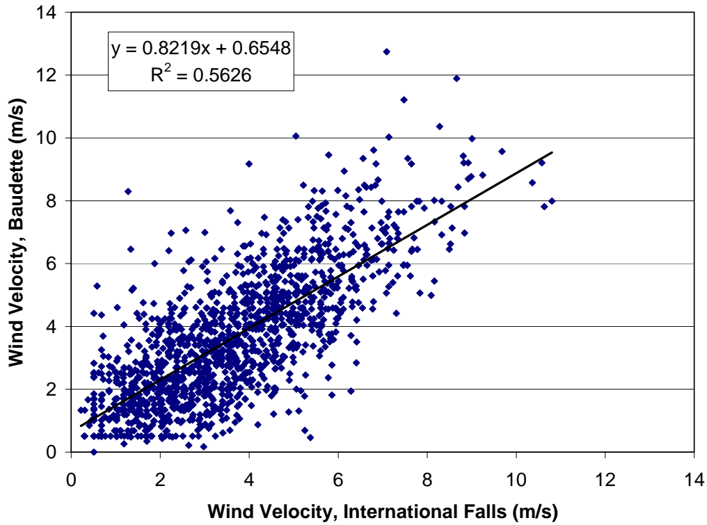
Figure 5.2. Three hour averaged wind velocity for Baudette versus International Falls, 2003.
