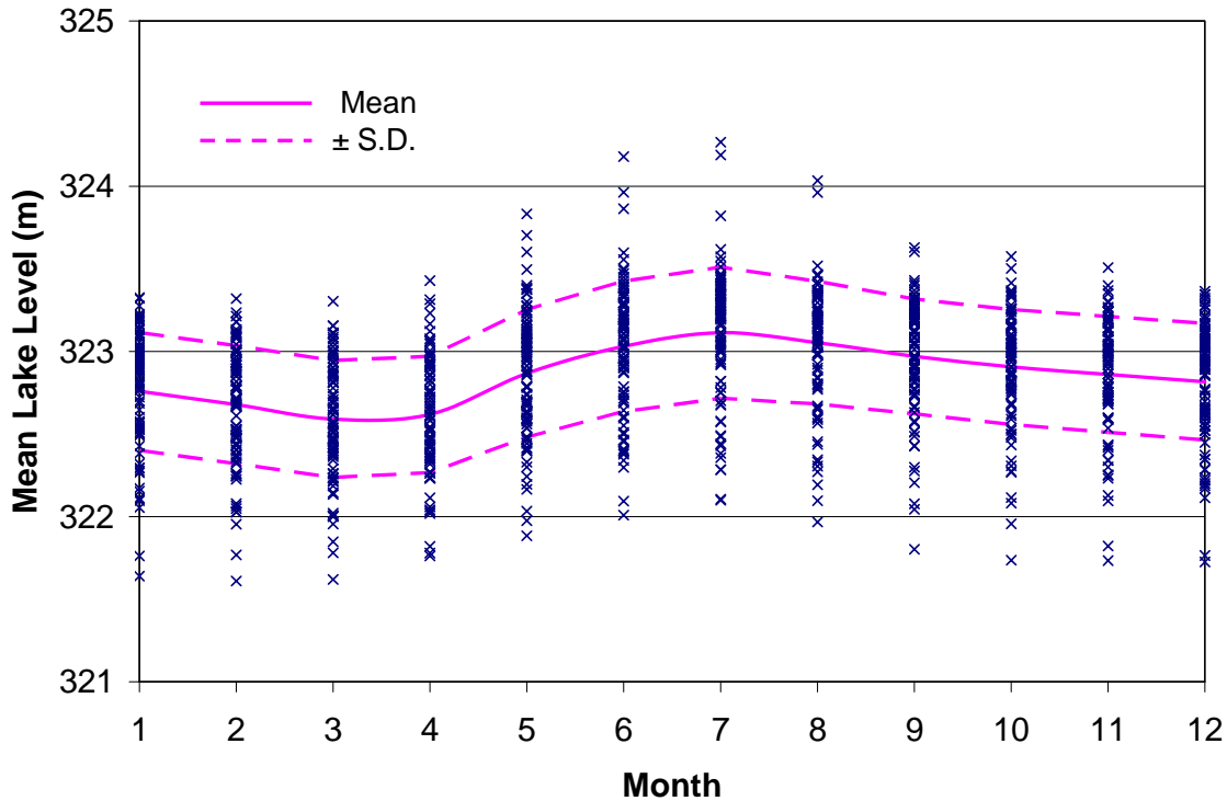
Figure 4.5. Seasonal variation in monthly mean lake level, averaged over multiple stations. Monthly mean values are plotted as a solid line with \pm 1 STD as a dashed line.
