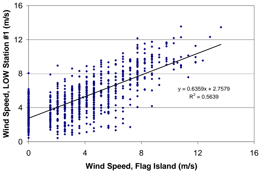
Figure 5.3. Pine Island station wind speed versus Flag Island wind speed for 1 hour averaged data, all directions, June 16 to July 20, 2004.
