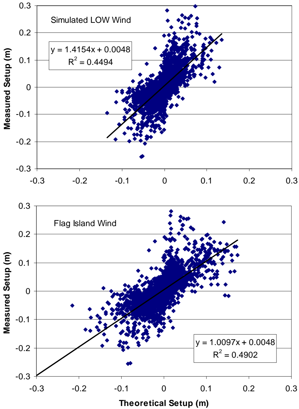
Figure 7.2. Calculated vs. measured wind setup for Warroad and Cyclone Island gages, 1 hour time scale, May 1 to November 1, 2000. Theoretical setup calculated using simulated LOW wind data (upper panel) and Flag Island wind data (lower panel).
