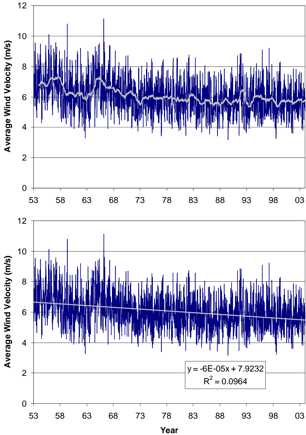
Figure 6.1. Weekly averaged wind velocity versus time for simulated LOW wind data, 1953 – 2003. The upper panel gives the weekly average data with a 52 week running average, while the lower panel gives a linear trend line. The overall mean is 6.06 m/s, with a standard deviation of 1.1 m/s.
