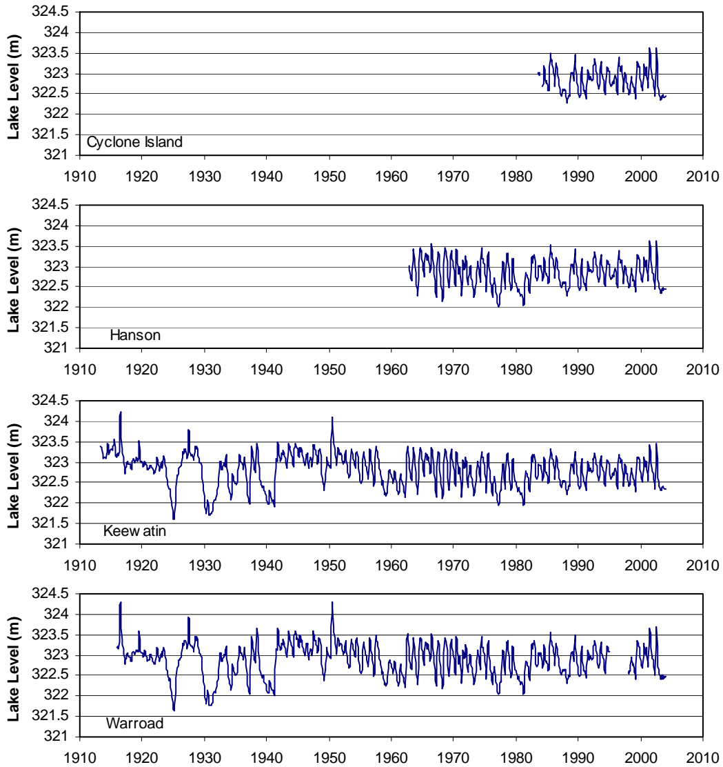
Figure 4.1. Monthly mean lake level for four Lake of the Woods measurement stations, 1913 to 2003.
