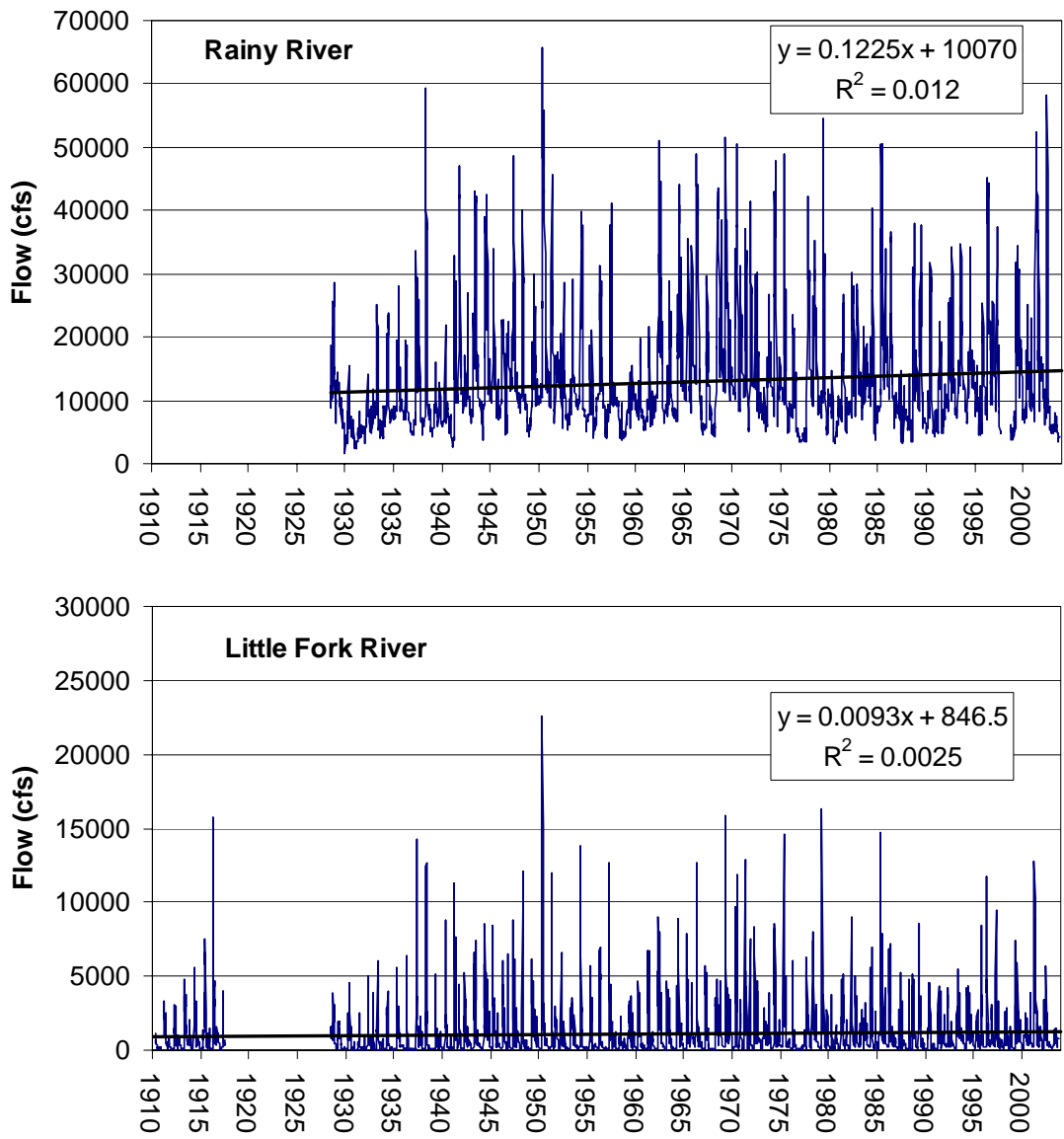
Figure 9.2. Weekly average flow rate for the Rainy River at Manitou Falls and the Little Fork River at Little Fork, MN, from USGS stream gaging stations.
