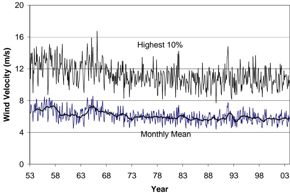
Figure 6.3. Monthly average and monthly average of highest 10% of wind velocity versus time for simulated LOW wind data, 1953 – 2003. The 12 month running average is also shown.
