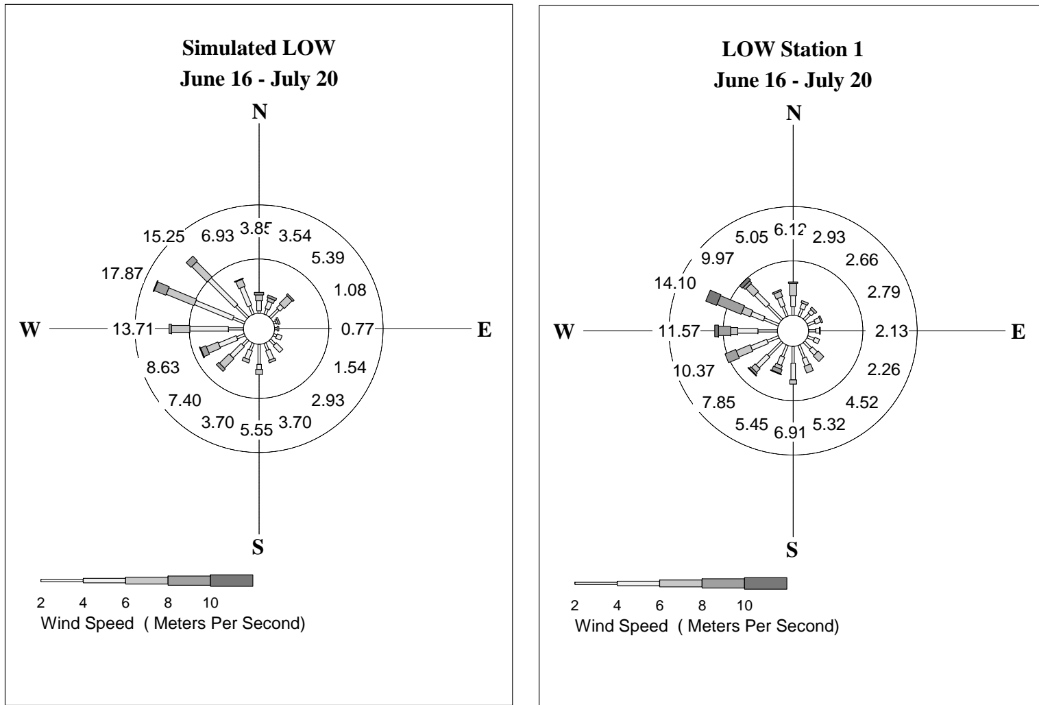
Figure 5.10. Wind rose plots for simulated LOW hourly wind record (Equation 5.1) and LOW station 1 (Pine Island) for June 16 to July 20, 2004.
