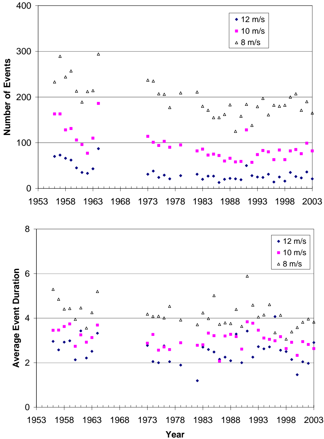
Figure 6.12. Number of wind events exceeding 8, 10, and 12 m/s per year (upper panel) and average event duration (lower panel) for simulated LOW wind data, 1953 – 2003. Event duration analysis was performed only on years with 1 hour data sets (37 years).
