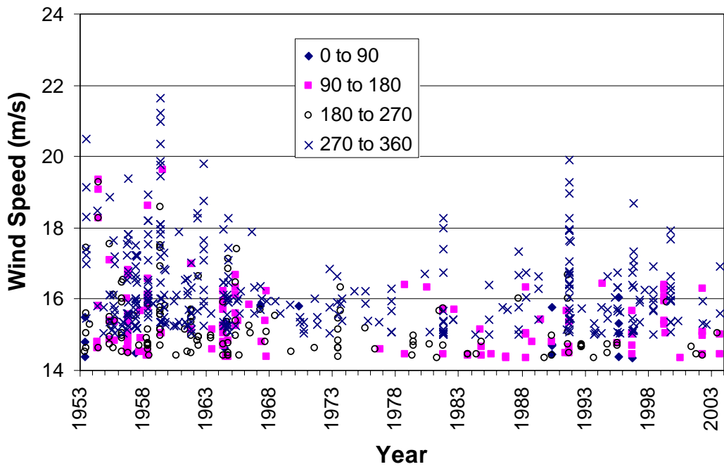
Figure 6.5. Highest hourly wind velocities versus time and direction for simulated LOW wind data, May – October, 1953 – 2003.
