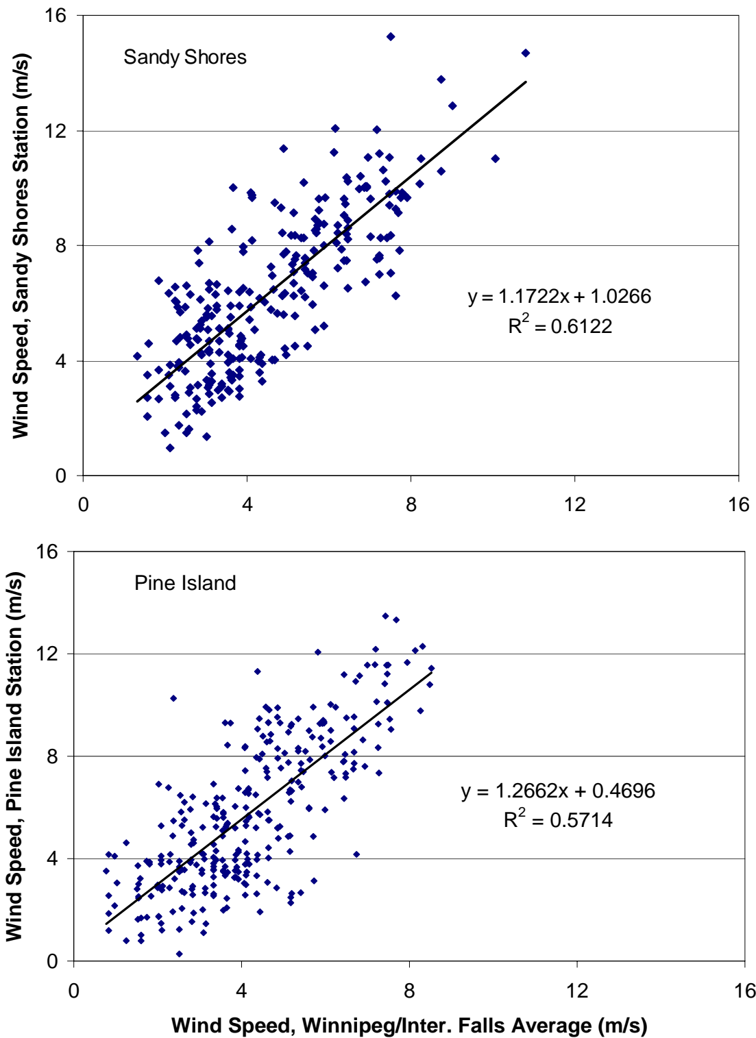
Figure 5.6. Measured LOW wind speed versus average Winnipeg-International Falls wind speed for Sandy Shores (upper panel) and Pine Island (lower panel) for 1 hour averaged winds from the northwest quadrant (270°-360°) only.
