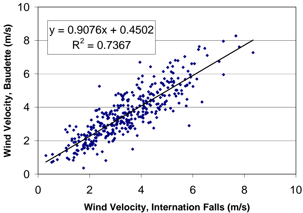
Figure 5.1. Daily averaged wind velocity for Baudette versus International Falls, 2003.
