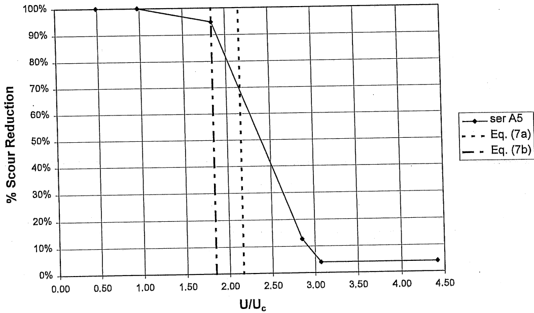
Figure 5.4. Riprap performance for series A5. The vertical lines denote values of U_{rc}/U_c from Eqs. (3.7a) and (3.7b).
