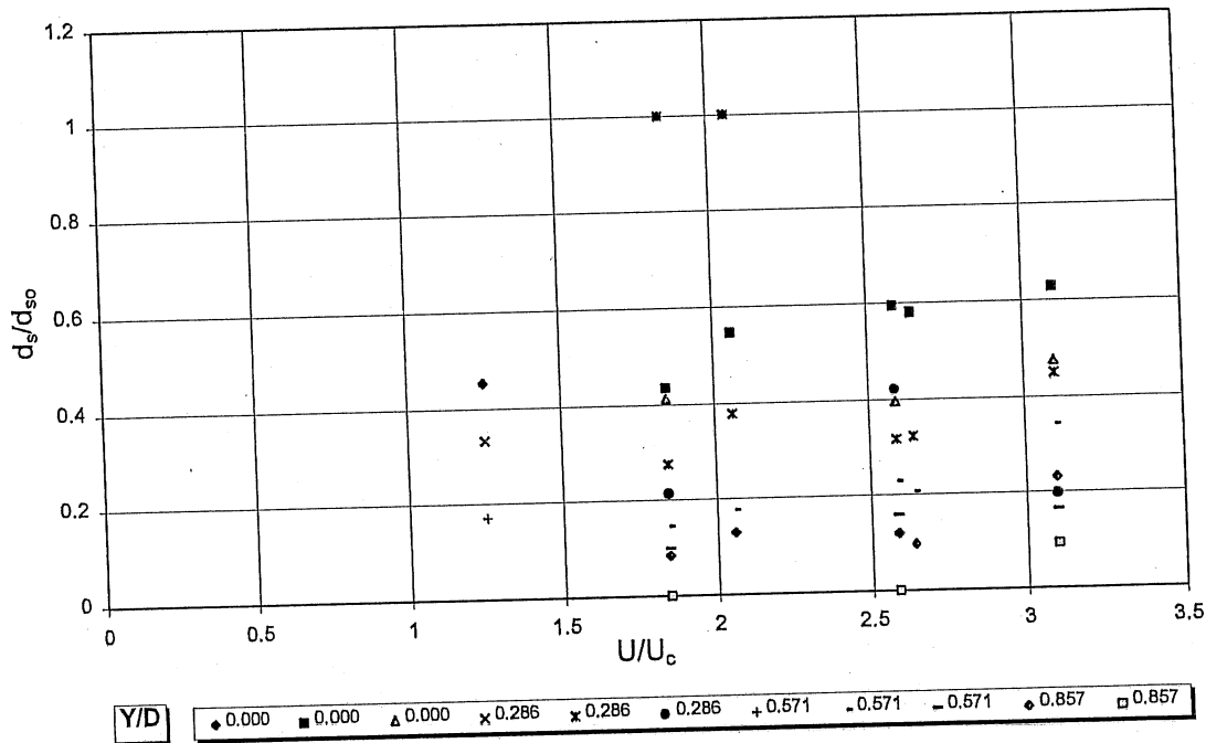
Figure 4.4. Scour reduction achieved as a function of U/U_c for various initial placement levels. The first, fourth and seventh values of Y/D correspond to the 7.8 mm riprap; the second, fifth, eighth and tenth values correspond to the 16 mm riprap; the third, sixth, ninth and eleventh points correspond to the 22 mm riprap.
