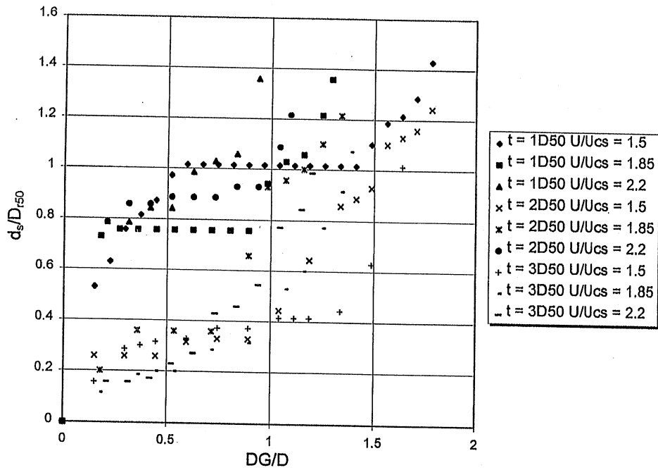
Figure 4.15. Comparison of thickness effects for a degrading bed for the case c = 4D , D_{150} = 16 mm. In the legend, “D50” indicates the notation D_{150} in the text, and “U/Ucs” indicates the notation U/U_c in the text.
