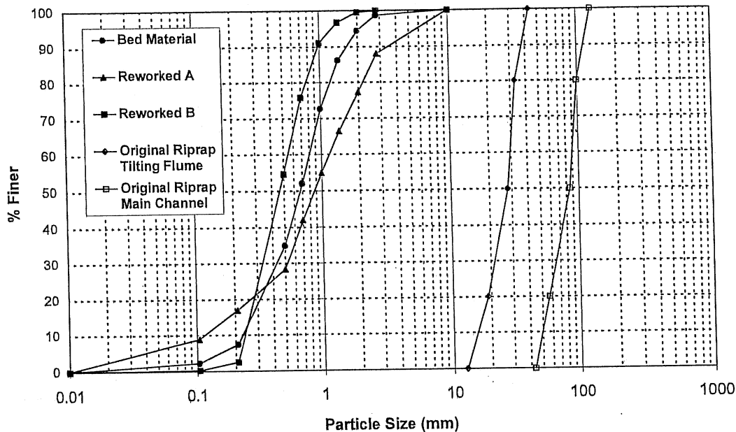
Figure 3.5. Grain size distributions of the sediment and riprap.
