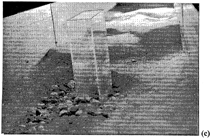
Figure 3.11. a) Side view of the rectangular pier at the end of Run 4 of series TF-RR1. b) View of the same rectangular pier looking upstream. c) View looking upstream of the rectangular pier at the end of Run 4 of series TF-RR2.
