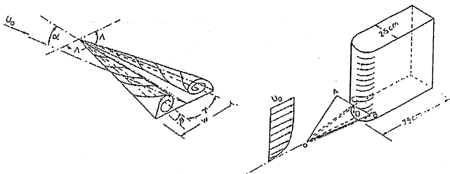
Figure 2.11. Delta wing plates.
