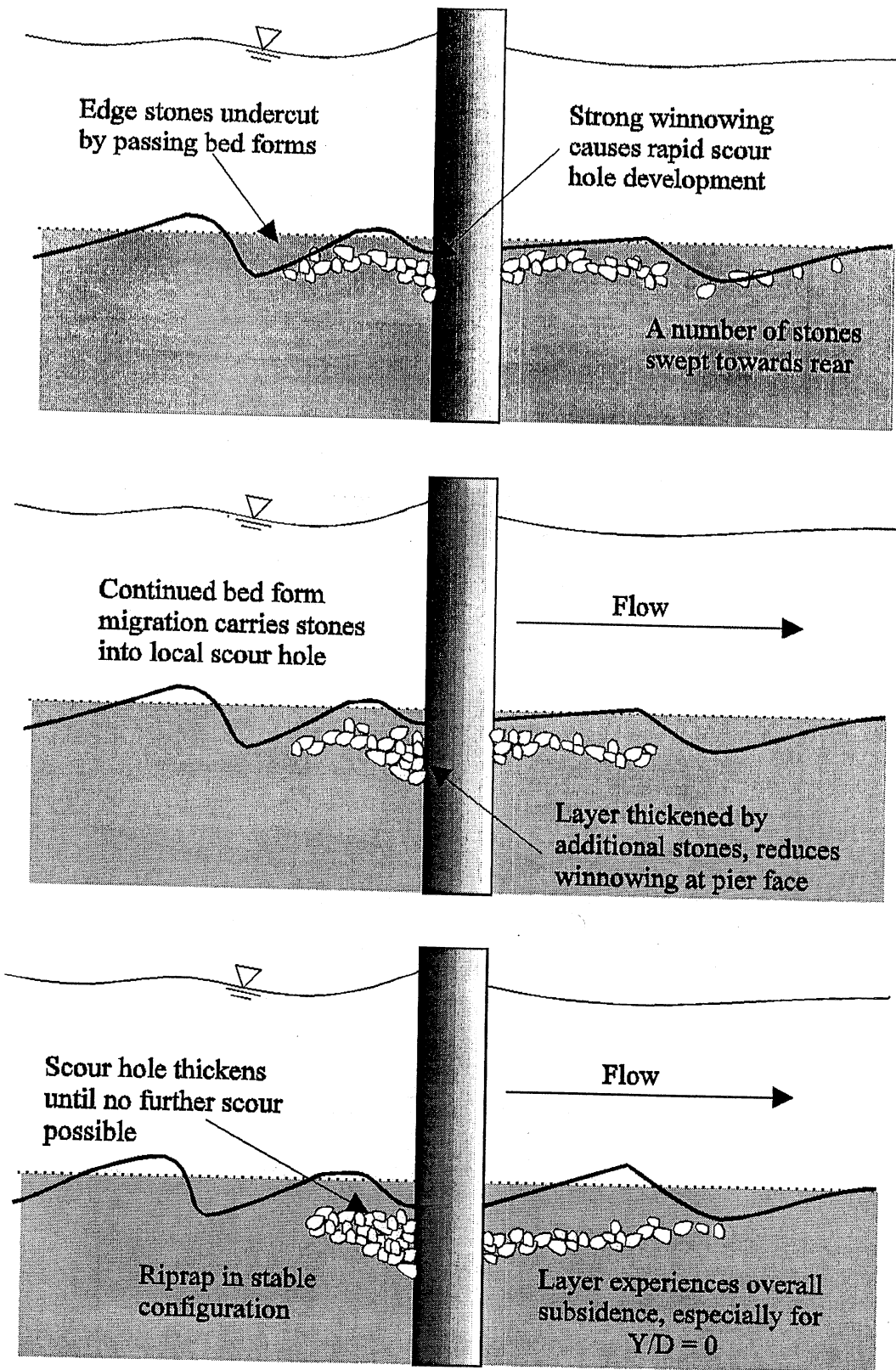
Figure 4.8b. Illustration of the failure of a riprap layer for t=1 D_{150} .
