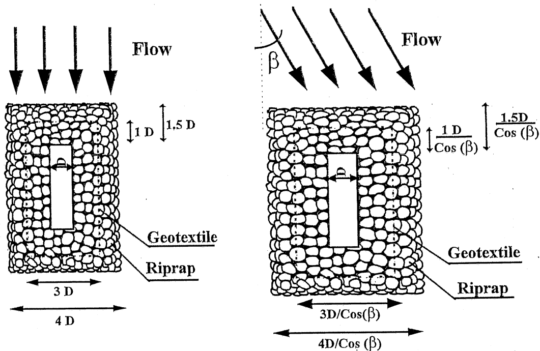
Figure 8.4. Riprap and geotextile cover with prior excavation.
