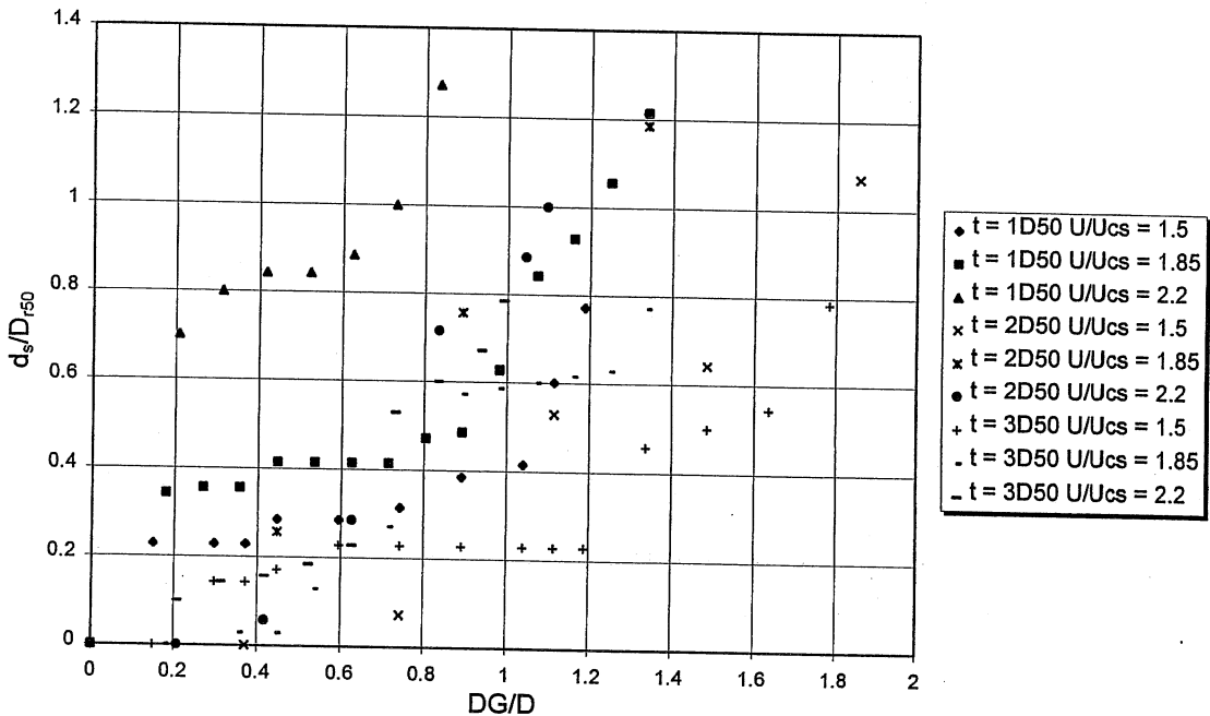
Figure 4.16 Comparison of thickness effects for a degrading bed for the case c = 4D , D_{150} = 22 mm. In the legend, “D50” indicates the notation D_{150} in the text, and “U/Ucs” indicates the notation U/U_c in the text.
