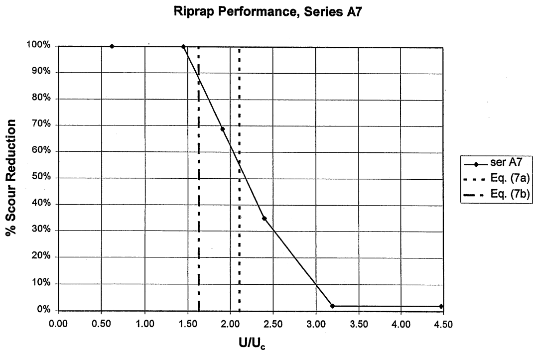
Figure 5.6. Riprap performance for series A7. The vertical lines denote values of U_r/U_c from Eqs. (3.7a) and (3.7b).
