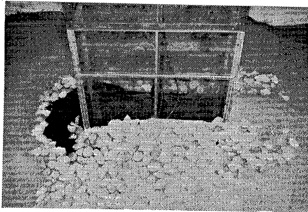
Figure 3.24. Riprap layer at the rectangular pier at the end of Run 3 of series MC-RNX.
