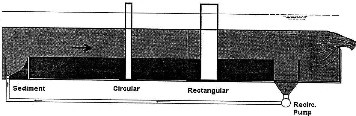
Figure 3.1. Schematic diagram of the Main Channel facility.
