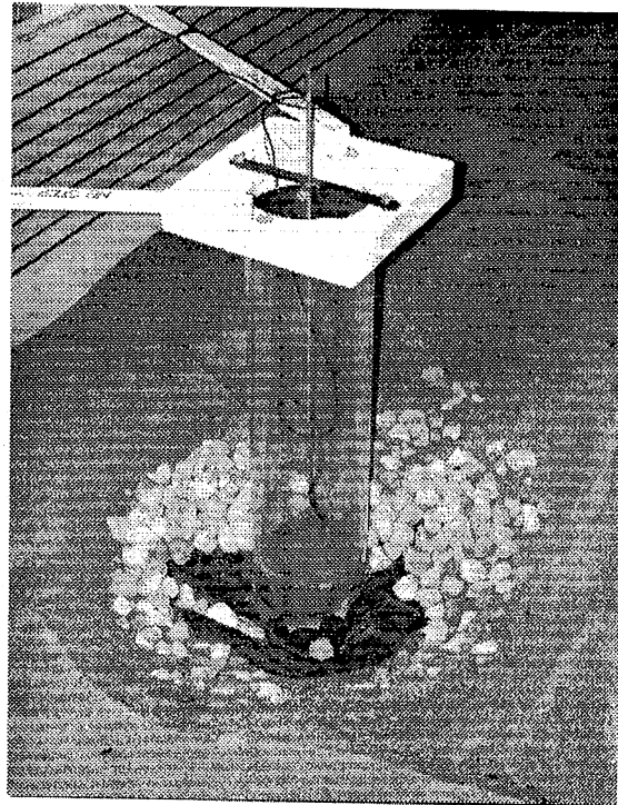
Figure 3.20. a) Side view of the riprap failure near the rectangular pier of Run 4 of series MC-RPG. b) Downstream view of the riprap failure near the rectangular pier (Run 4 of series MC-RPG). c) Downstream view of the riprap failure near the cylindrical pier (Run 4 of series MC-RPG).
