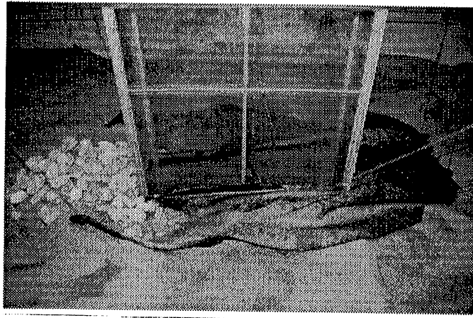
Figure 3.26. Illustration of the low-water installation technique for geotextile and riprap. The flow has been temporarily halted to improve visibility.
