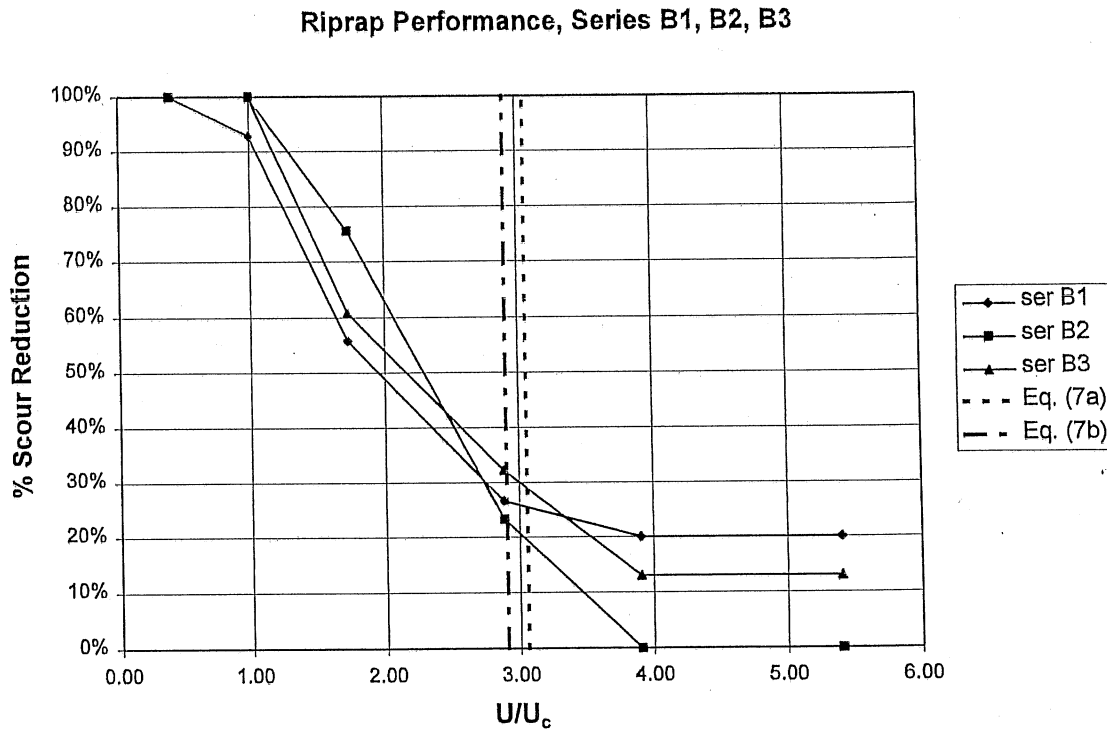
Figure 5.7. Riprap performance for series B1, B2 and B3. The vertical lines denote values of U_{tr}/U_c from Eqs. (3.7a) and (3.7b).
