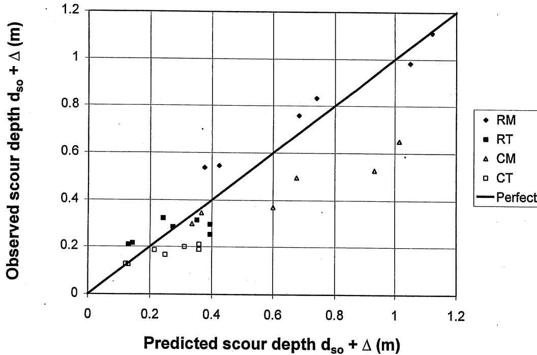
Figure 3.6c. Comparison of the data for unprotected scour with the Colorado State University predictor.
