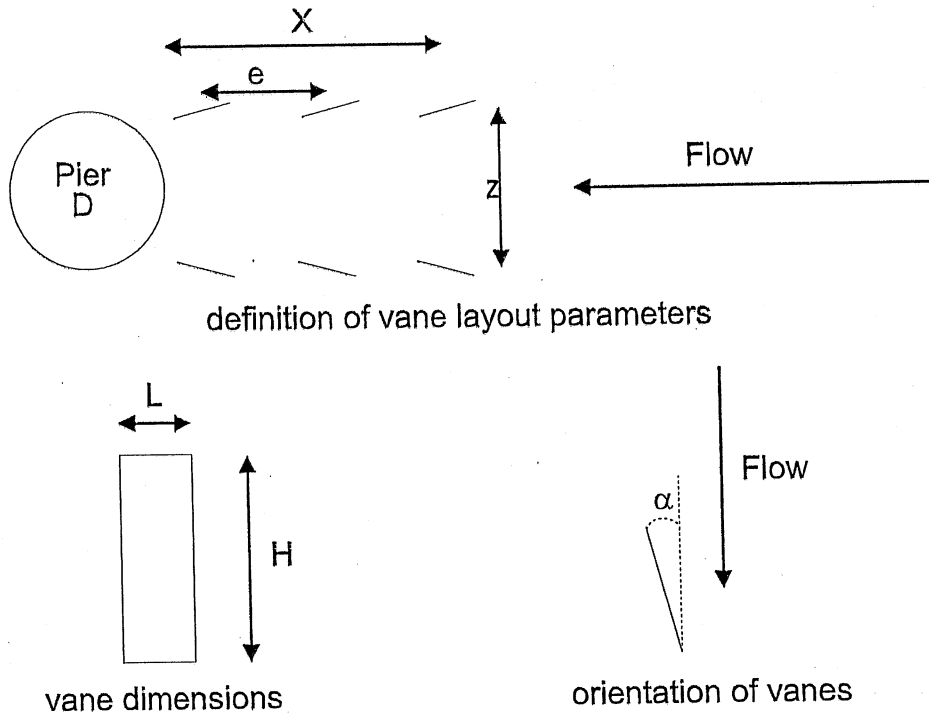
Figure 4.25. Definitions of parameters for submerged vanes.
