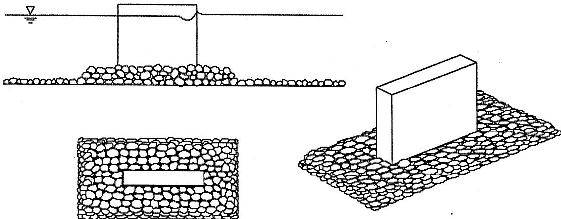
Figure 2.1. Riprap.
