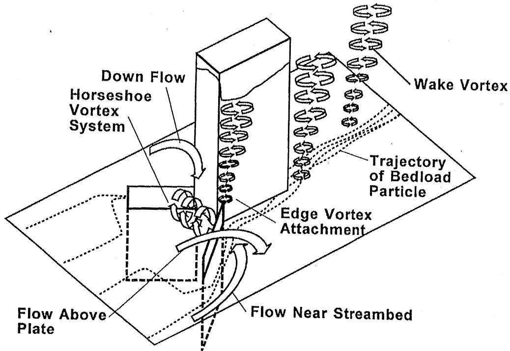
Figure 2.10. Vertical plates.
