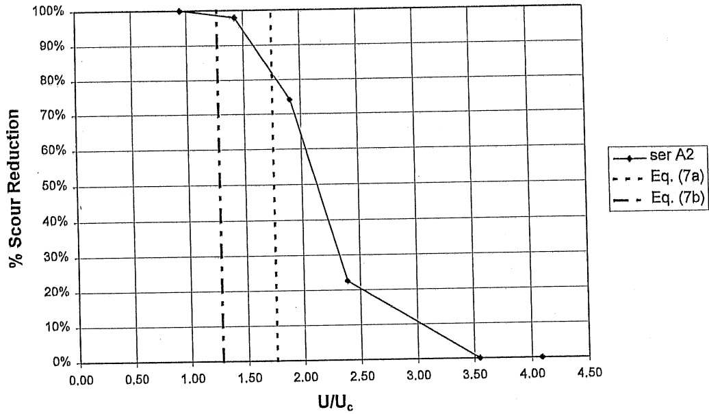
Figure 5.3. Riprap performance for series A2. The vertical lines denote values of U_{rc}/U_c from Eqs. (3.7a) and (3.7b).
