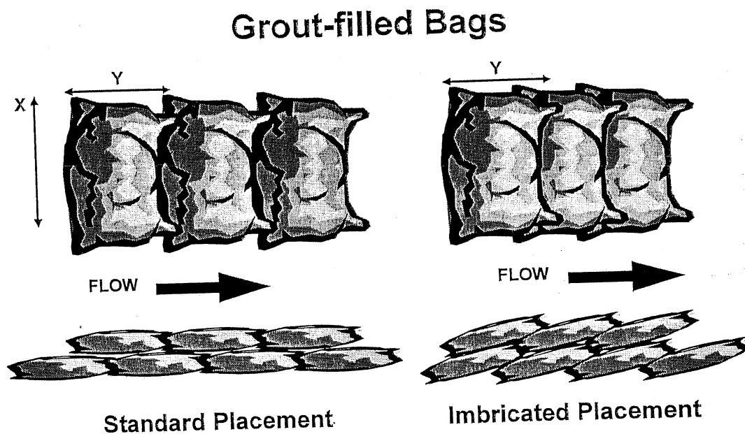
Figure 2.16. Grout filled bags.
