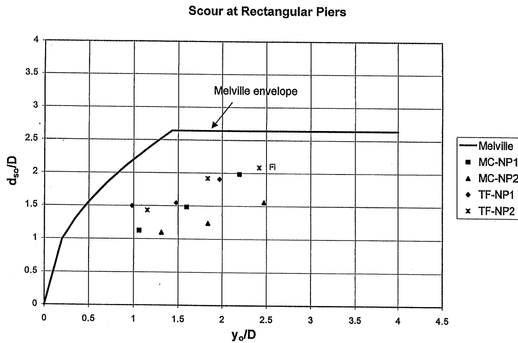
Figure 3.6b. Results for unprotected scour at rectangular piers.
