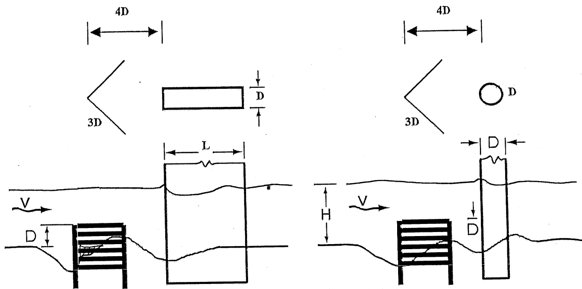
Figure 3.44a. Sheet pile configuration for series TF-SP1.
