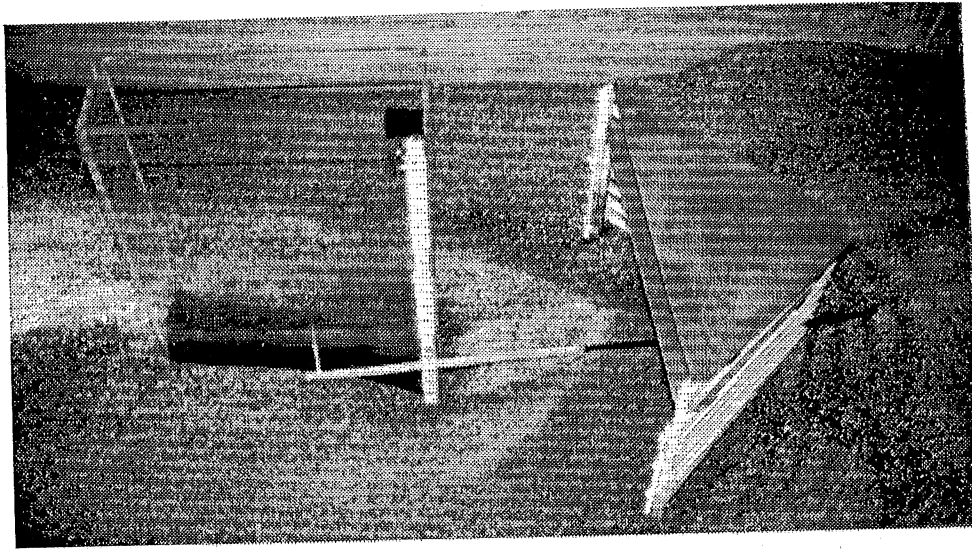
Figure 3.45c. View of the rectangular pier at the end of series TF-SP3.
