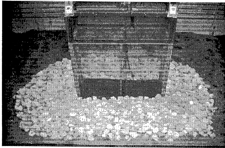
Figure 3.22. Placement of dumped riprap over a geotextile.
