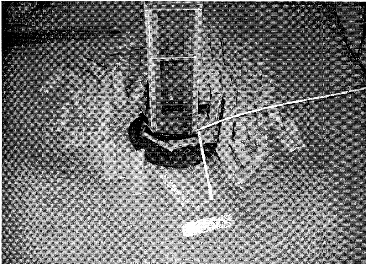
Figure 8.8c. Illustration of the dispersive sliding of grout filled bags under conditions for which the equivalent riprap did not fail.
