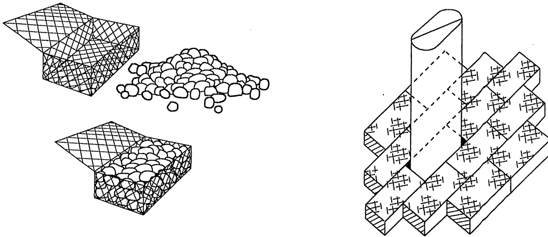
Figure 2.2. Gabions.
