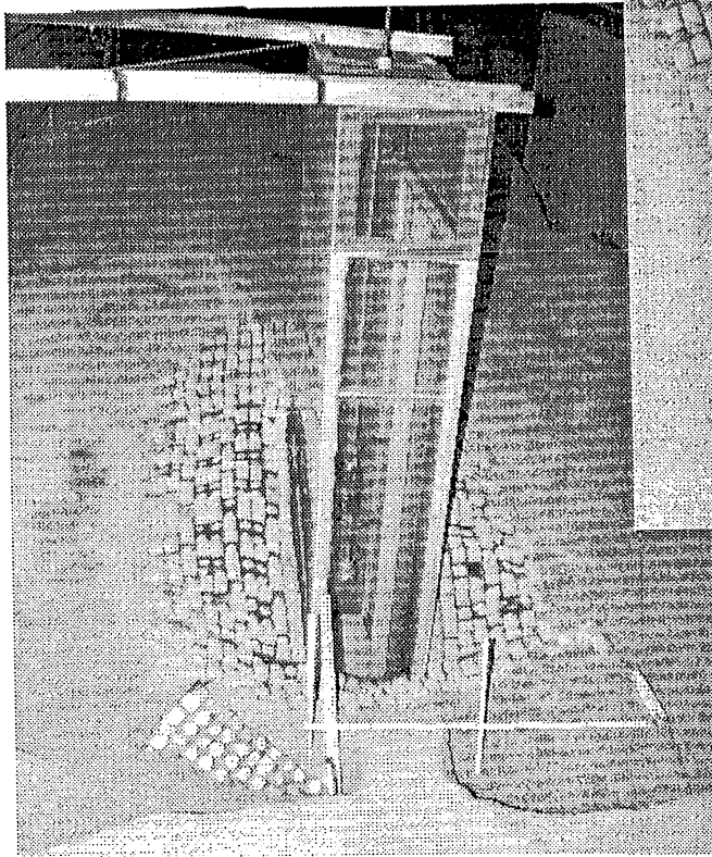
Figure 3.38. a) View of uplift failure at the rectangular pier at the end of Run 4 of series MC-CB3. b) Another view of the uplift failure.
