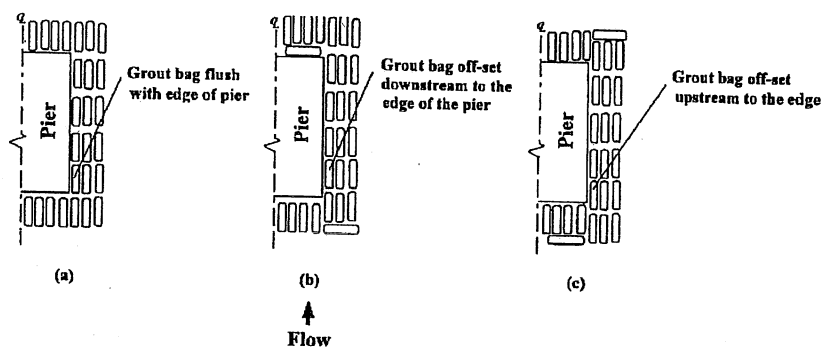
Figure 2.3. Grout filled bags.
