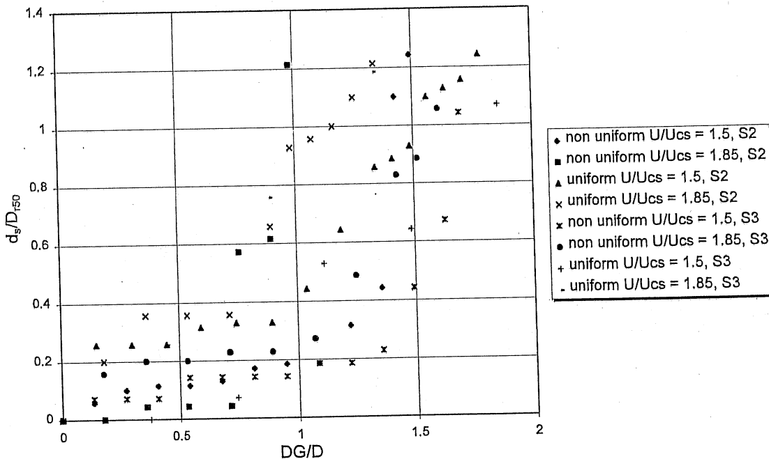
Figure 4.17. Comparison of local scour levels in uniform and non uniform sediments for c = 4D and t = 2D_{150} . In the legend "U/Ucs" indicates the notation U/U_c in the text, S2 denotes the riprap with D_{150} = 16 mm and S3 denotes the riprap with D_{150} = 22 mm.
