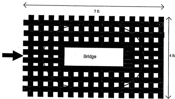
Figure 3.39d. Placement of grout filled bags around the rectangular pier for series MC-GB4, MC-GB5 and MC-GB6.
