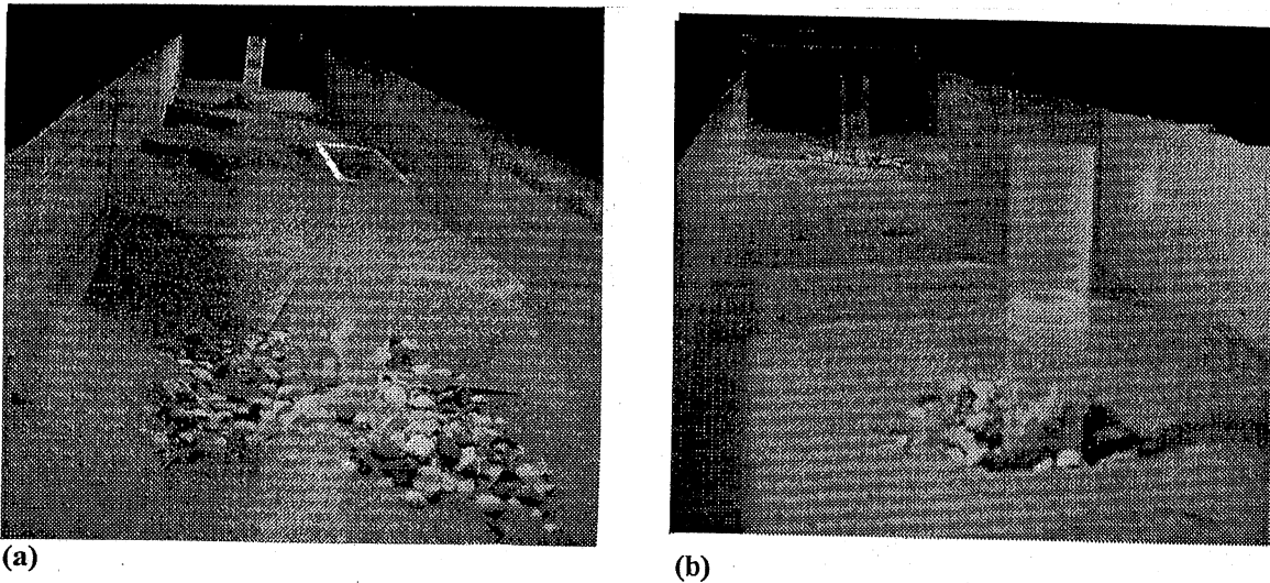
Figure 3.4. a) View of the Tilting Flume facility looking upstream. b) View of the Tilting Flume facility looking downstream.
