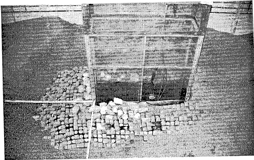
Figure 3.51. a) View of the rectangular pier at the end of Run 2 of series MC-CMB. b) View of the rectangular pier at the end of Run 3 of series MC-CMB.
