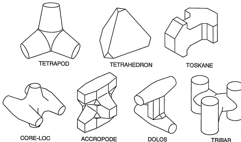
Figure 2.5. Tetrapods and related units.
