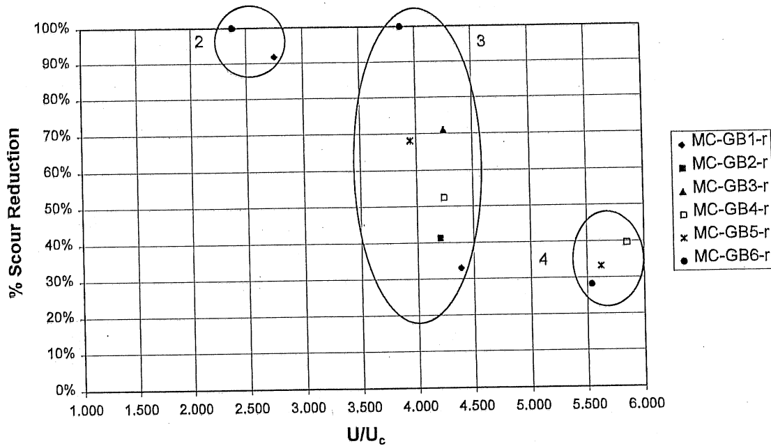
Figure 3.41. Performance of the grout filled bags at the rectangular pier for all the runs.
