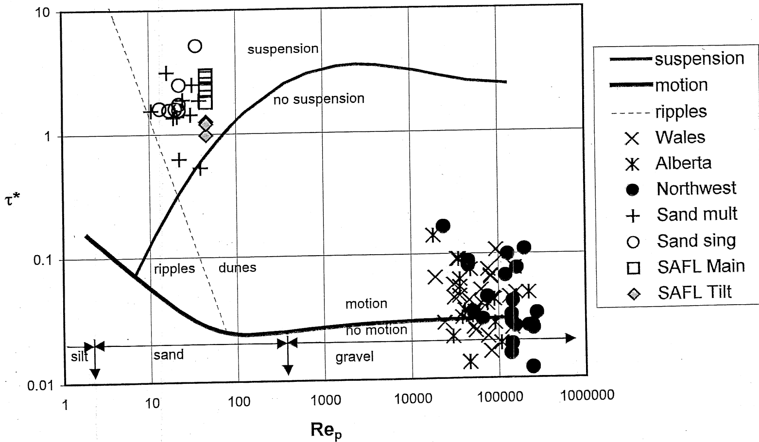
Figure 6.1. Regime diagram for rivers.
