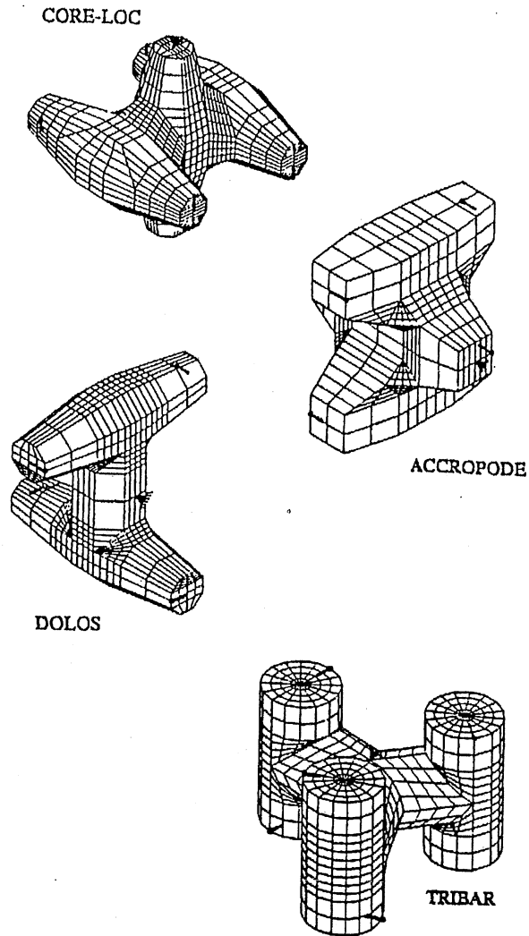
Figure 2.14. Artificial riprap.
