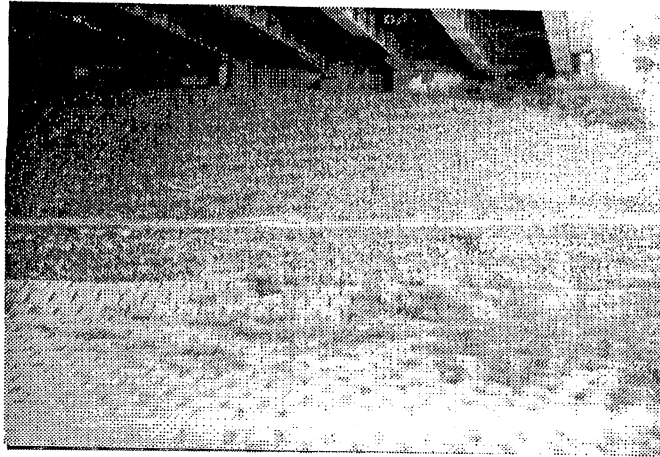
Figure 7.2. Shows cable tied blocks placed in channels underneath a multilane bridge.
