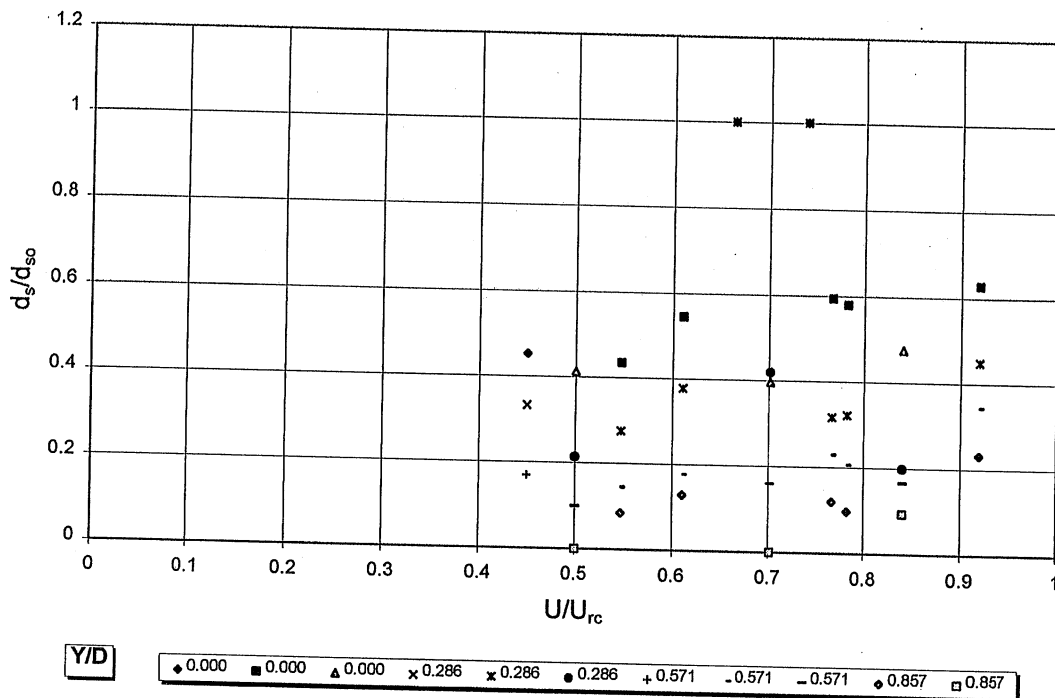
Figure 4.5. Scour reduction achieved as a function of U/U_{rc} for various initial placement levels. The first, fourth and seventh values of Y/D correspond to the 7.8 mm riprap; the second, fifth, eighth and tenth values correspond to the 16 mm riprap; the third, sixth, ninth and eleventh points correspond to the 22 mm riprap.
