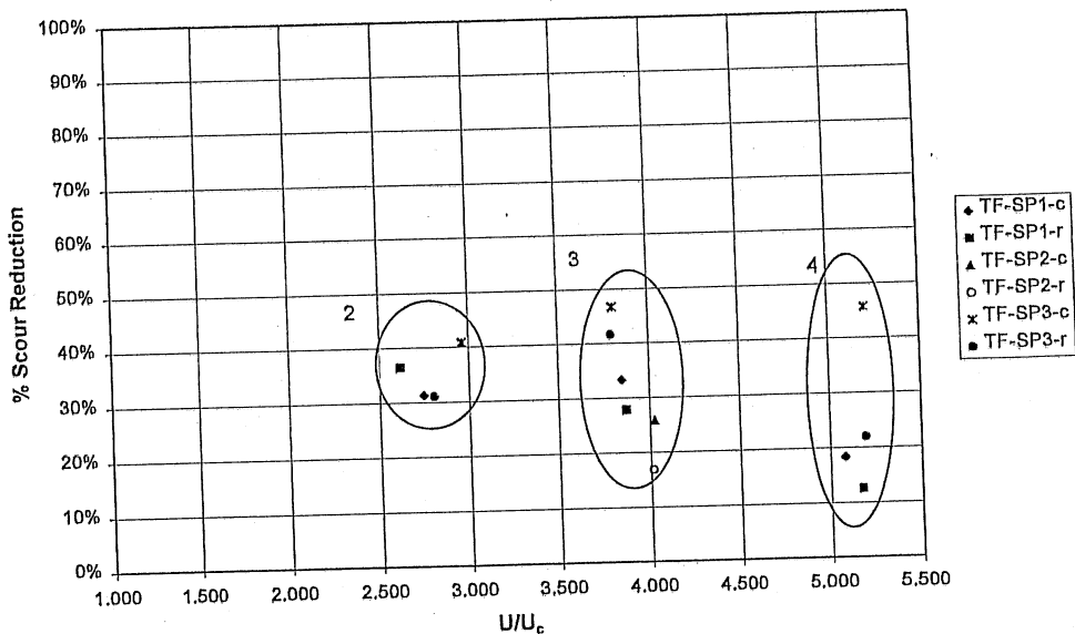
Figure 3.46. Performance of permeable sheet piles.
