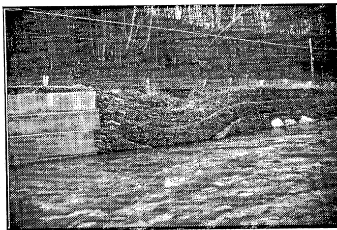
Figure 7.1. Shows baskets that have deformed and ruptured.
