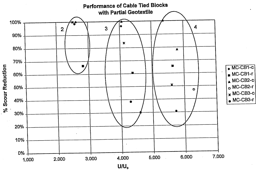
Figure 3.35. Comparison of the performance of cable tied blocks in the runs of series MC-CB1, MC-CB2 and MC-CB3.
