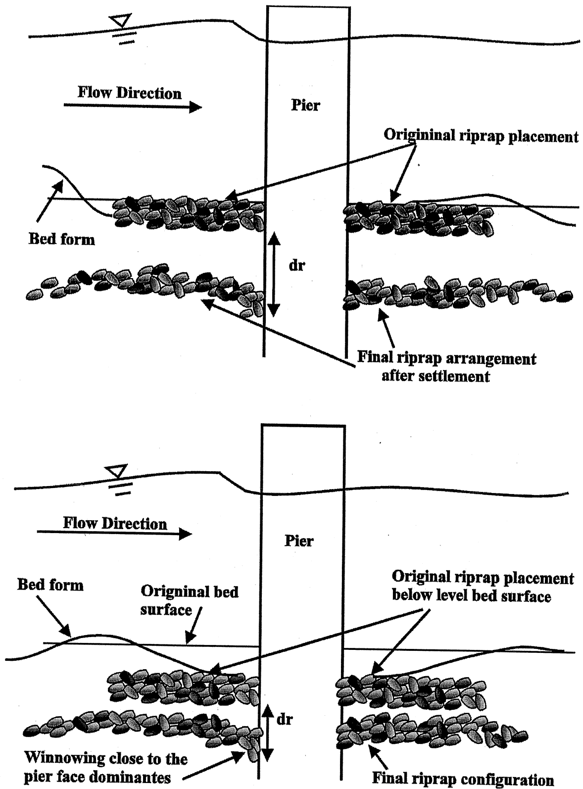
Figure 4.3. Effect of riprap placement on ultimate disposition.
