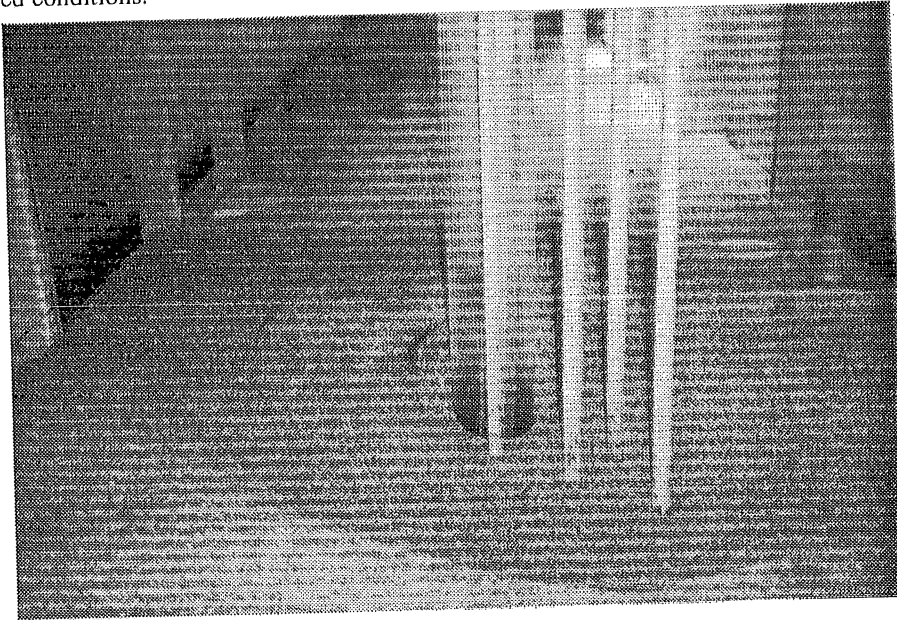
Figure 4.22. Illustration of a typical experiment on sacrificial piles under mobile bed conditions.
