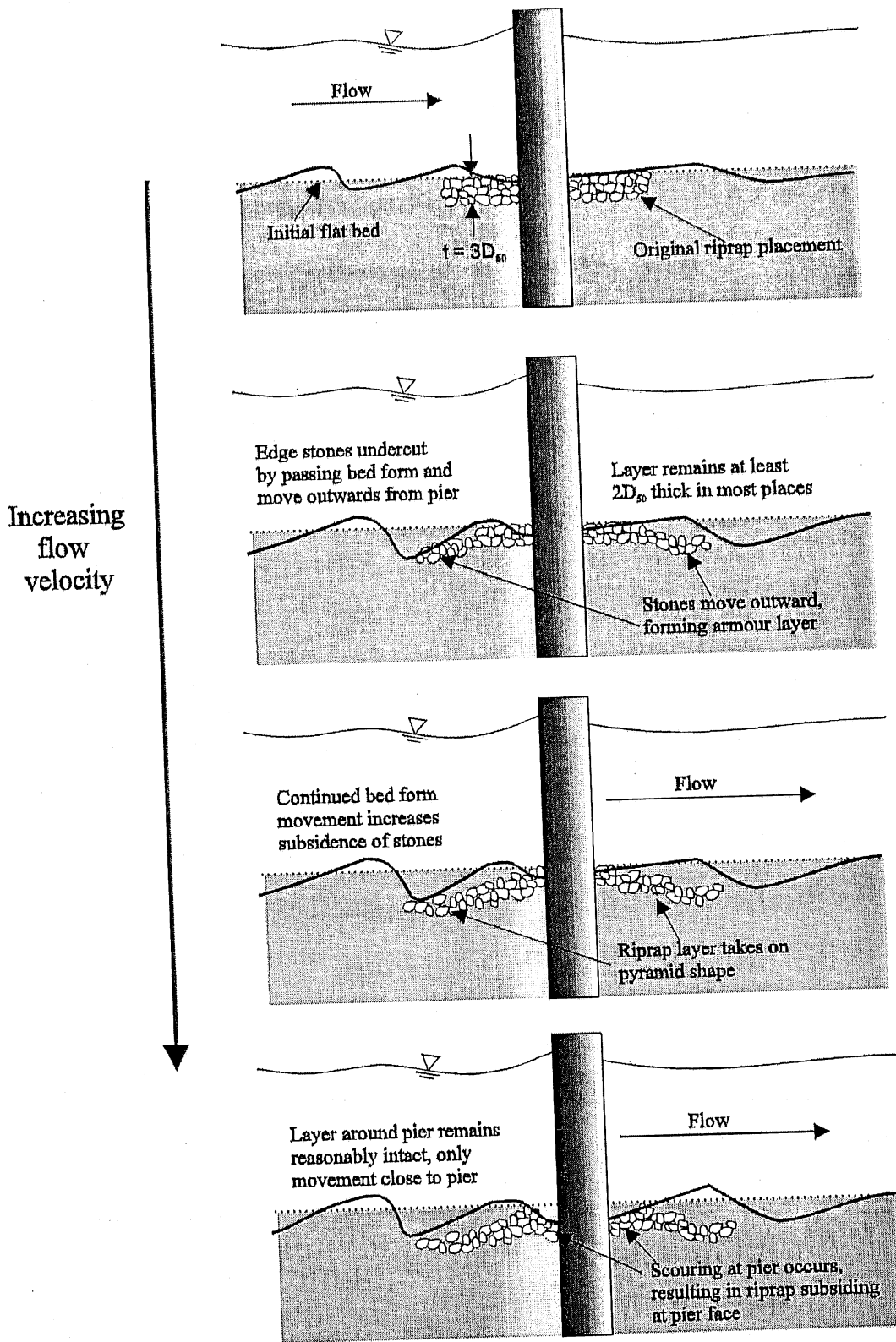
Figure 4.8a. Illustration of the failure of a riprap layer for t=3 D_{150} .
