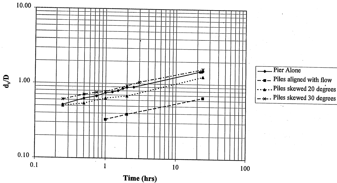
Figure 4.23. Clear-water scour depths for sacrificial pile arrangement no. 2 ( u./u_{*c} = 0.9 ).
