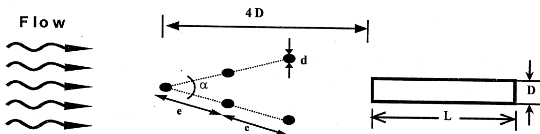
Figure 2.6. Sacrificial piles.
