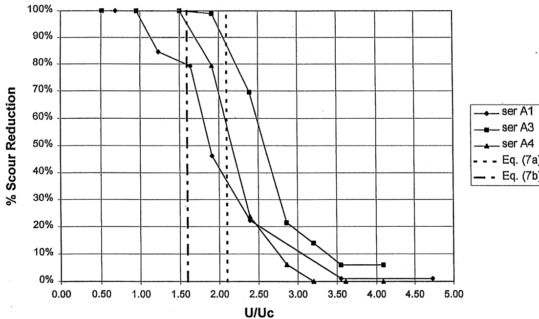
Figure 5.2. Riprap performance for series A1, A3 and A4. The vertical lines denote values of U_{cr}/U_c from Eqs. (3.7a) and (3.7b).
