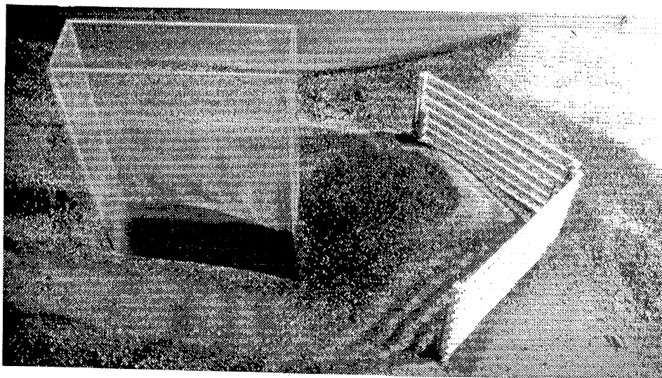
Figure 3.45a. View of the rectangular pier at the end of series TF-SP1.
