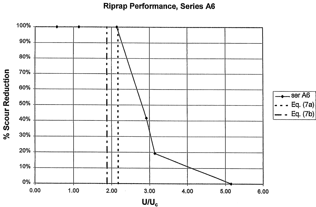
Figure 5.5. Riprap performance for series A6. The vertical lines denote values of U_r/U_c from Eqs. (3.7a) and (3.7b).
