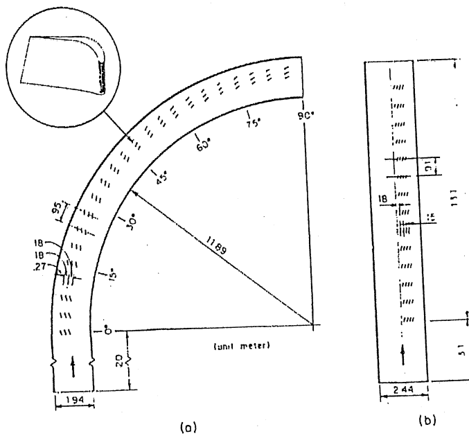
Figure 2.9. Iowa vanes.
