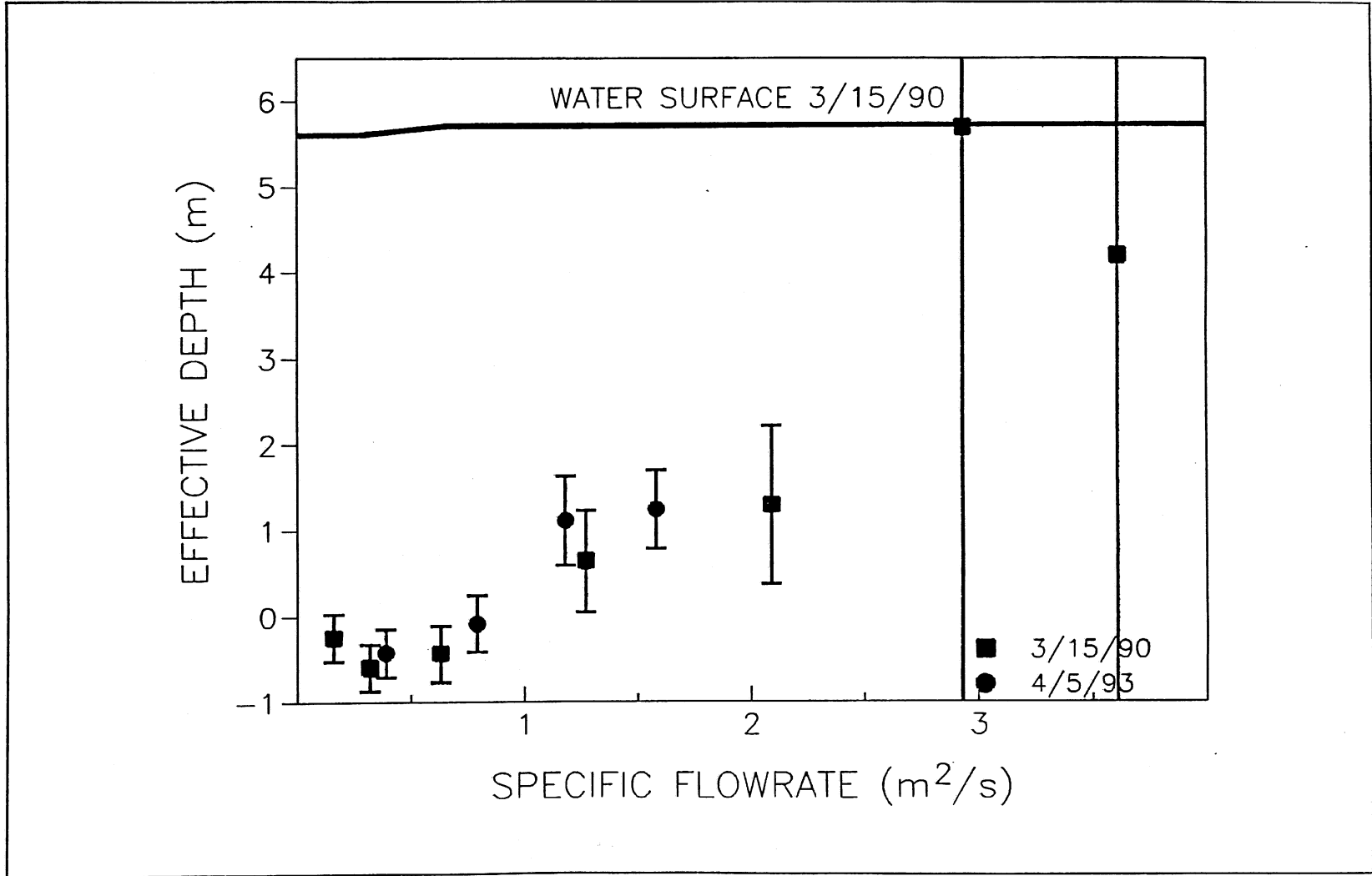
Figure 12. Effective depth versus specific discharge at St. Cloud Dam
