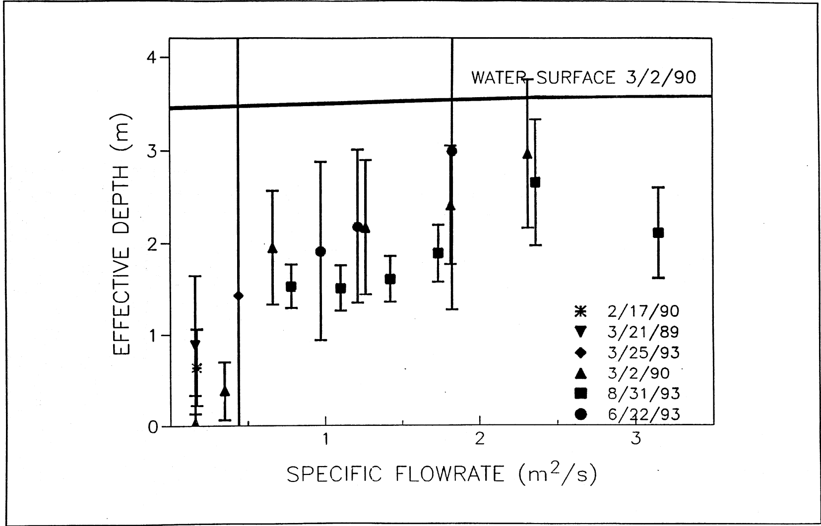
Figure 11. Effective depth versus specific discharge at Rum River Dam
