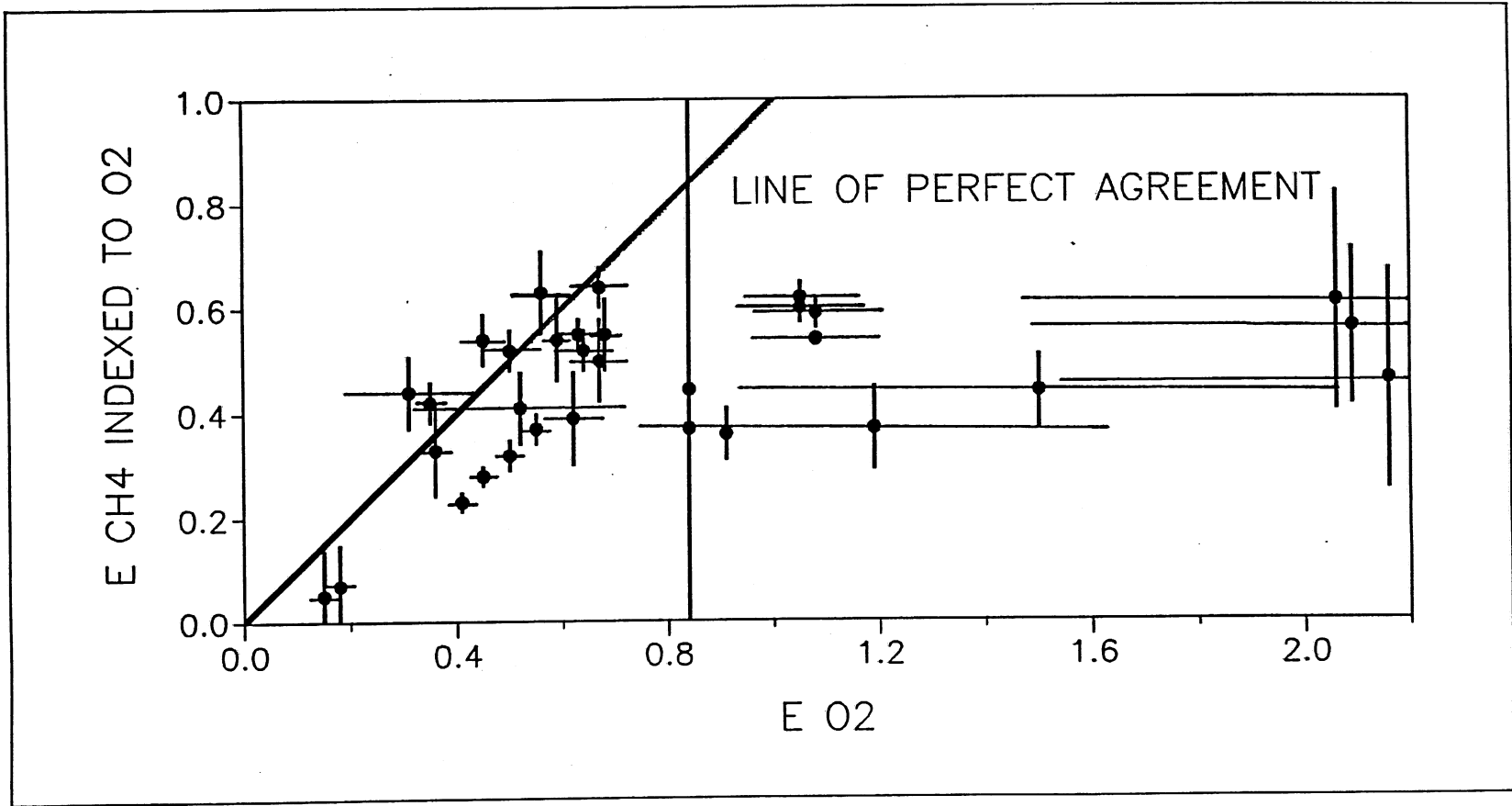
Figure 3. Oxygen transfer efficiency versus methane transfer efficiency indexed to oxygen
