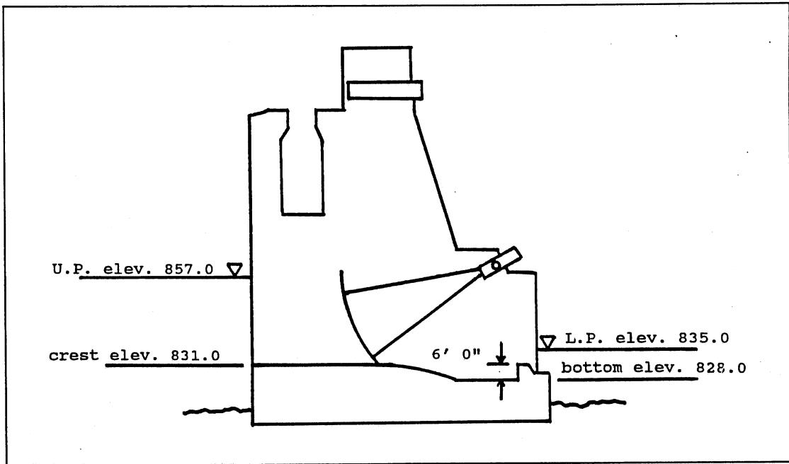
Figure B9. Profile view of Opekiska Lock and Dam
