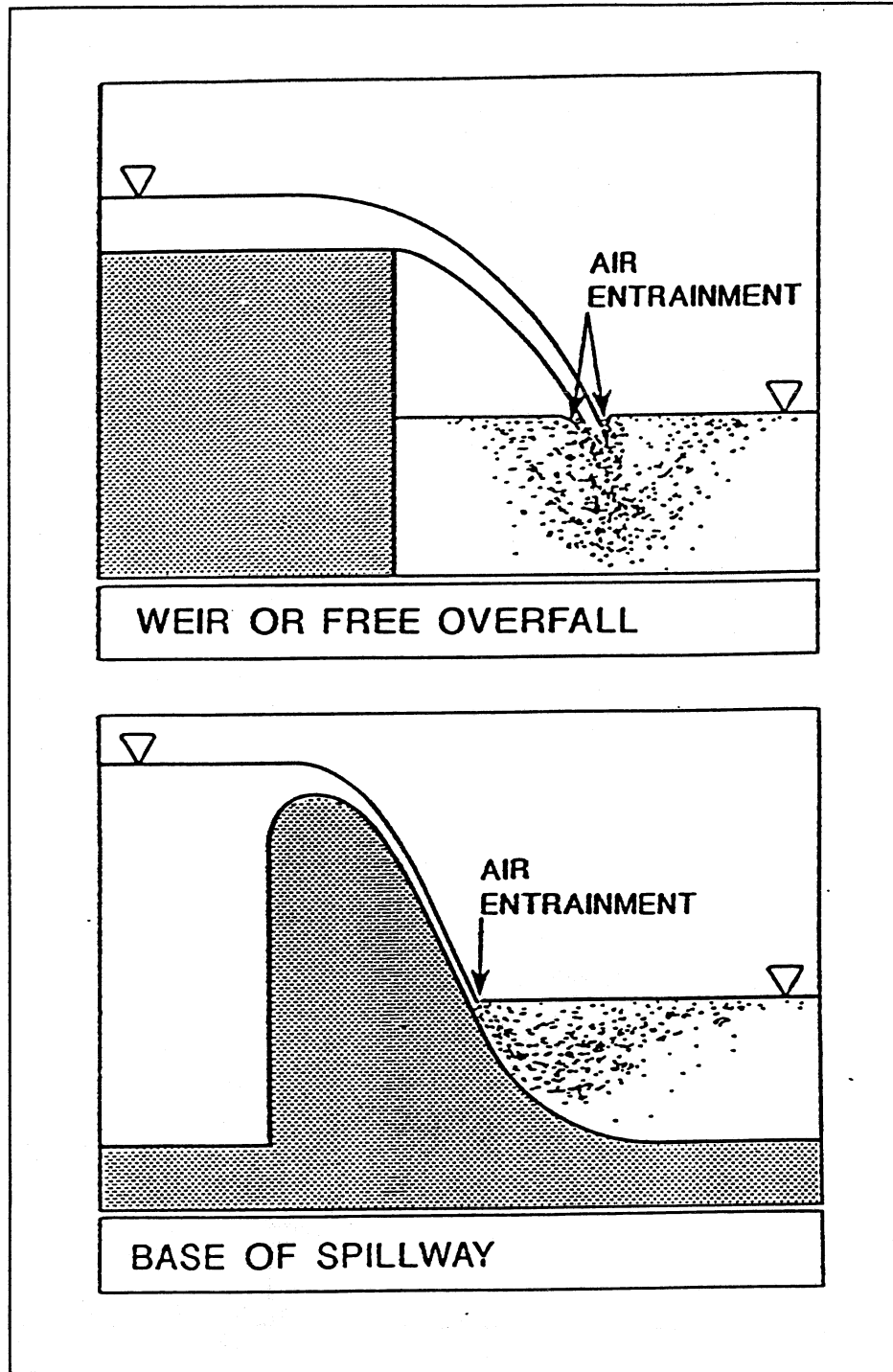
Figure 4. Air entrainment at plunge pool surface
