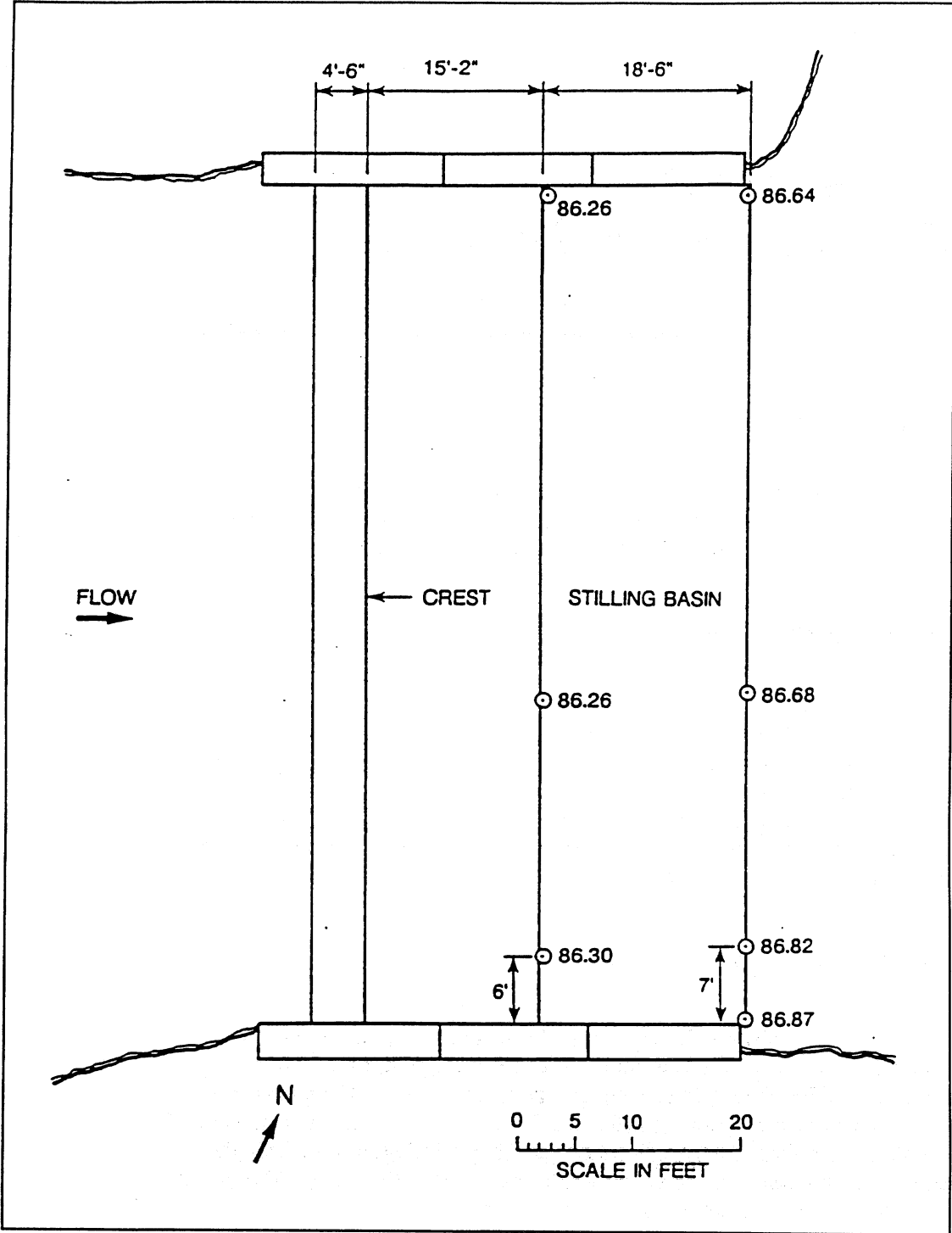
Figure B1. Plan view of Kost Dam
