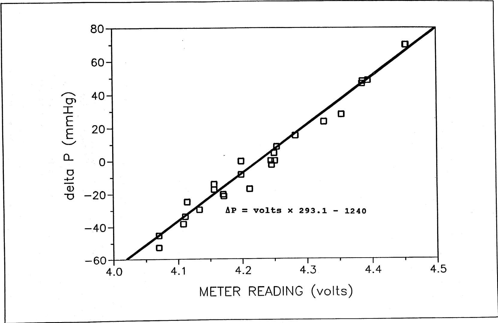
Figure 5. Total gas meter calibration
