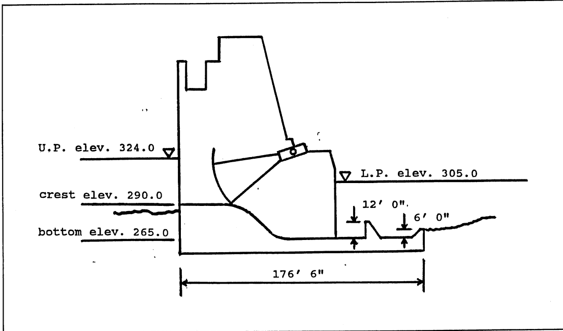
Figure B8. Profile view of Smithland Lock and Dam
