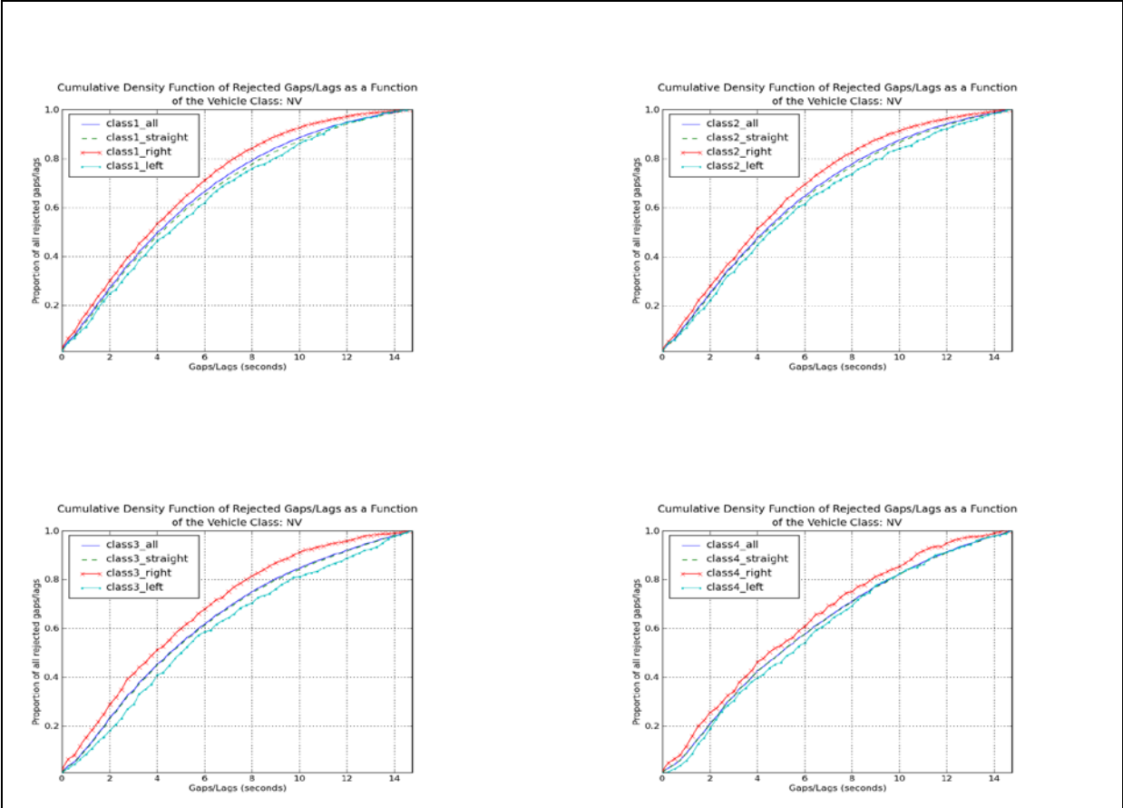
Figure 37. Gap rejection cumulative distribution plots for the NV intersection as a function of vehicle class and maneuver.
