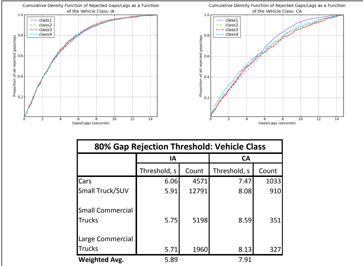
Figure 26. Gap rejection cumulative distribution plots for “T” intersections as a function of vehicle class.
