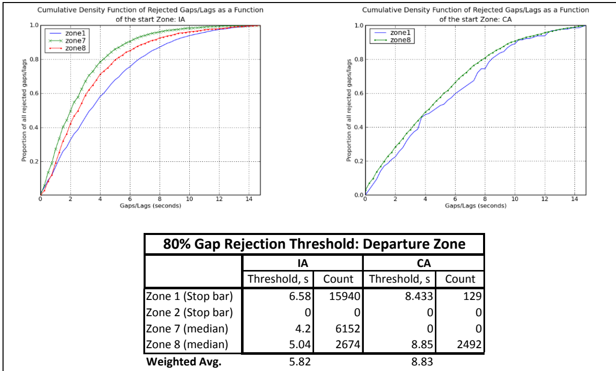
Figure 25. Gap rejection cumulative distribution plots for “T” intersections as a function of departure zone.
