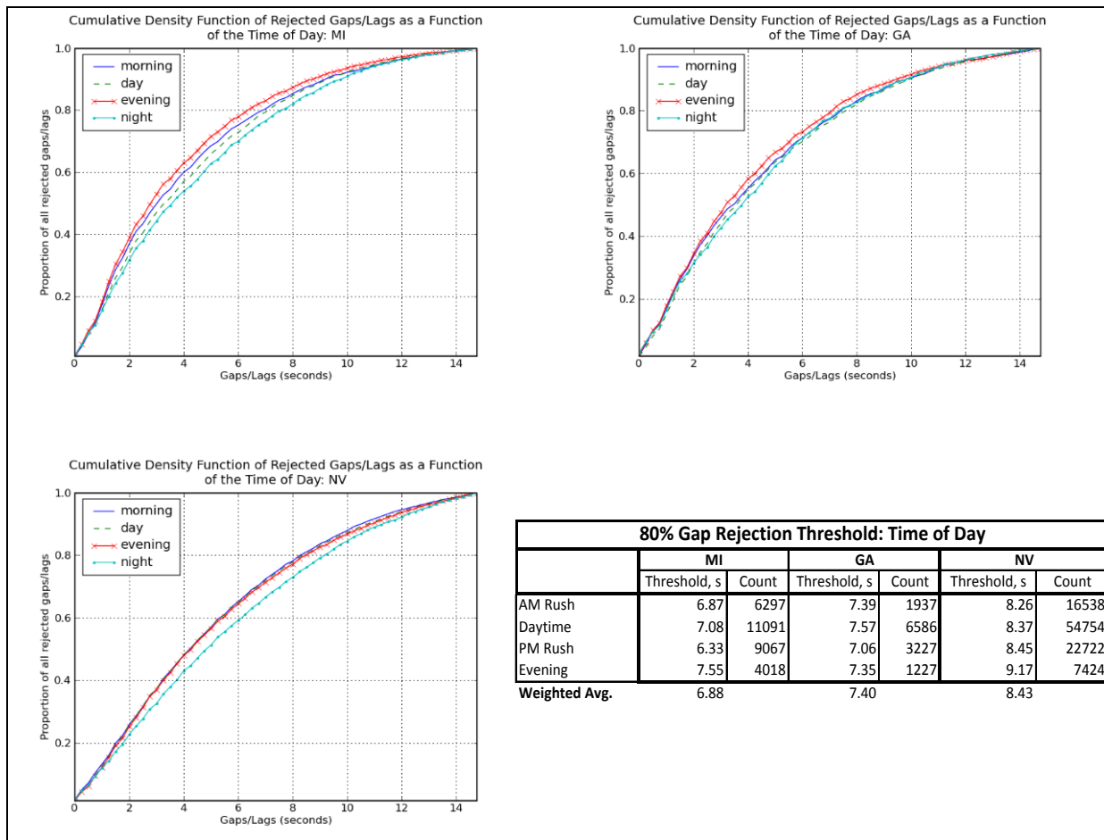
Figure 29. Gap rejection cumulative distribution plots as a function of time of day for rural highway, thru-Stop non-median separated intersections.
