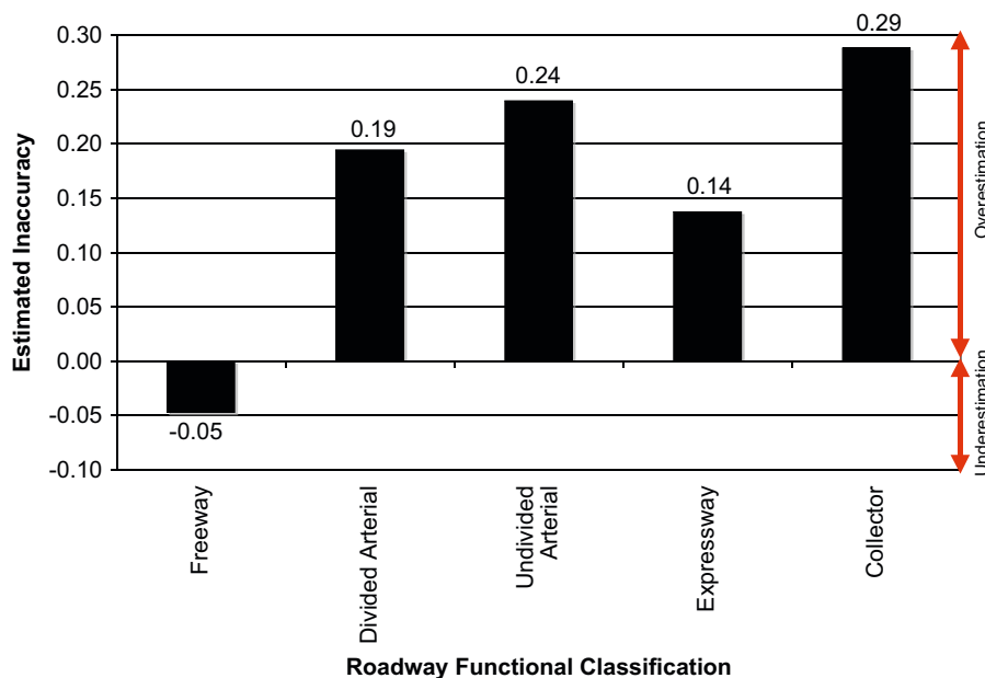
Fig. 6. Estimated average inaccuracy by roadway functional classification.
