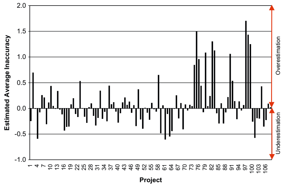
Fig. 3. Estimated average inaccuracy by project.
