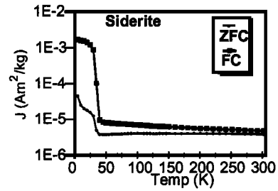
Figure 6. Low temperature remanence results for a siderite powder, as in Fig. 3.
